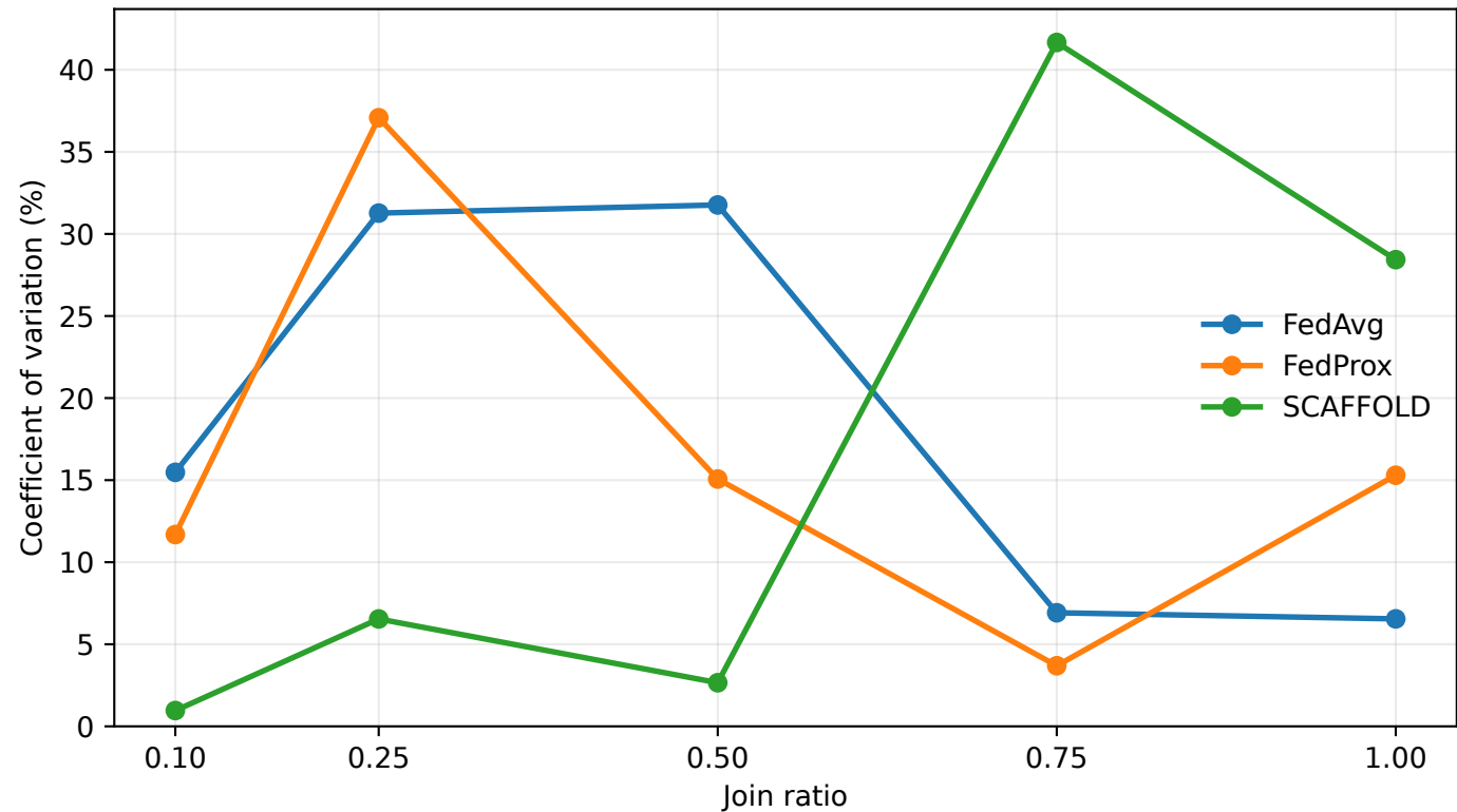
Stability across repetitions: Estimated energy (kJ)
