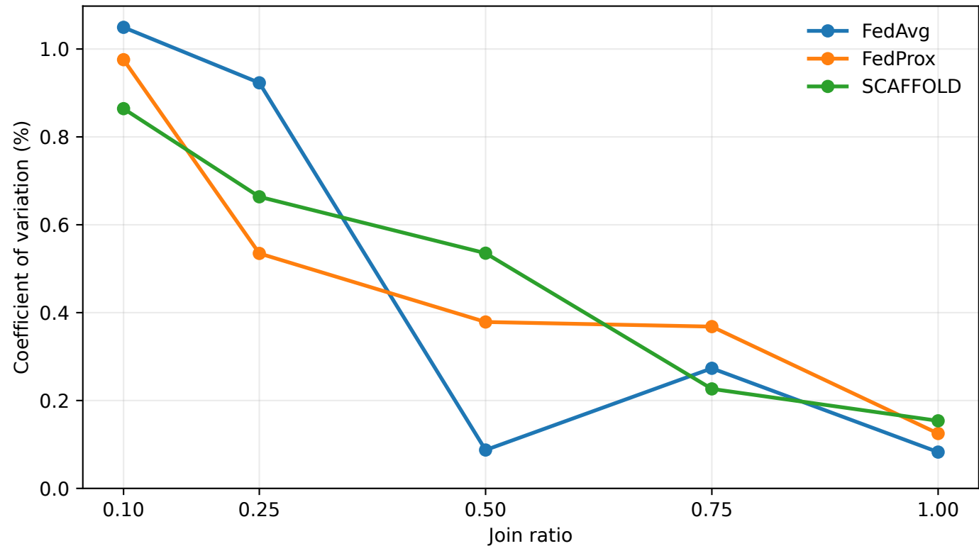
Stability across repetitions: Best accuracy
