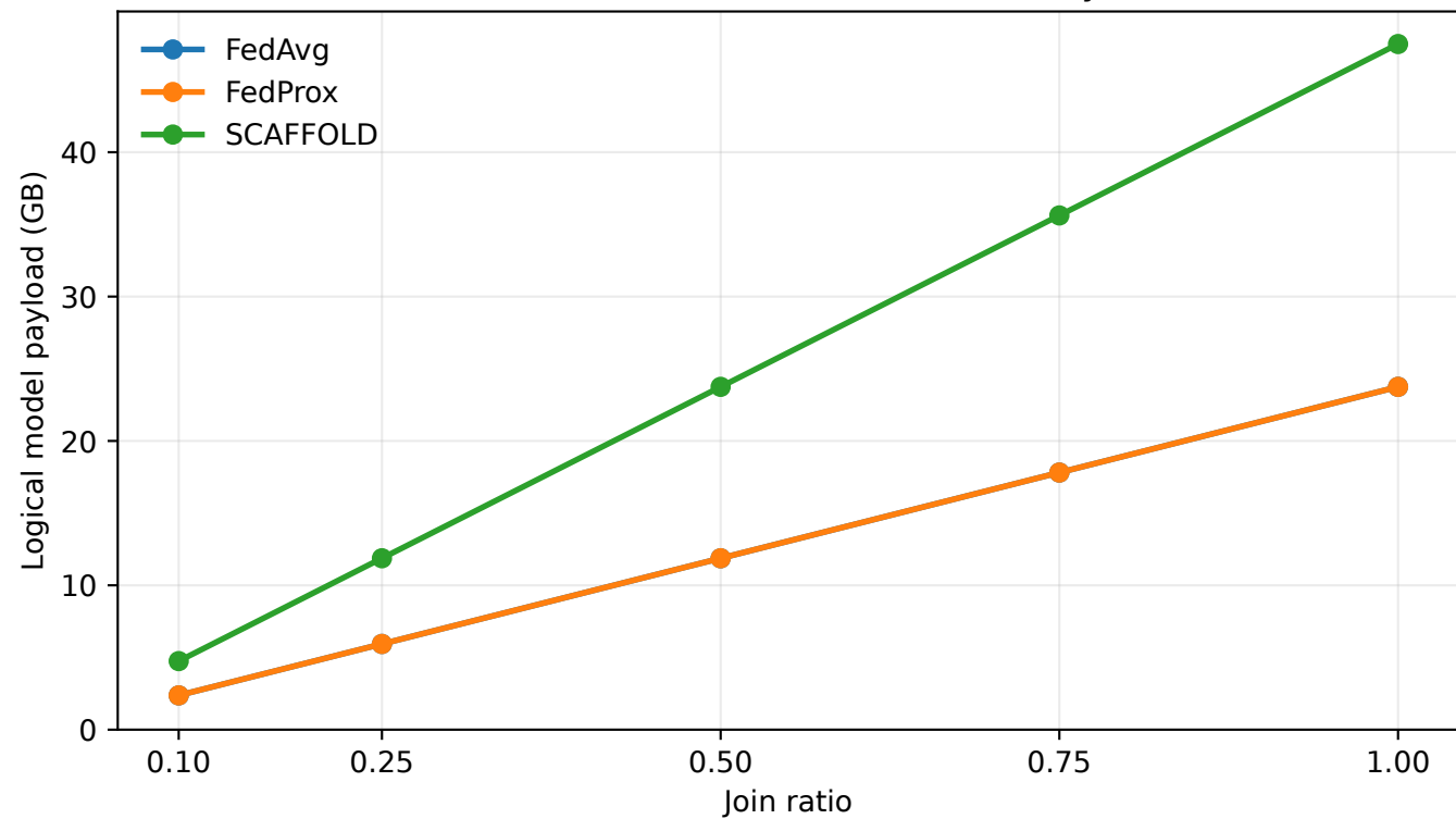
Selected-client communication scenario (51 cycles, FP32)
