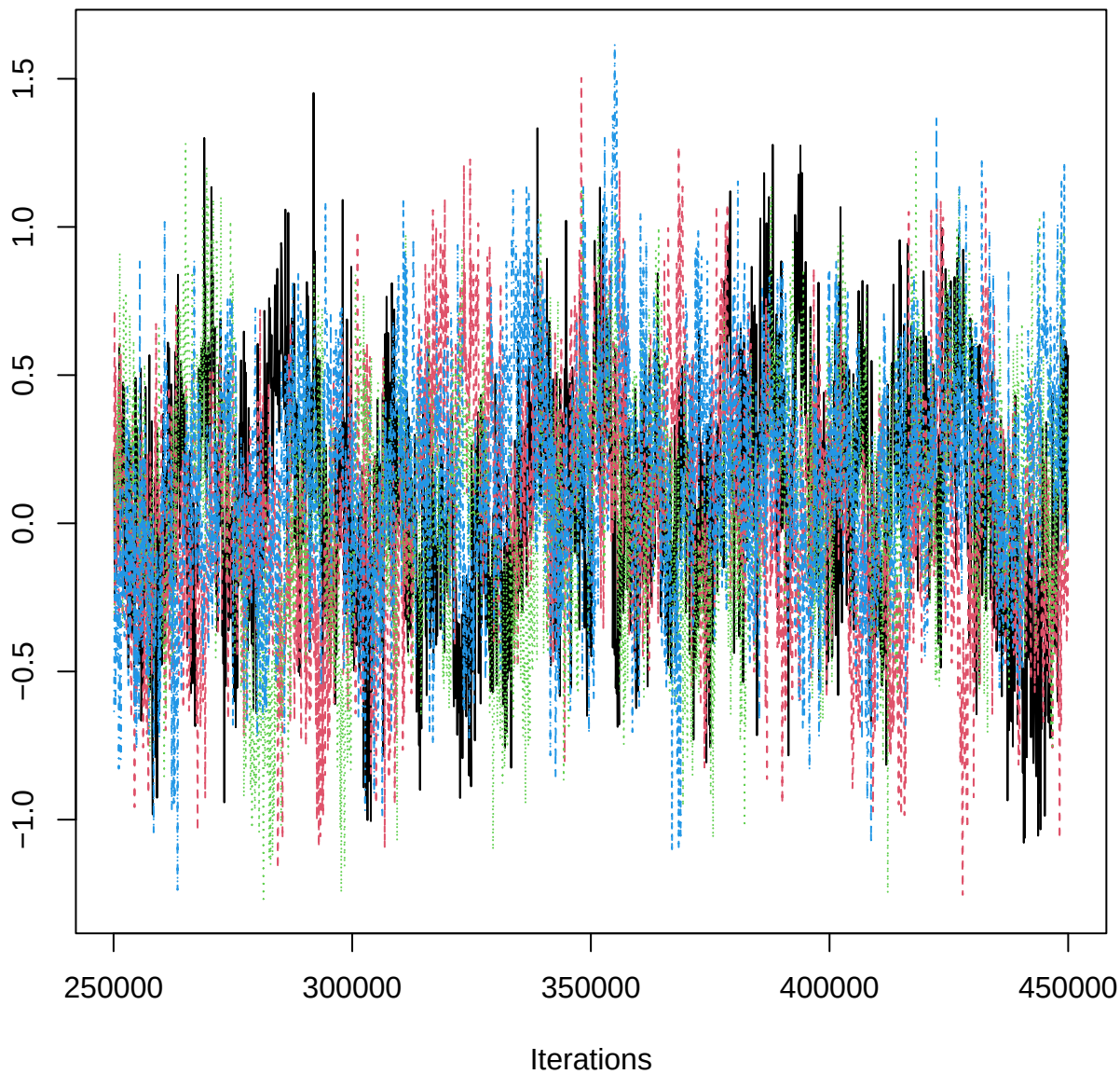
Traceplot – B[aspect_classN (C11), THO_n (S10)]
