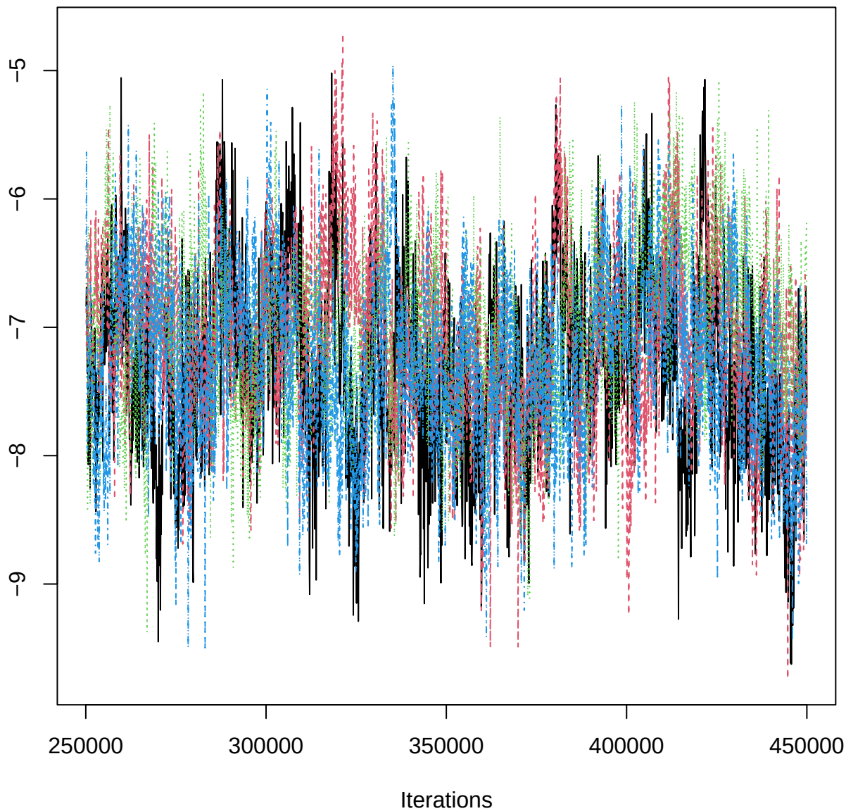
Traceplot – B[pH (C4), BOJ_n (S4)]
