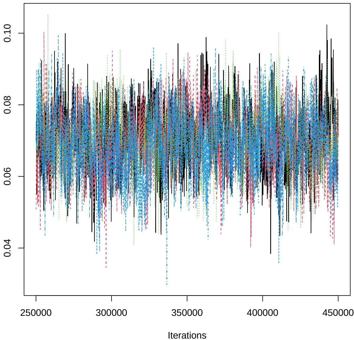
Traceplot – B[Clay (C5), PET_n (S12)]
