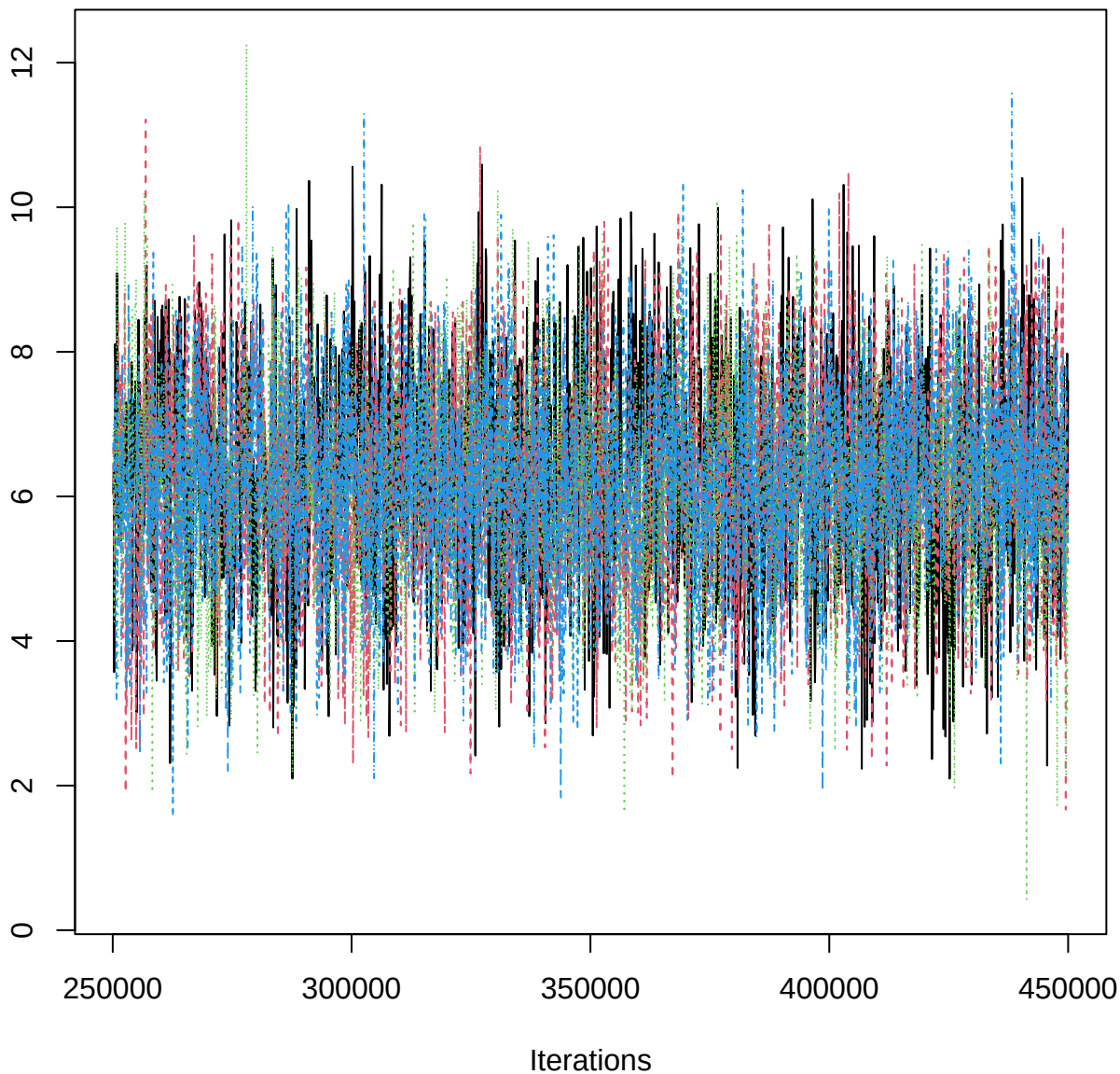
Traceplot – B[(Intercept) (C1), SAB_n (S8)]
