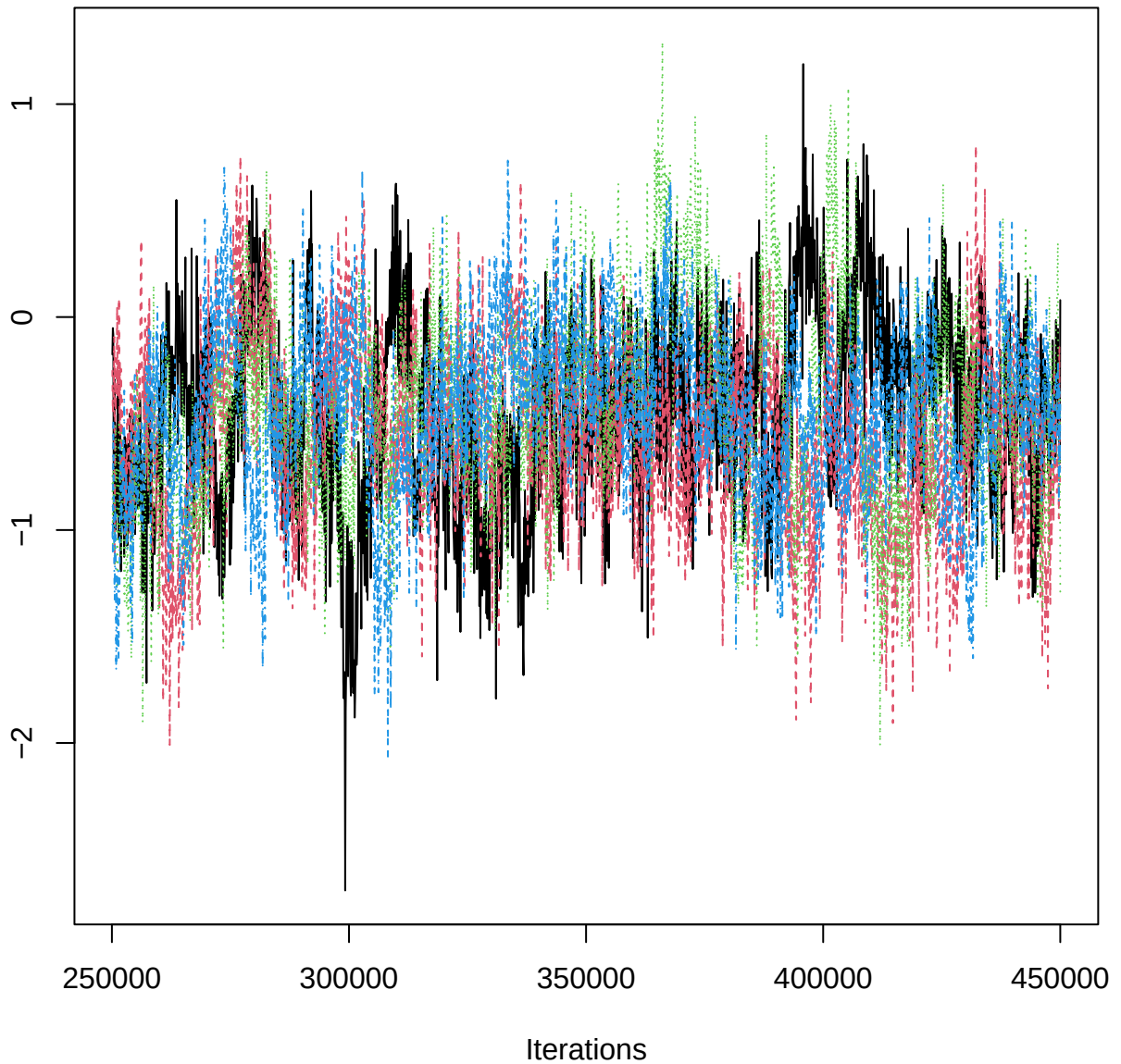
Traceplot – B[aspect_classSE (C15), HEG_n (S3)]
