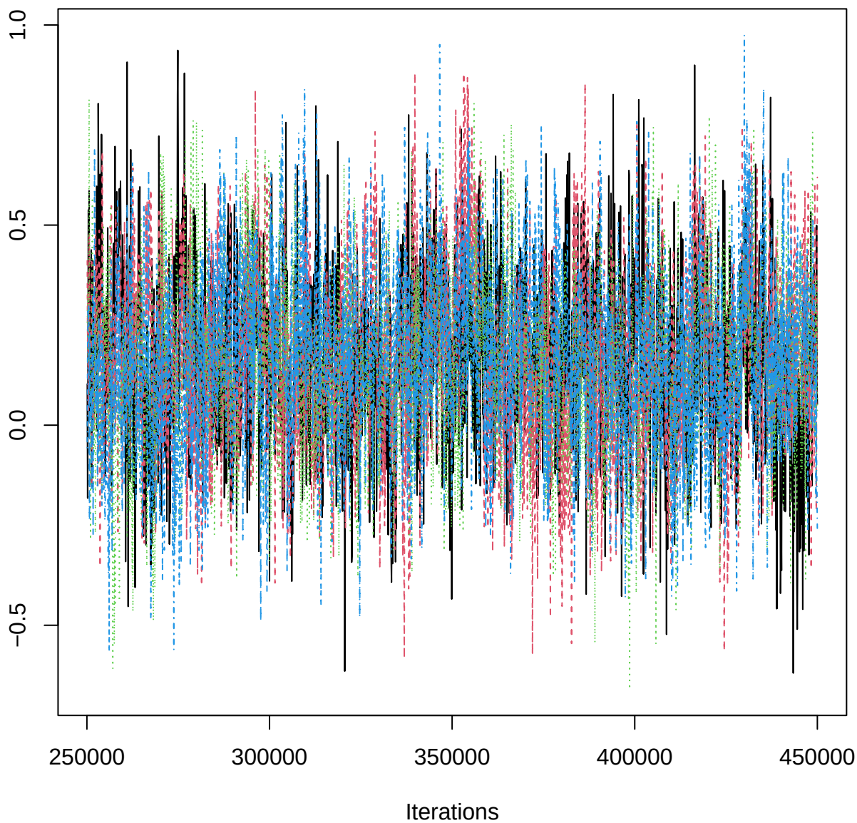
Traceplot – B[aspect_classS (C14), EPB_n (S6)]
