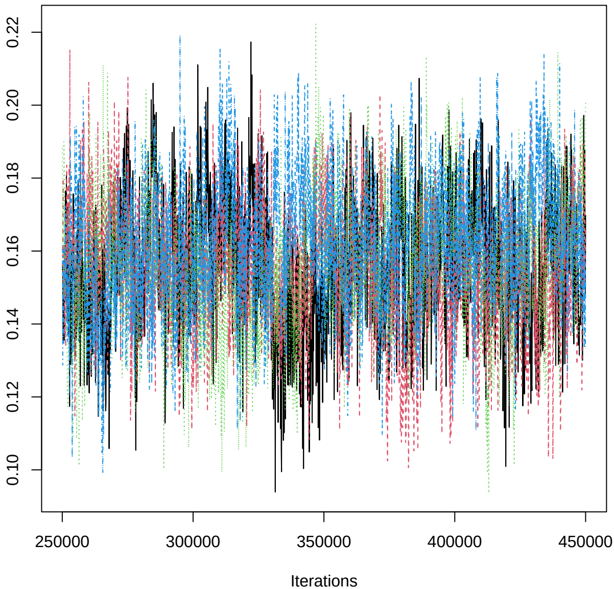
Traceplot – B[slope (C9), ERS_n (S2)]
