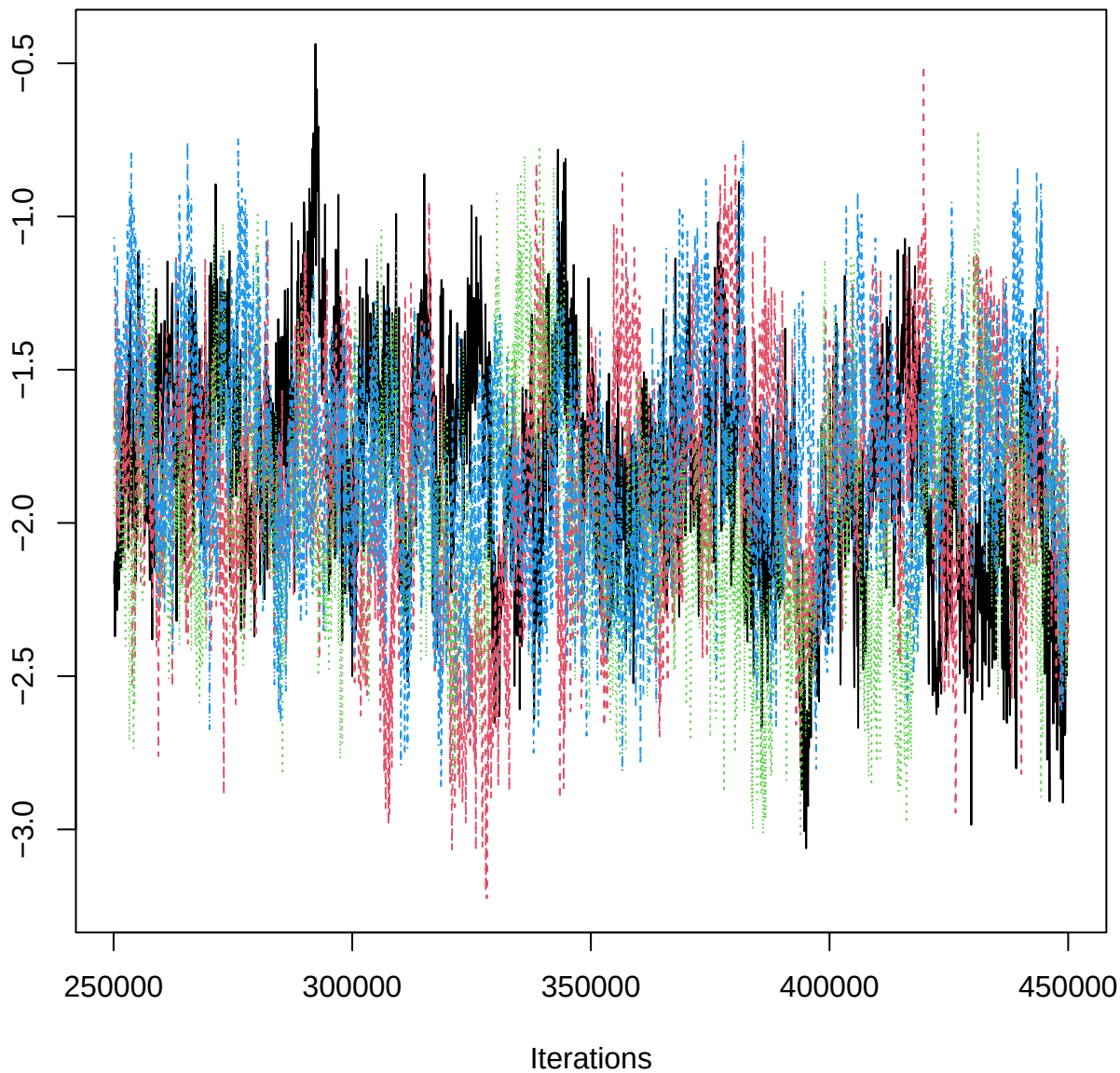
Traceplot – B[rtp (C7), THO_n (S10)]
