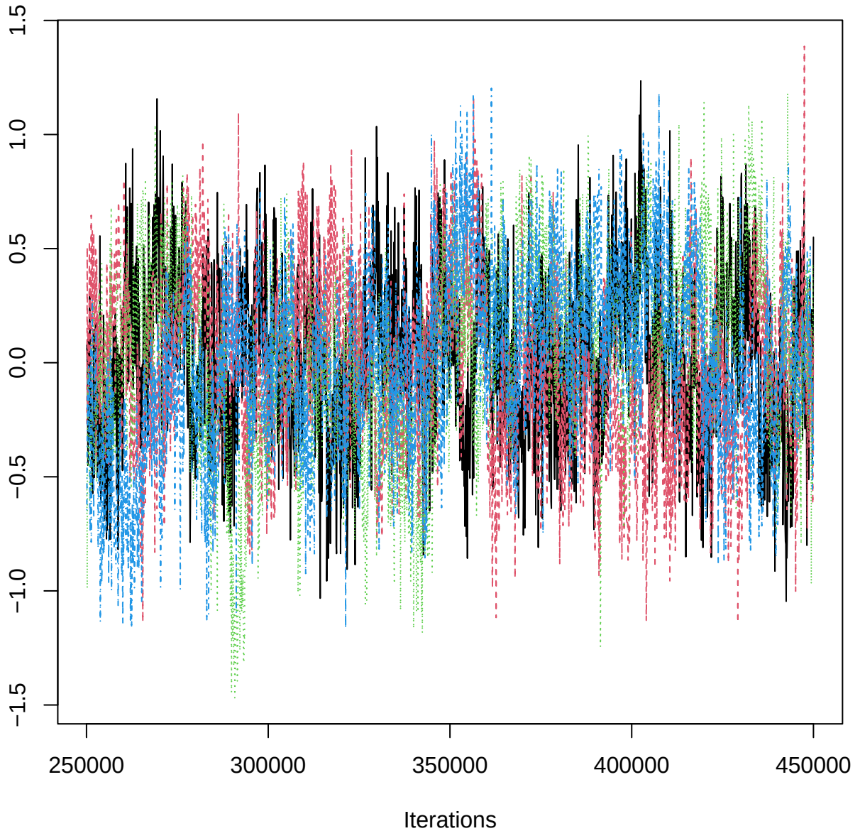
Traceplot – B[aspect_classW (C17), PRP_n (S11)]
