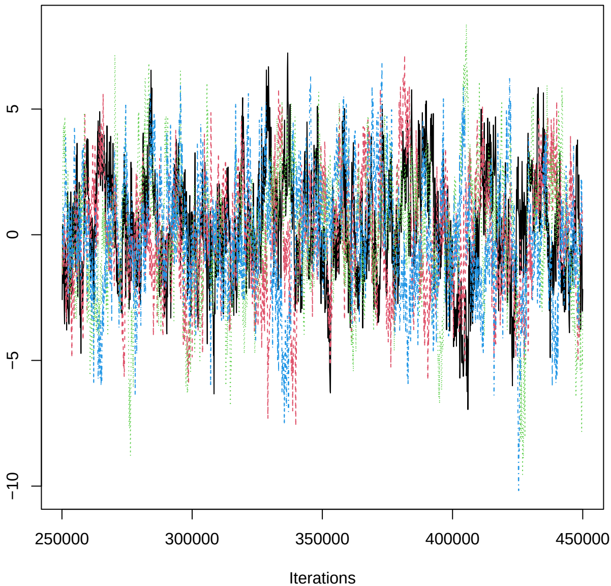
Traceplot – B[aspect_classFlat (C10), BOJ_n (S4)]
