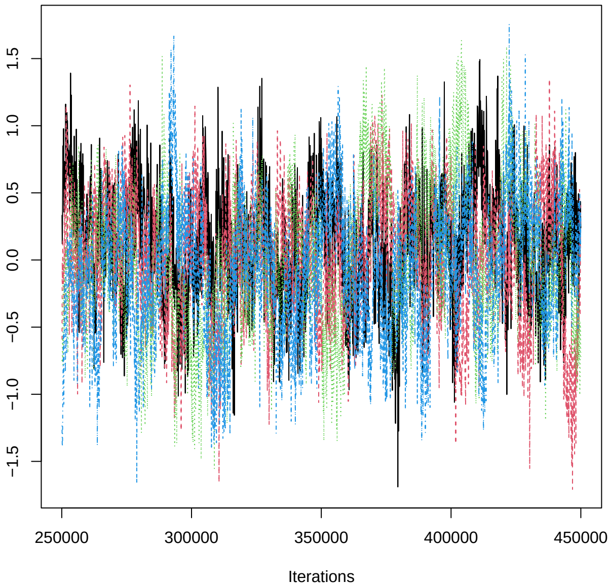
Traceplot – B[aspect_classNE (C12), EPR_n (S7)]
