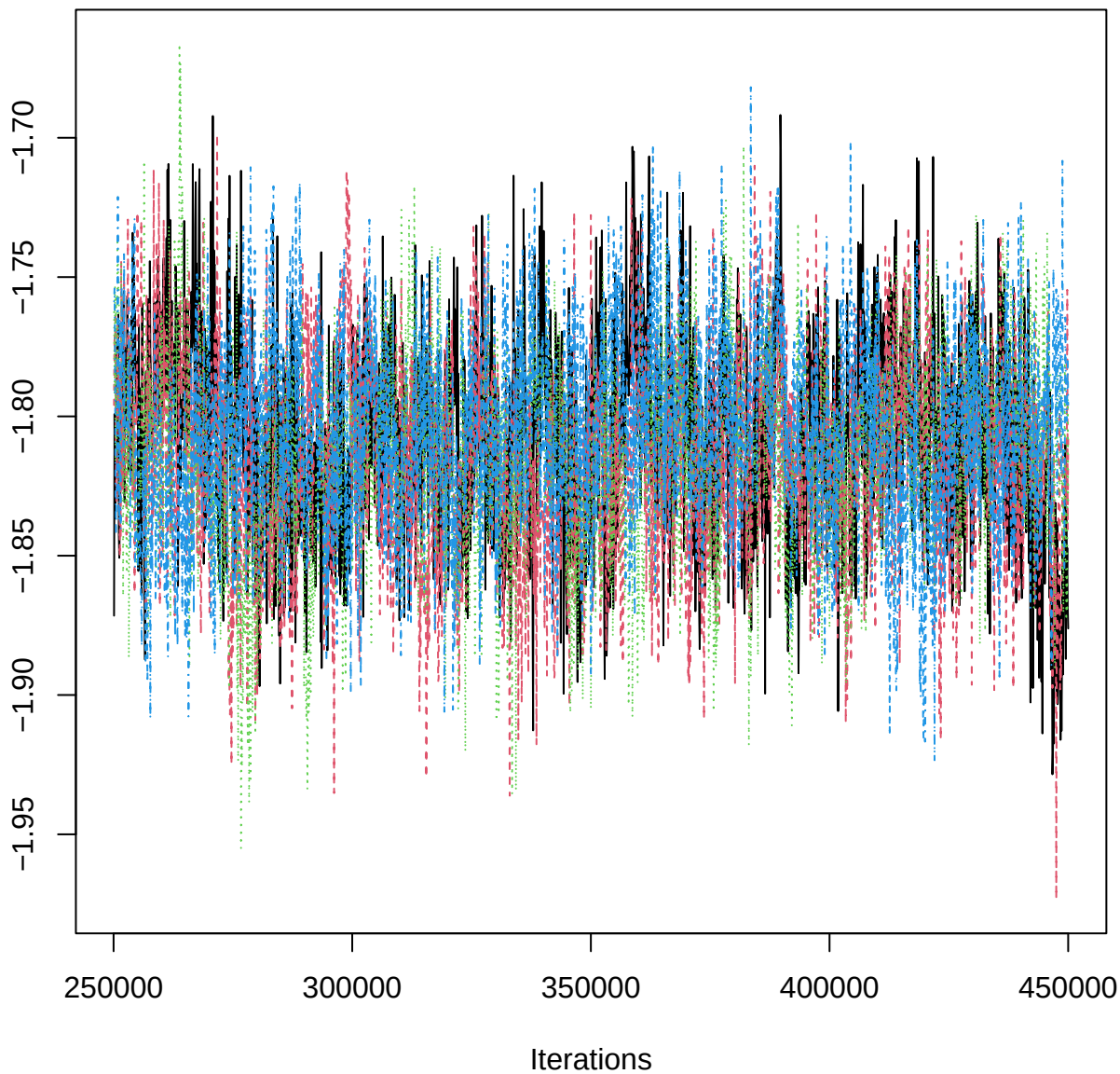
Traceplot – B[MAT (C3), EPN_n (S9)]
