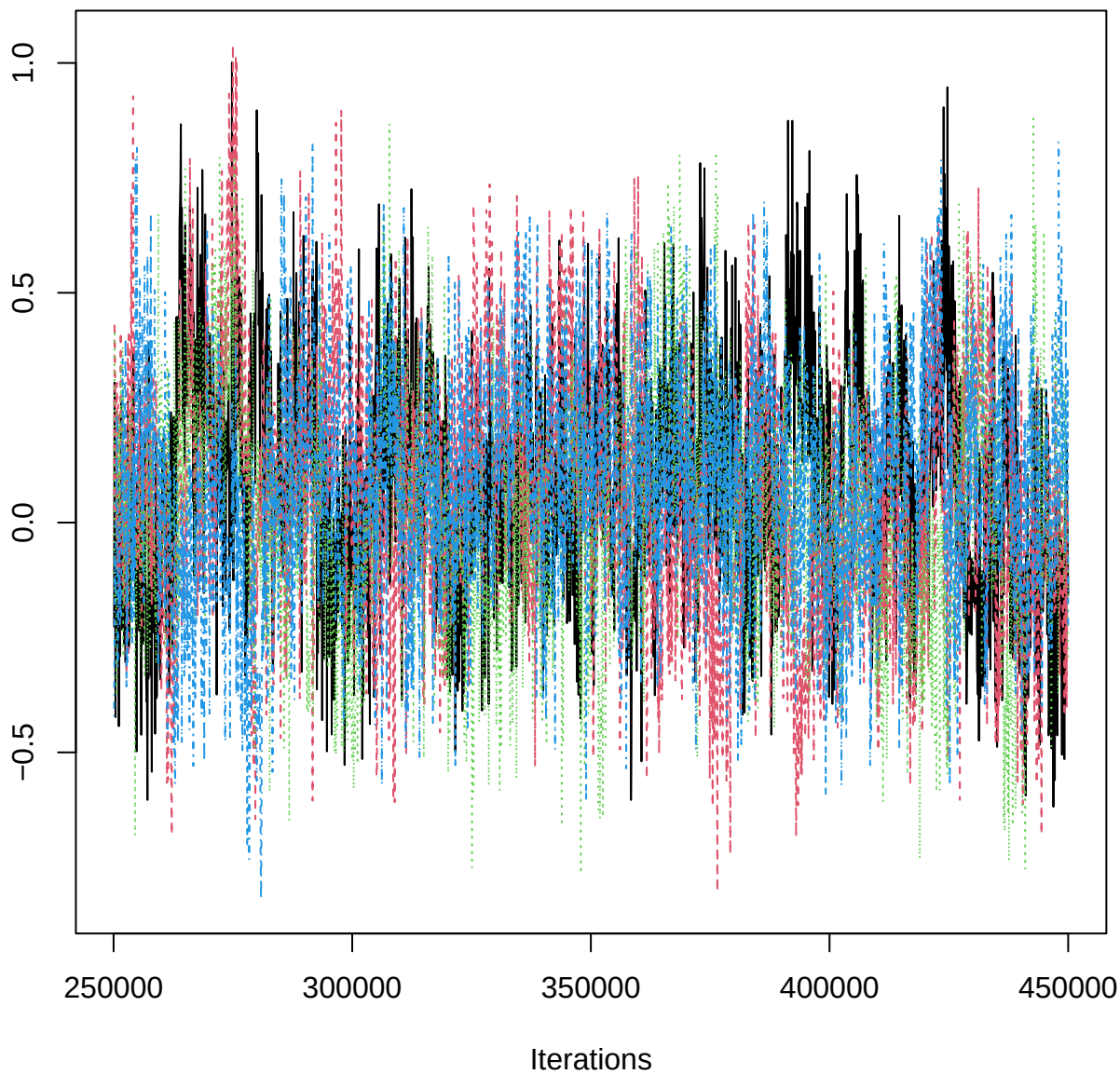
Traceplot – B[aspect_classNE (C12), ERS_n (S2)]
