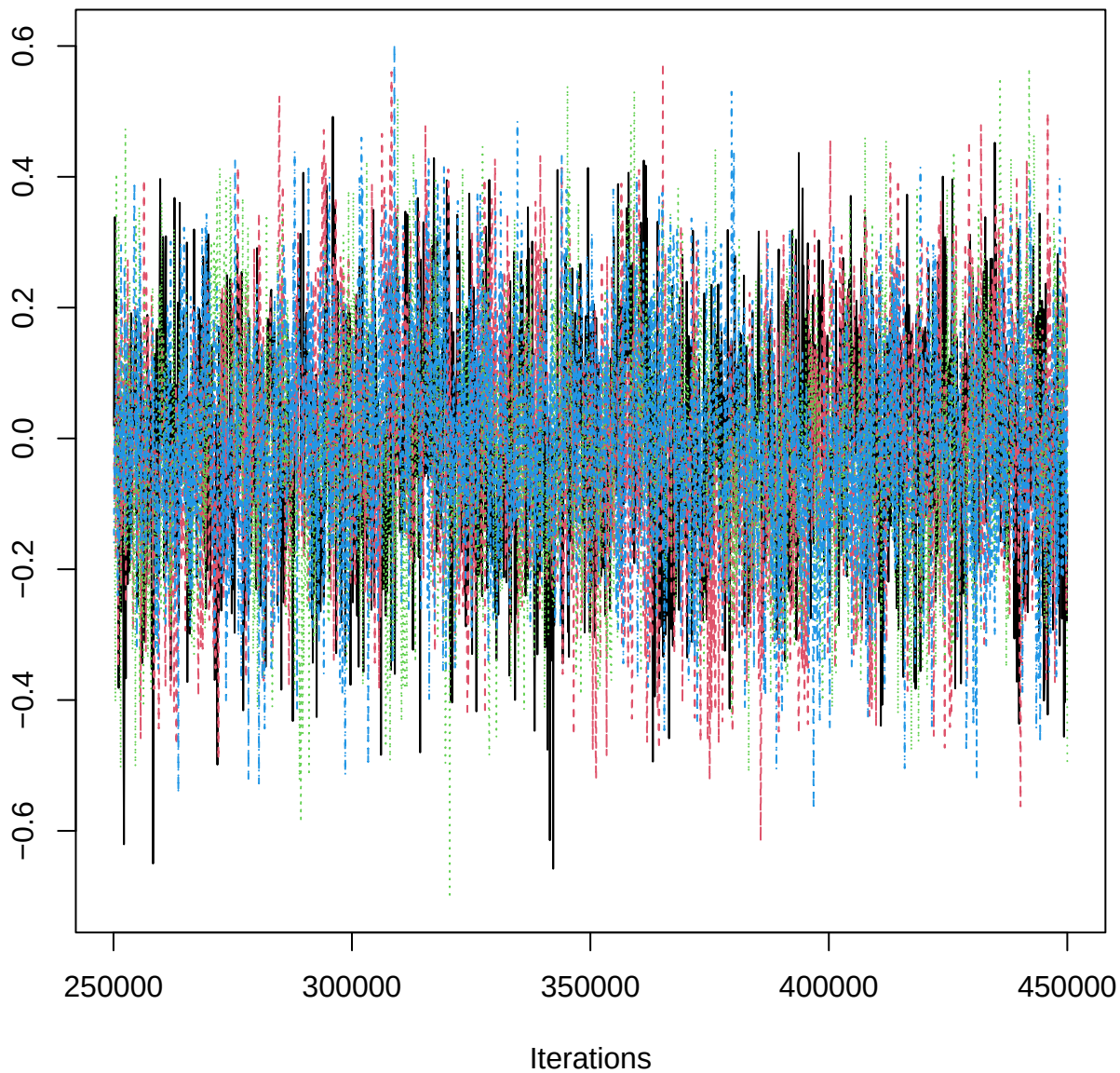
Traceplot – B[aspect_classSE (C15), BOP_n (S5)]
