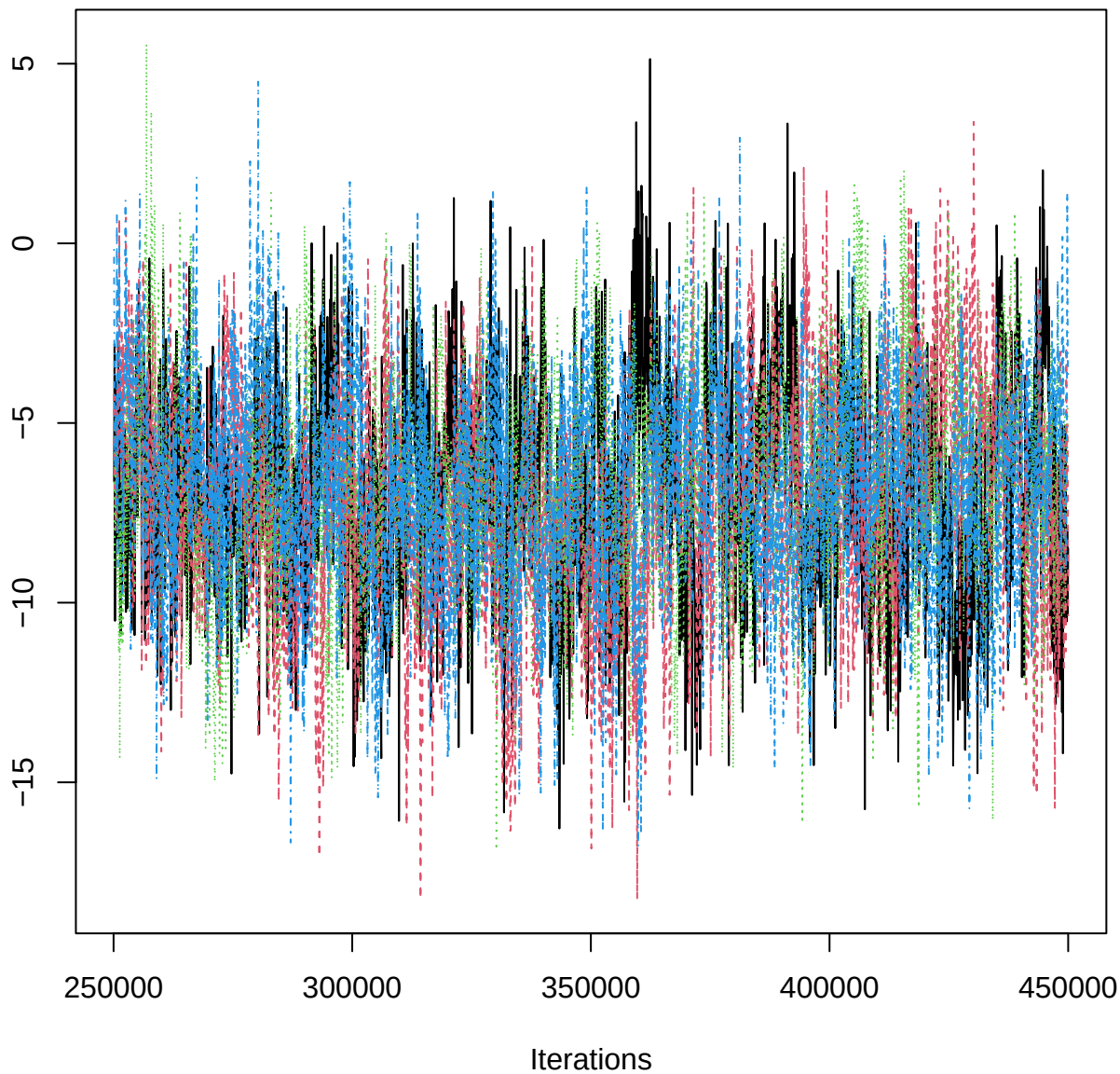
Traceplot – B[(Intercept) (C1), PET_n (S12)]
