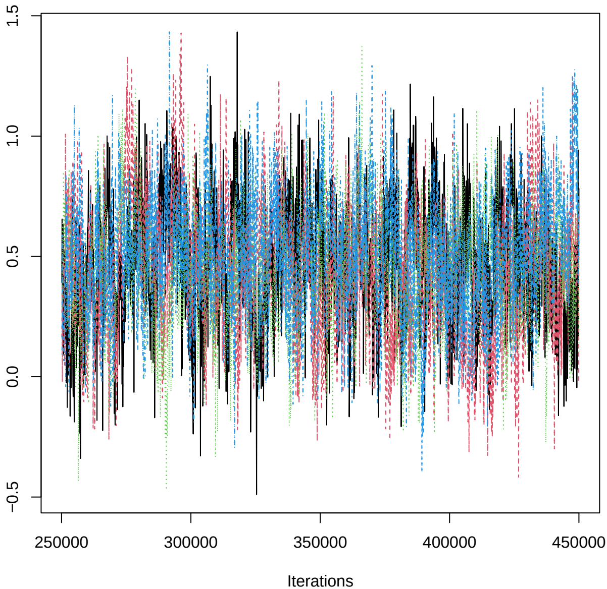
Traceplot – B[aspect_classSE (C15), ERS_n (S2)]
