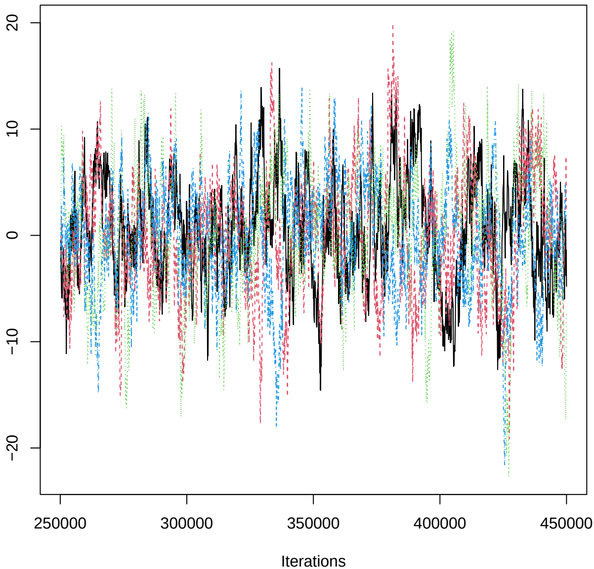
Traceplot – B[aspect_classFlat (C10), HEG_n (S3)]
