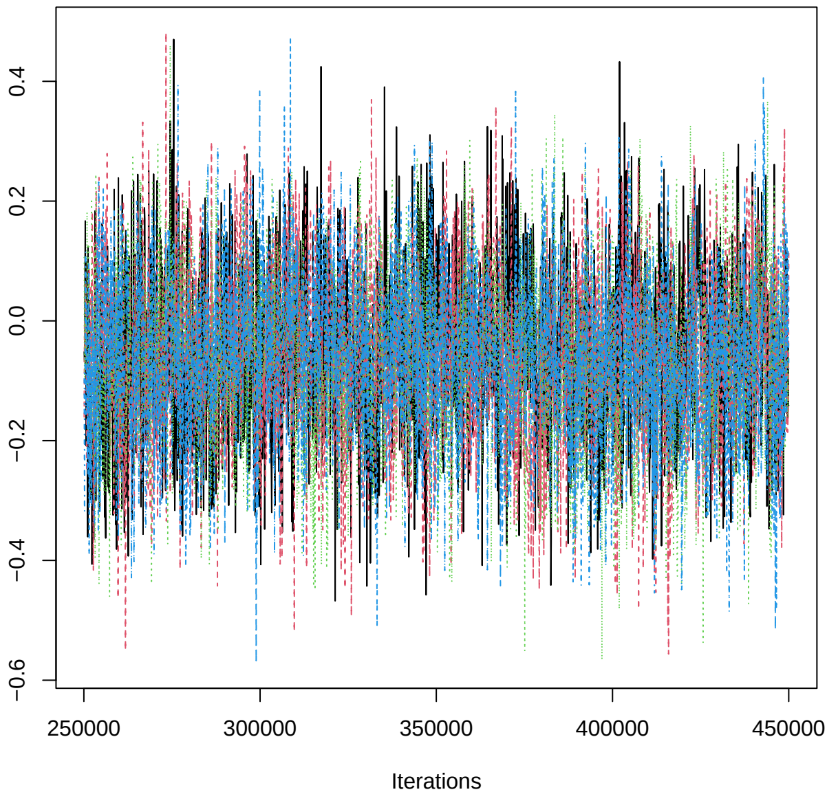
Traceplot – B[aspect_classN (C11), SAB_n (S8)]
