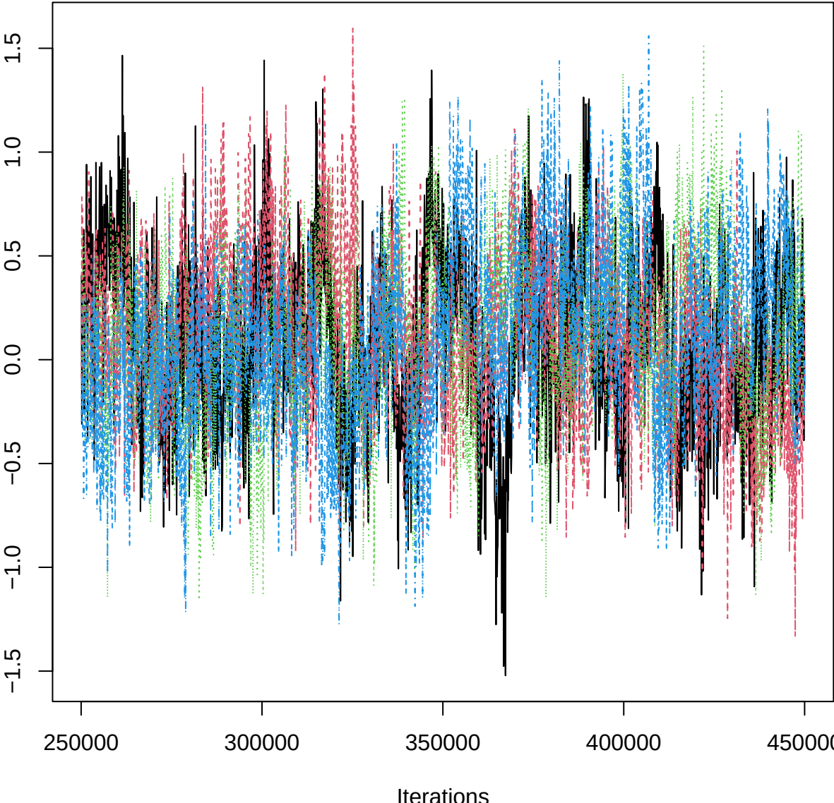
Traceplot – B[aspect_classNE (C12), THO_n (S10)]
