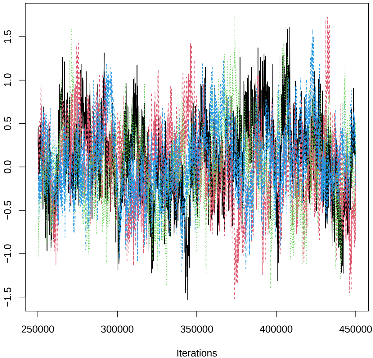
Traceplot – B[aspect_classNE (C12), HEG_n (S3)]
