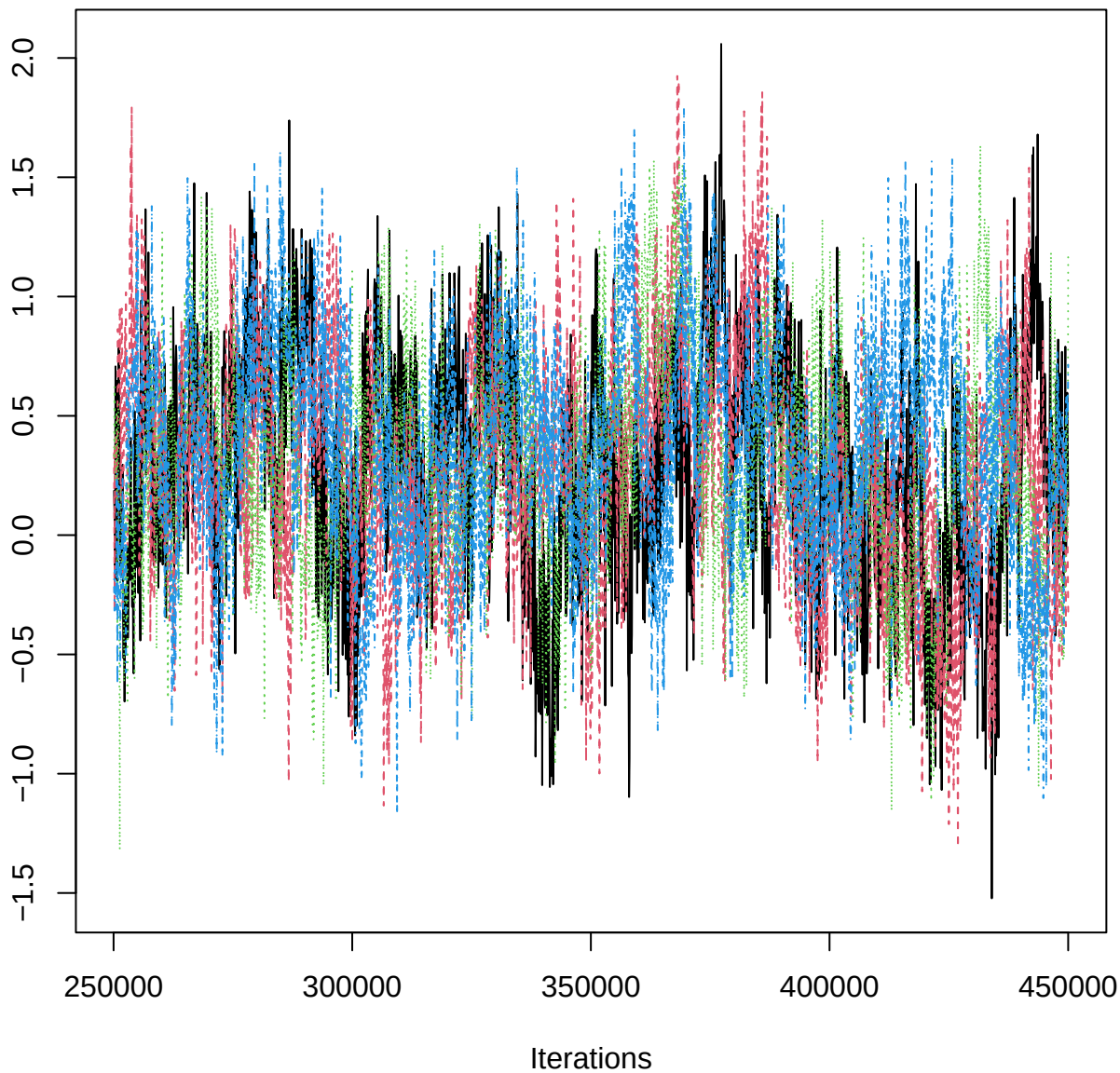
Traceplot – B[aspect_classW (C17), PIG_n (S14)]
