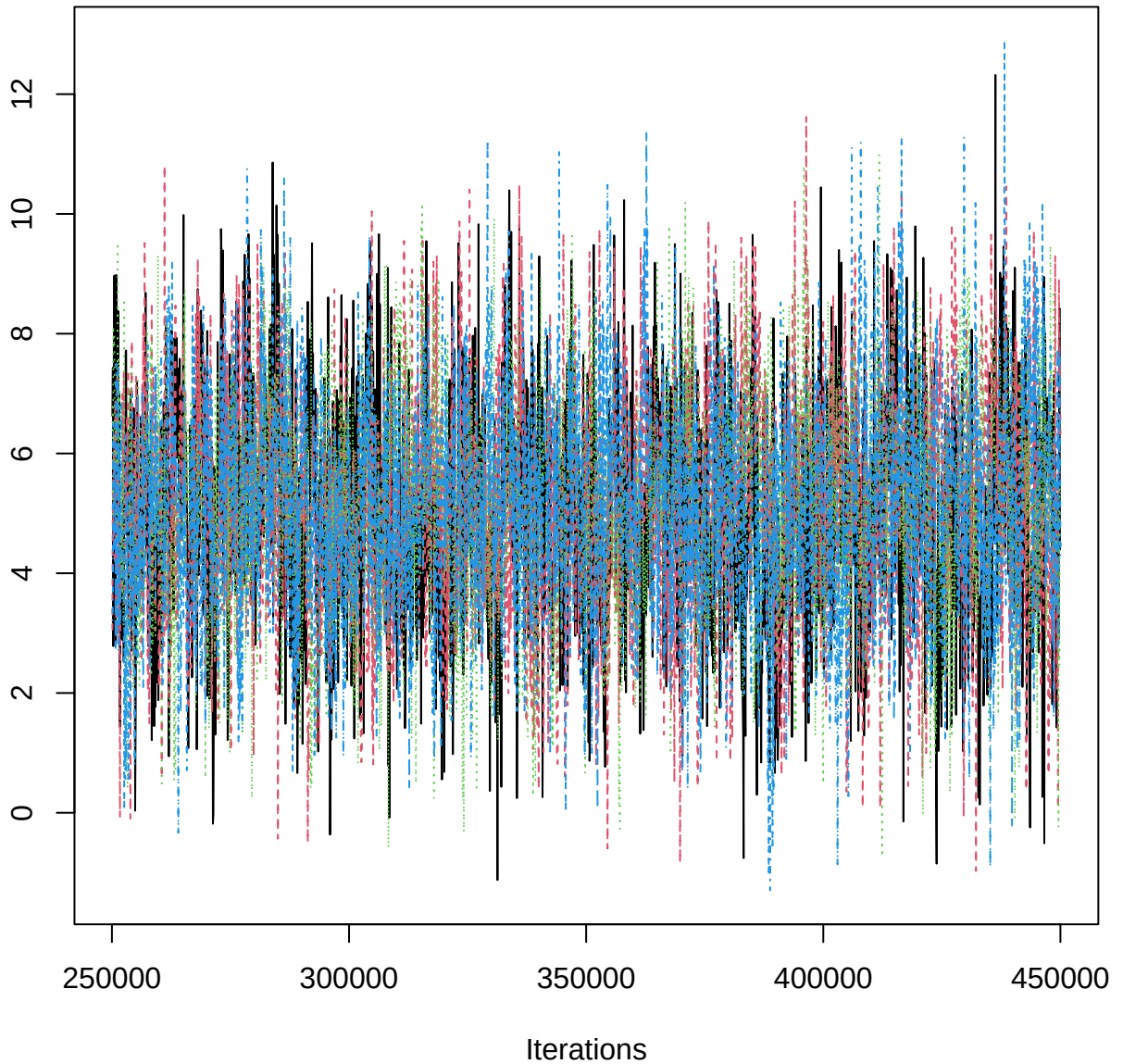
Traceplot – B[(Intercept) (C1), BOP_n (S5)]
