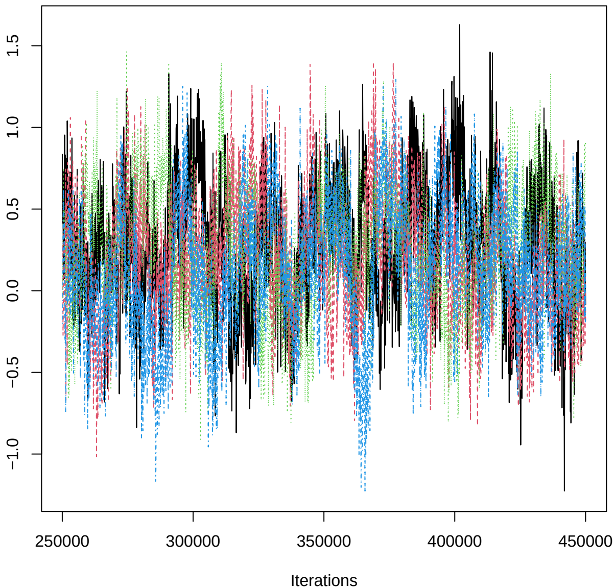
Traceplot – B[aspect_classNW (C13), PRP_n (S11)]
