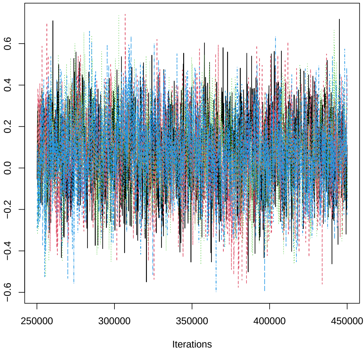
Traceplot – B[aspect_classS (C14), BOP_n (S5)]
