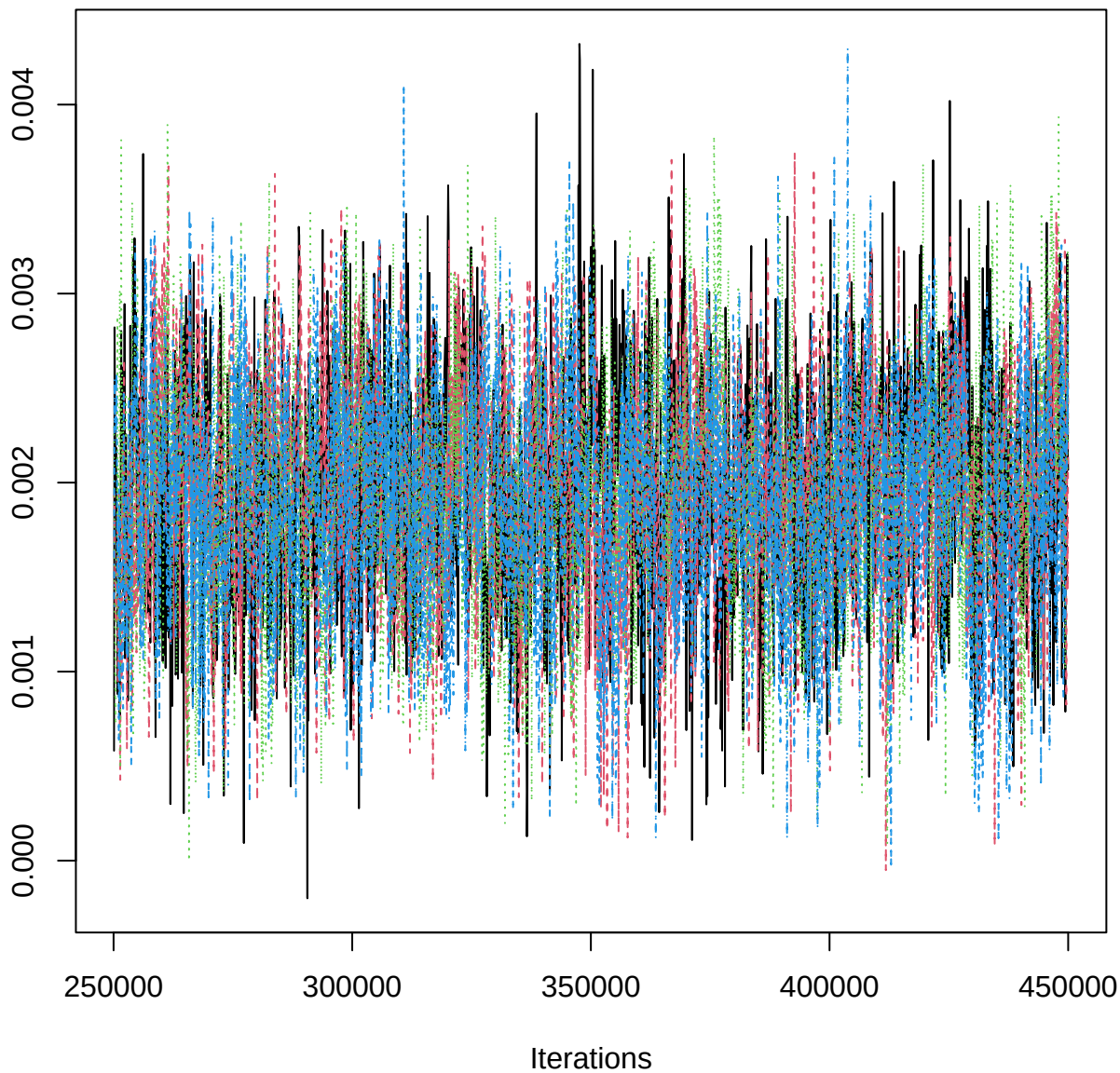
Traceplot – B[MAP (C2), EPB_n (S6)]
