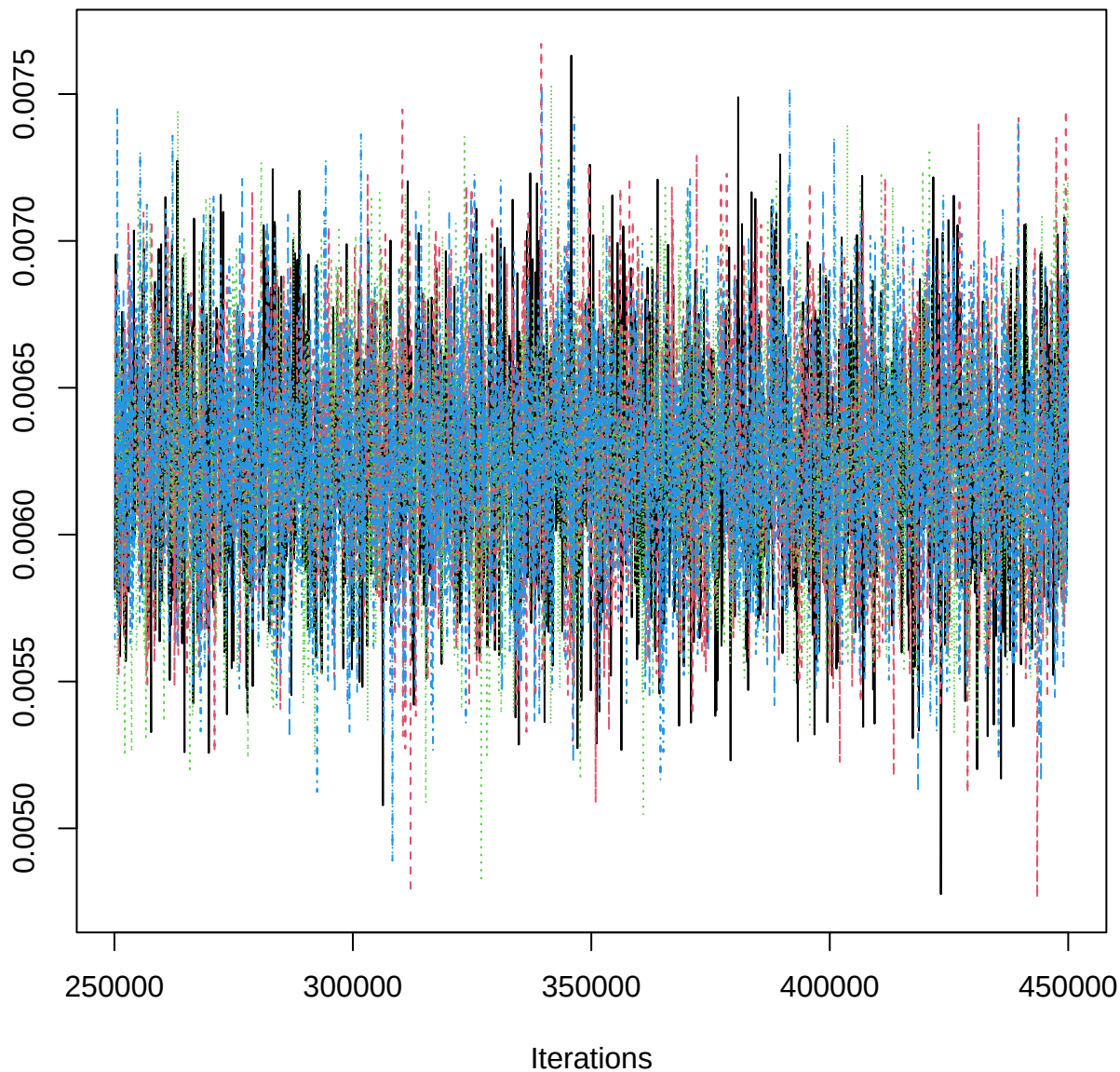
Traceplot – B[MAP (C2), SAB_n (S8)]
