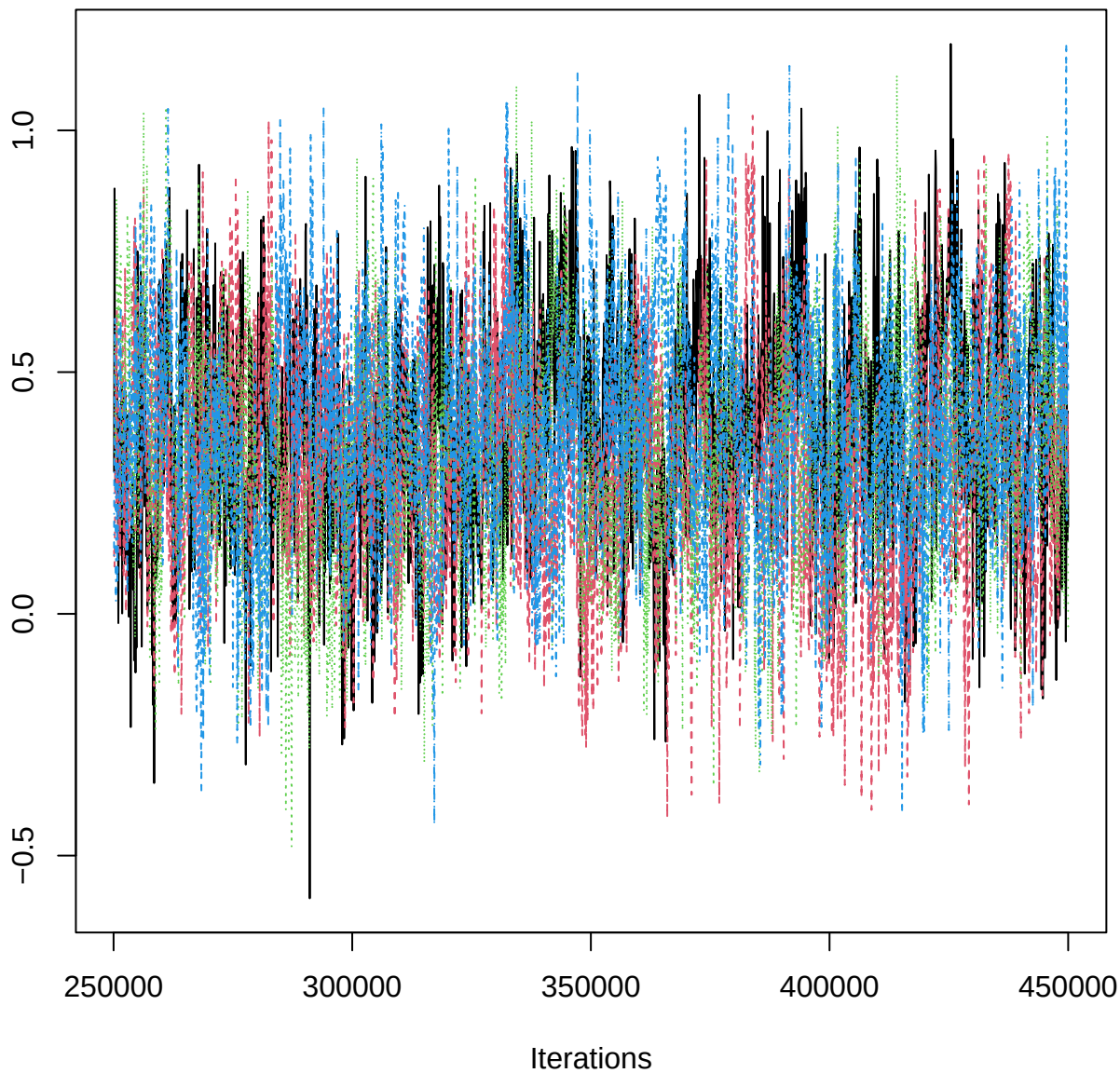
Traceplot – B[aspect_classSE (C15), ERR_n (S1)]
