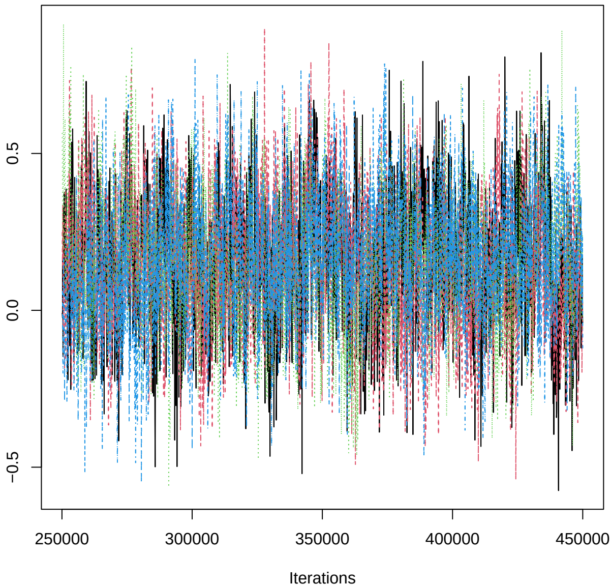
Traceplot – B[aspect_classSE (C15), EPB_n (S6)]
