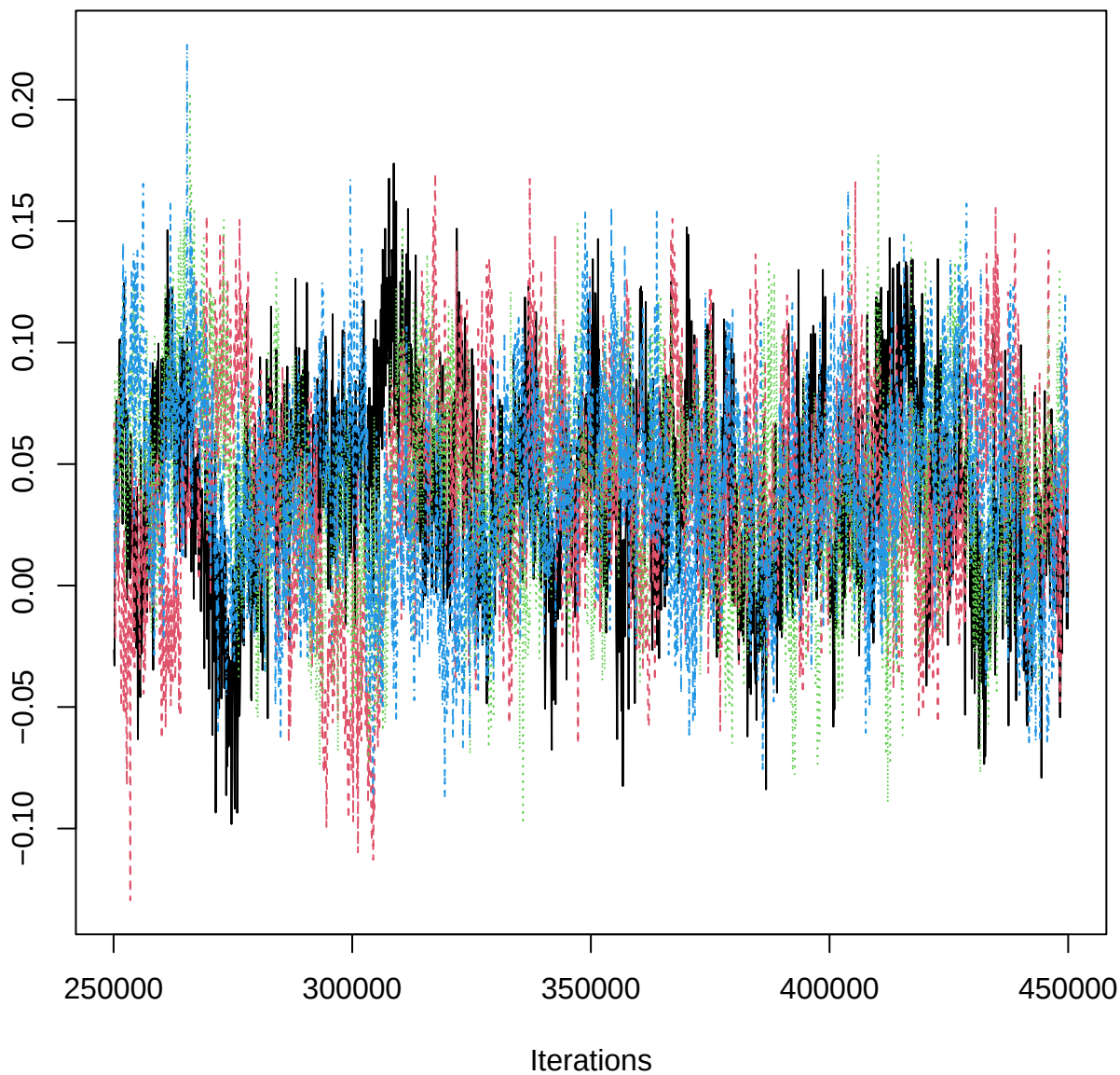
Traceplot – B[twi (C8), PIG_n (S14)]
