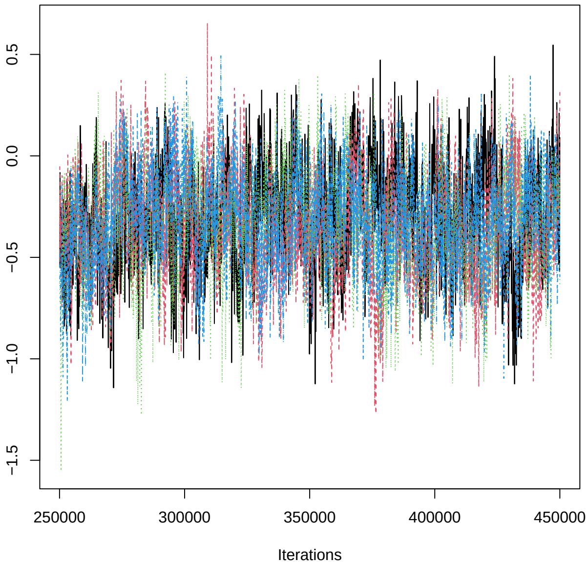
Traceplot – B[aspect_classSW (C16), ERS_n (S2)]
