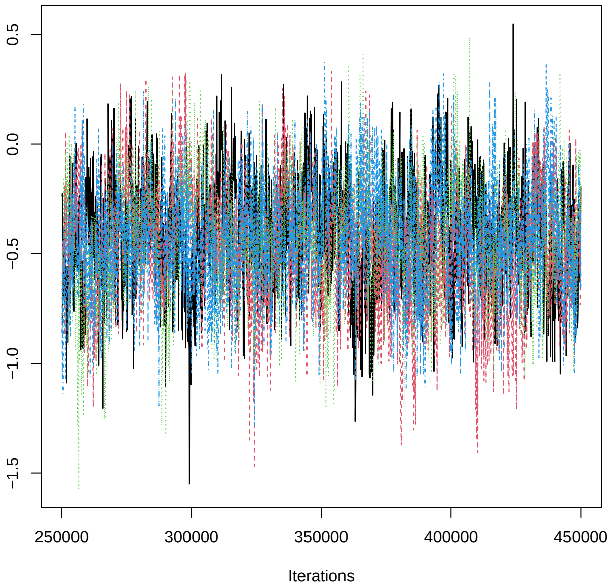
Traceplot – B[aspect_classSE (C15), BOJ_n (S4)]
