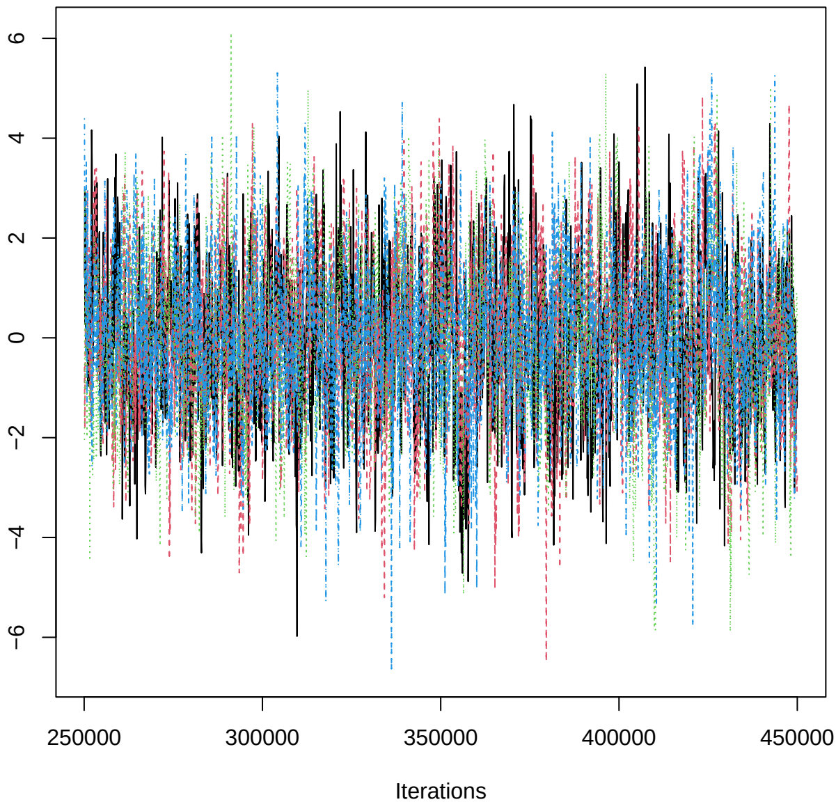
Traceplot – B[aspect_classFlat (C10), EPN_n (S9)]
