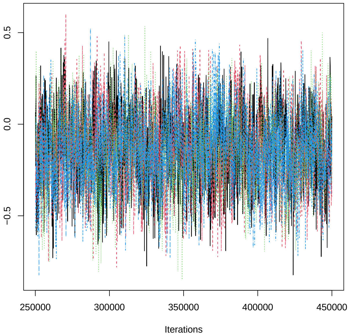
Traceplot – B[aspect_classNE (C12), EPN_n (S9)]
