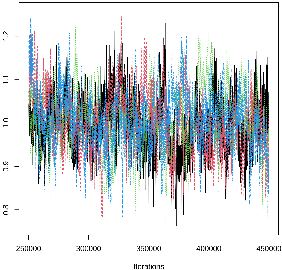
Traceplot – B[MAT (C3), PET_n (S12)]
