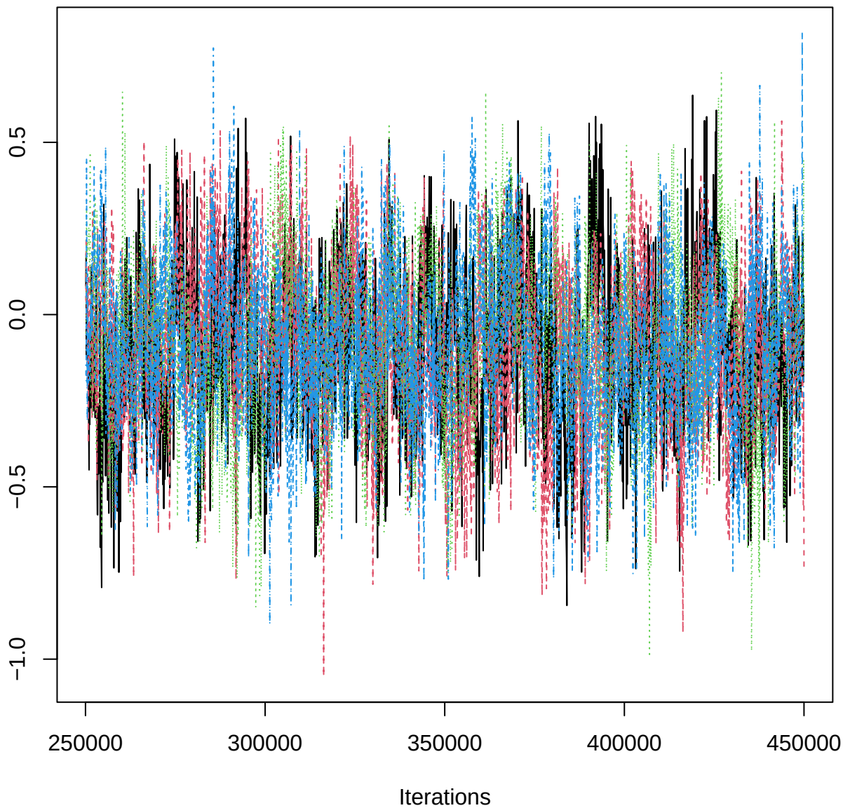
Traceplot – B[aspect_classNW (C13), ERR_n (S1)]
