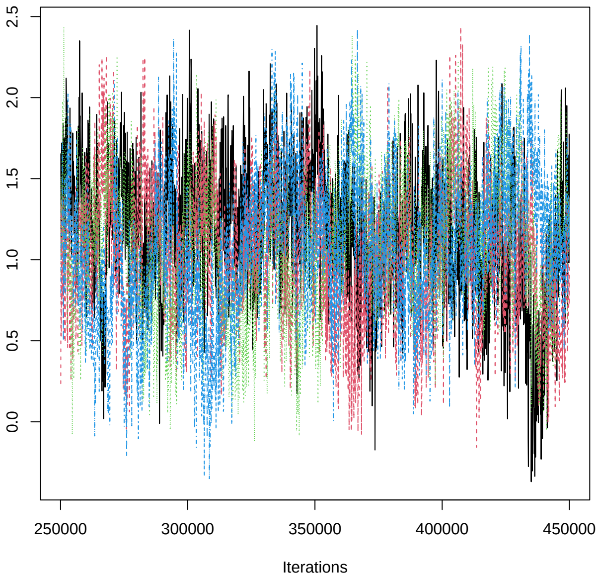
Traceplot – B[aspect_classW (C17), THO_n (S10)]
