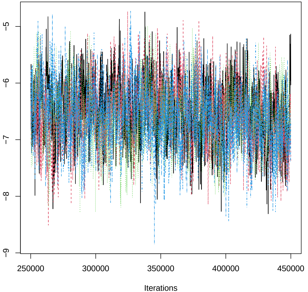
Traceplot – B[pH (C4), ERR_n (S1)]
