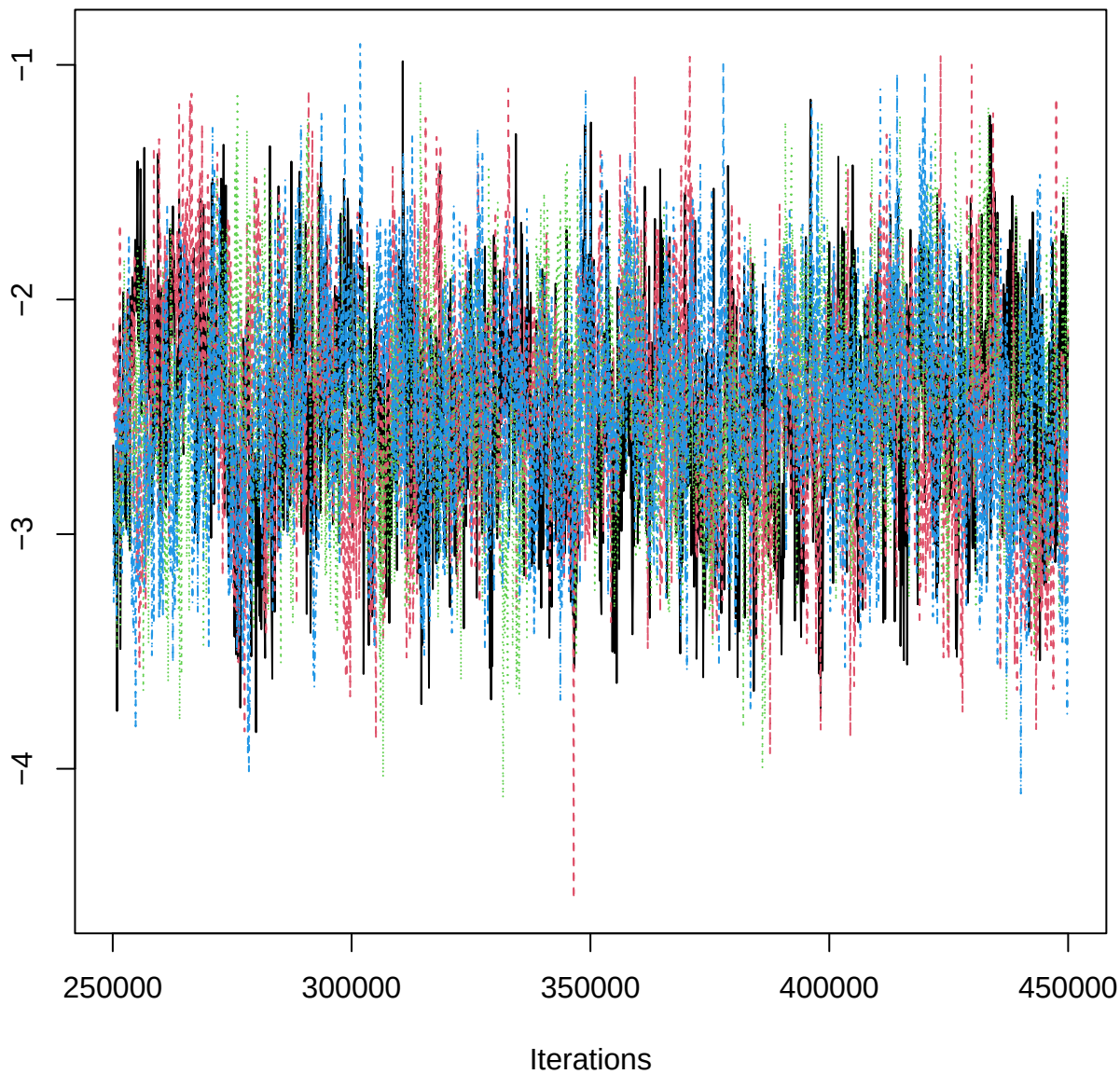
Traceplot – B[pH (C4), EPN_n (S9)]
