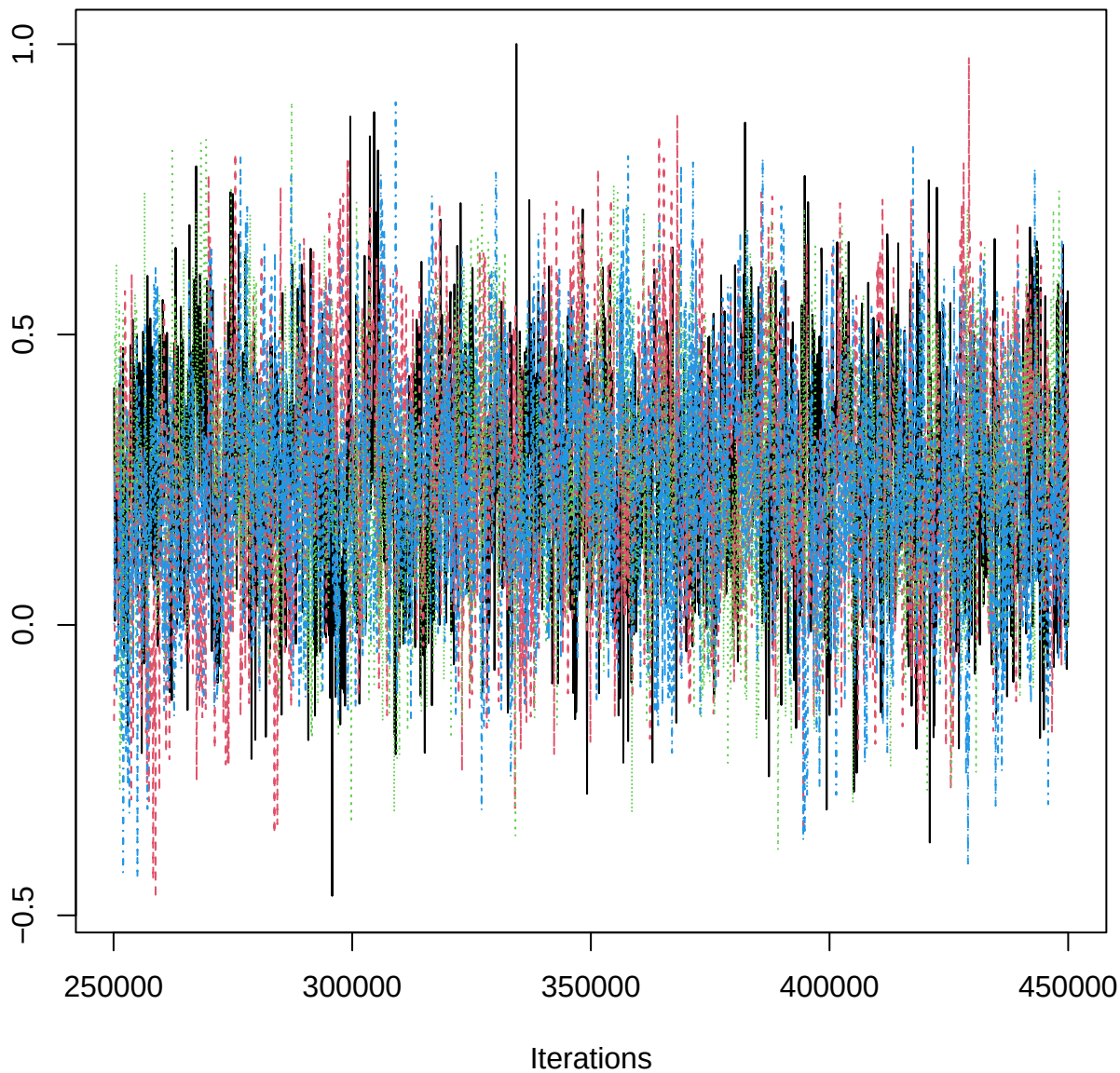
Traceplot – B[aspect_classSW (C16), EPN_n (S9)]
