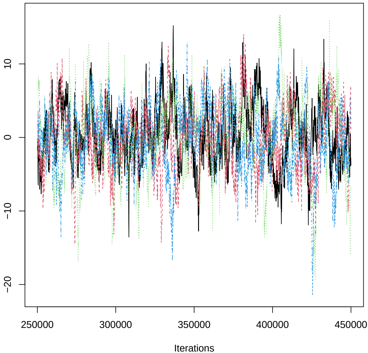
Traceplot – B[aspect_classFlat (C10), EPR_n (S7)]
