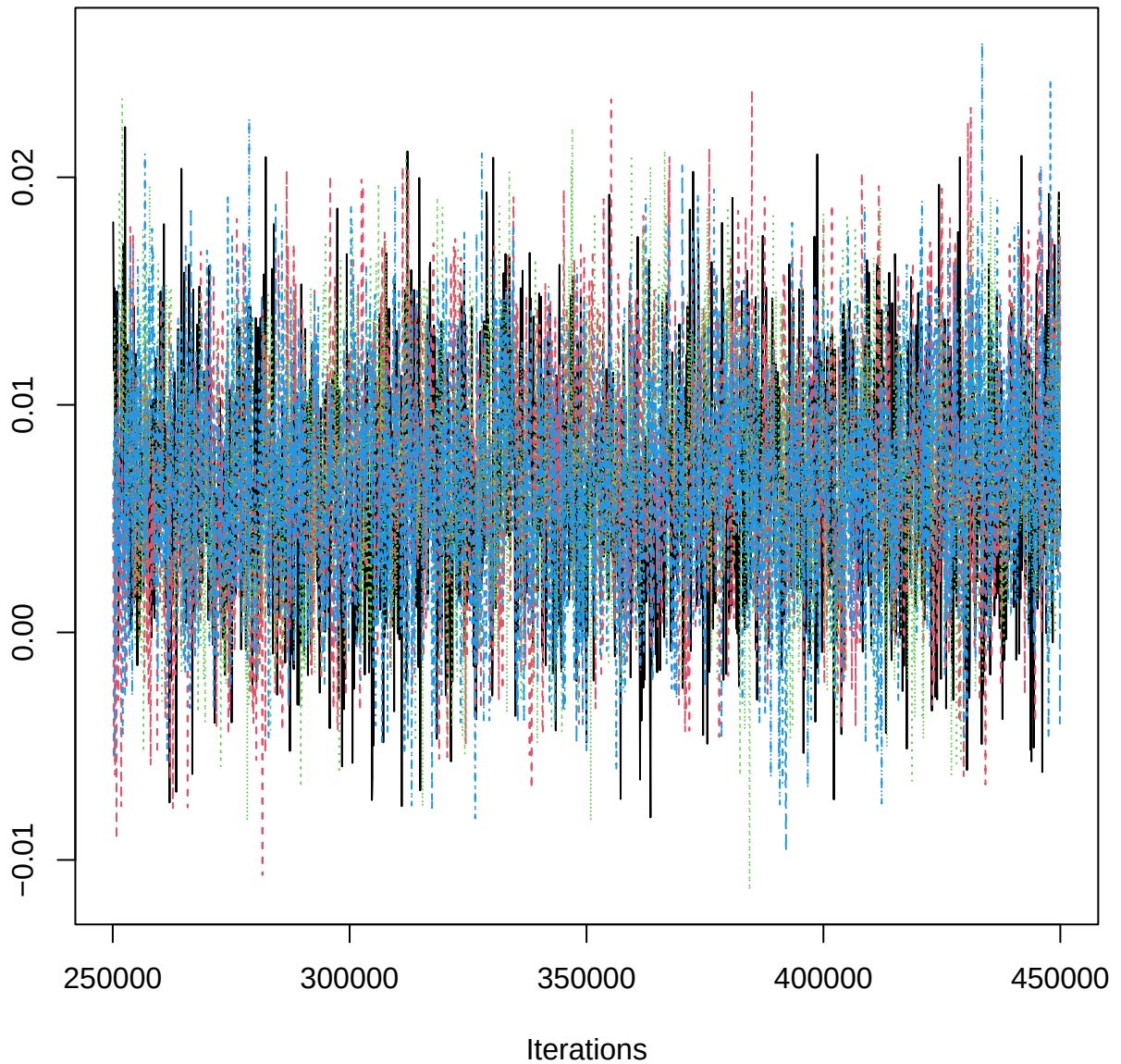
Traceplot – B[Clay (C5), EPN_n (S9)]
