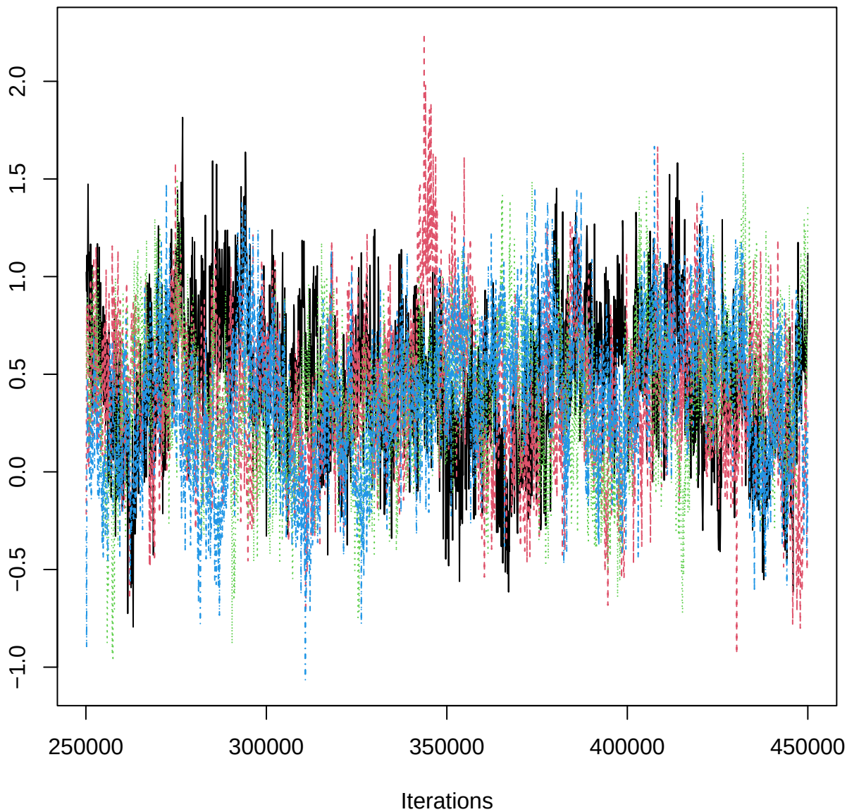
Traceplot – B[aspect_classNE (C12), PRP_n (S11)]
