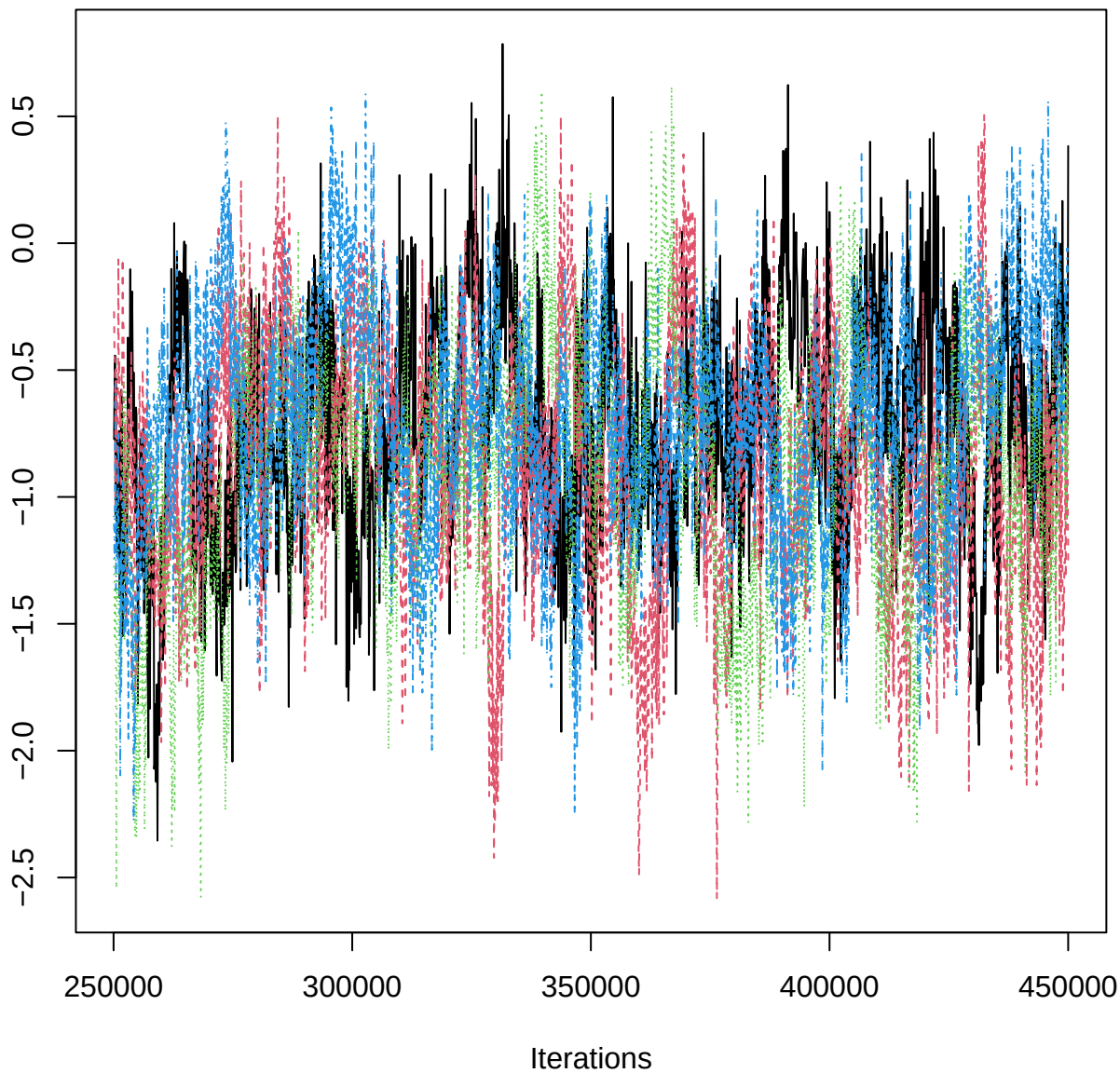
Traceplot – B[aspect_classSW (C16), HEG_n (S3)]
