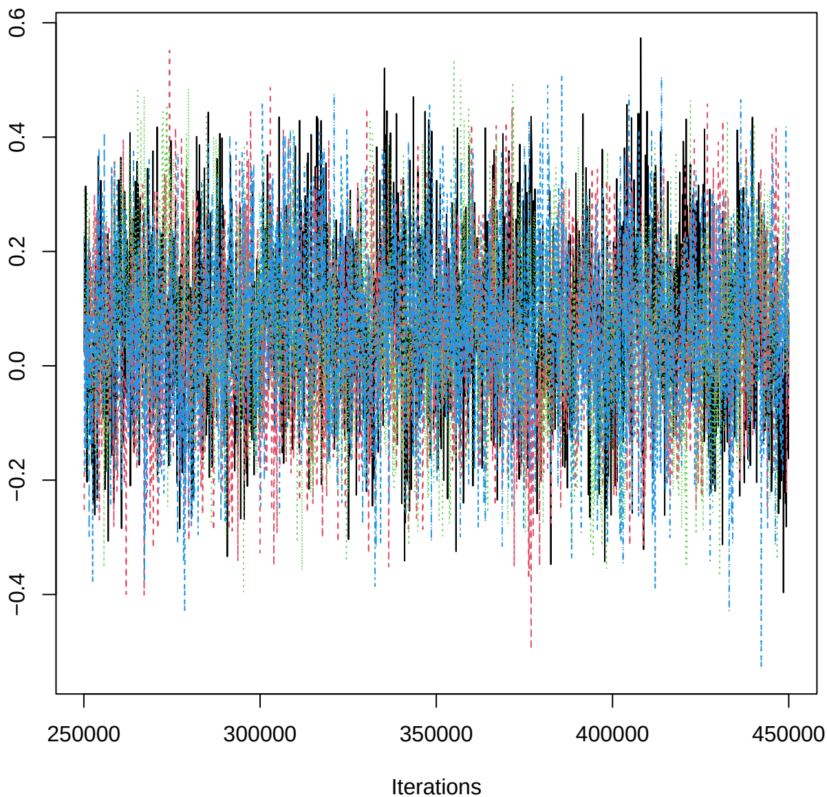
Traceplot - B[aspect_classNE (C12), SAB_n (S8)]
