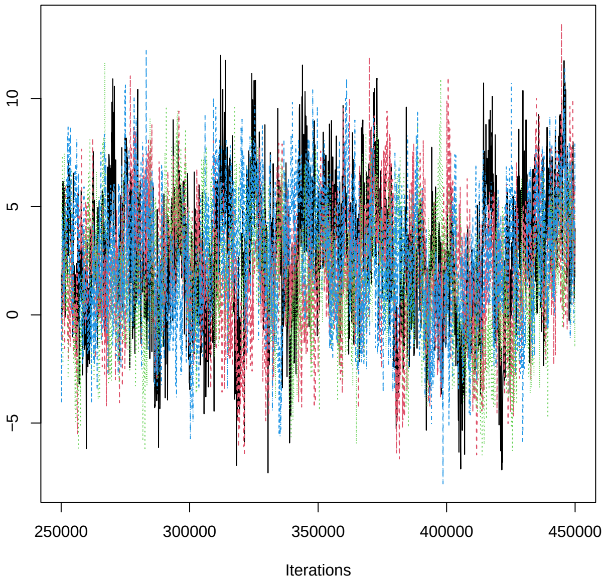
Traceplot – B[(Intercept) (C1), BOJ_n (S4)]
