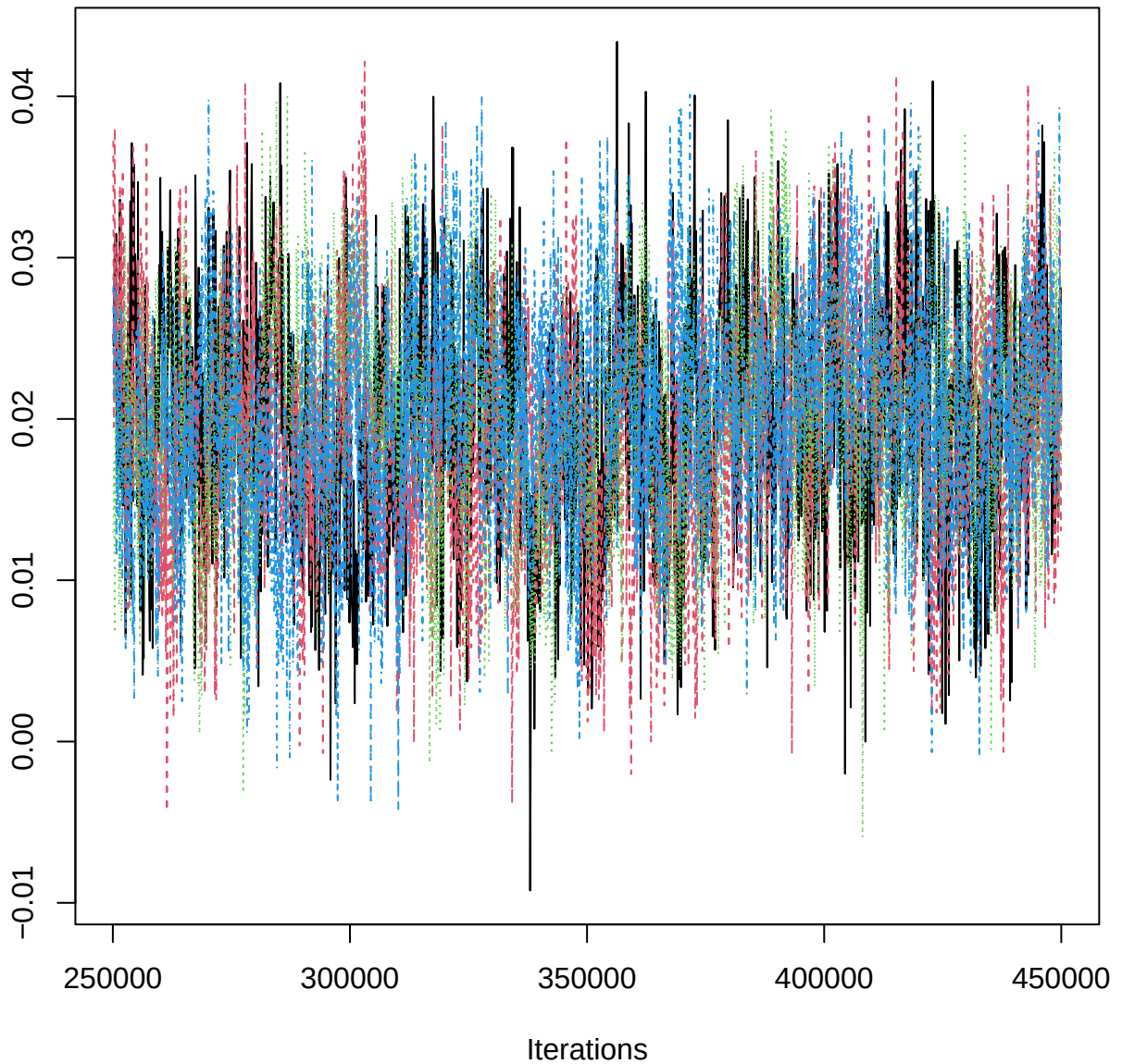
Traceplot – B[Clay (C5), EPB_n (S6)]
