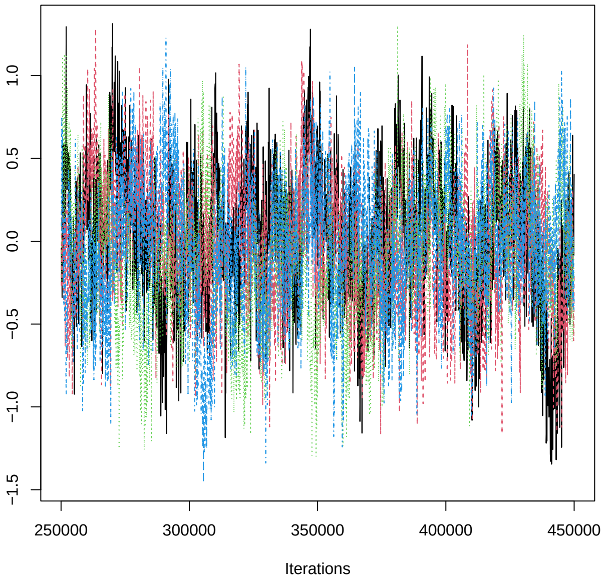
Traceplot – B[aspect_classSE (C15), THO_n (S10)]
