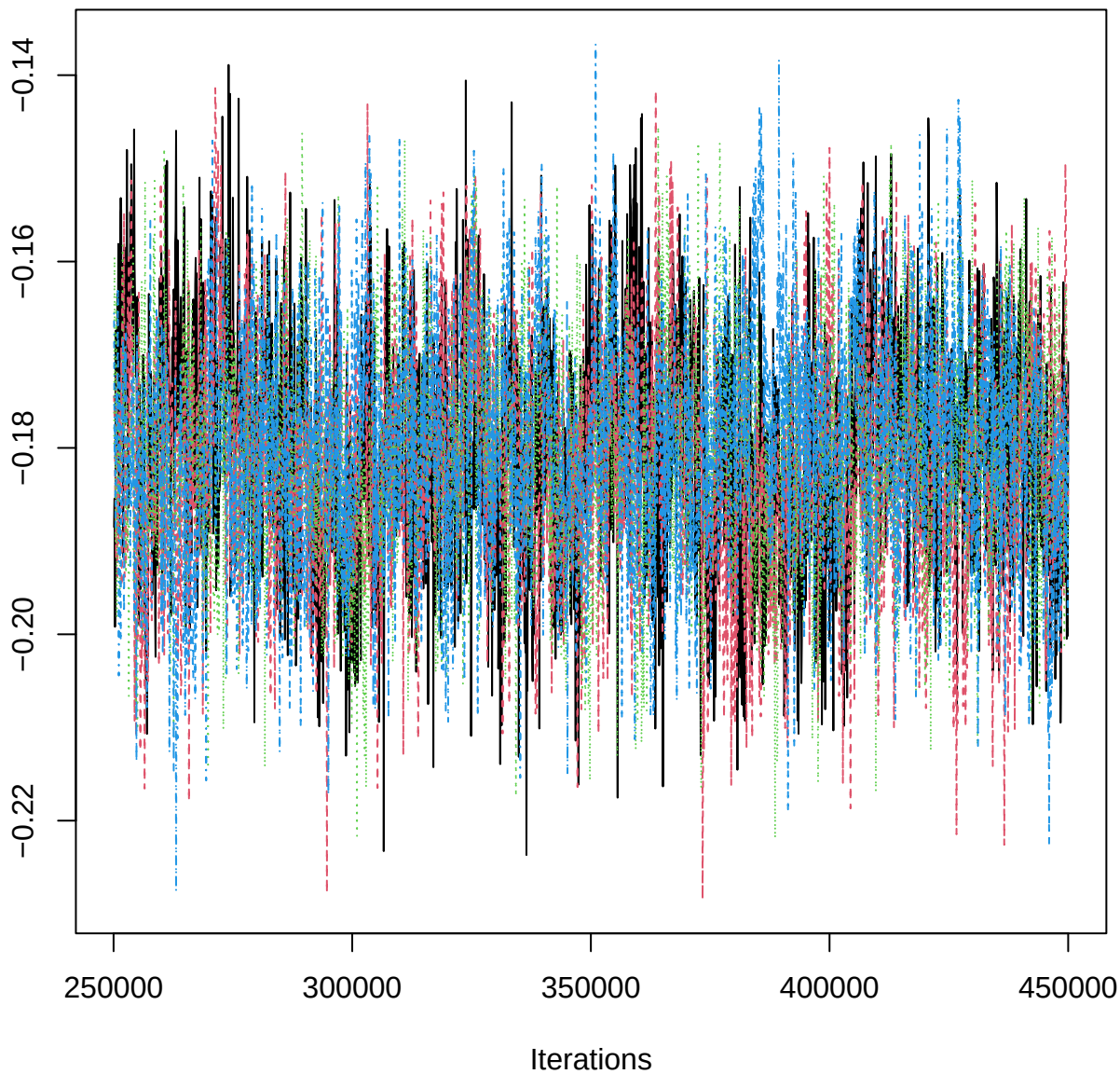
Traceplot – B[slope (C9), EPN_n (S9)]
