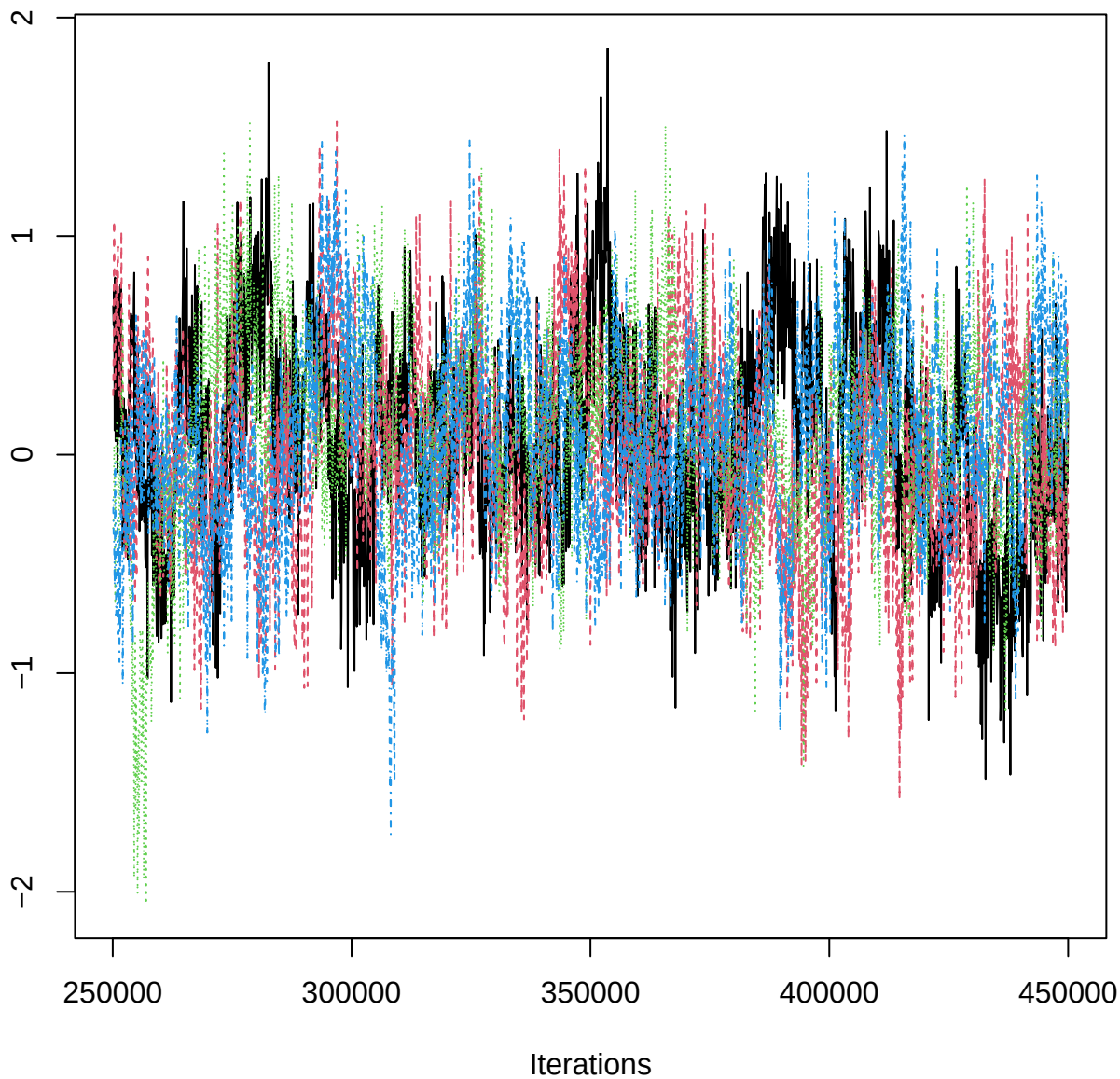
Traceplot – B[aspect_classS (C14), HEG_n (S3)]
