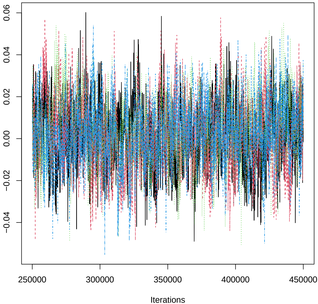
Traceplot – B[slope (C9), ERR_n (S1)]
