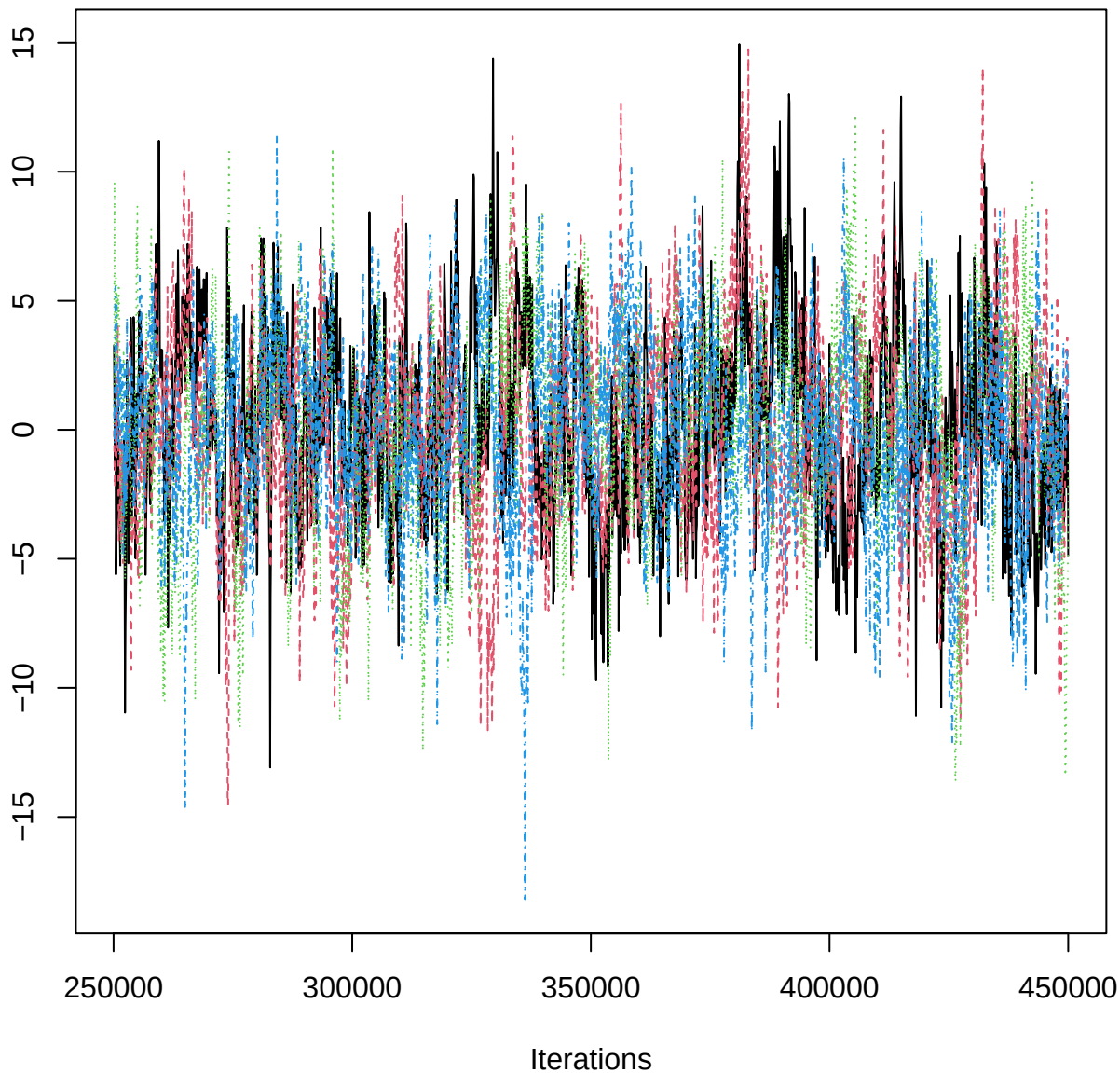
Traceplot – B[aspect_classFlat (C10), PIG_n (S14)]
