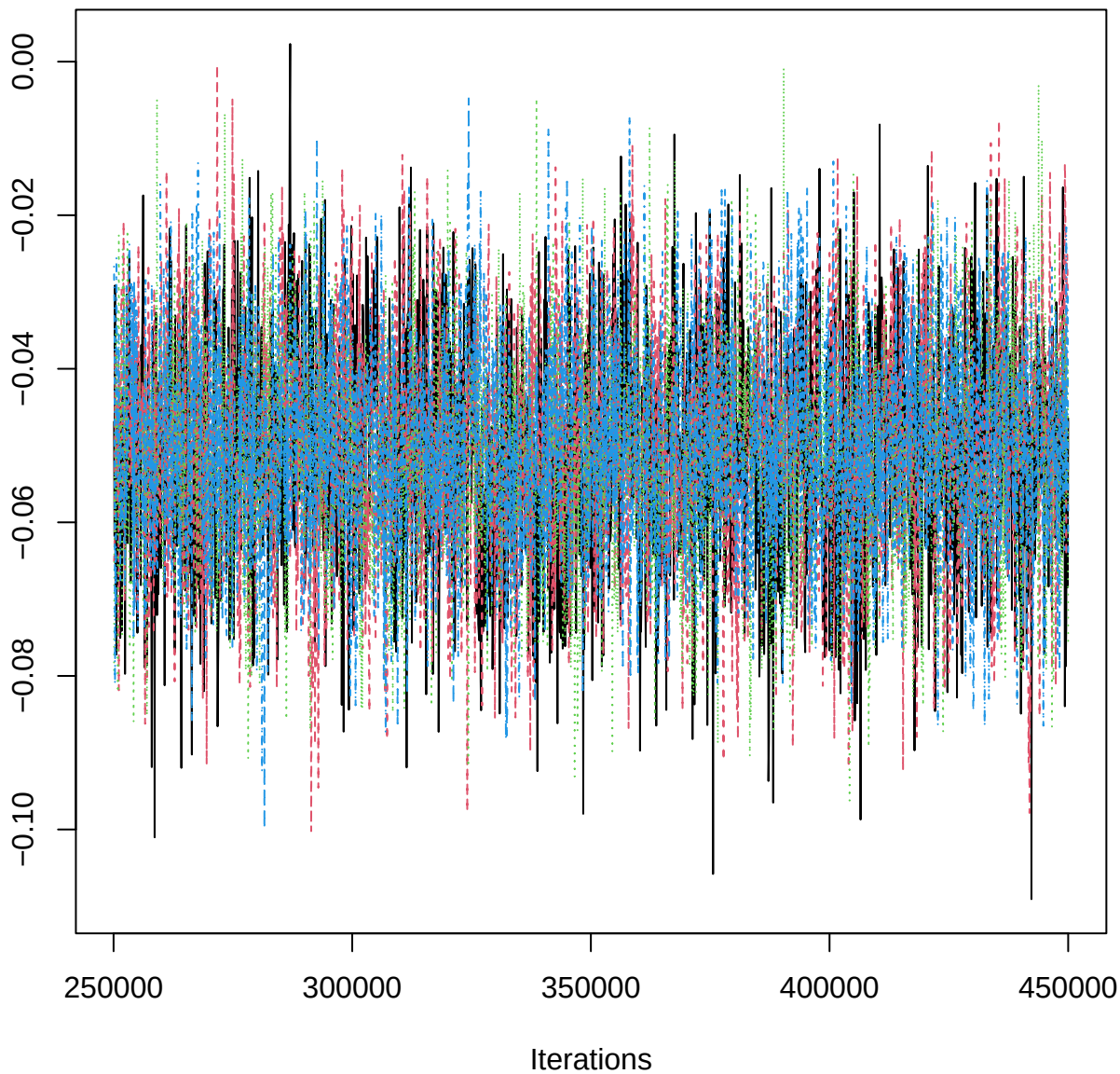
Traceplot – B[twi (C8), SAB_n (S8)]
