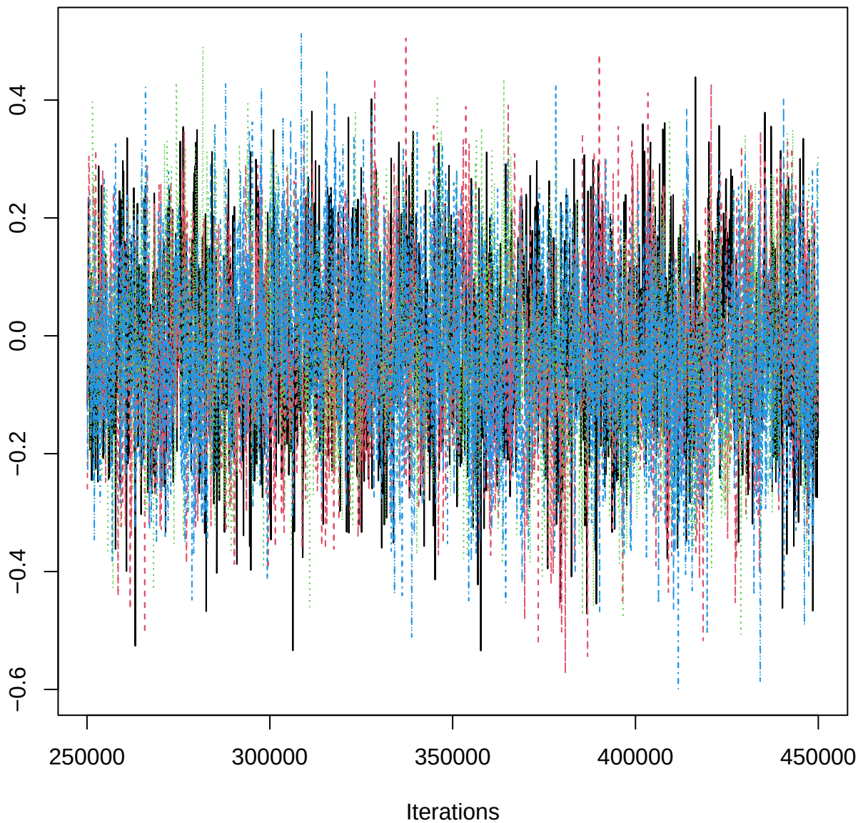
Traceplot – B[aspect_classS (C14), SAB_n (S8)]
