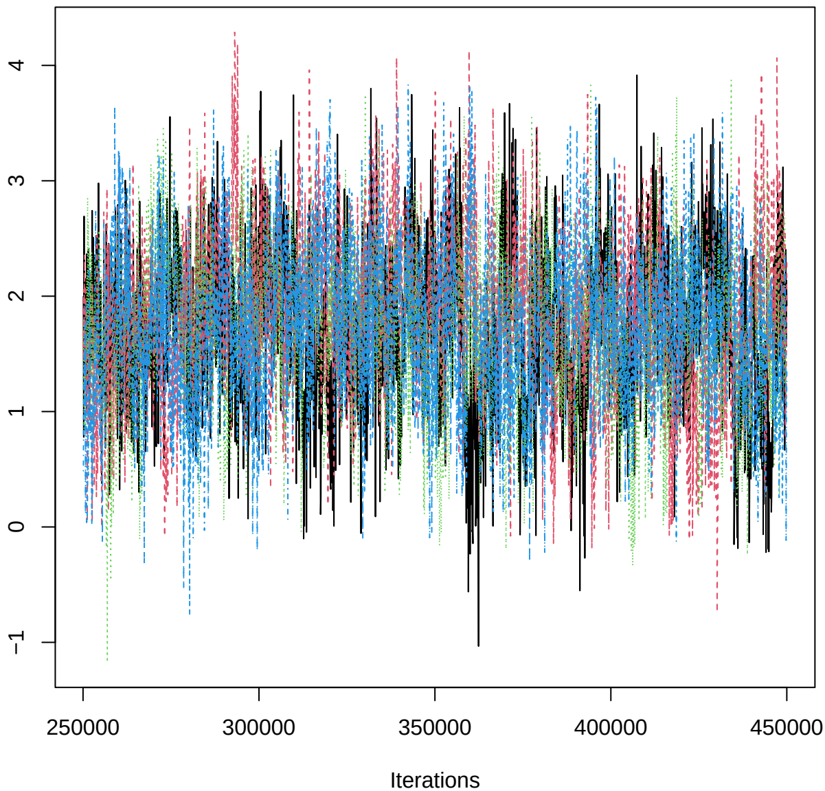
Traceplot – B[pH (C4), PET_n (S12)]
