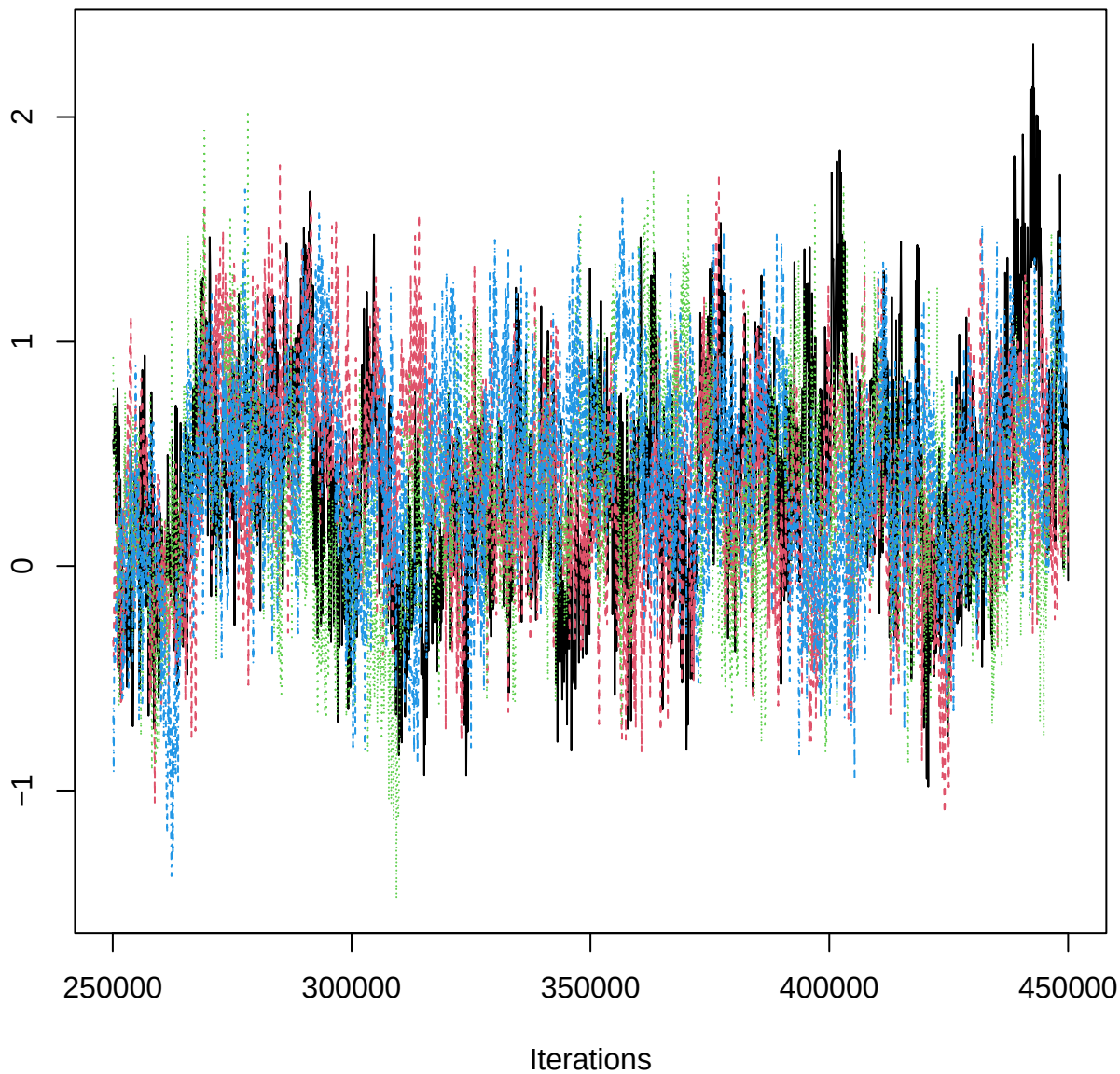
Traceplot – B[aspect_classSW (C16), PIG_n (S14)]
