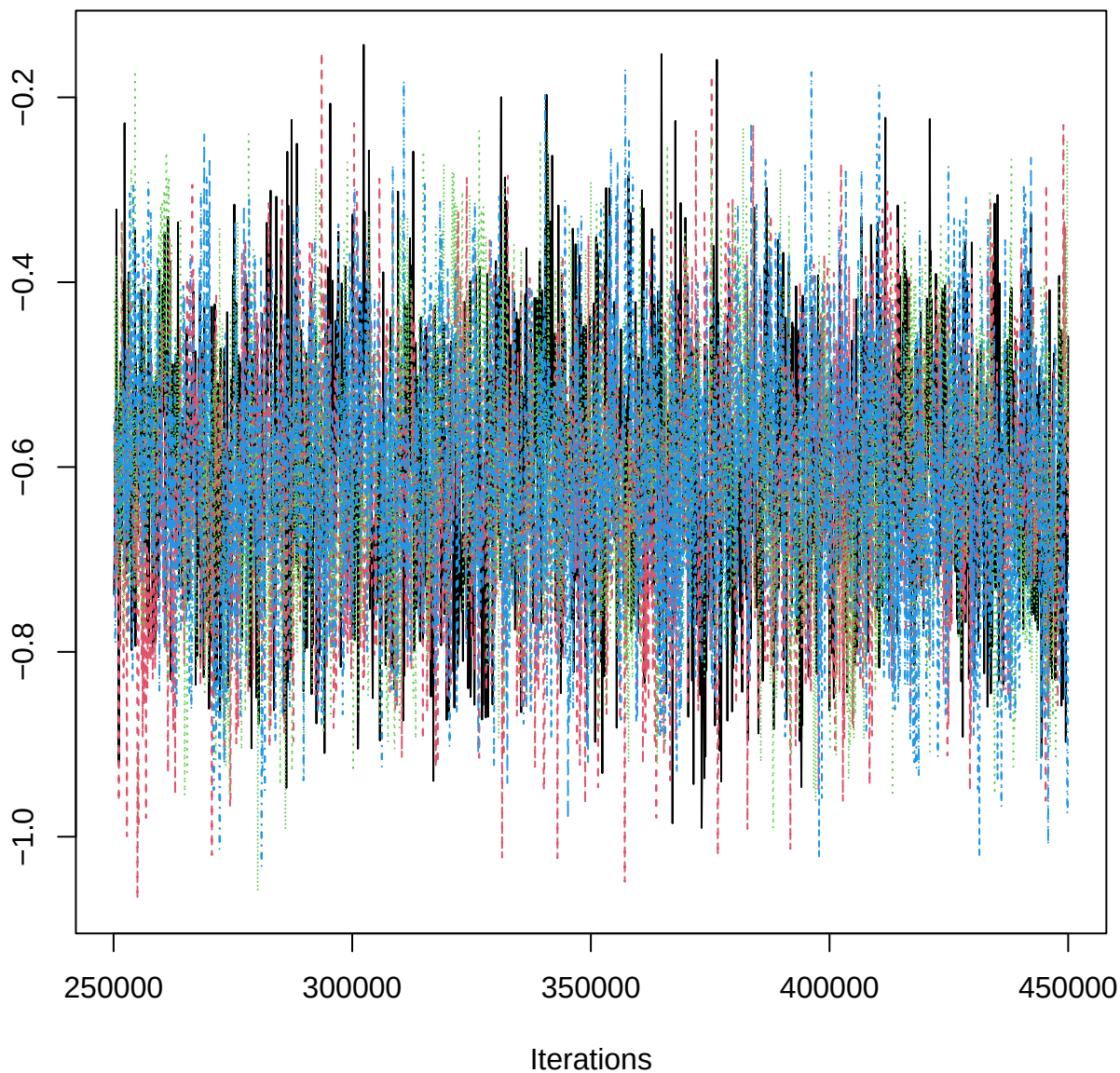
Traceplot – B[rtp (C7), EPN_n (S9)]
