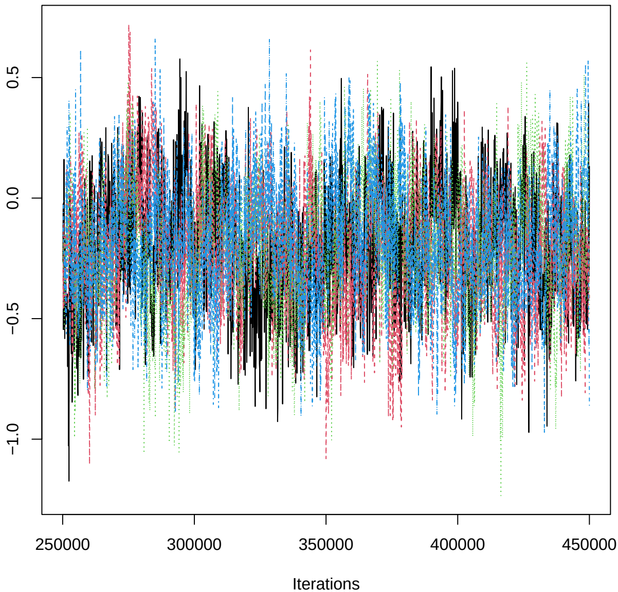
Traceplot – B[aspect_classNW (C13), ERS_n (S2)]
