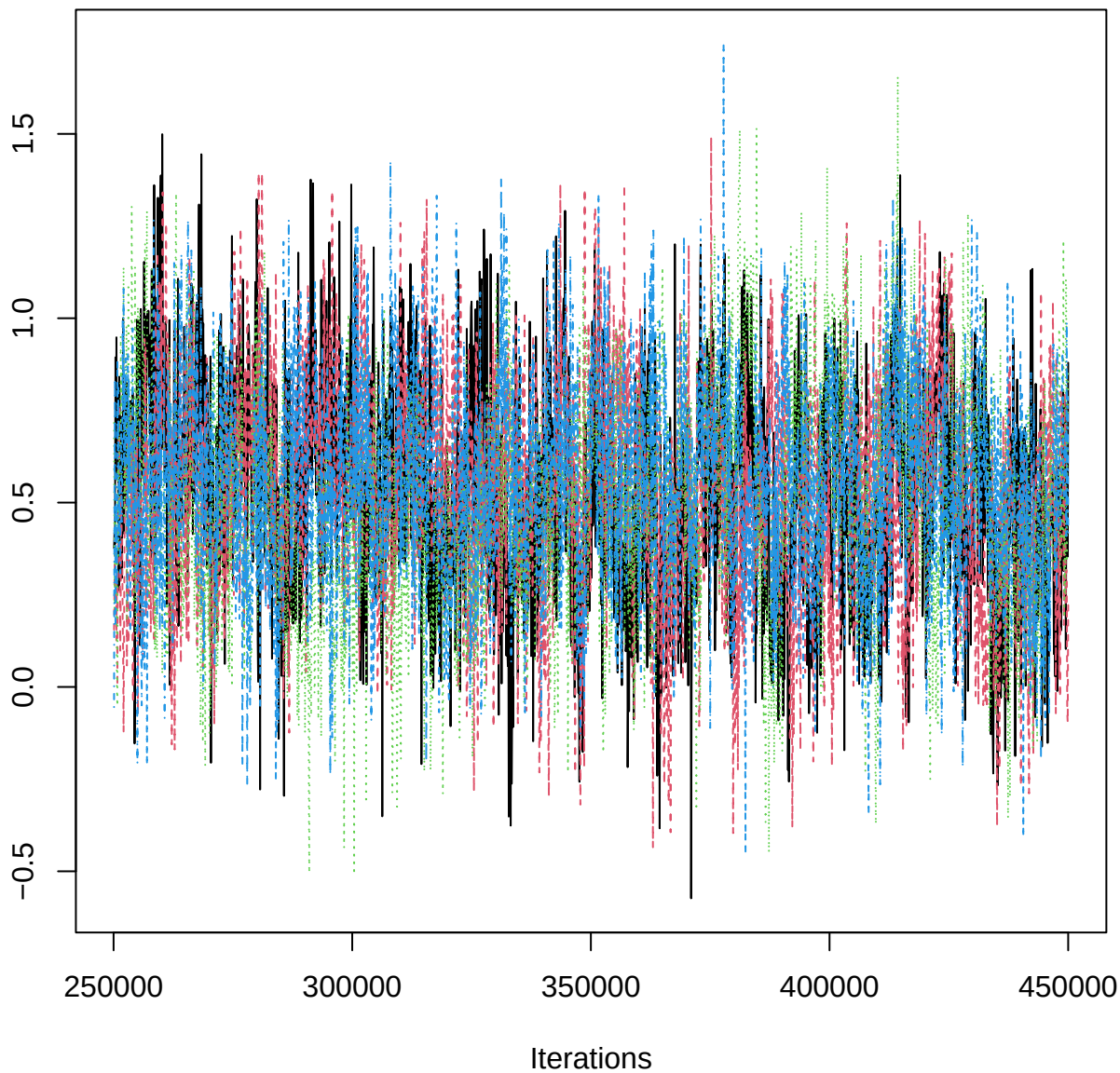
Traceplot – B[aspect_classS (C14), PET_n (S12)]
