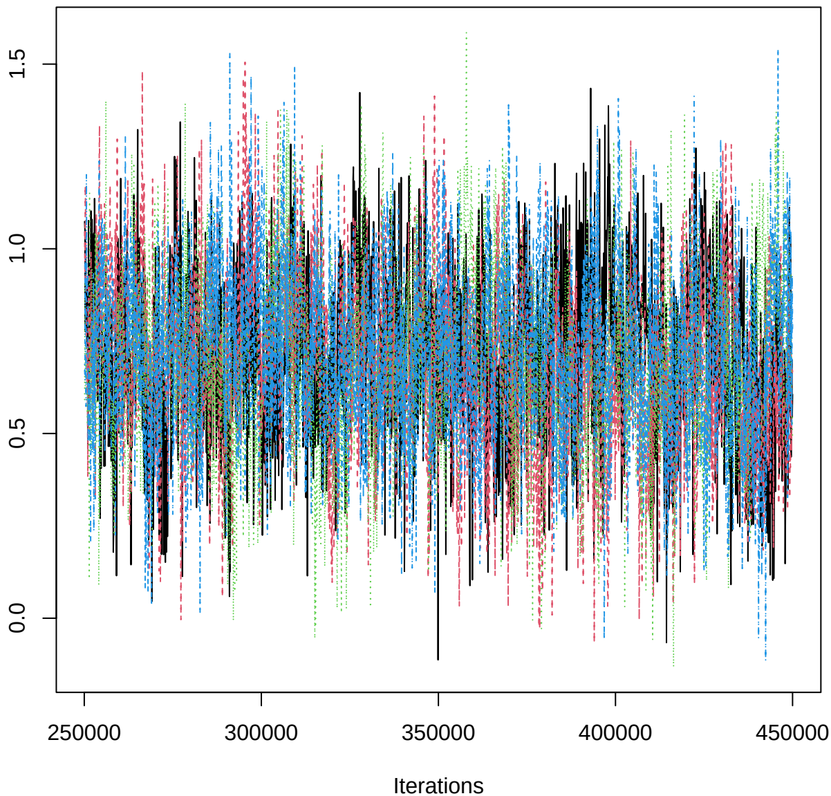
Traceplot – B[aspect_classS (C14), ERR_n (S1)]
