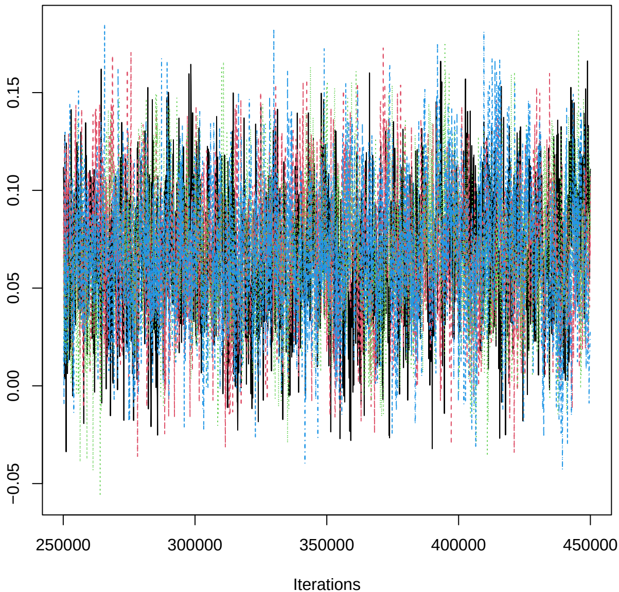
Traceplot – B[OM (C6), EPN_n (S9)]
