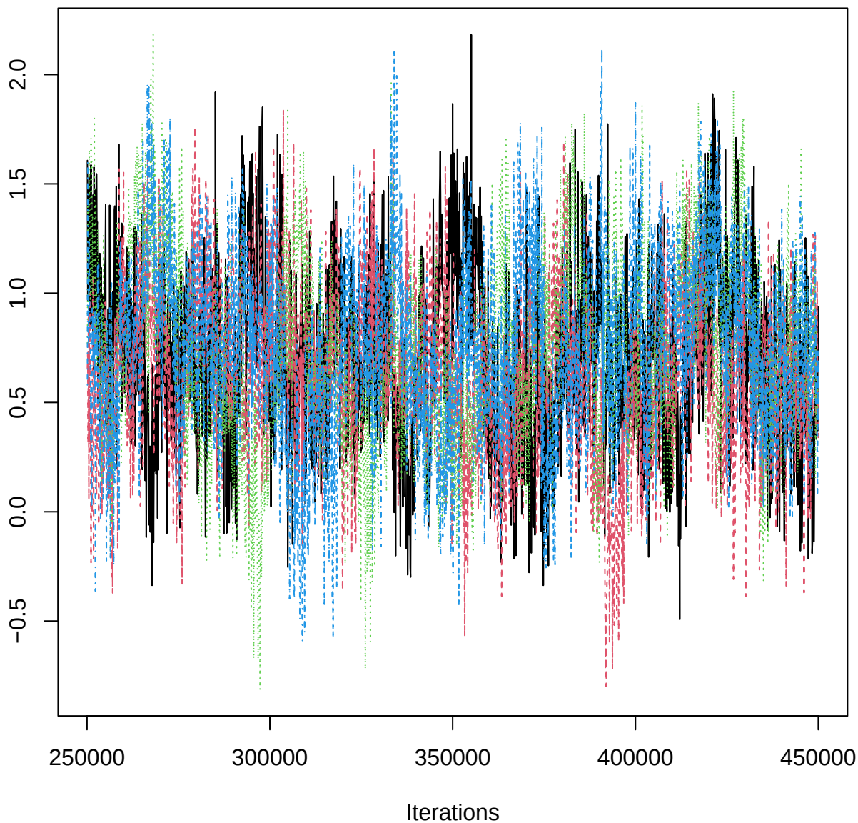
Traceplot – B[aspect_classSW (C16), THO_n (S10)]
