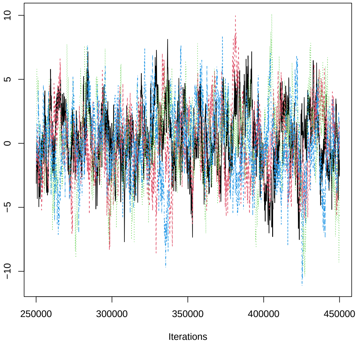
Traceplot – B[aspect_classFlat (C10), ERS_n (S2)]
