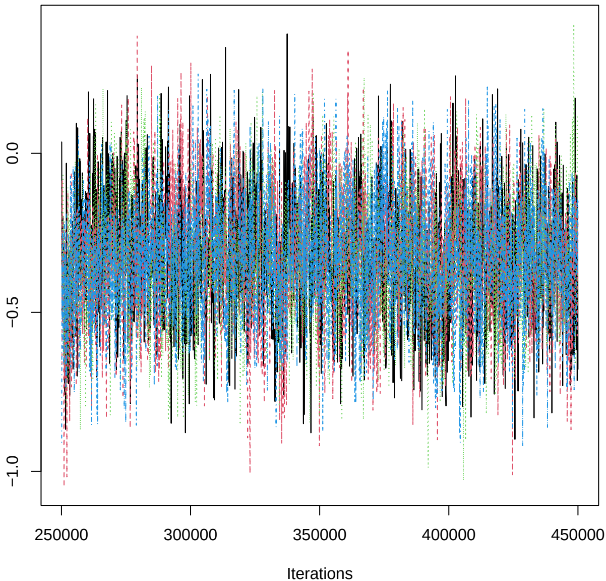
Traceplot – B[aspect_classN (C11), EPN_n (S9)]
