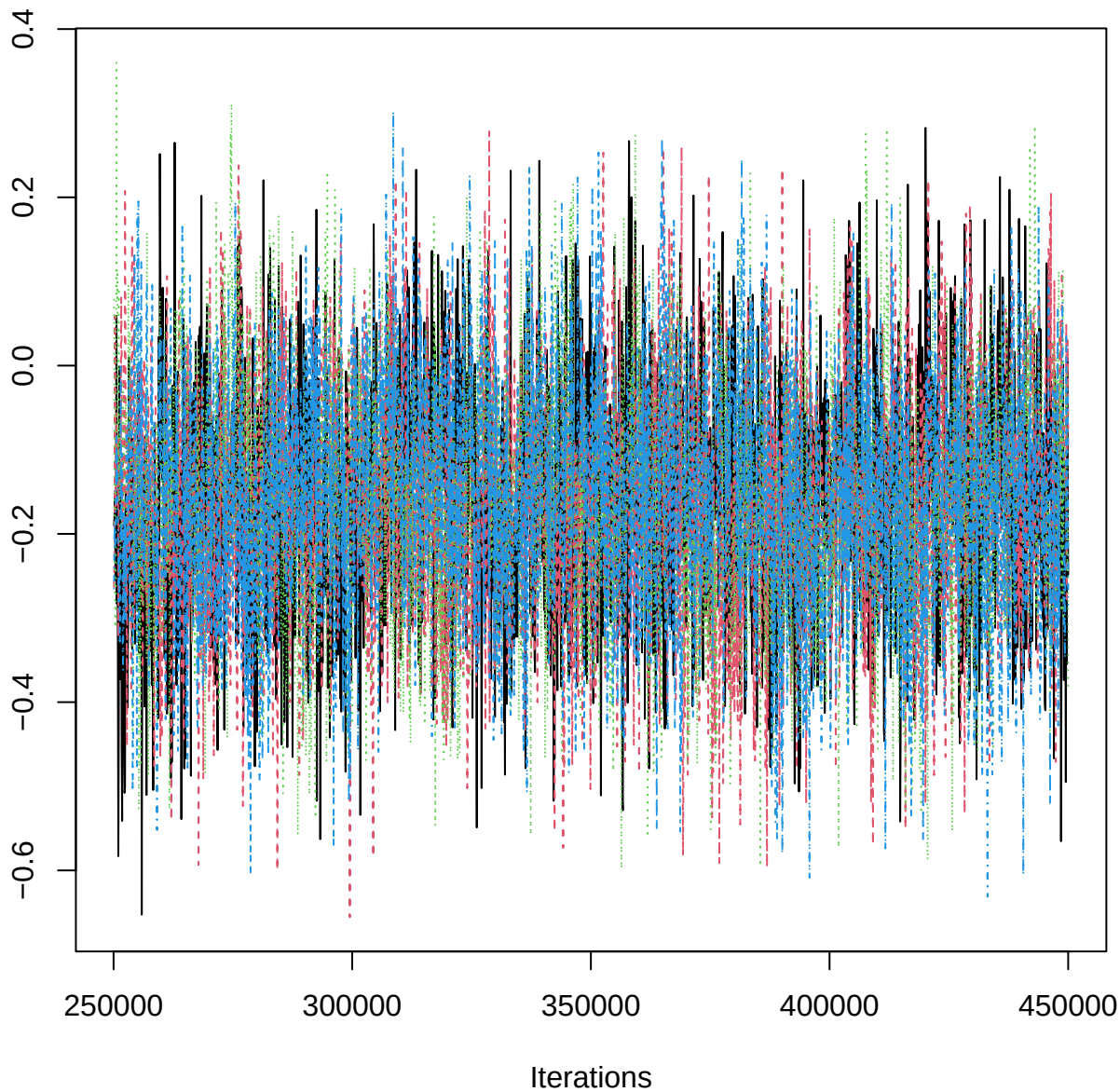
Traceplot – B[aspect_classSE (C15), SAB_n (S8)]
