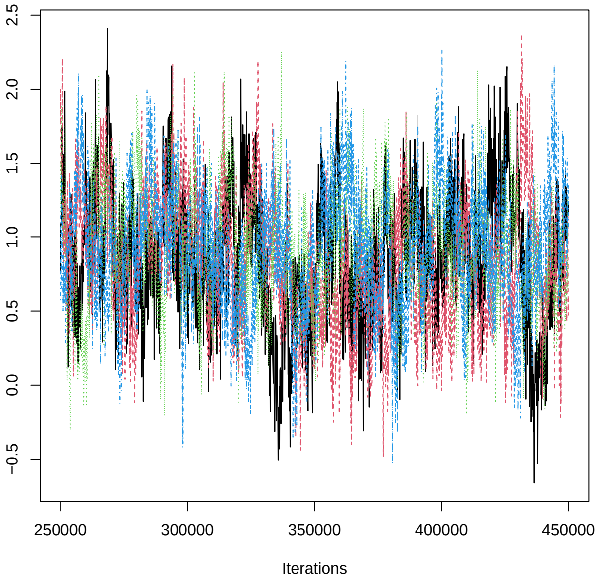
Traceplot – B[aspect_classS (C14), PIB_n (S13)]
