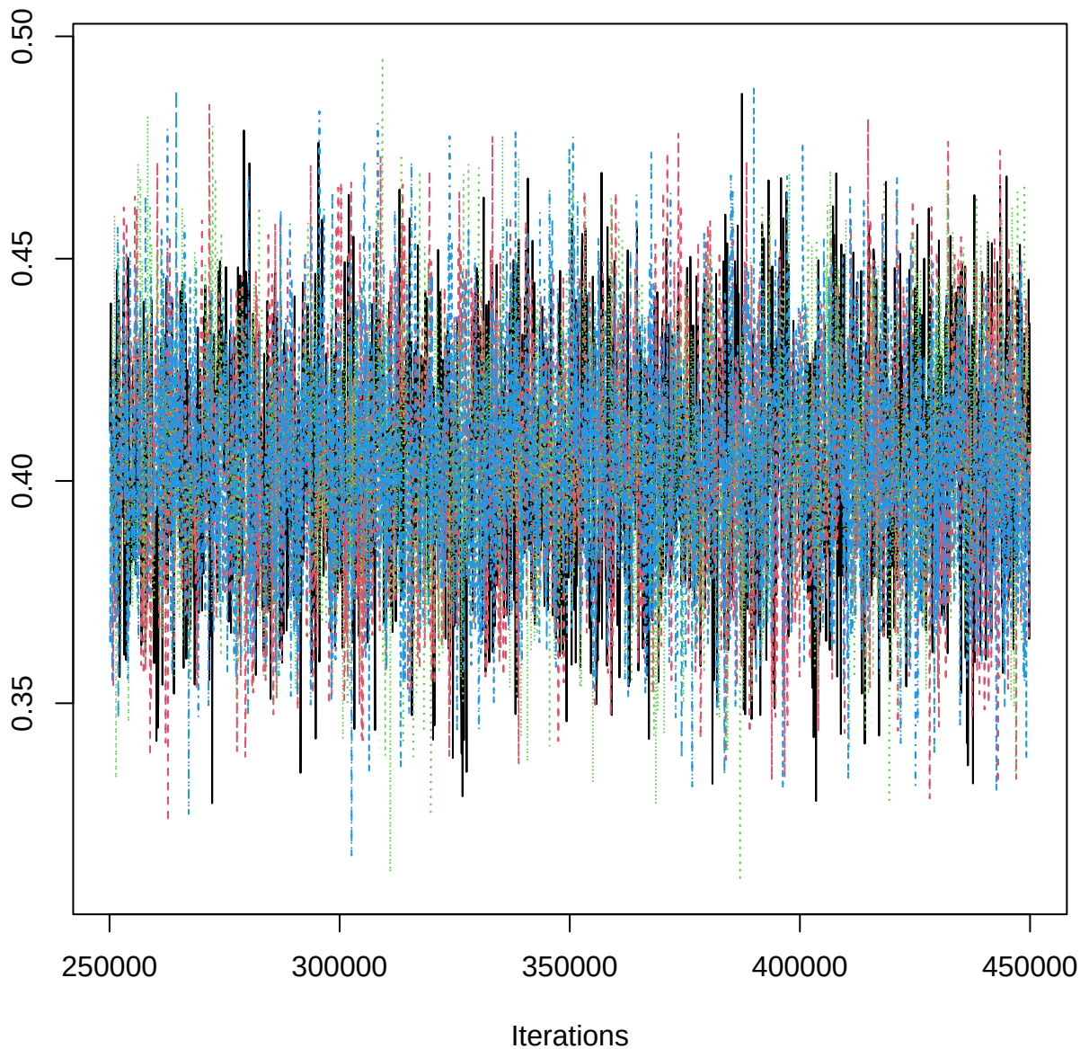
Traceplot – B[OM (C6), SAB_n (S8)]
