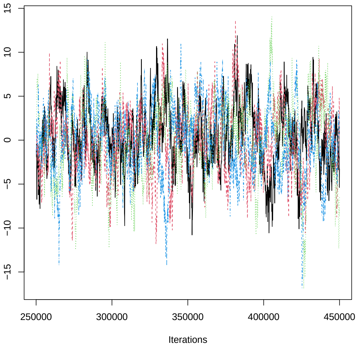
Traceplot – B[aspect_classFlat (C10), THO_n (S10)]
