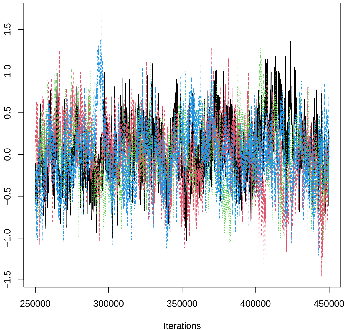
Traceplot – B[aspect_classSW (C16), PRP_n (S11)]
