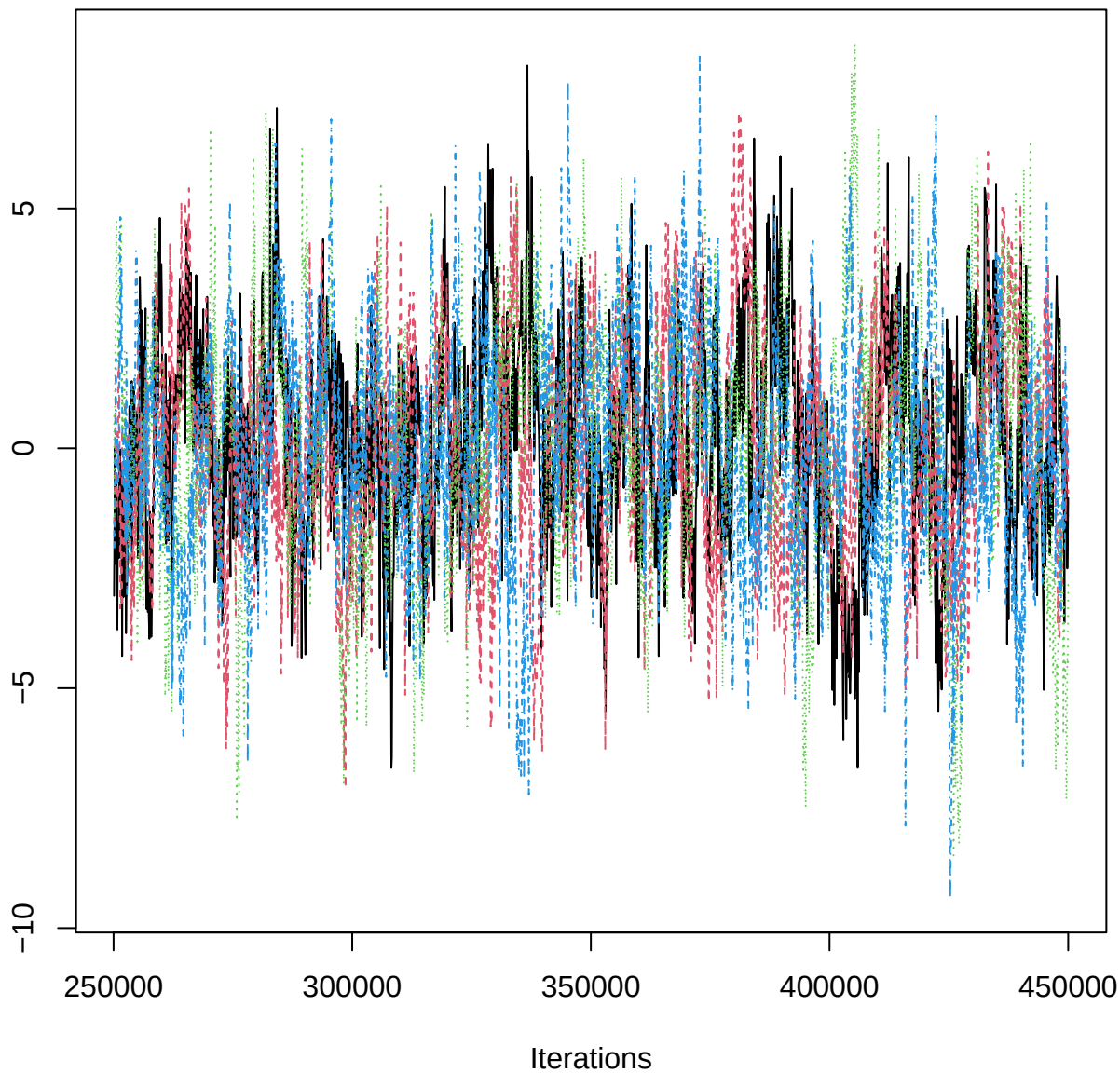
Traceplot – B[aspect_classFlat (C10), ERR_n (S1)]
