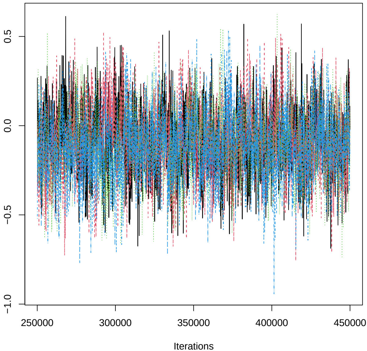
Traceplot – B[aspect_classNW (C13), EPN_n (S9)]
