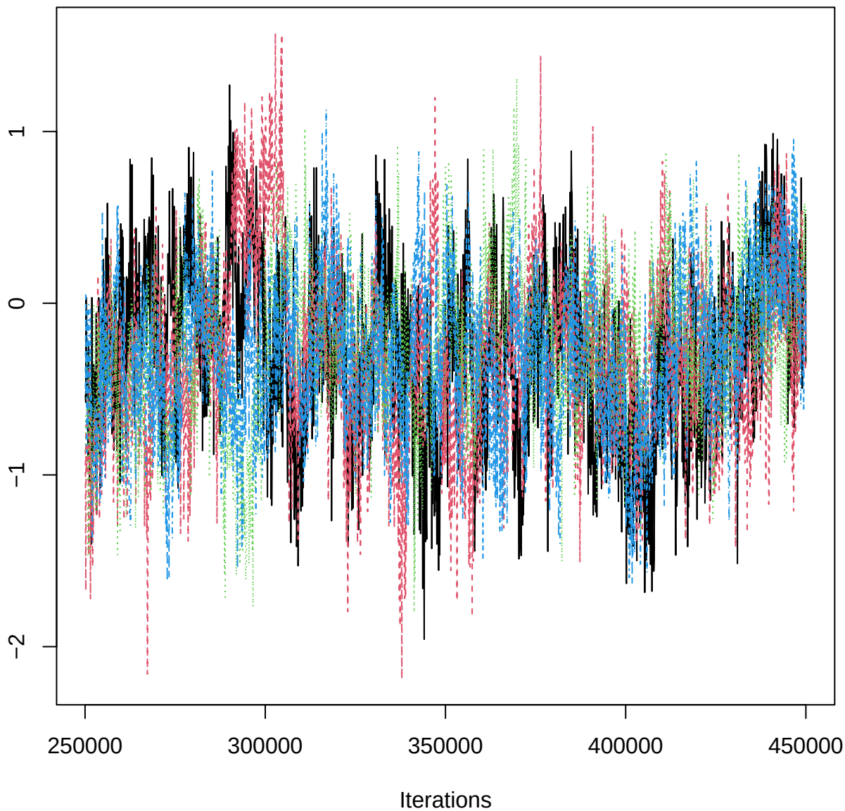
Traceplot – B[aspect_classN (C11), PIG_n (S14)]
