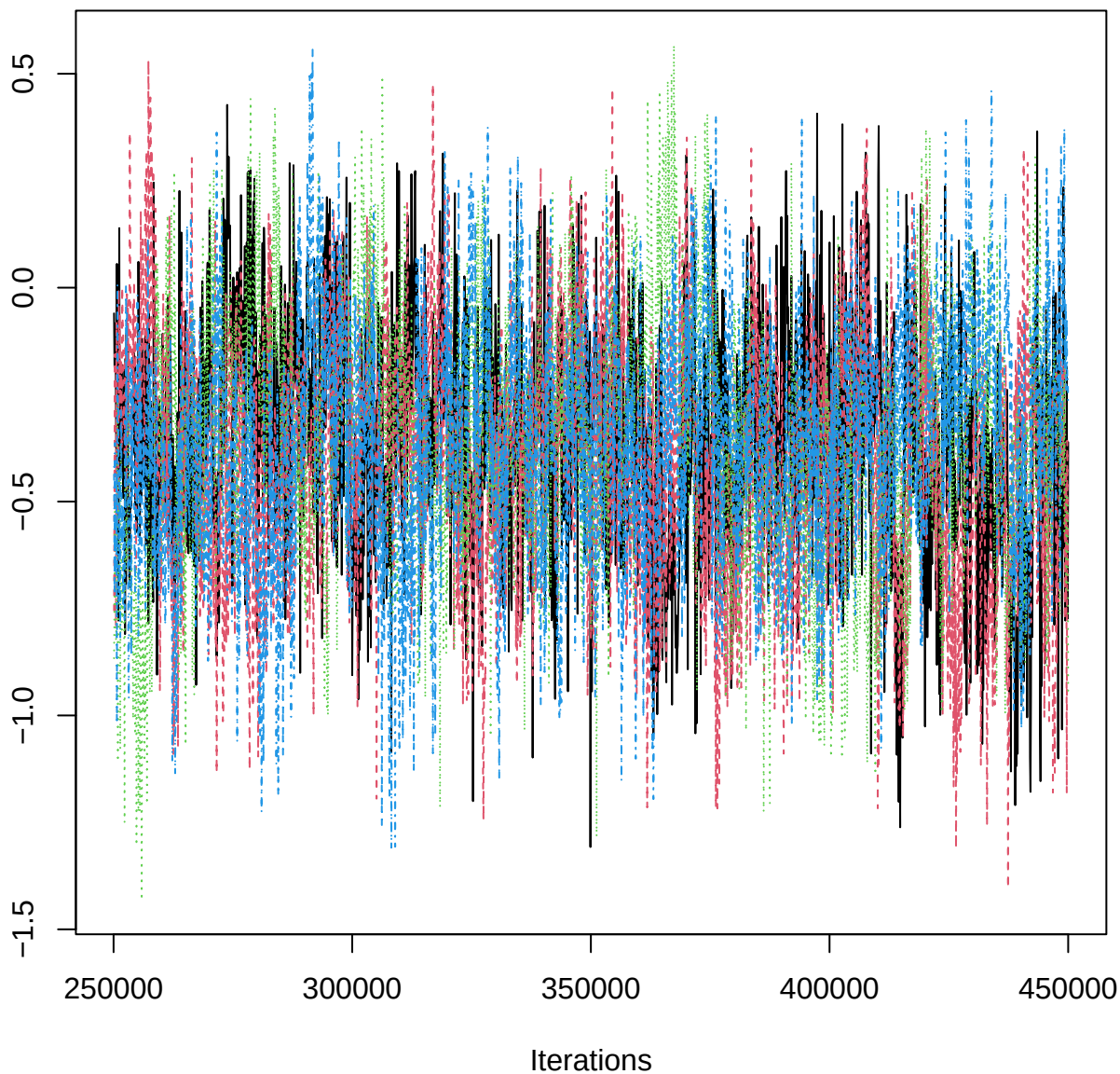
Traceplot – B[aspect_classS (C14), BOJ_n (S4)]
