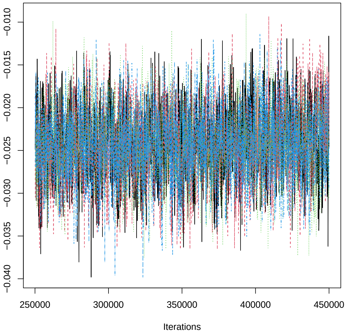
Traceplot – B[Clay (C5), SAB_n (S8)]
