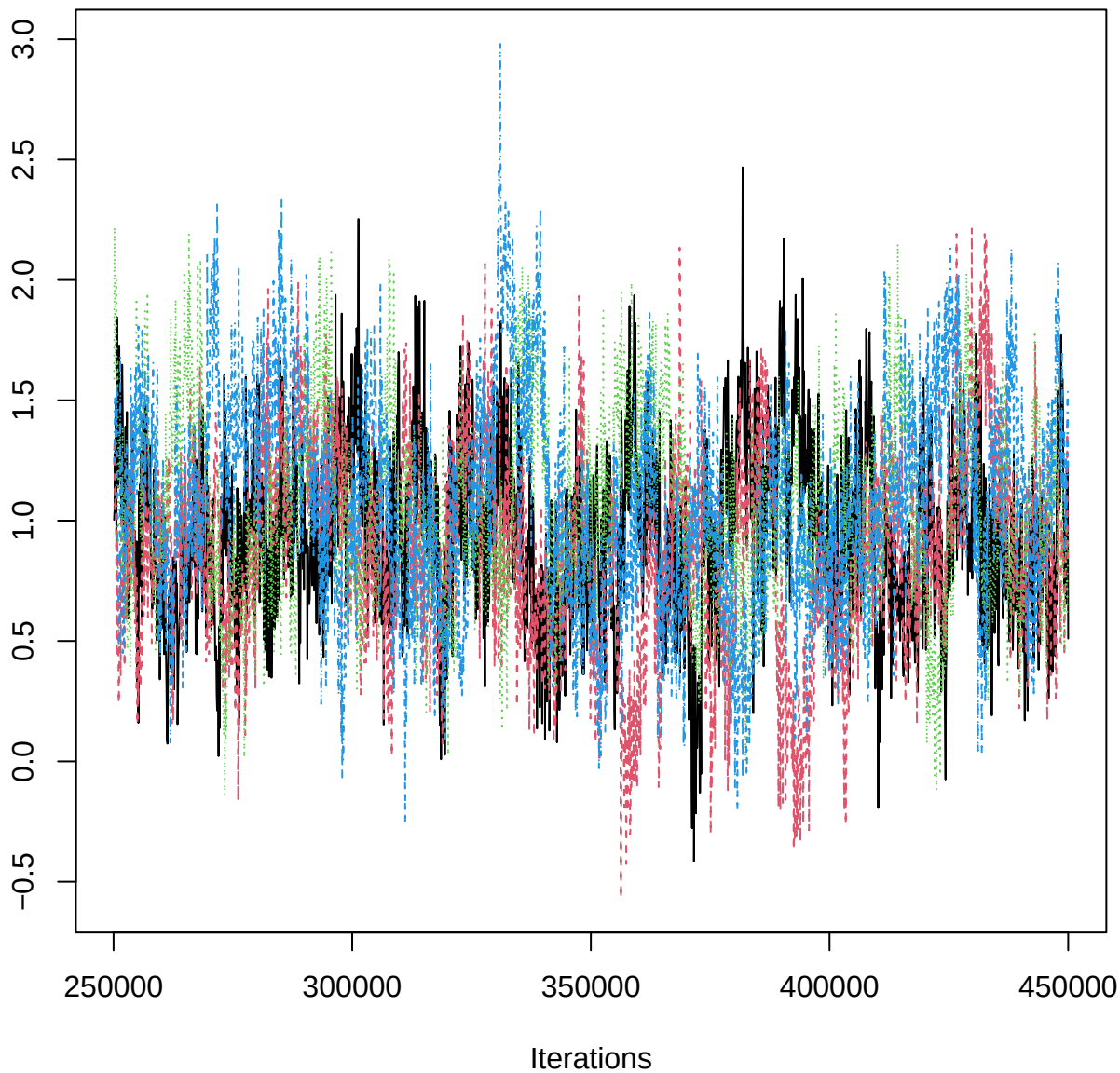
Traceplot – B[aspect_classW (C17), PIB_n (S13)]
