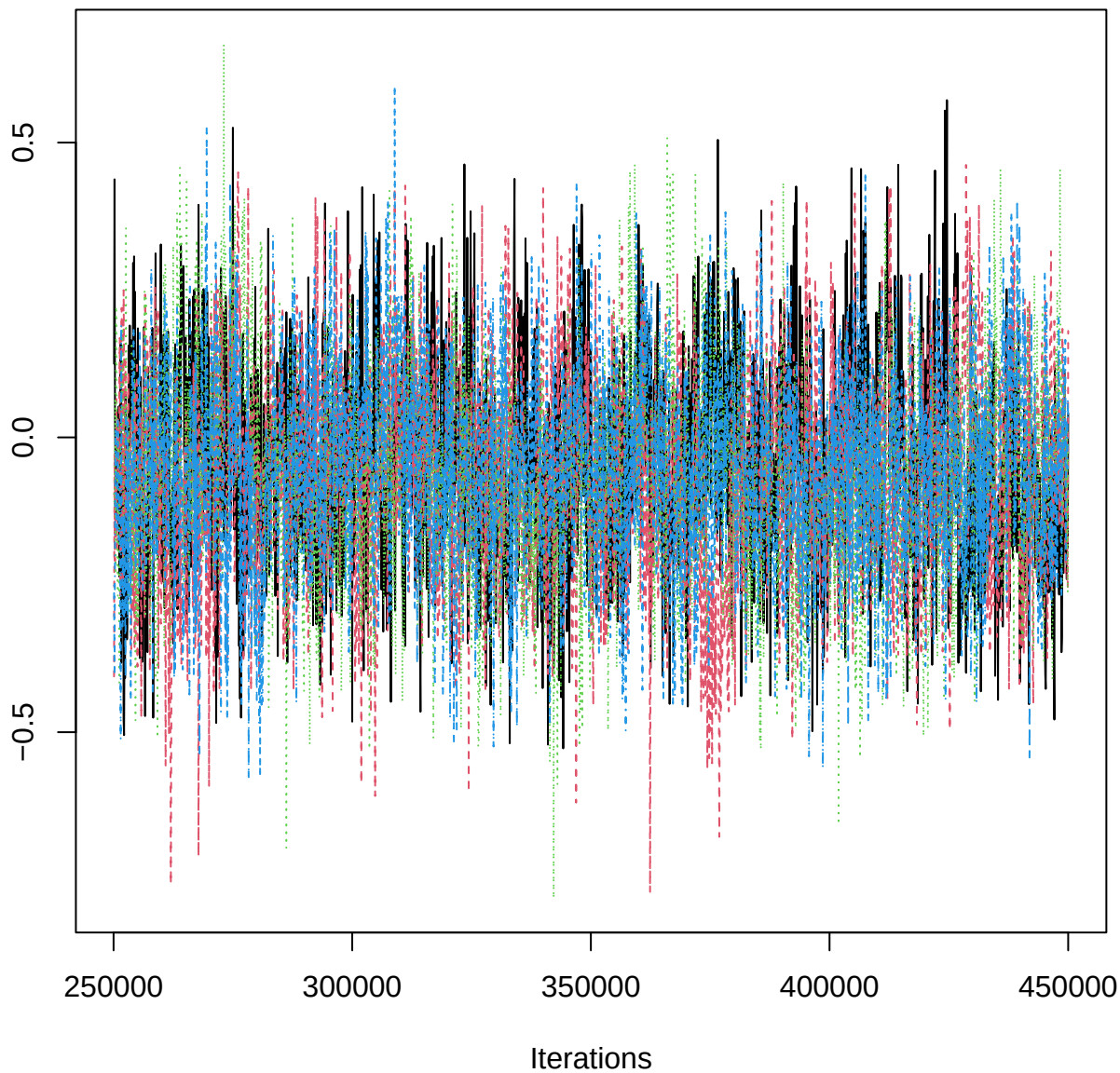
Traceplot – B[aspect_classNE (C12), BOP_n (S5)]
