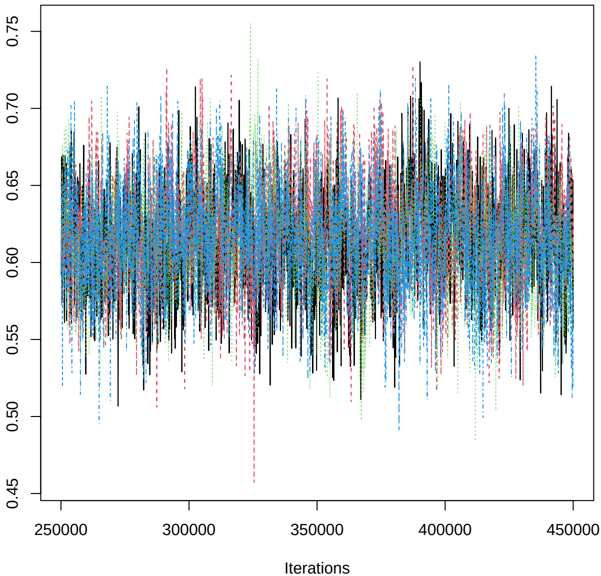
Traceplot – B[OM (C6), BOP_n (S5)]
