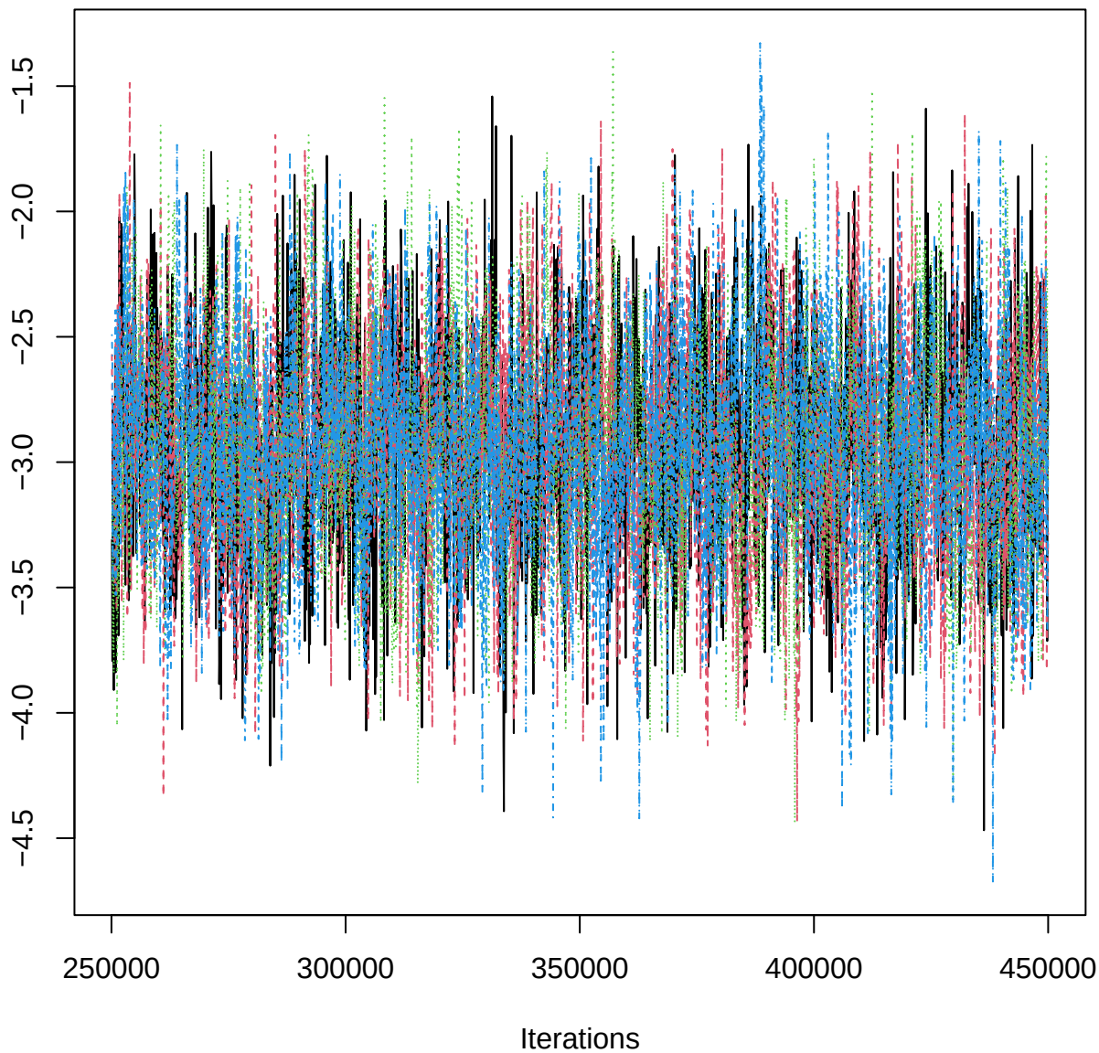
Traceplot – B[pH (C4), BOP_n (S5)]
