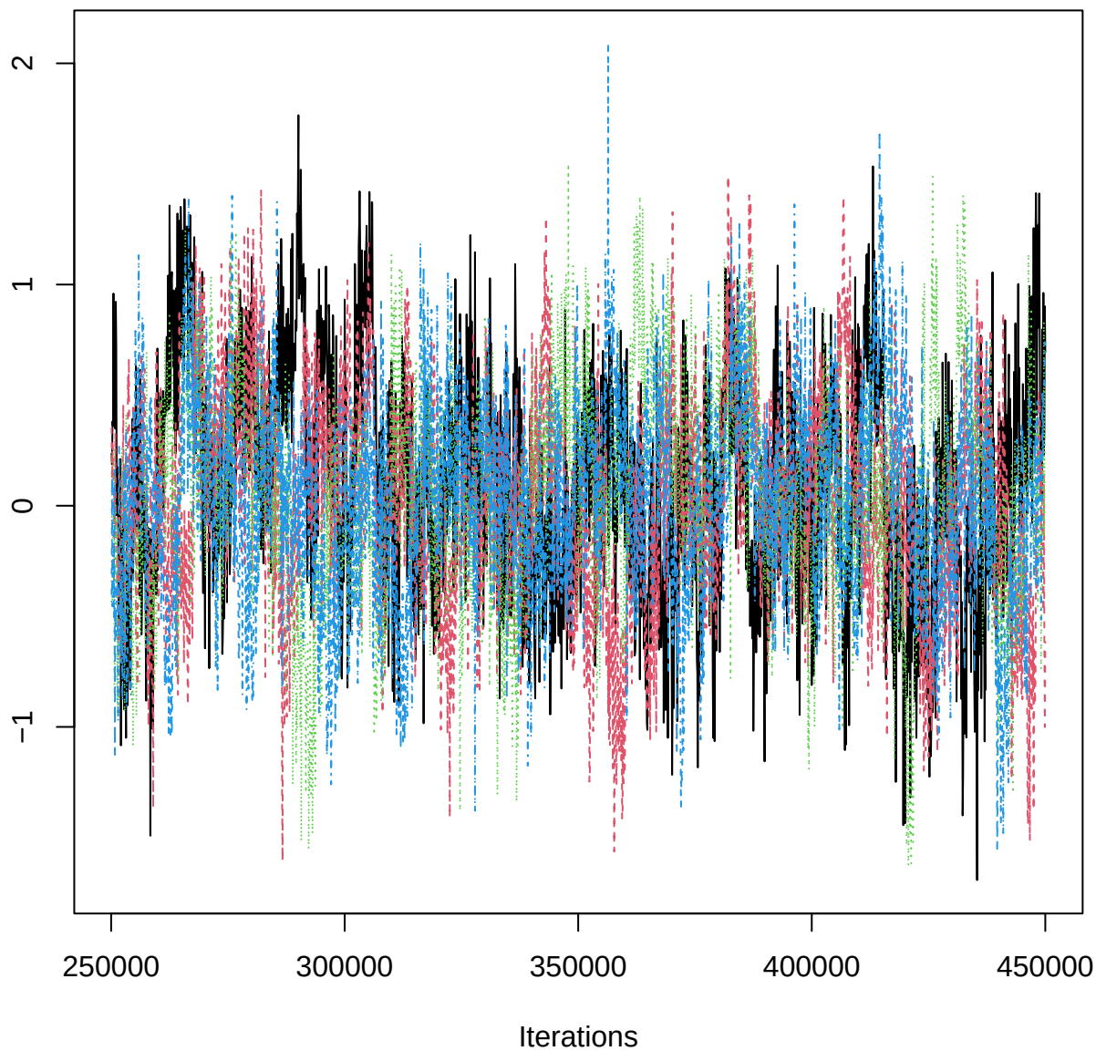
Traceplot – B[aspect_classS (C14), PIG_n (S14)]
