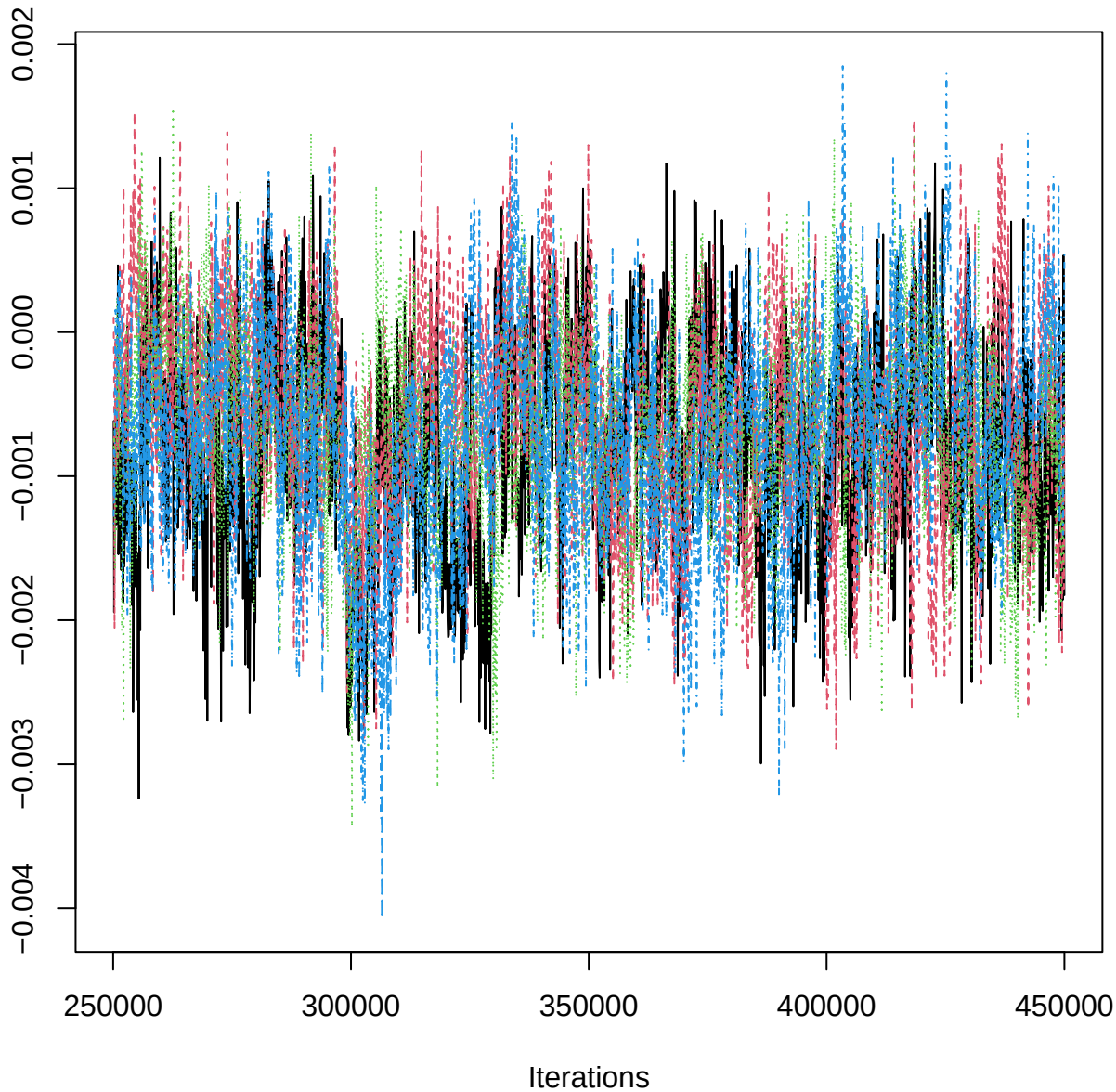
Traceplot – B[MAP (C2), ERR_n (S1)]
