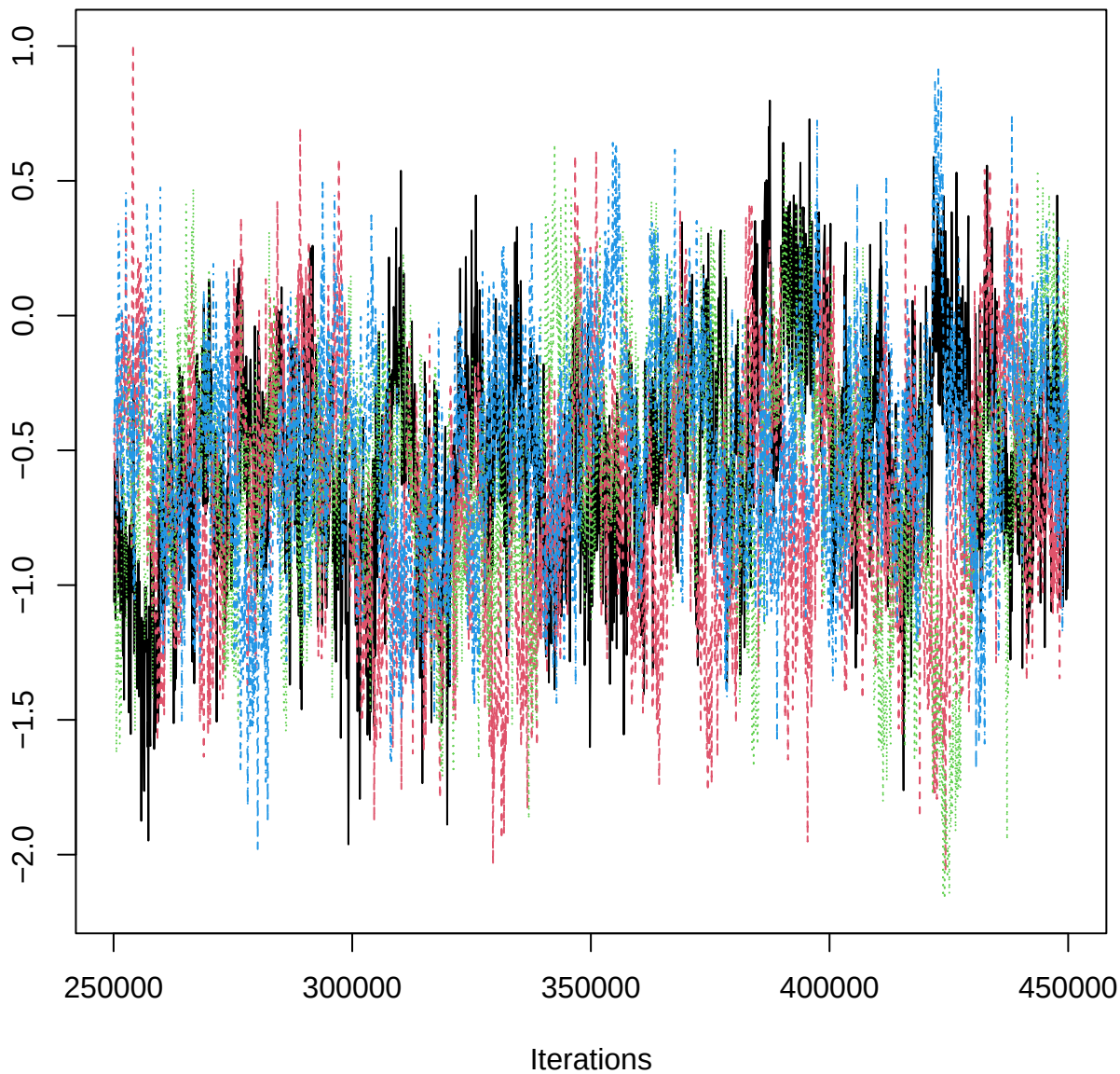
Traceplot – B[aspect_classW (C17), HEG_n (S3)]
