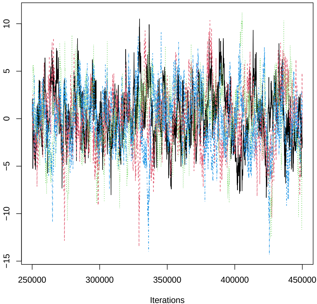
Traceplot – B[aspect_classFlat (C10), PRP_n (S11)]
