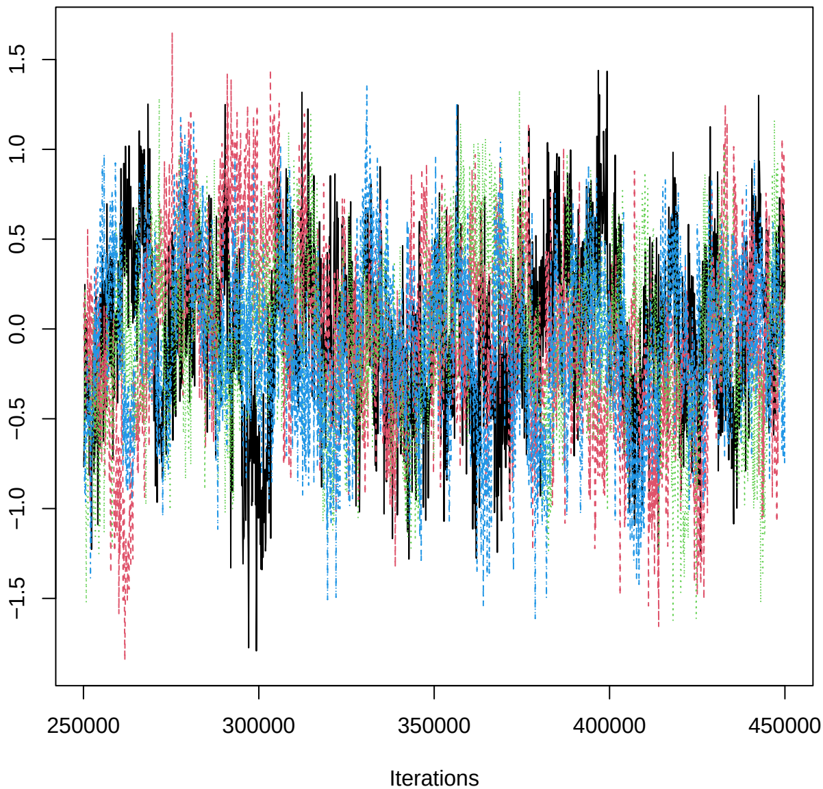
Traceplot – B[aspect_classSE (C15), PIG_n (S14)]
