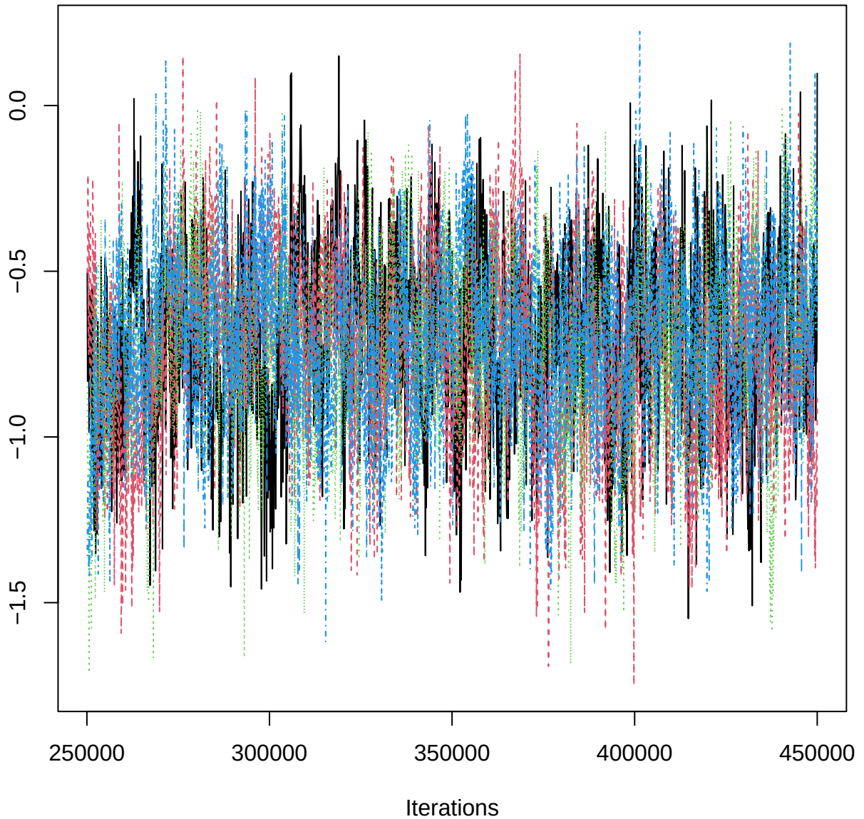
Traceplot – B[aspect_classSW (C16), BOJ_n (S4)]
