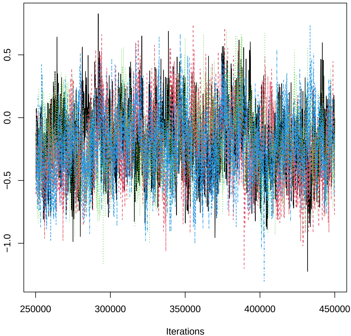
Traceplot – B[aspect_classN (C11), PET_n (S12)]
