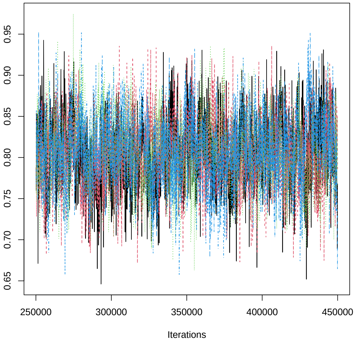
Traceplot – B[OM (C6), EPB_n (S6)]
