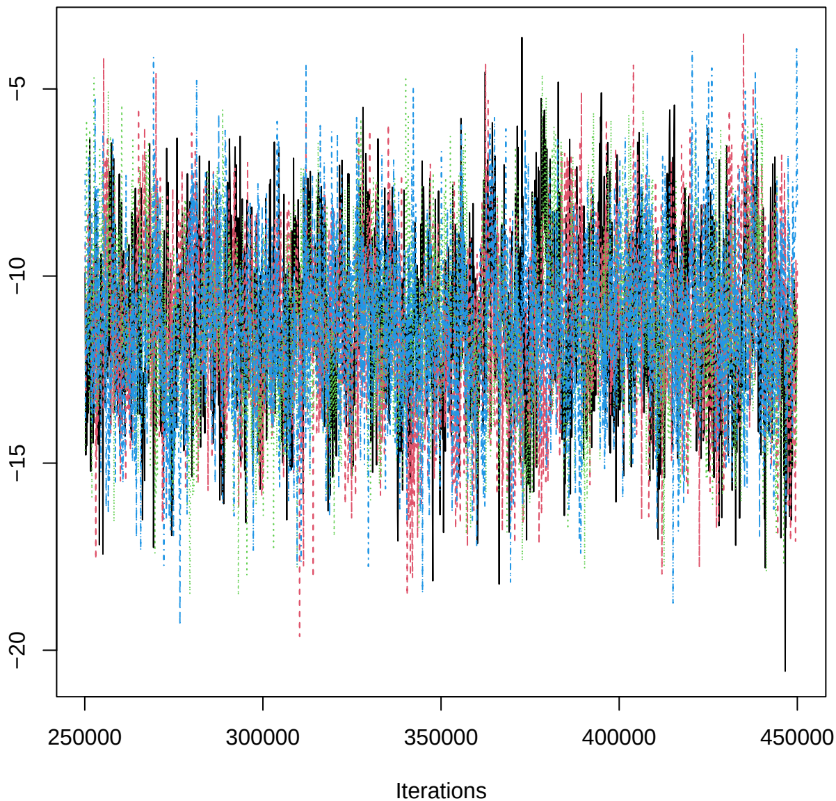
Traceplot – B[(Intercept) (C1), EPB_n (S6)]
