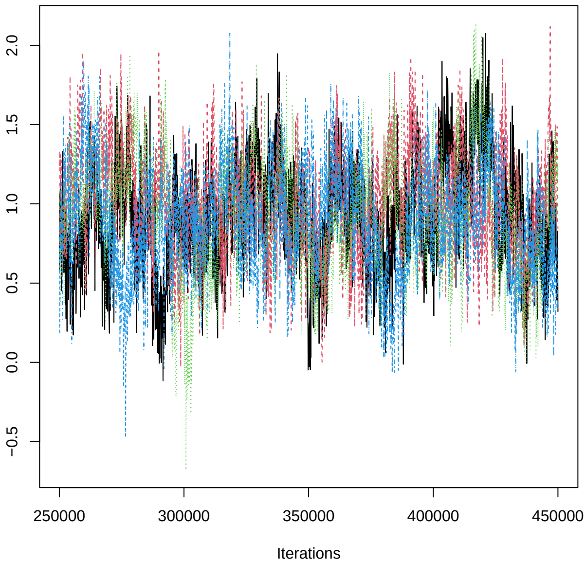
Traceplot – B[rtp (C7), PIG_n (S14)]
