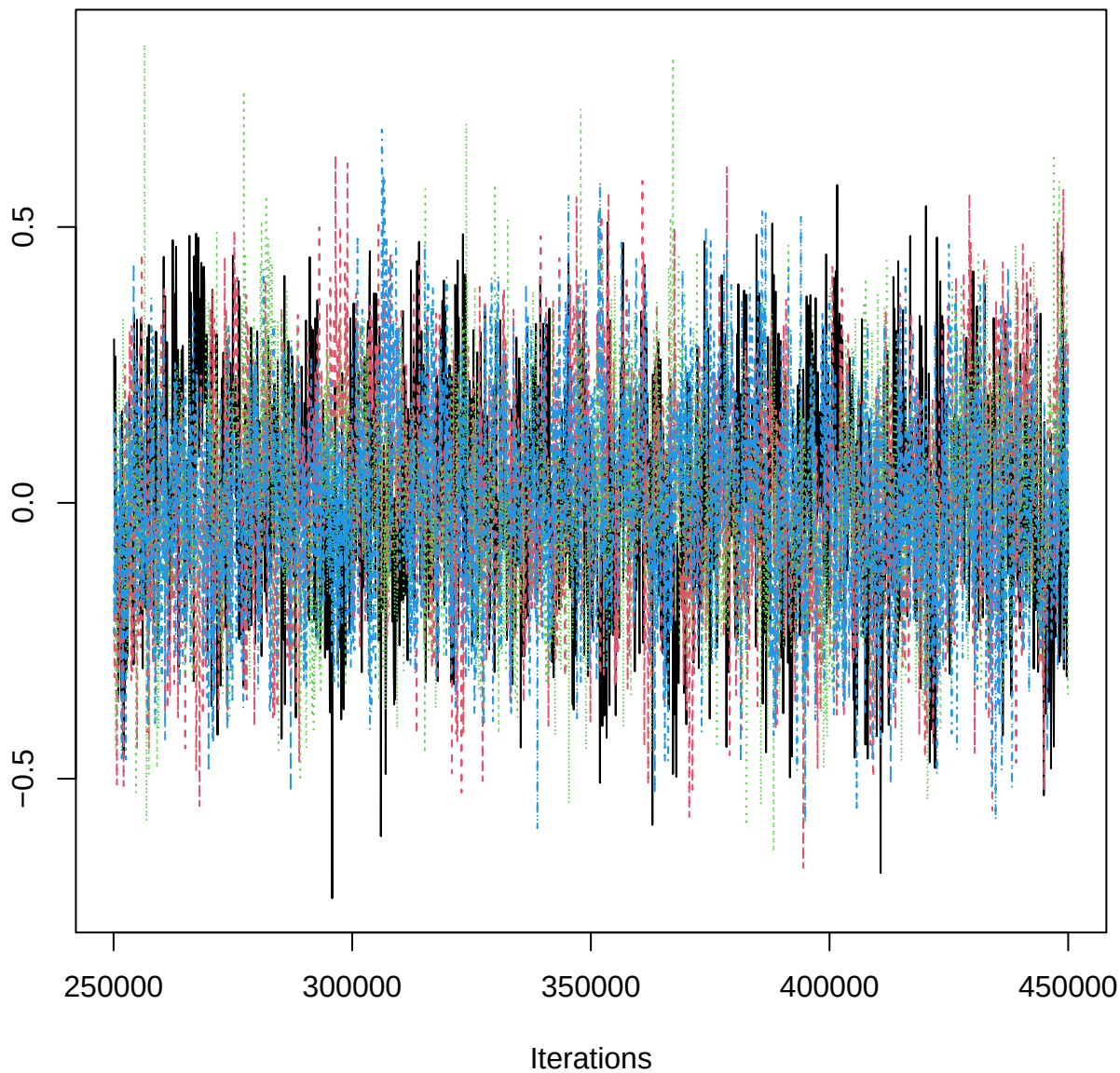
Traceplot – B[aspect_classSE (C15), EPN_n (S9)]
