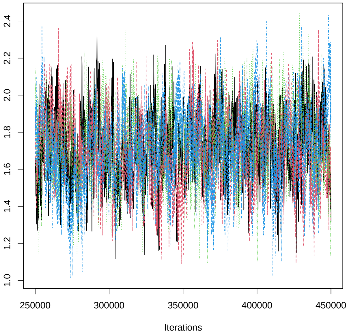
Traceplot – B[rtp (C7), ERR_n (S1)]
