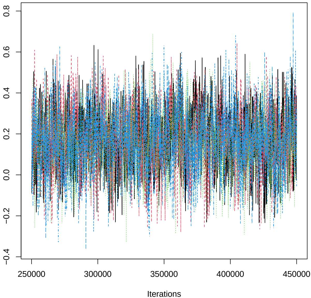
Traceplot – B[rtp (C7), BOP_n (S5)]
