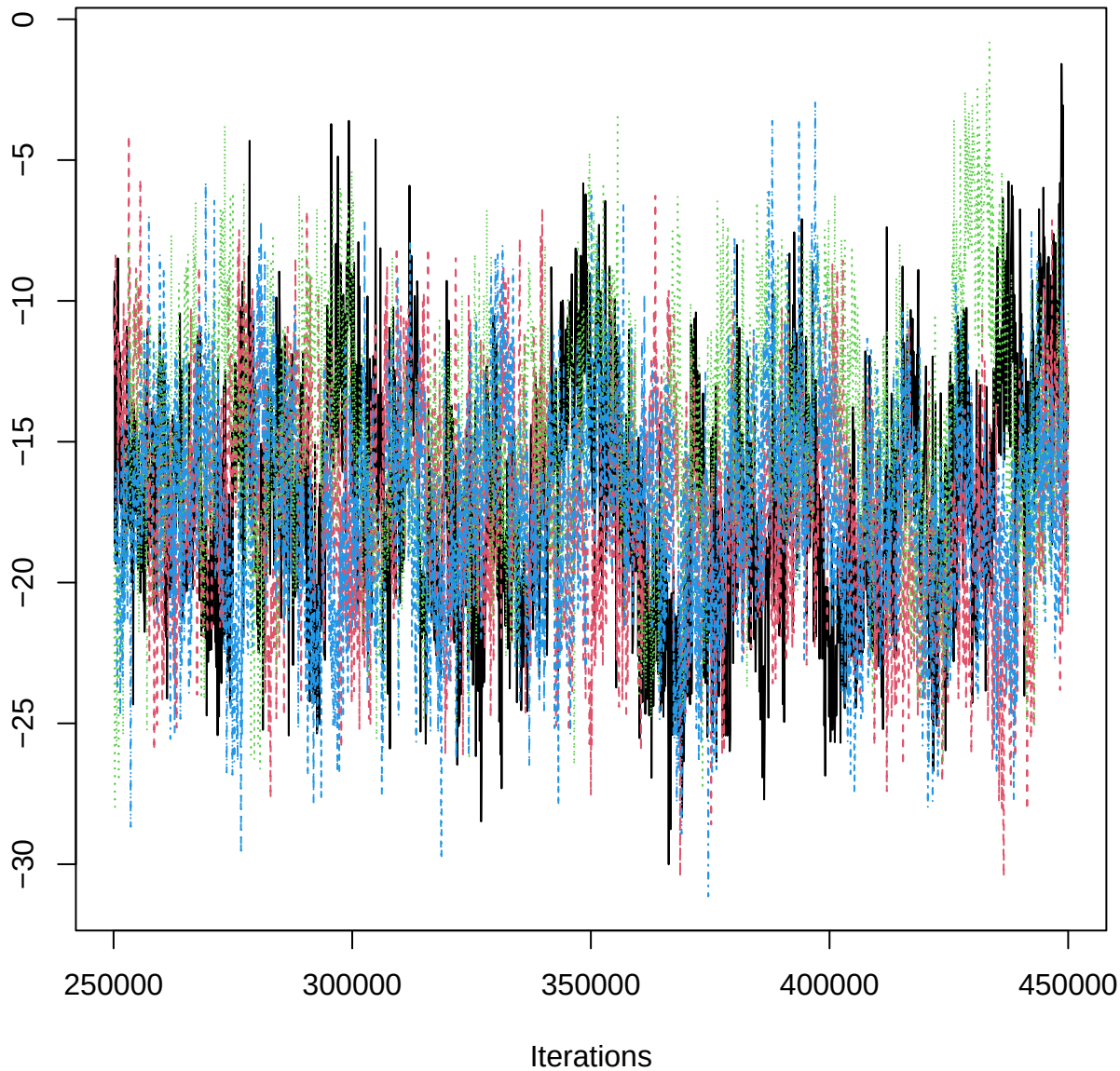
Traceplot – B[(Intercept) (C1), THO_n (S10)]
