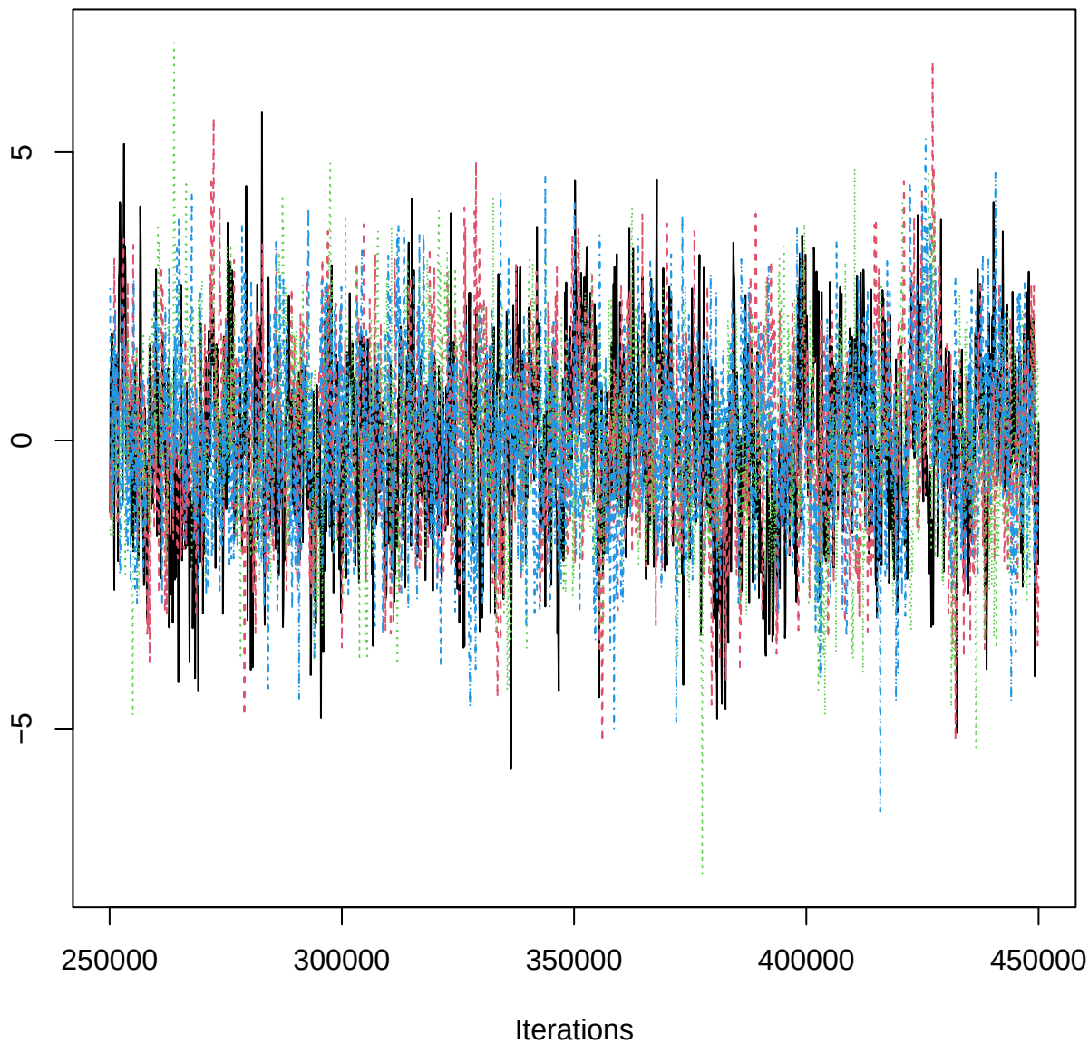
Traceplot – B[aspect_classFlat (C10), SAB_n (S8)]
