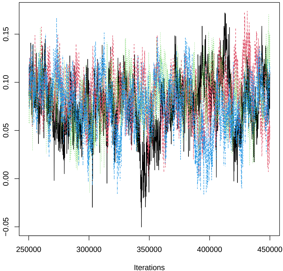
Traceplot – B[slope (C9), PIB_n (S13)]
