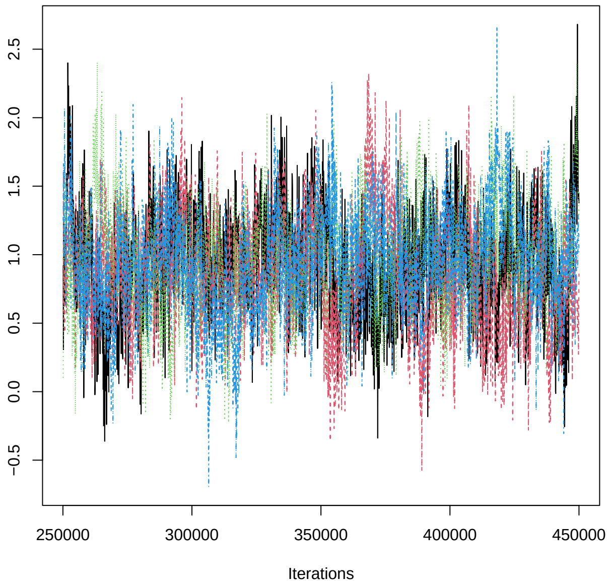
Traceplot – B[aspect_classNW (C13), THO_n (S10)]
