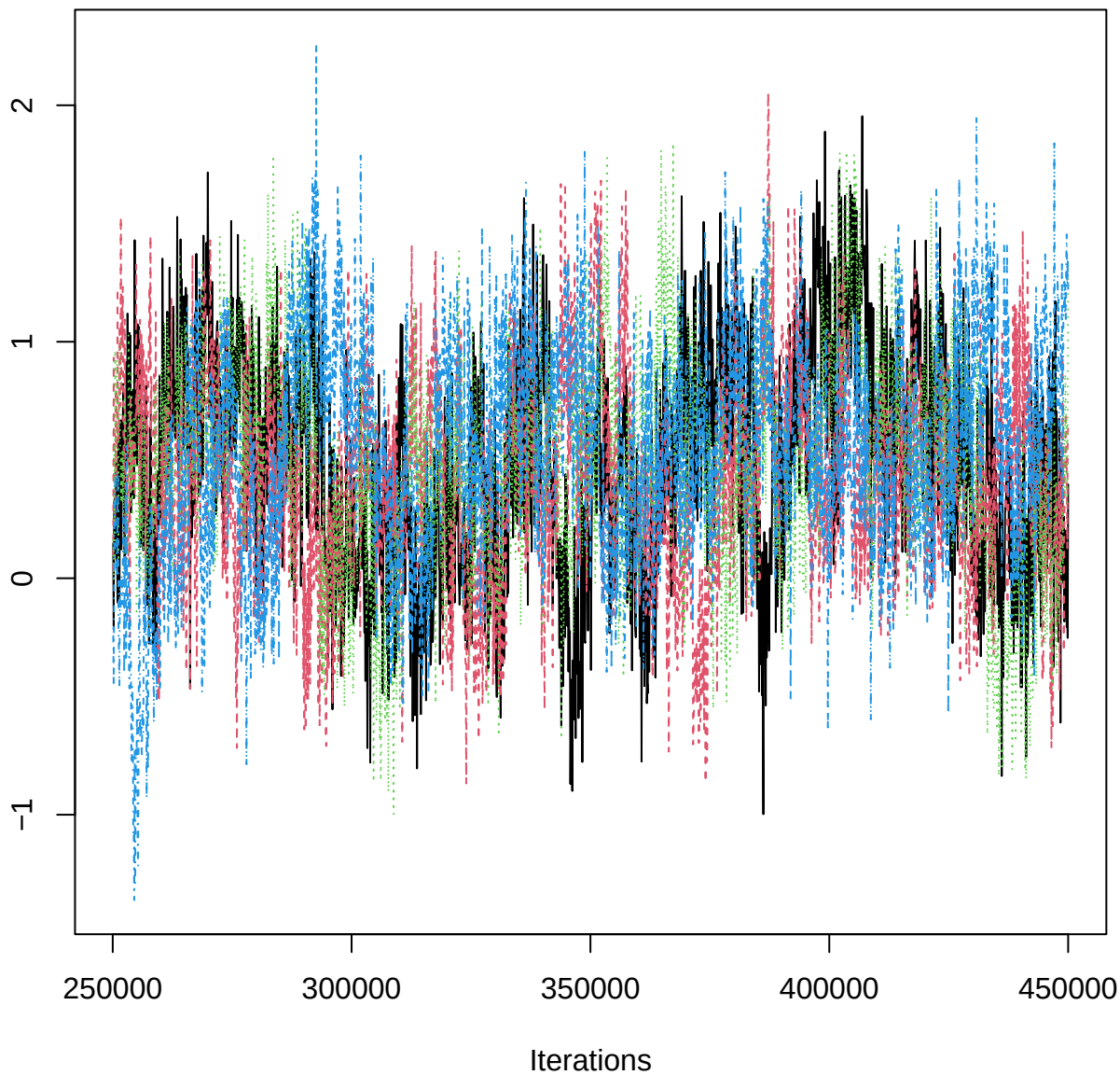
Traceplot – B[aspect_classN (C11), EPR_n (S7)]
