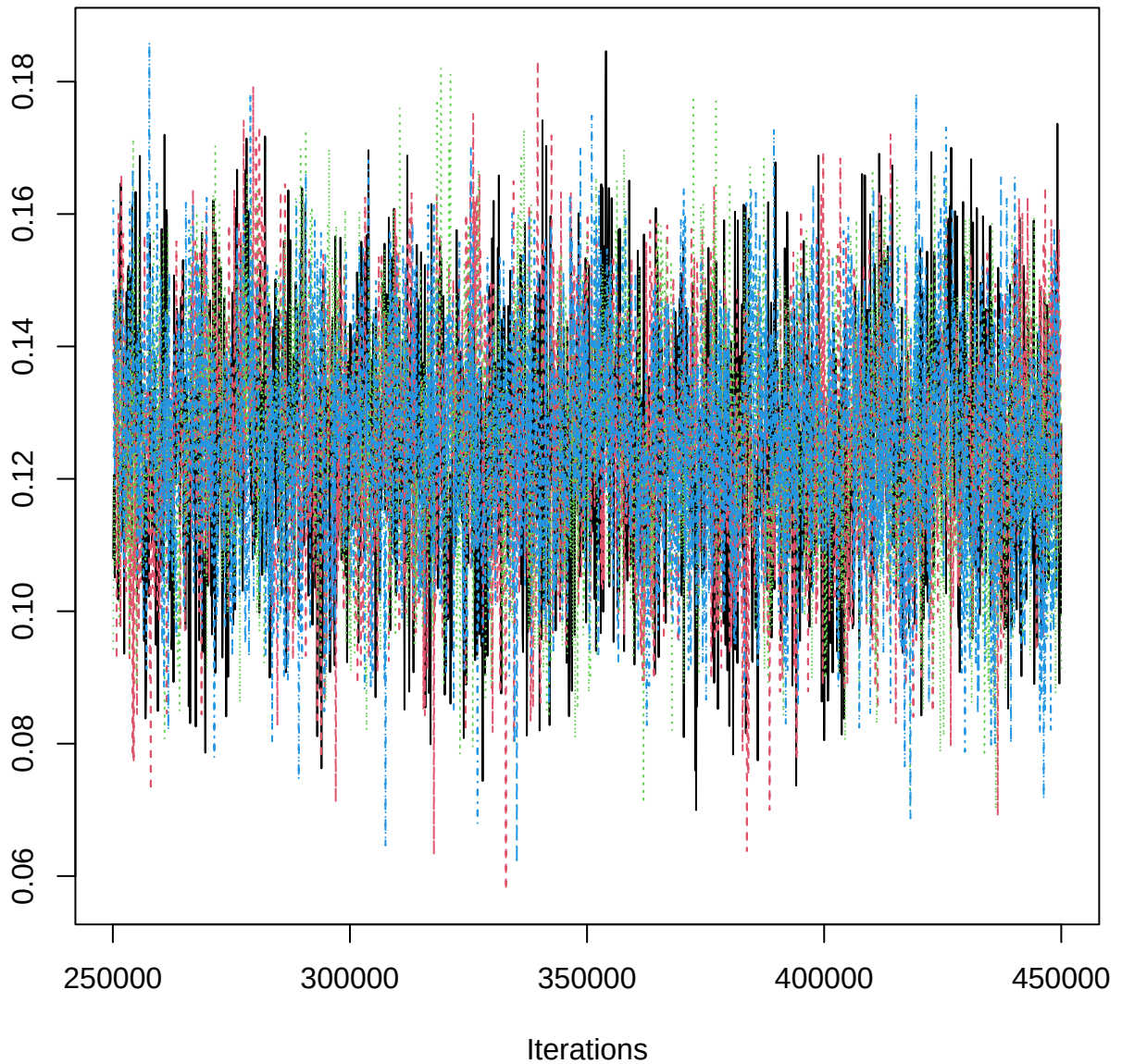
Traceplot – B[twi (C8), EPN_n (S9)]
