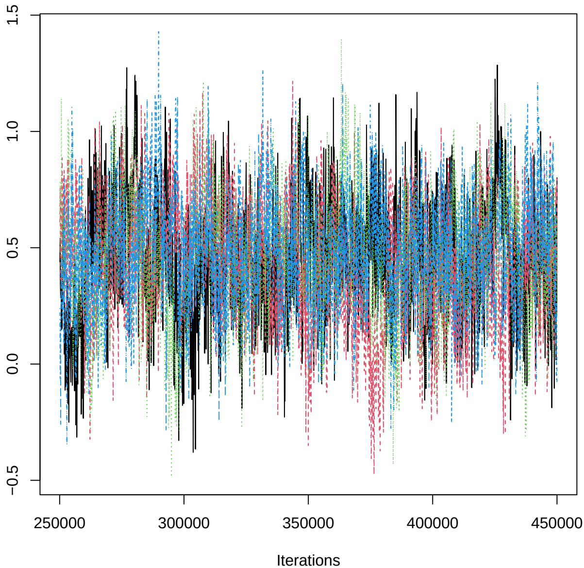
Traceplot – B[aspect_classN (C11), ERS_n (S2)]
