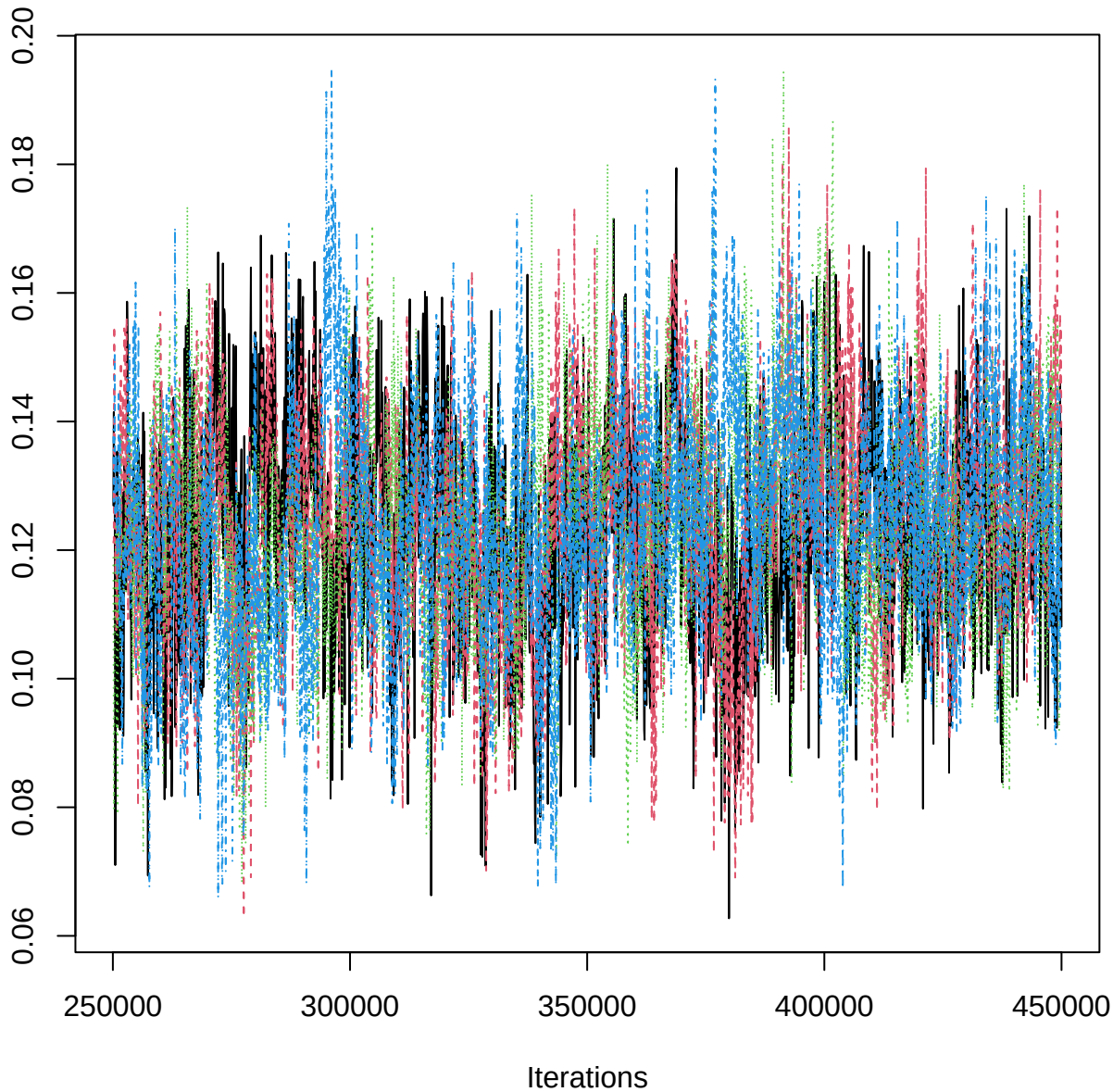
Traceplot – B[slope (C9), BOJ_n (S4)]
