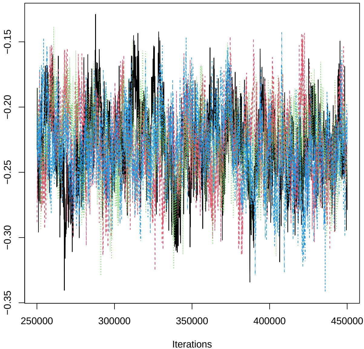
Traceplot – B[twi (C8), ERR_n (S1)]
