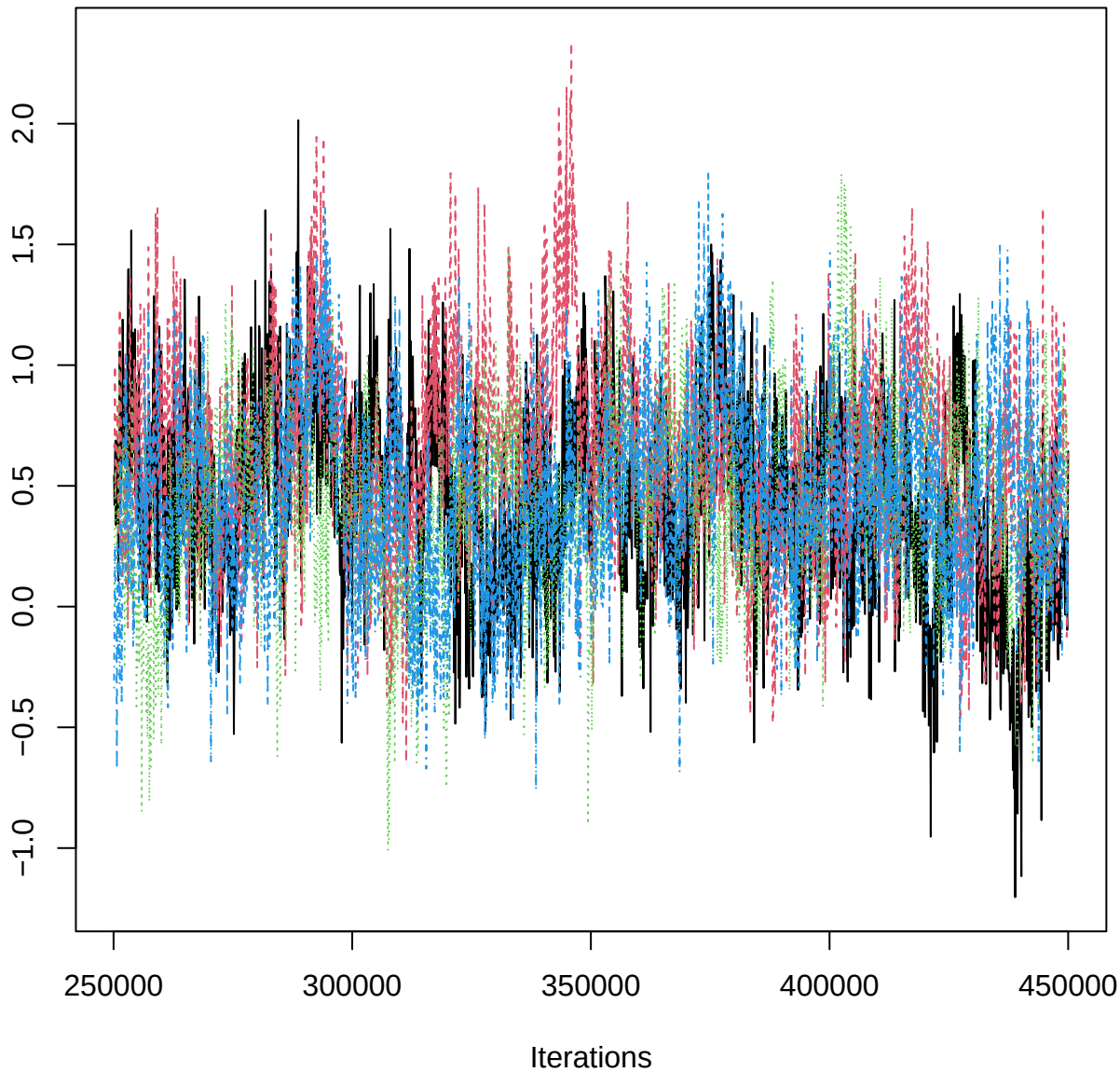
Traceplot – B[aspect_classS (C14), PRP_n (S11)]
