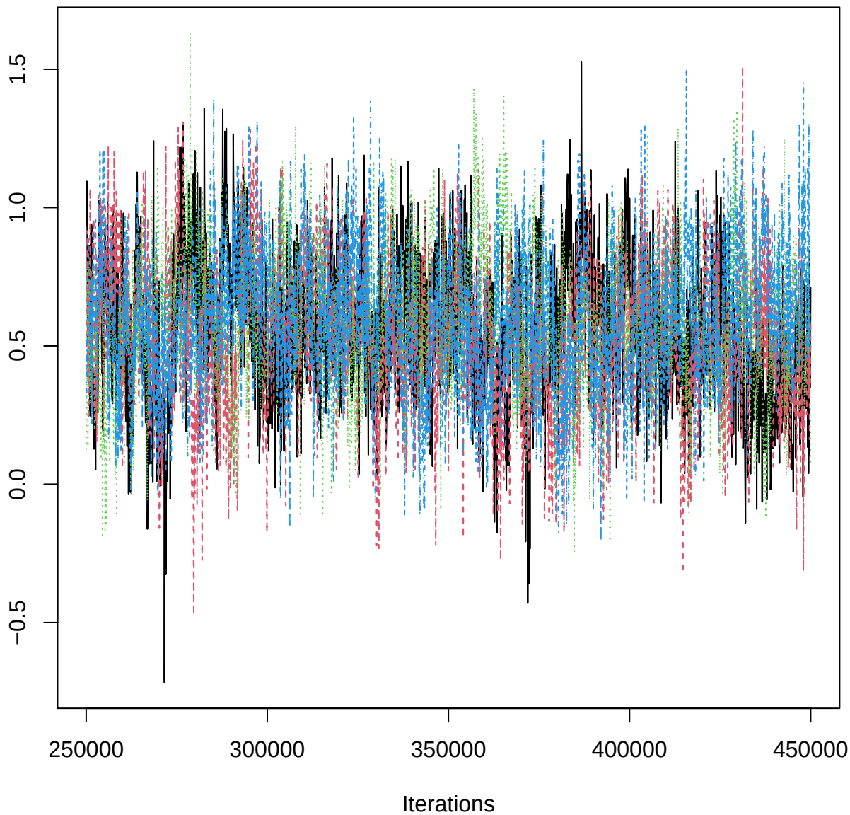
Traceplot – B[aspect_classS (C14), ERS_n (S2)]
