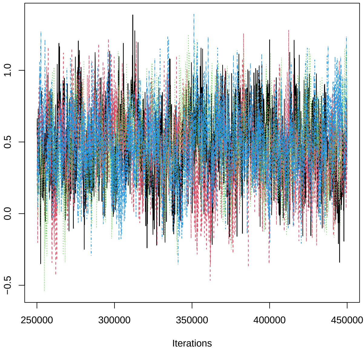
Traceplot – B[aspect_classNW (C13), BOJ_n (S4)]
