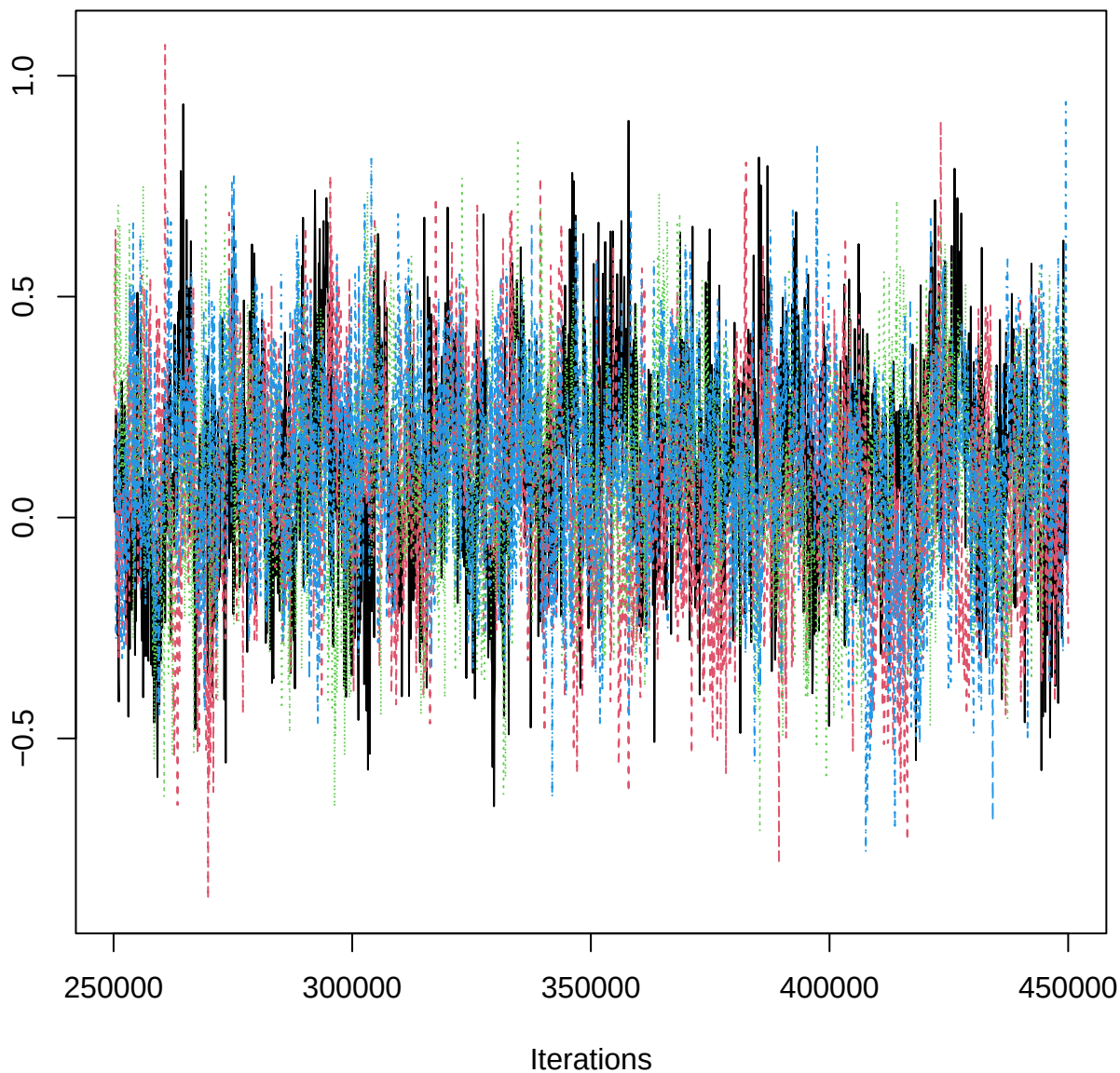
Traceplot – B[aspect_classN (C11), ERR_n (S1)]
