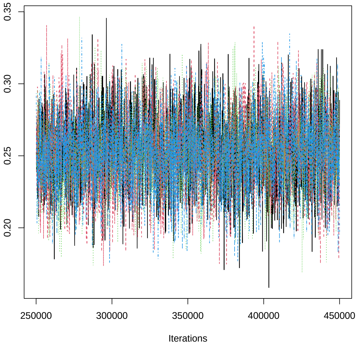
Traceplot – B[MAT (C3), SAB_n (S8)]
