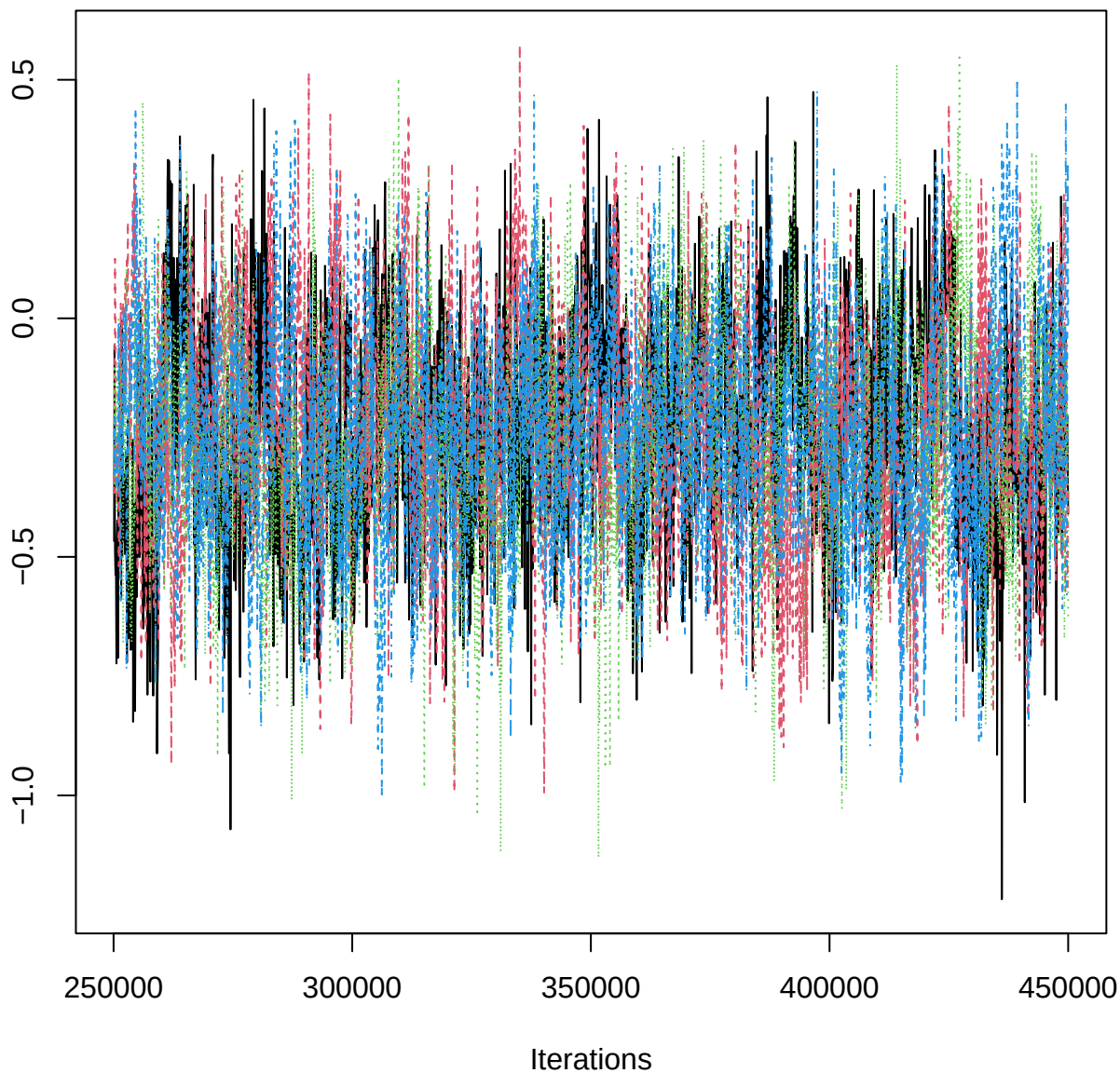
Traceplot – B[aspect_classNE (C12), ERR_n (S1)]
