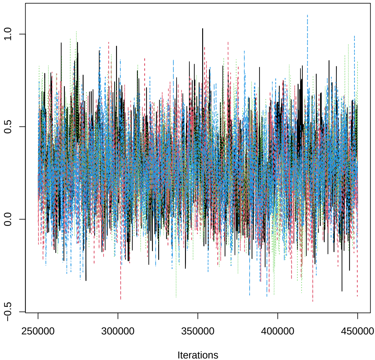
Traceplot – B[aspect_classNW (C13), EPB_n (S6)]
