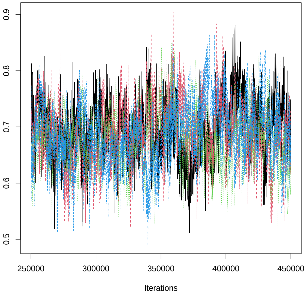
Traceplot – B[OM (C6), BOJ_n (S4)]
