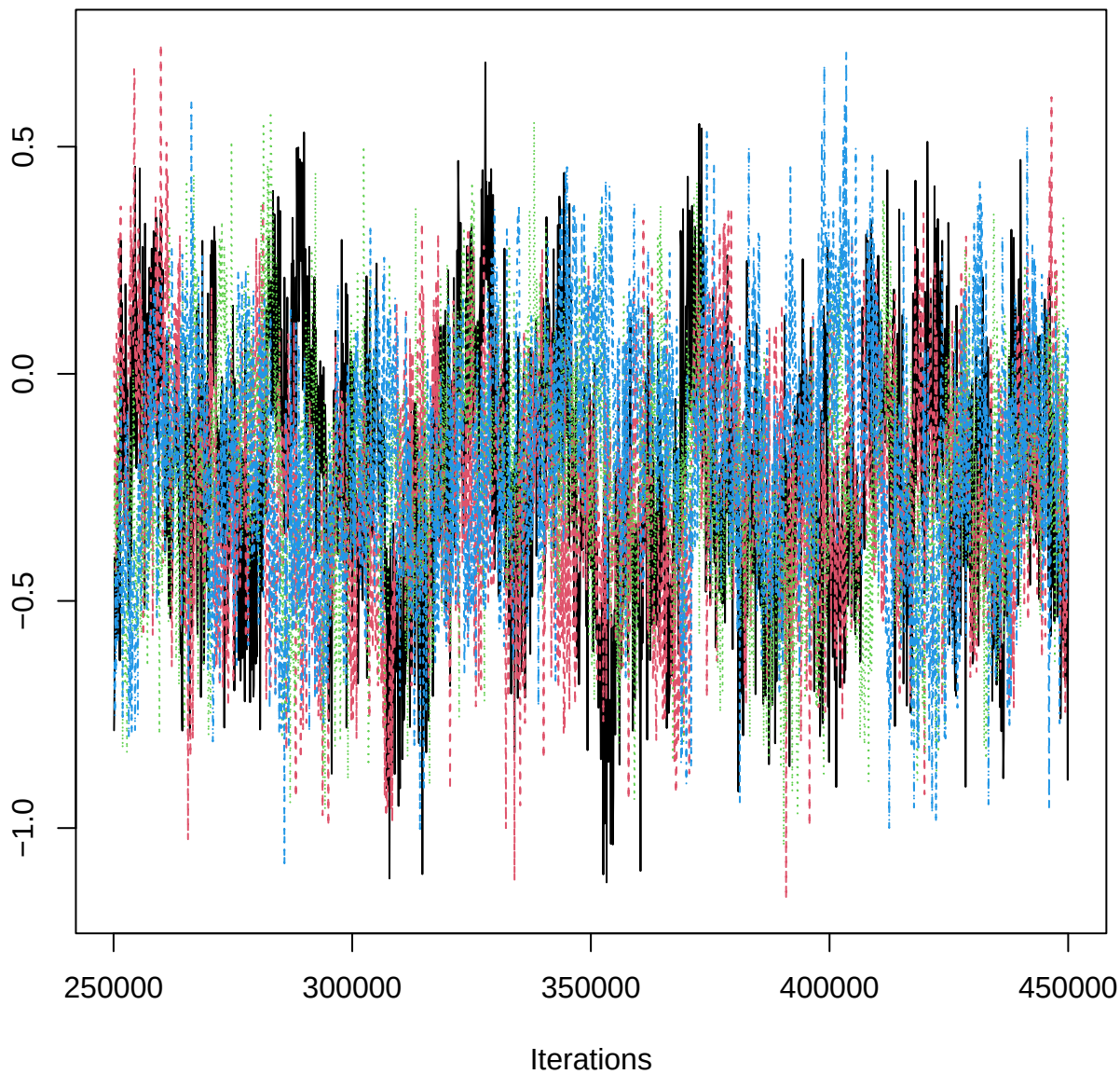
Traceplot – B[rtp (C7), PET_n (S12)]
