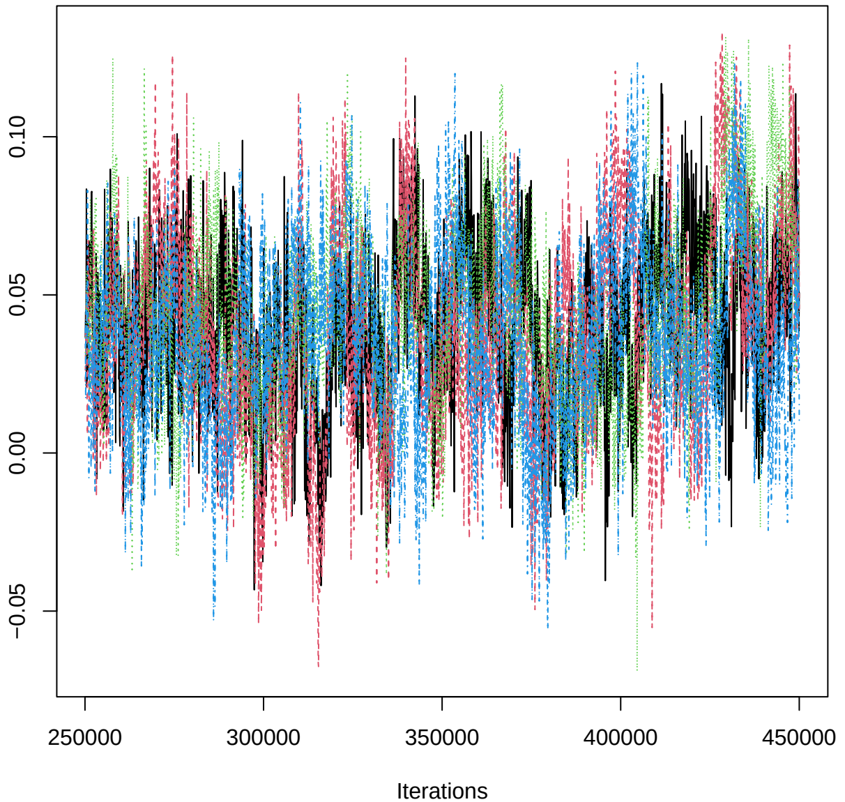
Traceplot – B[slope (C9), PRP_n (S11)]
