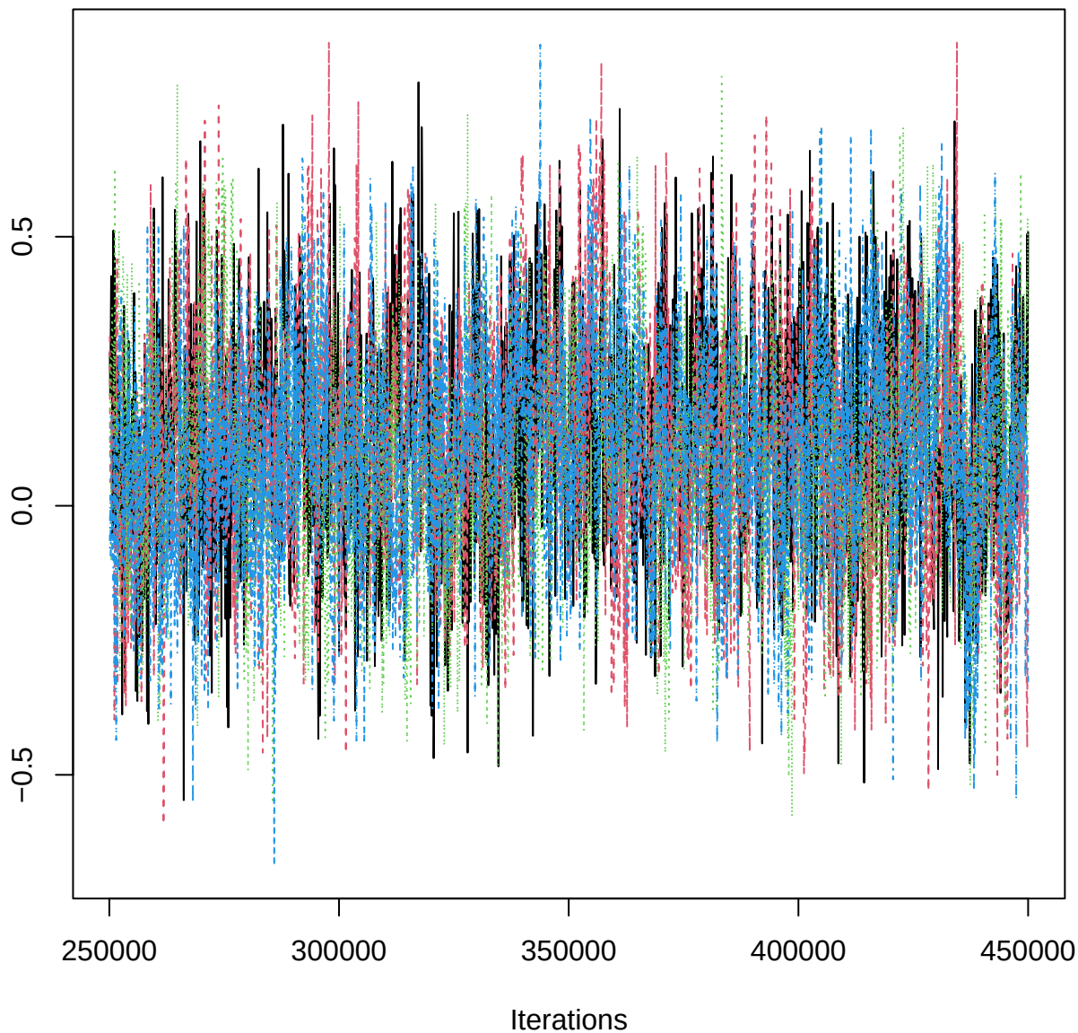
Traceplot – B[aspect_classN (C11), EPB_n (S6)]
