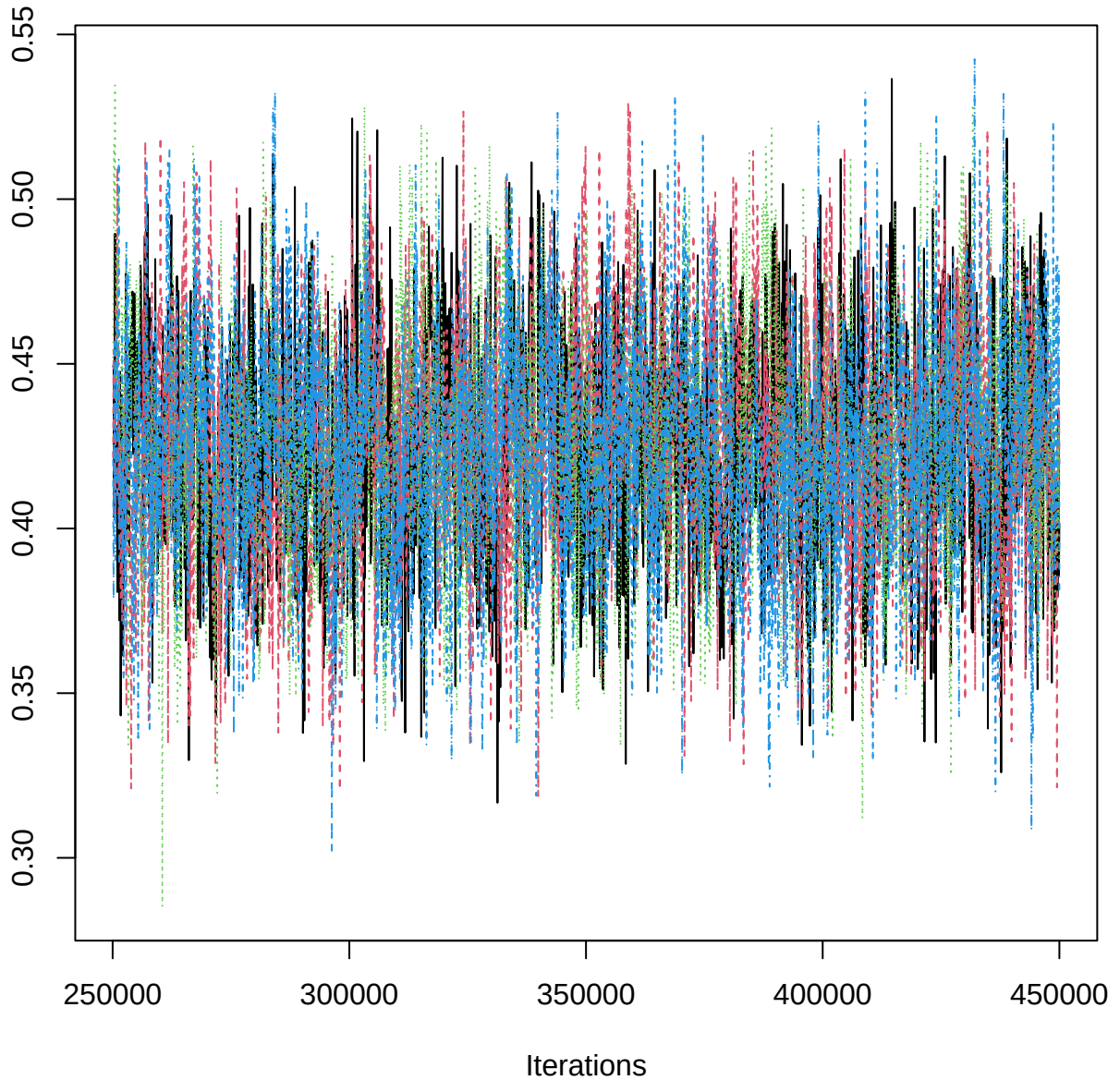
Traceplot – B[MAT (C3), BOP_n (S5)]
