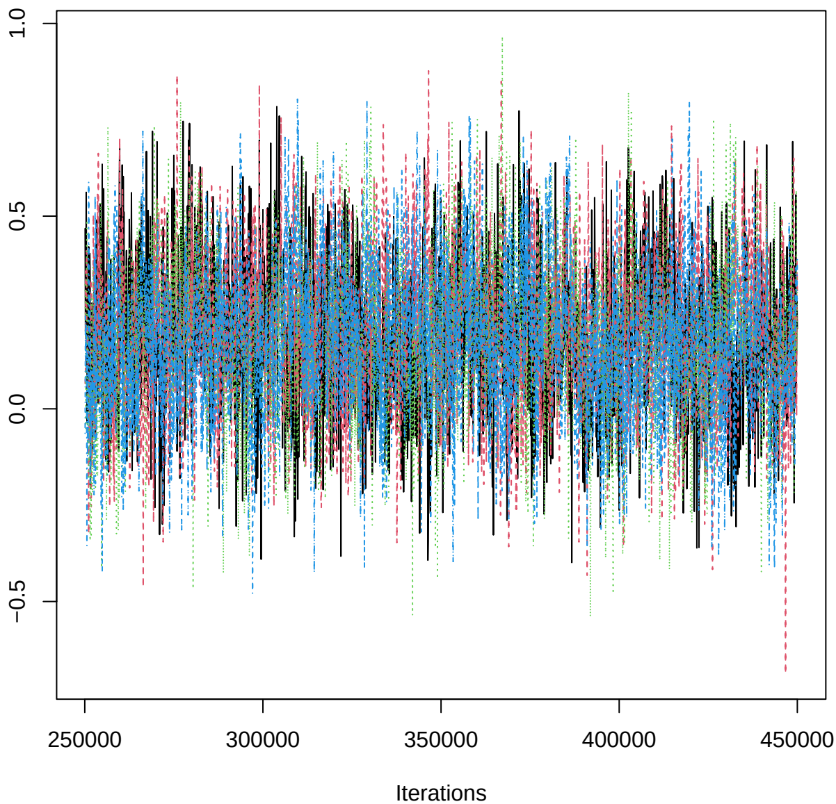
Traceplot – B[aspect_classS (C14), EPN_n (S9)]
