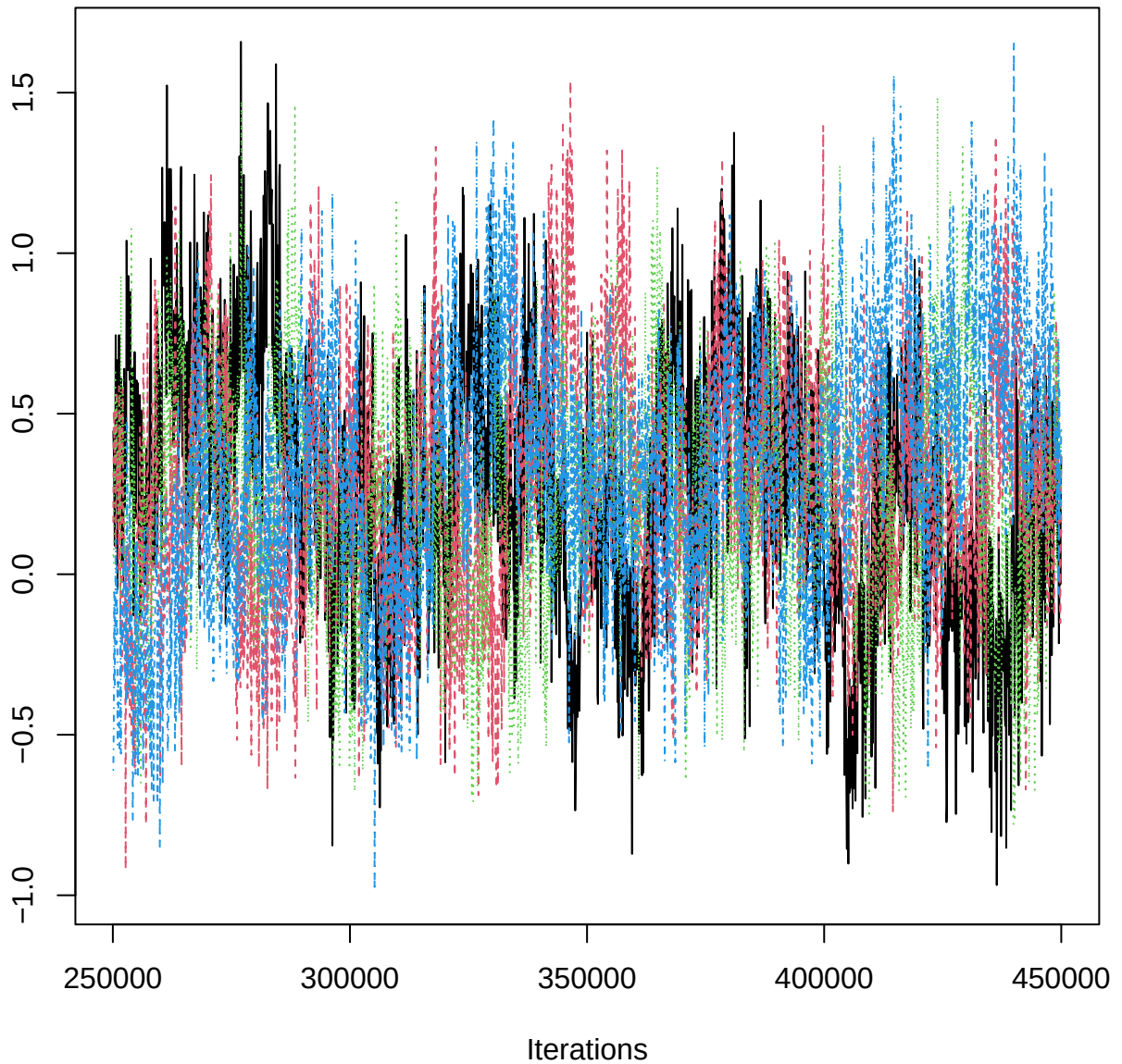
Traceplot – B[aspect_classN (C11), PRP_n (S11)]
