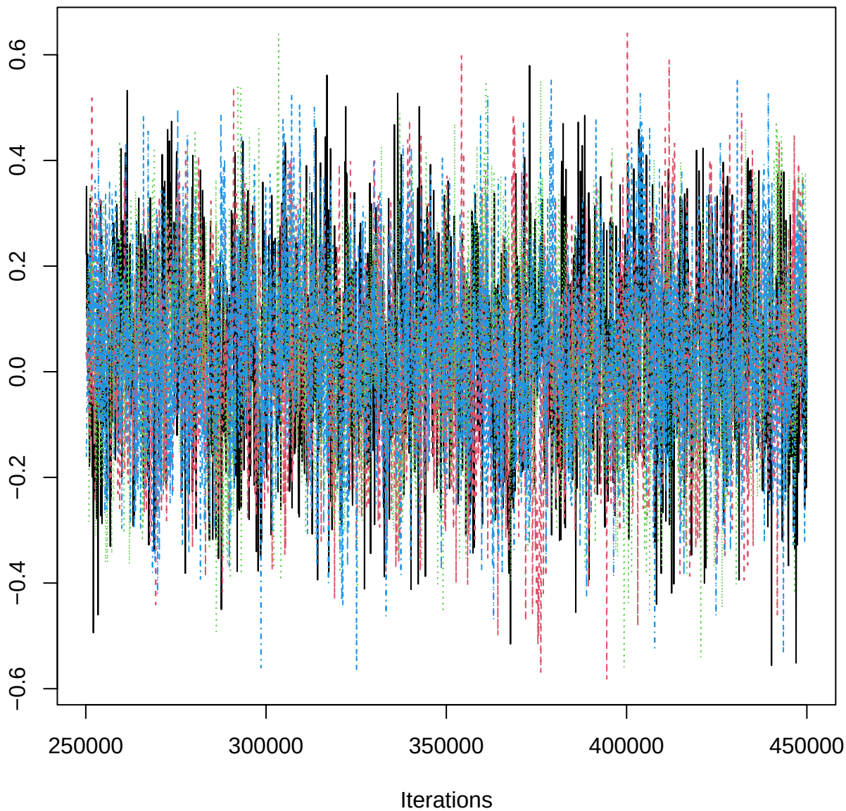
Traceplot – B[aspect_classW (C17), BOP_n (S5)]
