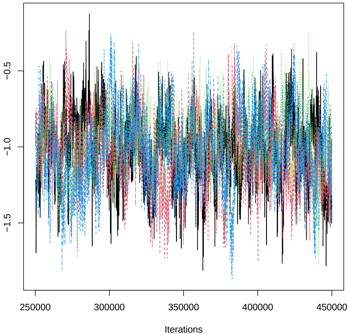
Traceplot – B[rtp (C7), BOJ_n (S4)]
