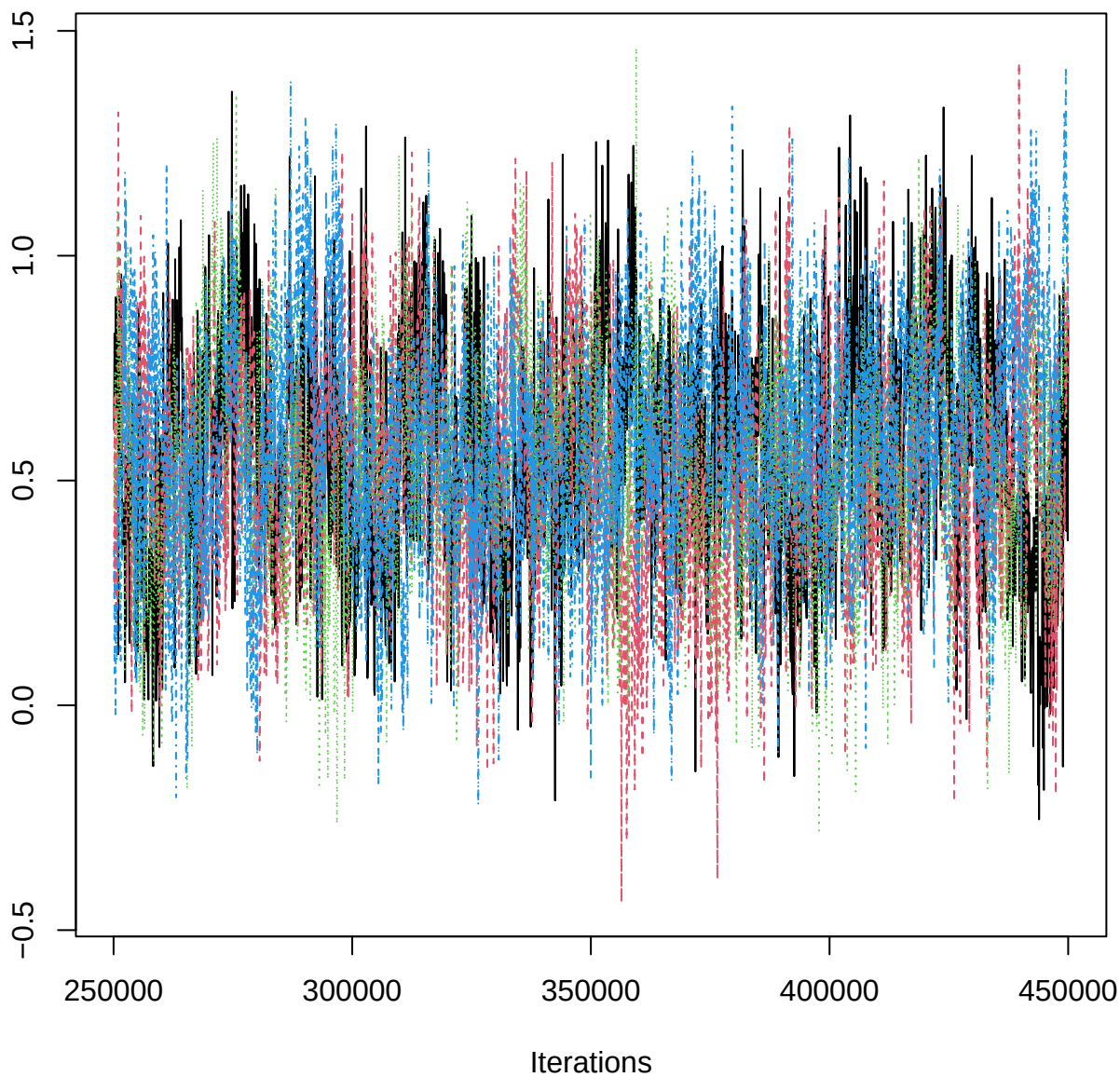
Traceplot – B[aspect_classN (C11), BOJ_n (S4)]
