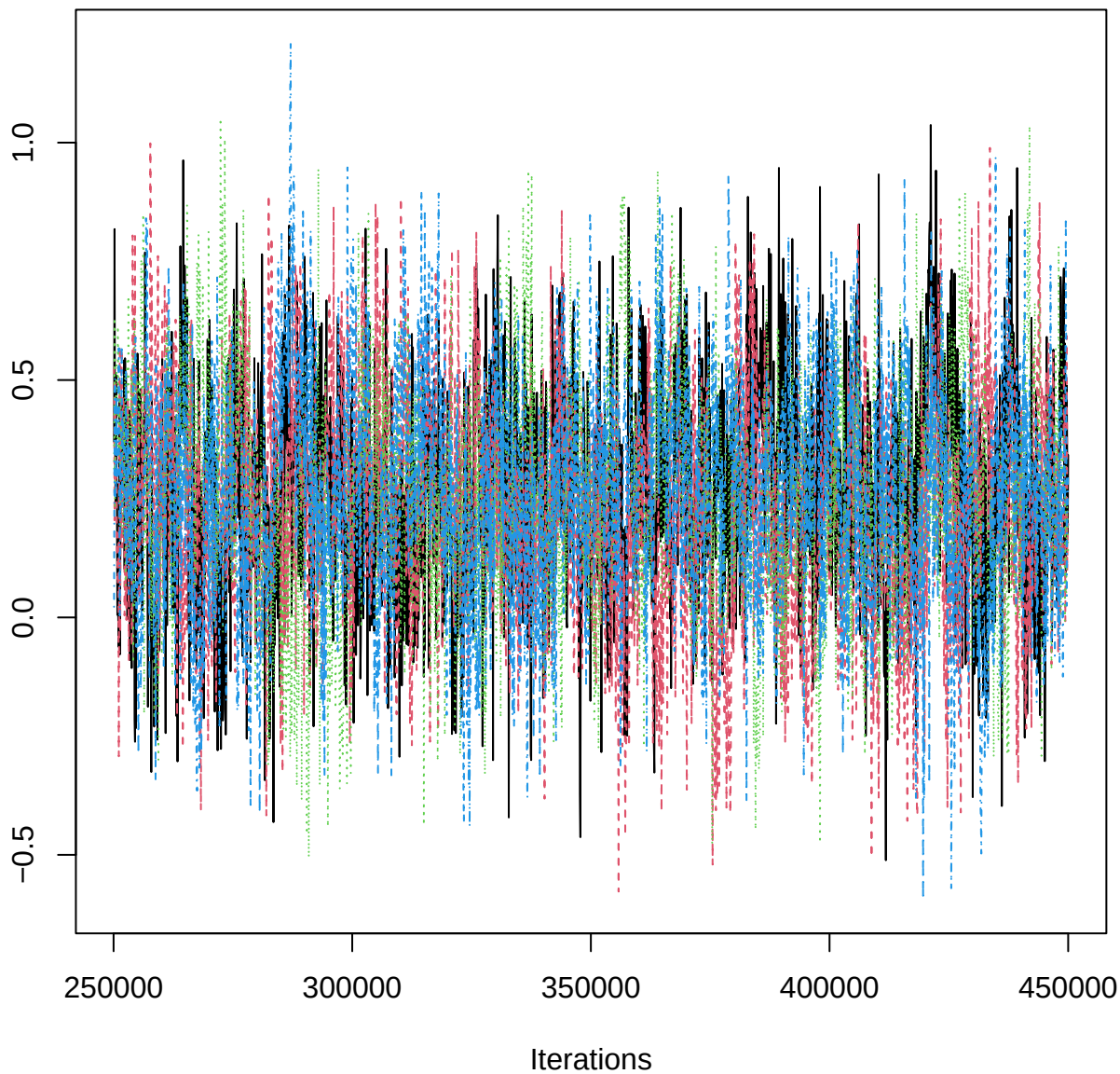
Traceplot – B[aspect_classSW (C16), ERR_n (S1)]
