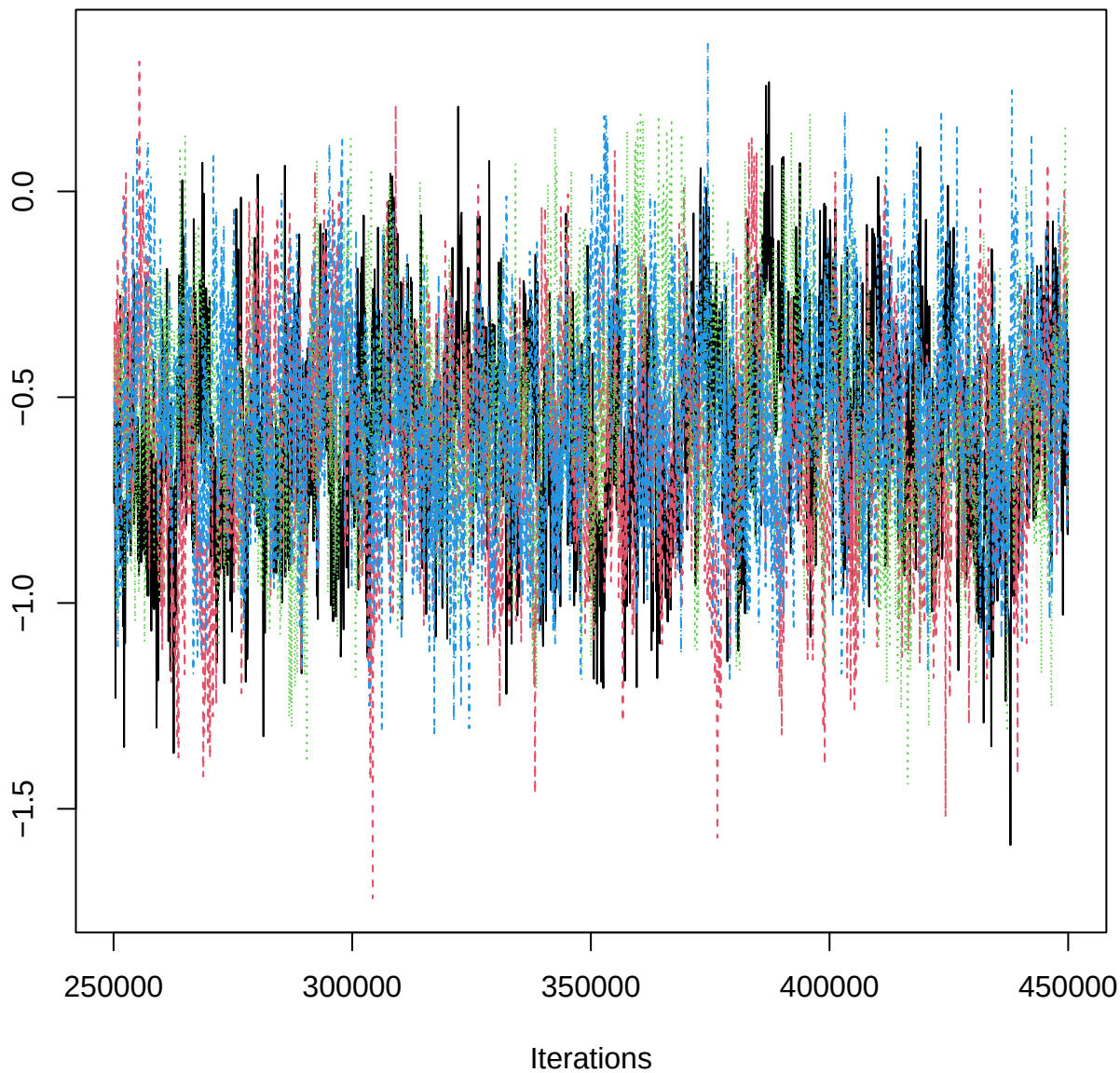
Traceplot – B[aspect_classW (C17), ERS_n (S2)]
