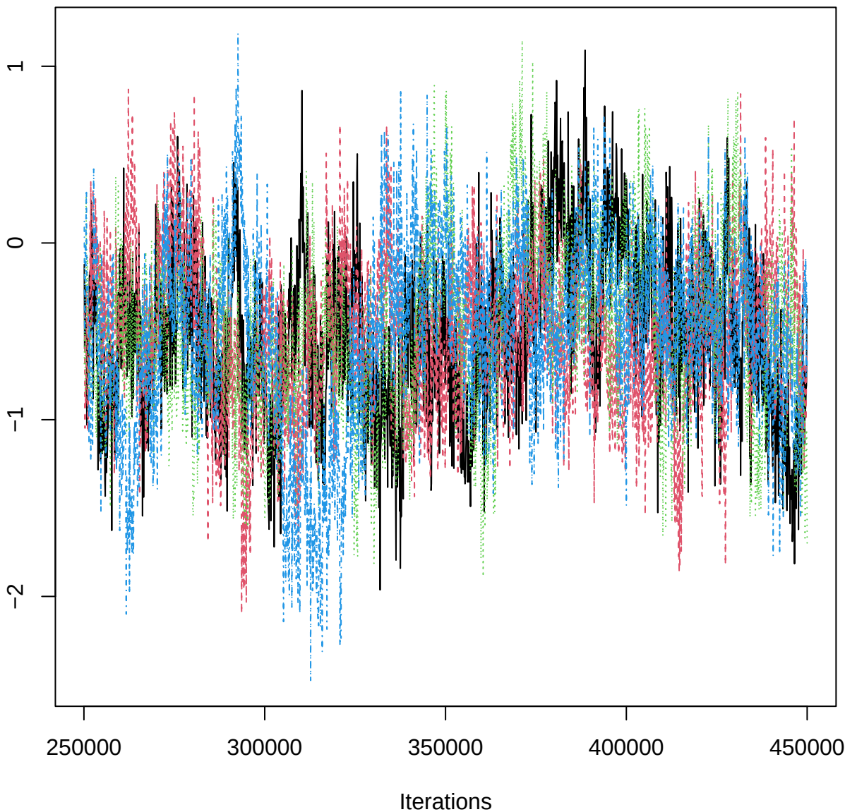
Traceplot – B[aspect_classSE (C15), EPR_n (S7)]
