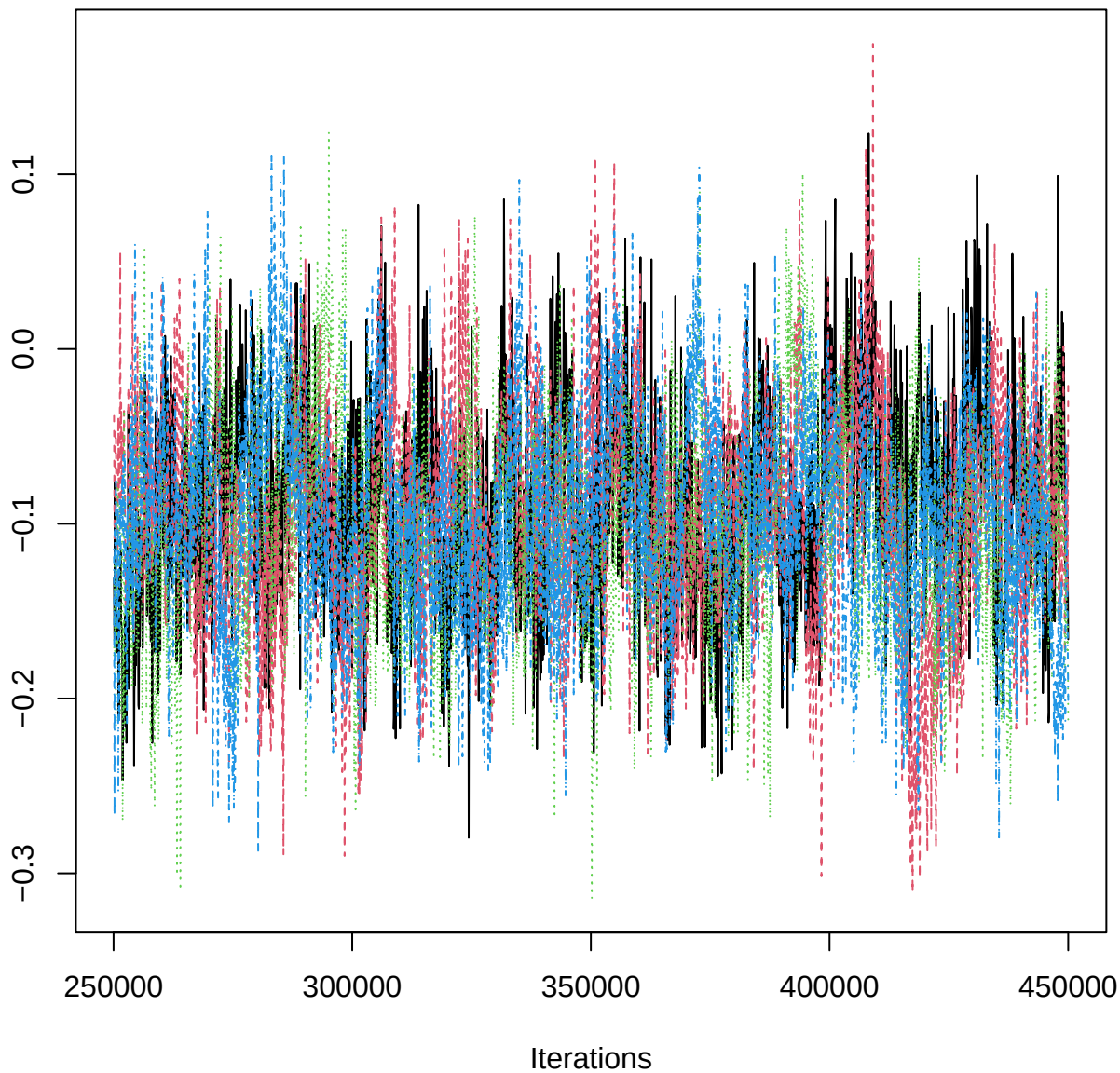
Traceplot – B[OM (C6), PET_n (S12)]
