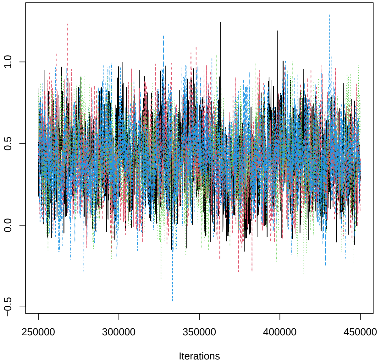
Traceplot – B[aspect_classW (C17), EPB_n (S6)]
