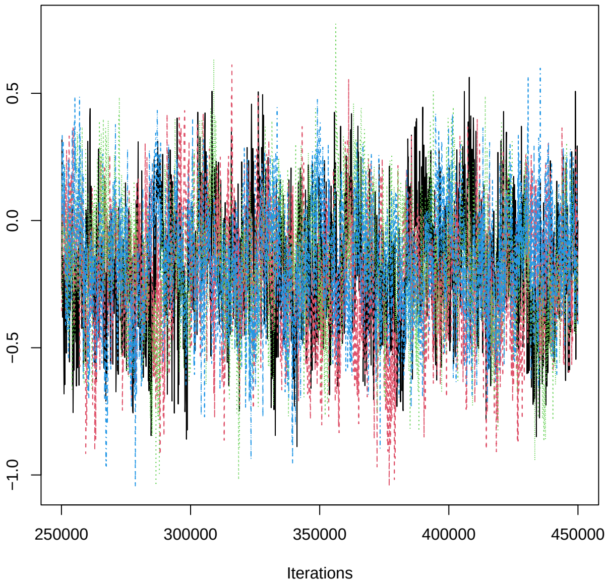
Traceplot – B[aspect_classW (C17), ERR_n (S1)]
