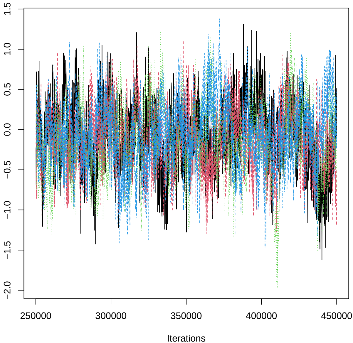
Traceplot – B[aspect_classS (C14), THO_n (S10)]
