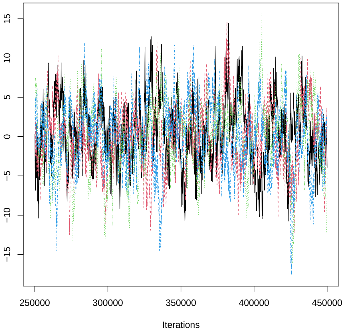
Traceplot – B[aspect_classFlat (C10), PIB_n (S13)]
