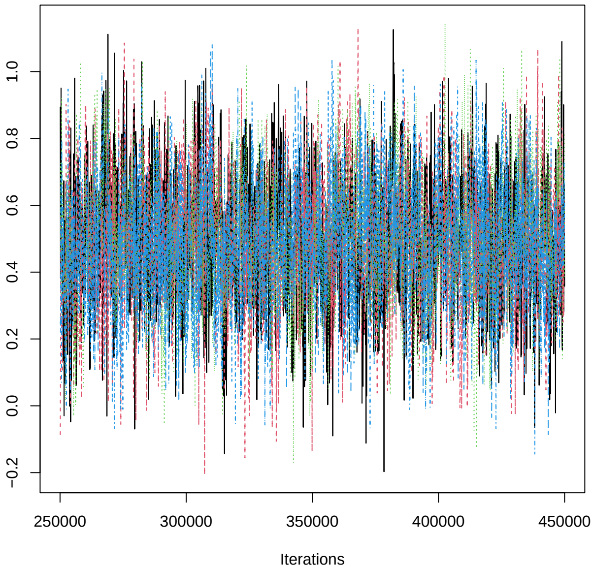
Traceplot – B[aspect_classW (C17), EPN_n (S9)]
