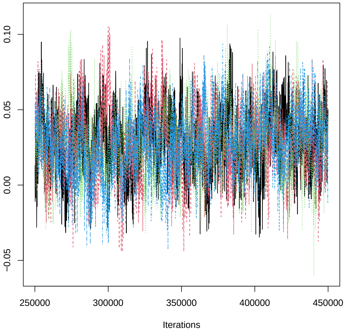
Traceplot – B[slope (C9), PET_n (S12)]
