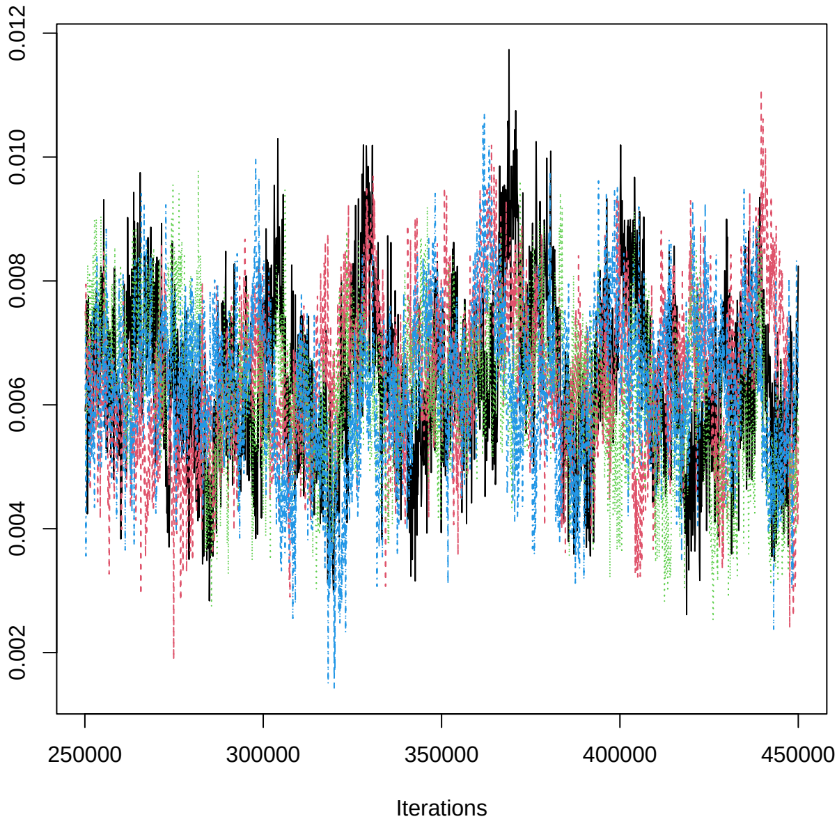
Traceplot – B[MAP (C2), PRP_n (S11)]
