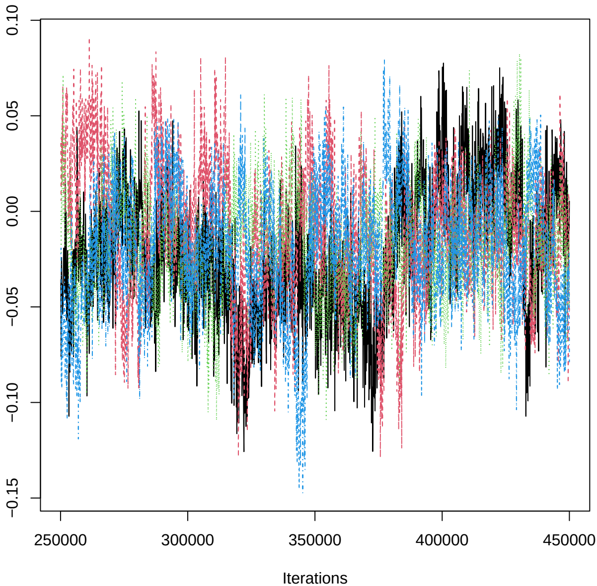
Traceplot – B[slope (C9), THO_n (S10)]
