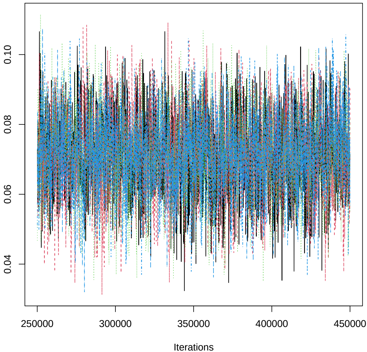
Traceplot – B[slope (C9), BOP_n (S5)]
