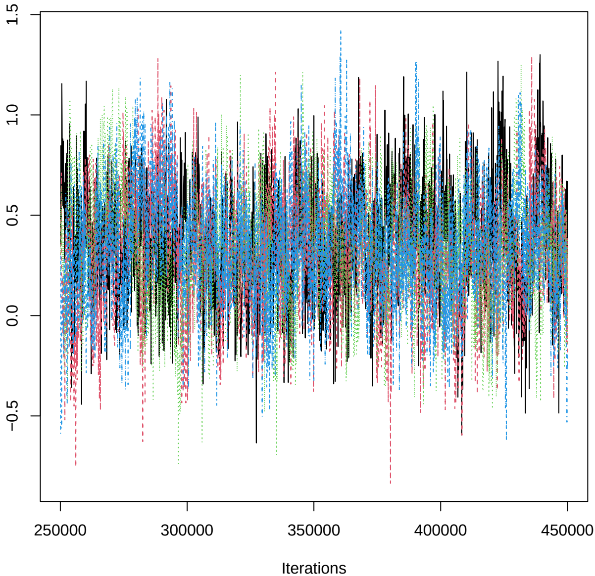
Traceplot – B[aspect_classSW (C16), PET_n (S12)]
