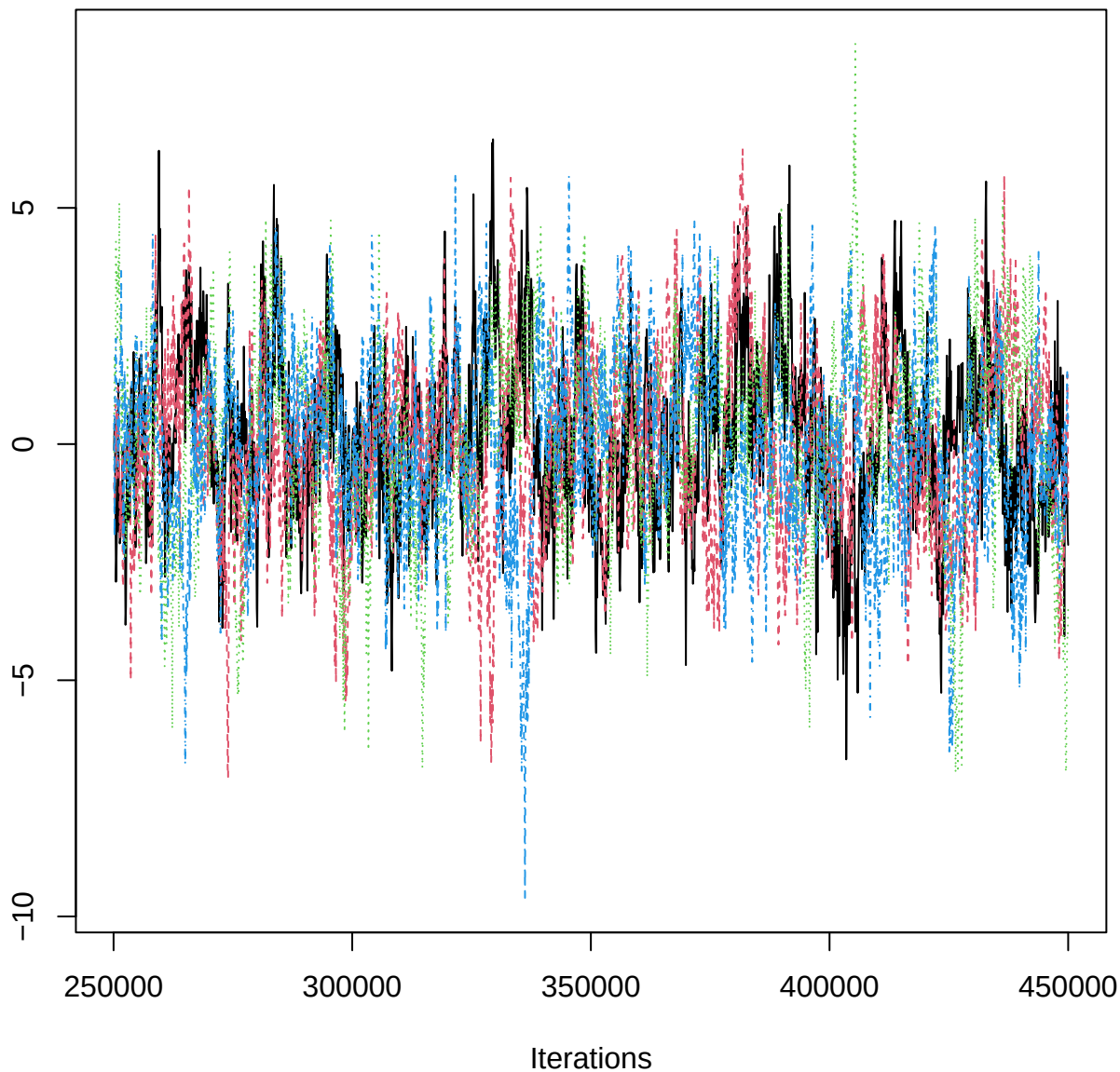
Traceplot – B[aspect_classFlat (C10), PET_n (S12)]
