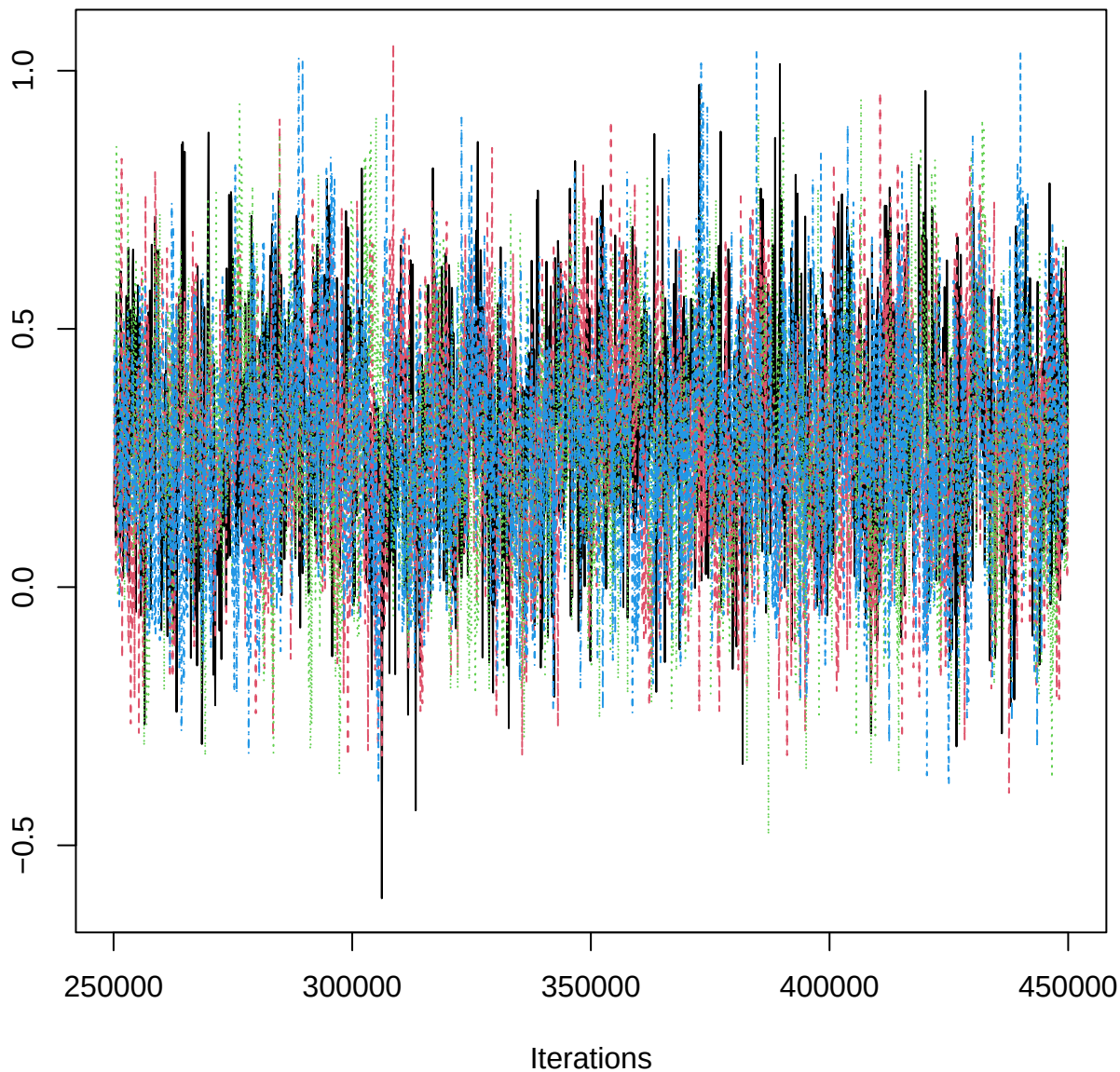
Traceplot – B[aspect_classSW (C16), EPB_n (S6)]
