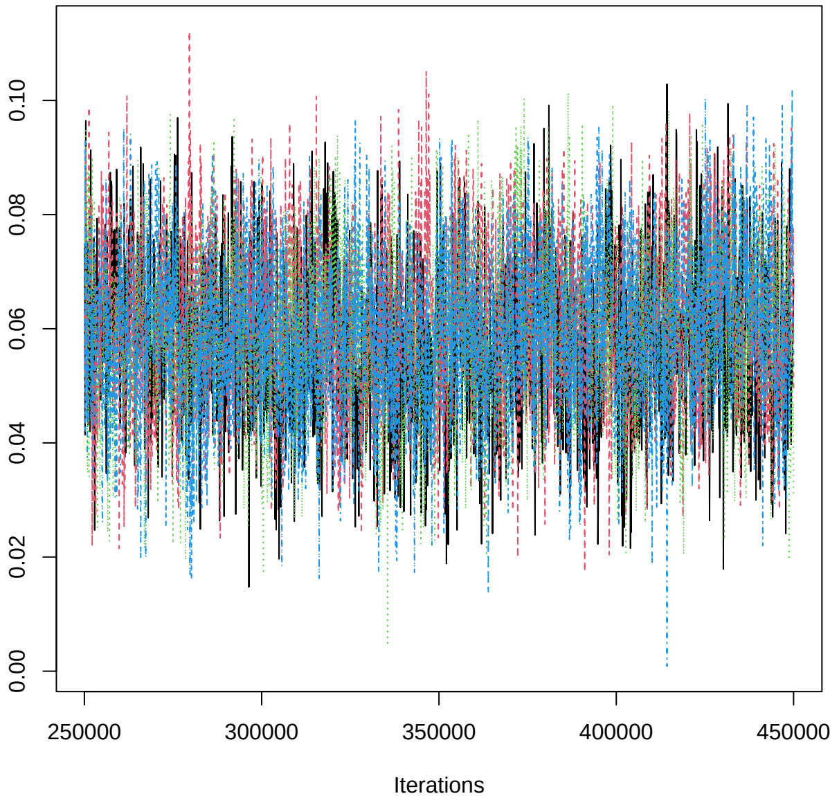
Traceplot – B[slope (C9), EPB_n (S6)]
