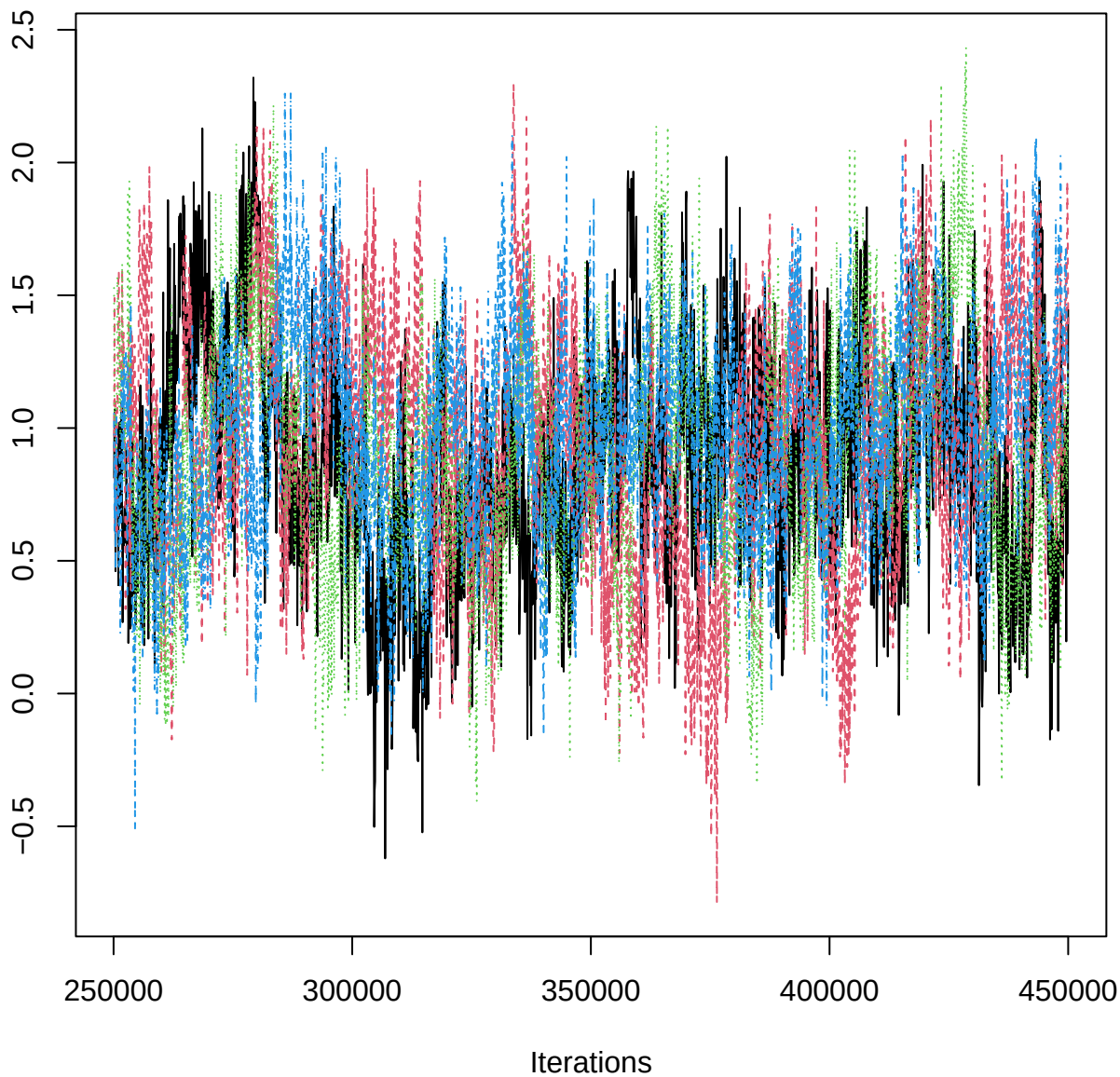
Traceplot – B[aspect_classN (C11), HEG_n (S3)]
