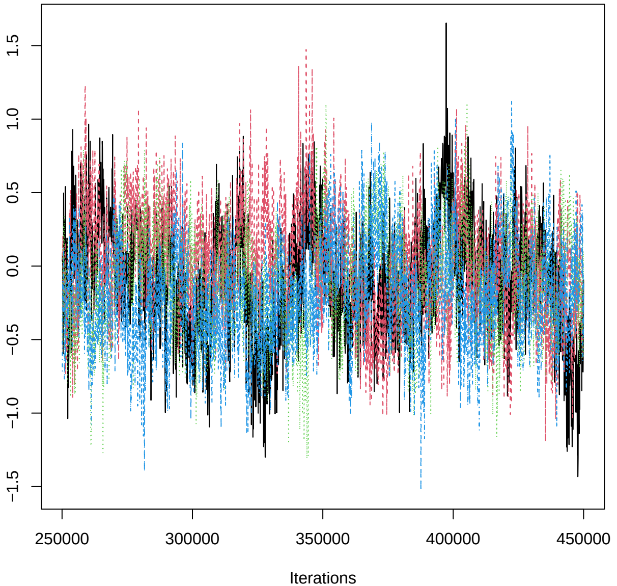
Traceplot – B[aspect_classSE (C15), PRP_n (S11)]
