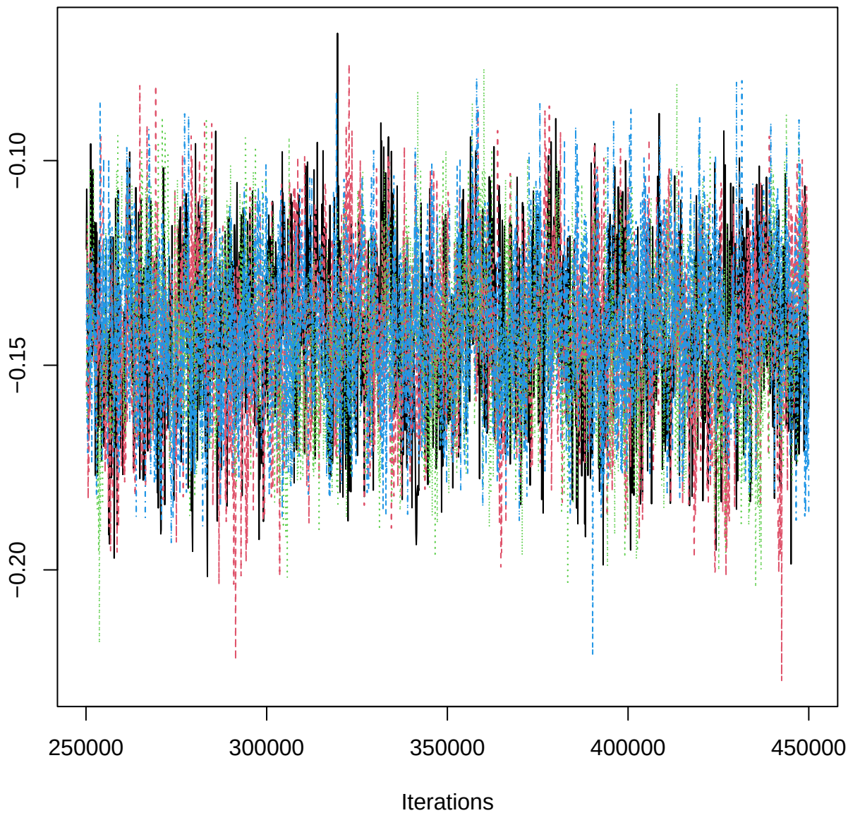
Traceplot – B[twi (C8), BOP_n (S5)]
