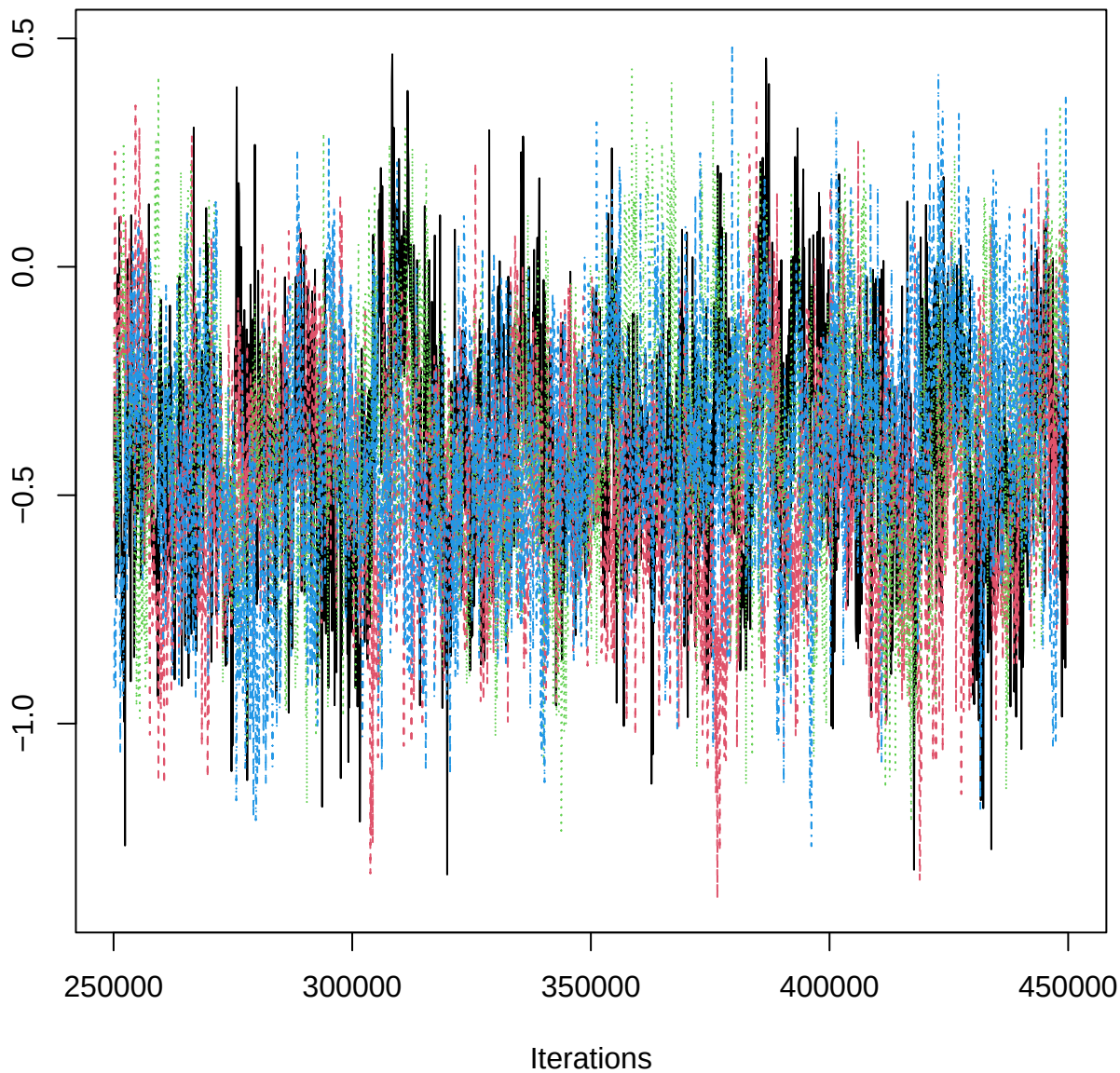
Traceplot – B[aspect_classW (C17), BOJ_n (S4)]
