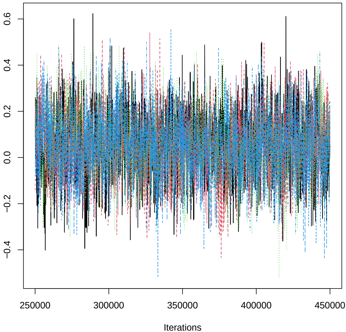
Traceplot – B[aspect_classW (C17), SAB_n (S8)]
