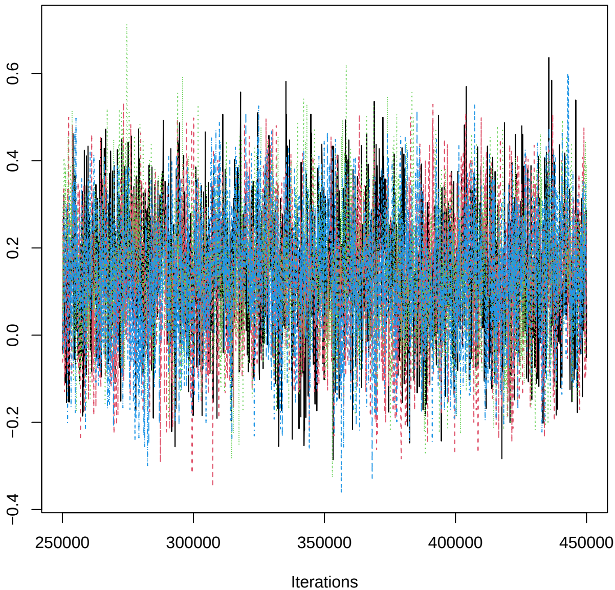
Traceplot – B[aspect_classNW (C13), SAB_n (S8)]
