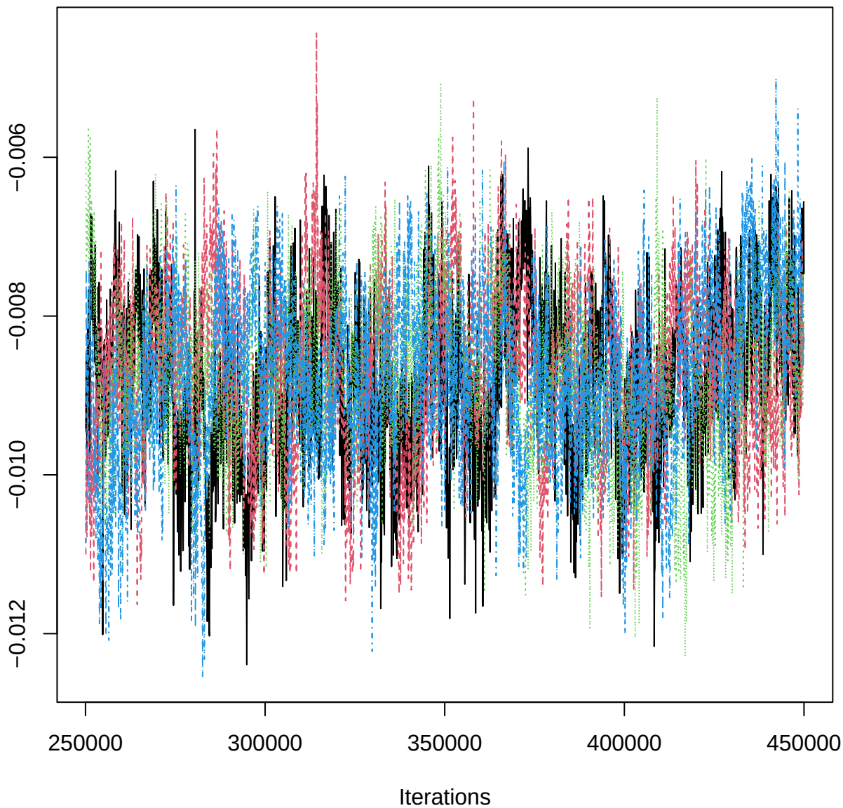
Traceplot – B[MAP (C2), PET_n (S12)]
