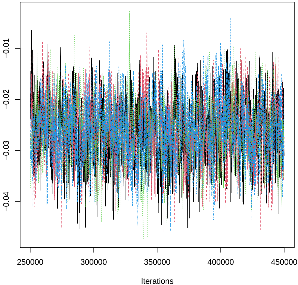
Traceplot – B[Clay (C5), BOP_n (S5)]
