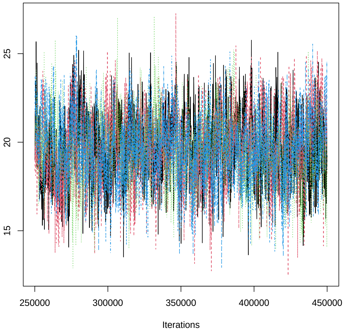
Traceplot – B[(Intercept) (C1), EPN_n (S9)]
