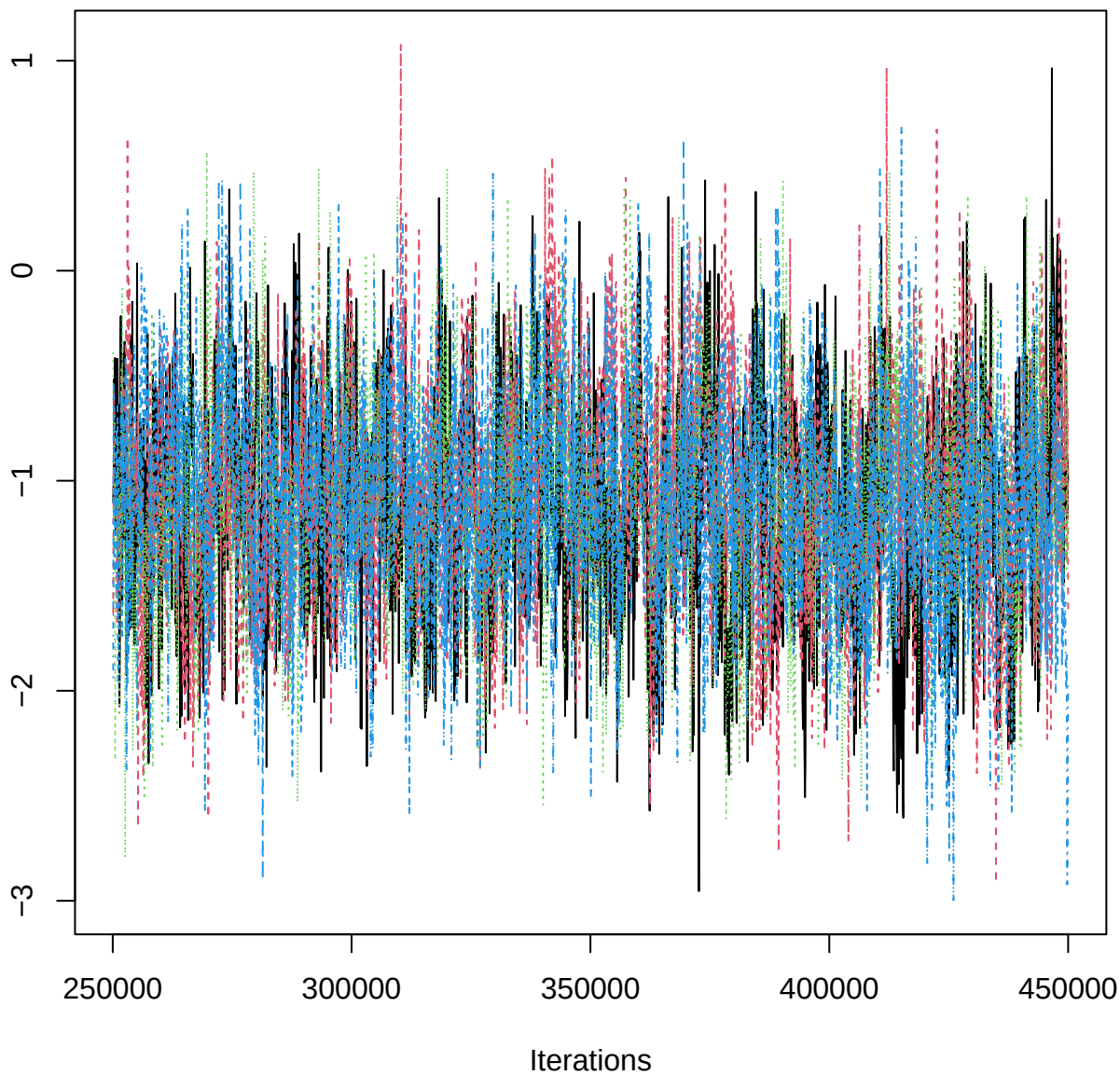
Traceplot – B[pH (C4), EPB_n (S6)]
