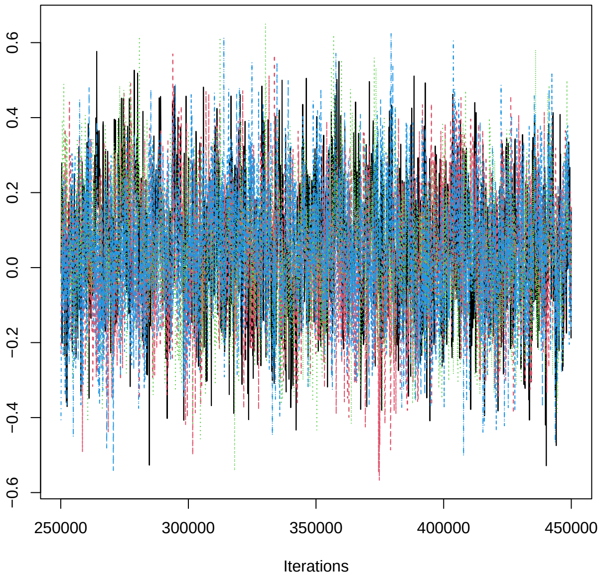
Traceplot – B[aspect_classNW (C13), BOP_n (S5)]
