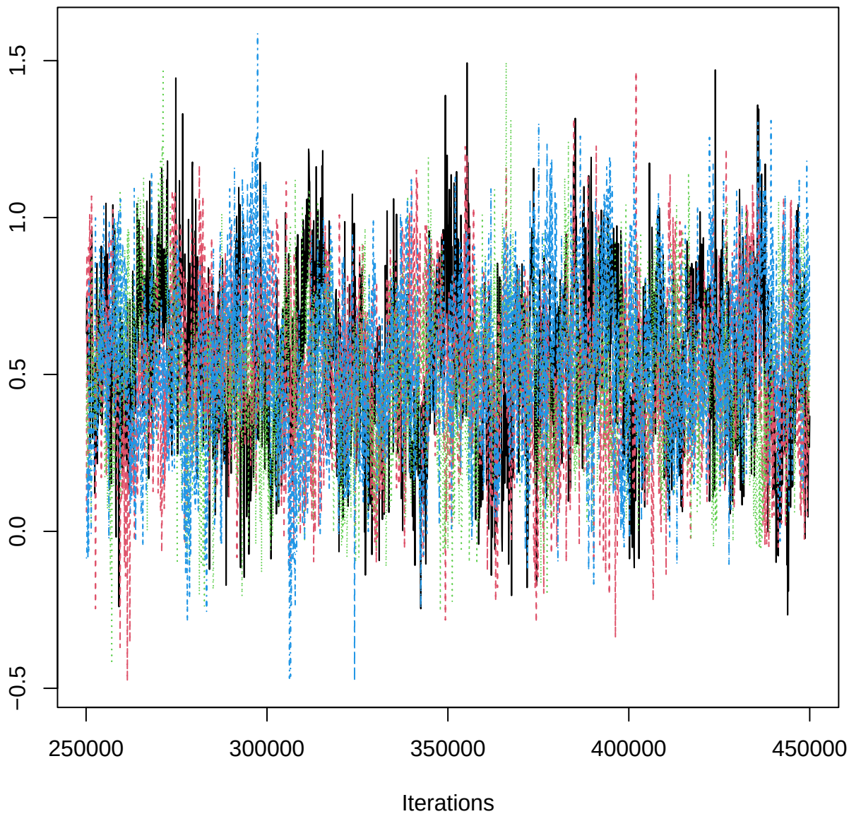
Traceplot – B[aspect_classNE (C12), BOJ_n (S4)]
