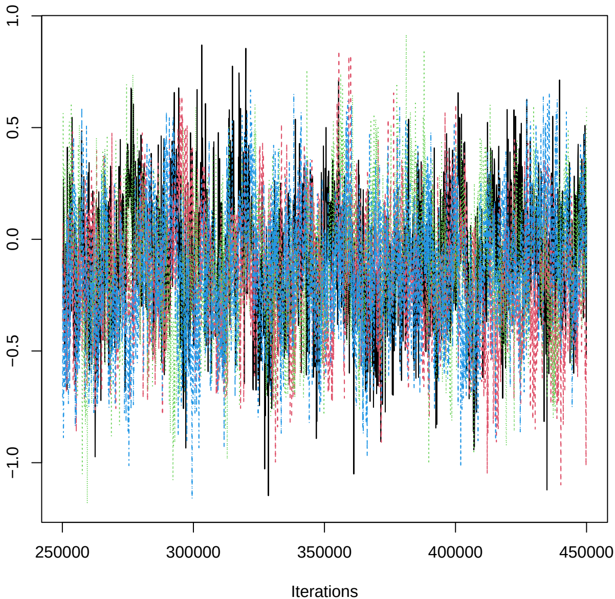
Traceplot – B[aspect_classNW (C13), PET_n (S12)]
