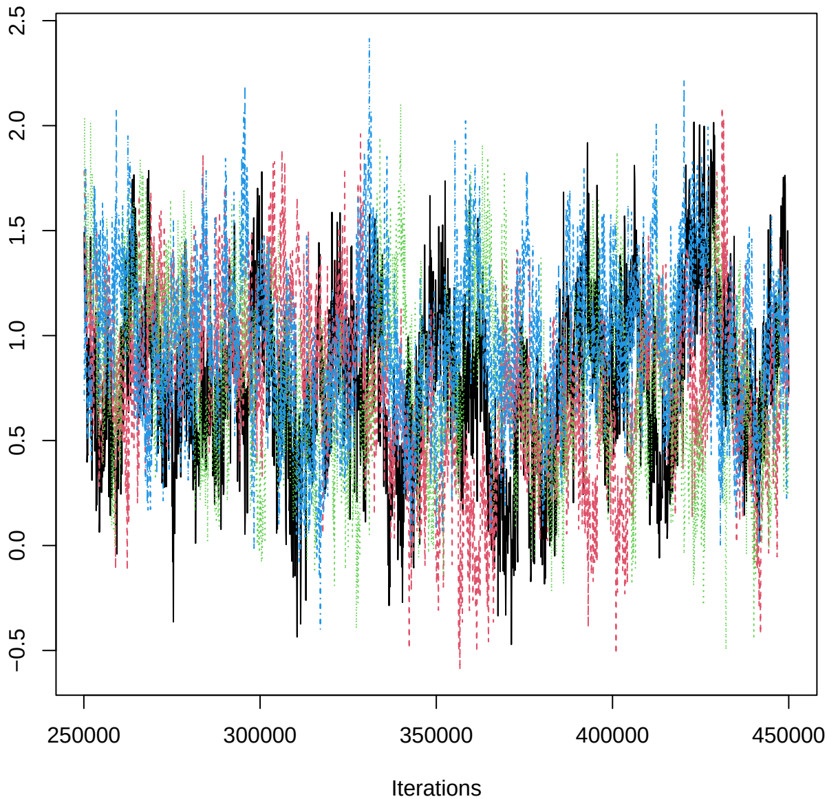
Traceplot – B[aspect_classSW (C16), PIB_n (S13)]
