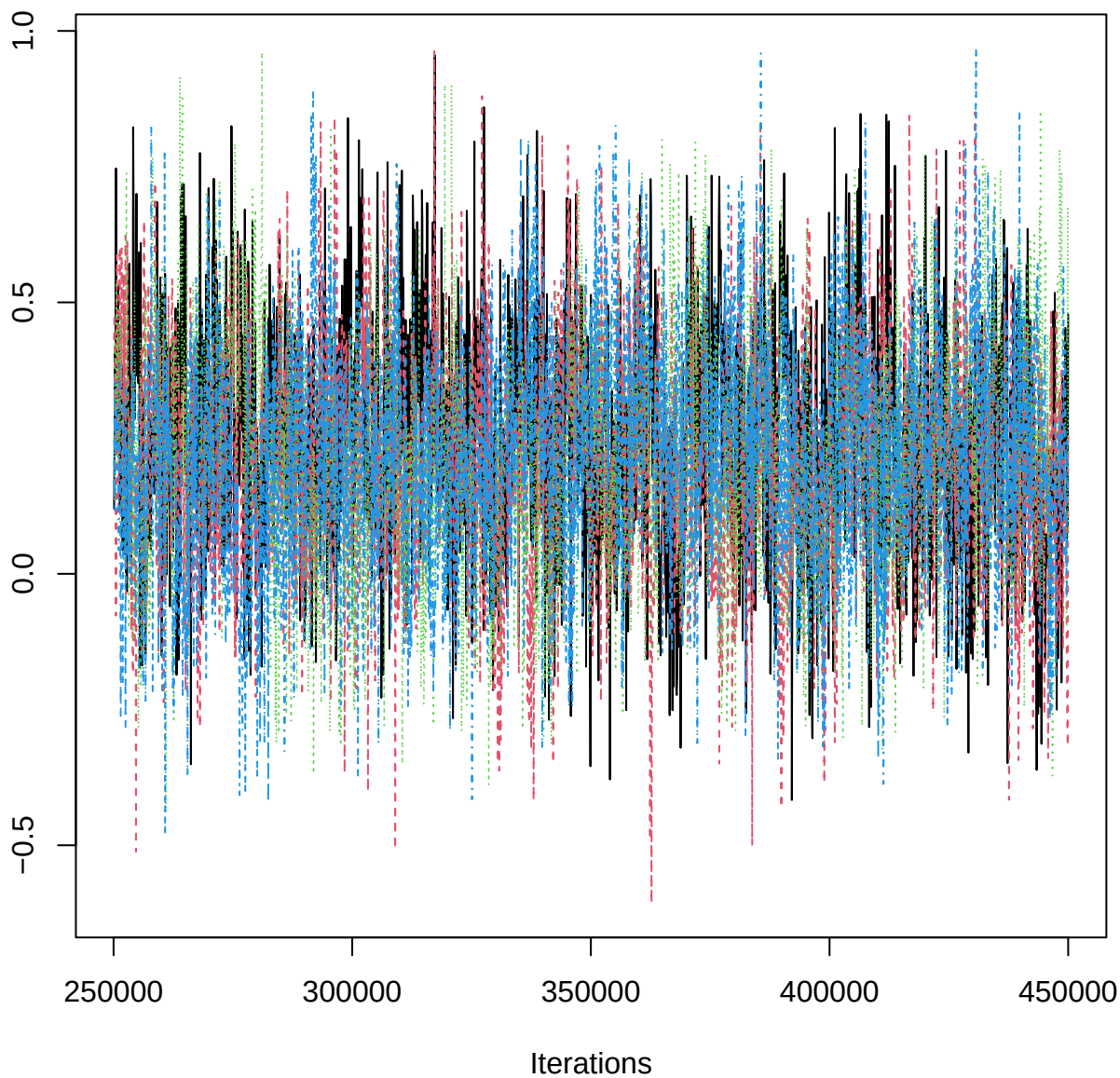
Traceplot – B[aspect_classNE (C12), EPB_n (S6)]
