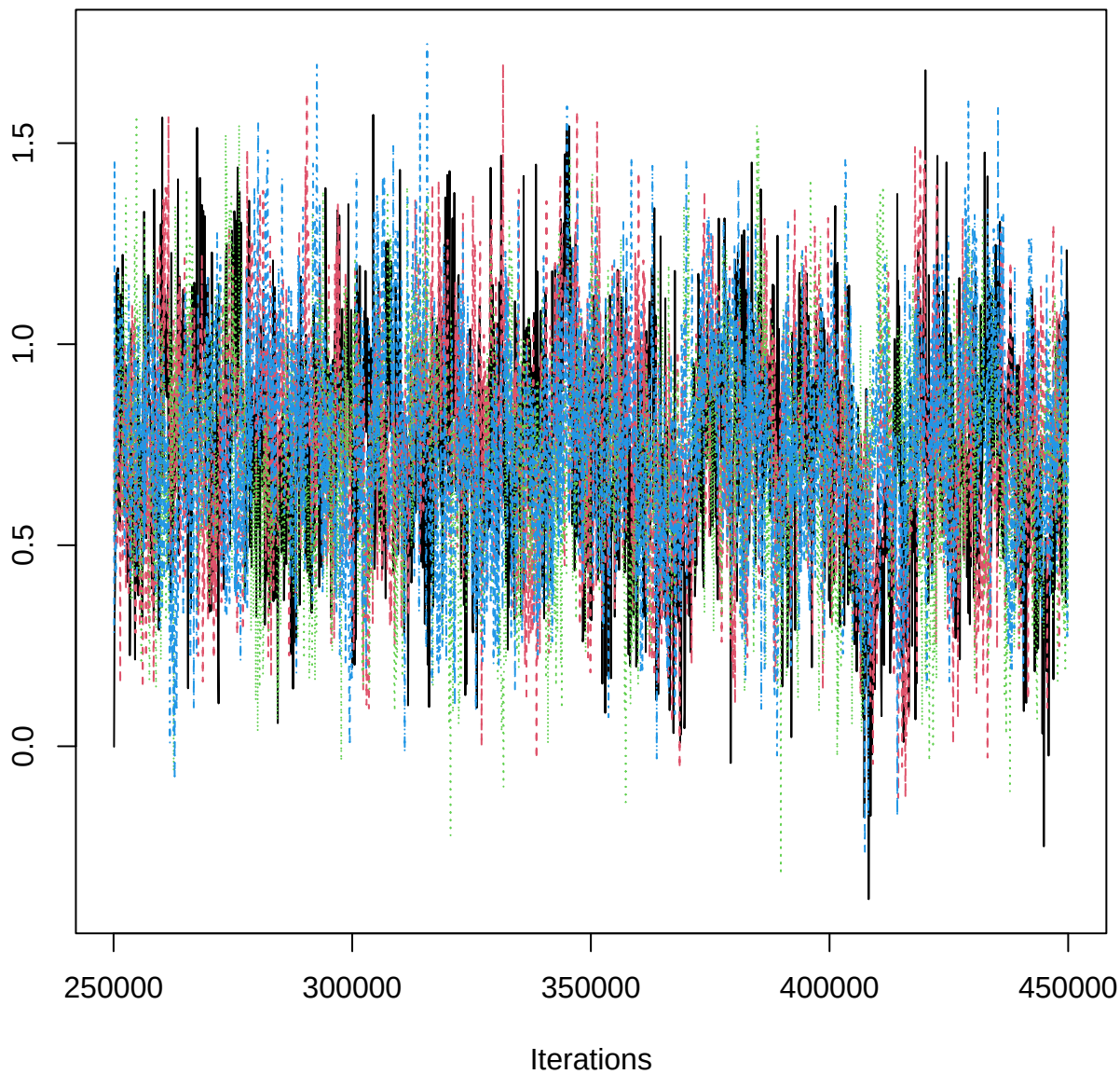
Traceplot – B[aspect_classSE (C15), PET_n (S12)]
