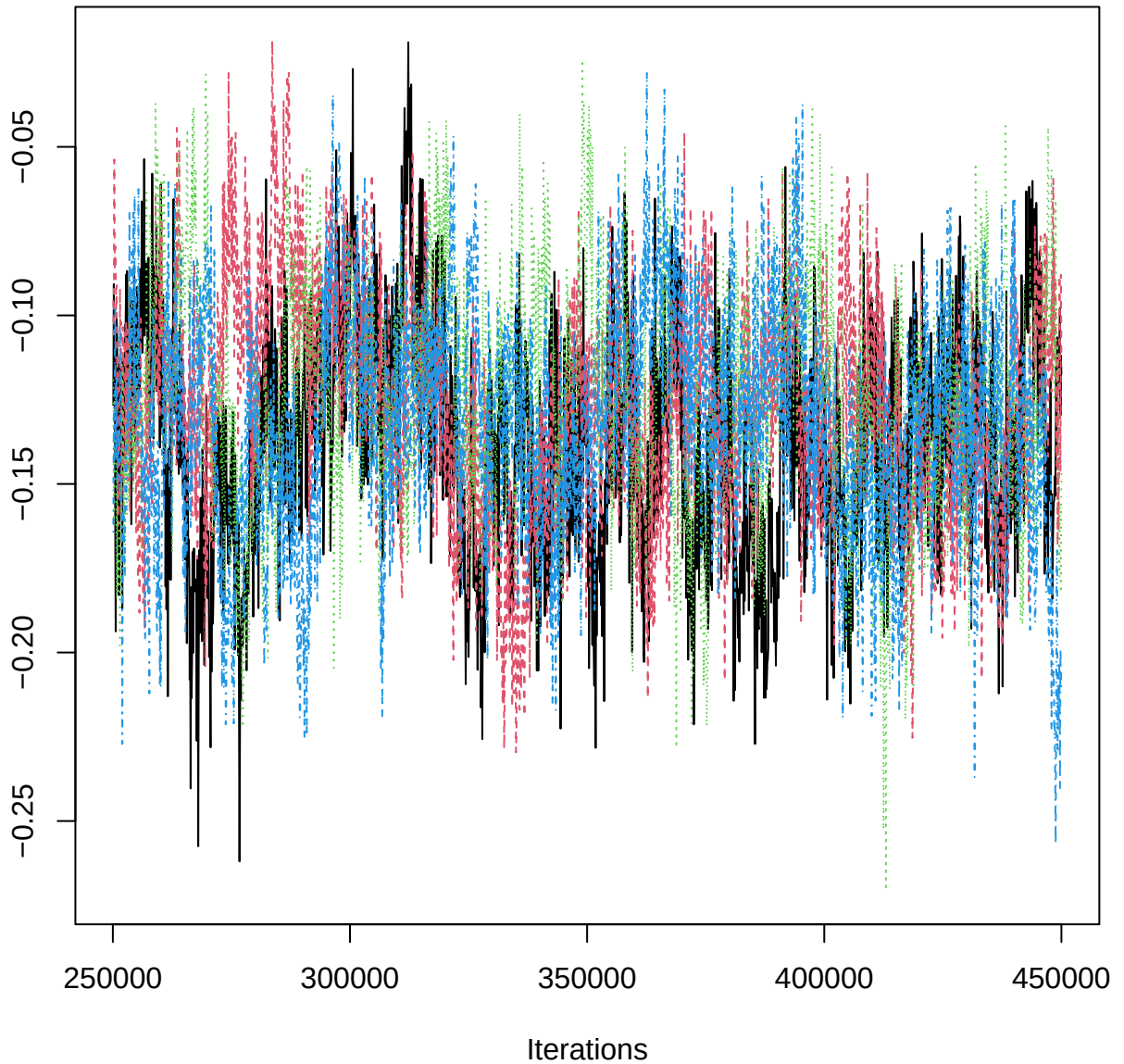
Traceplot – B[twi (C8), BOJ_n (S4)]
