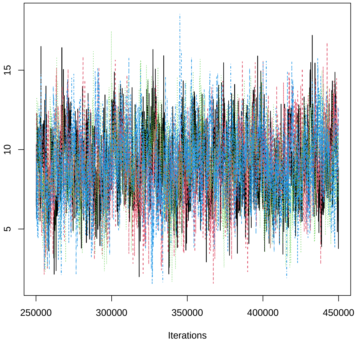
Traceplot – B[(Intercept) (C1), ERR_n (S1)]
