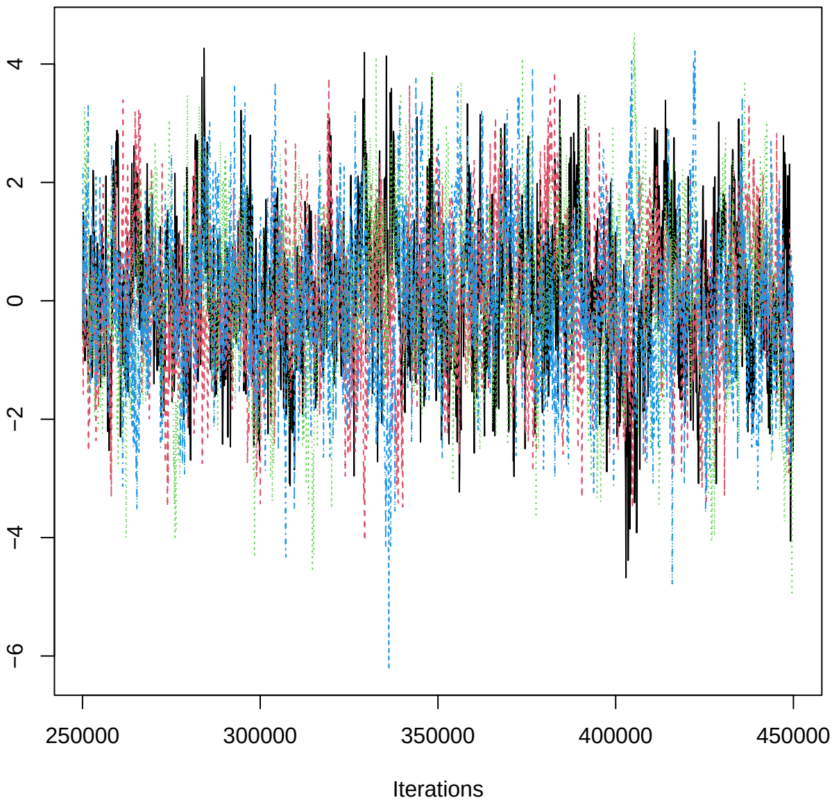
Traceplot – B[aspect_classFlat (C10), EPB_n (S6)]
