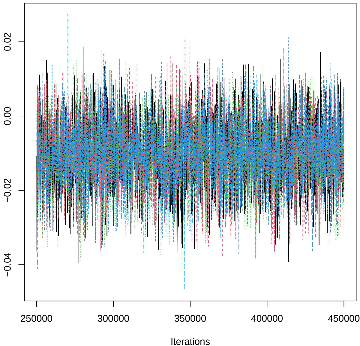
Traceplot – B[slope (C9), SAB_n (S8)]
