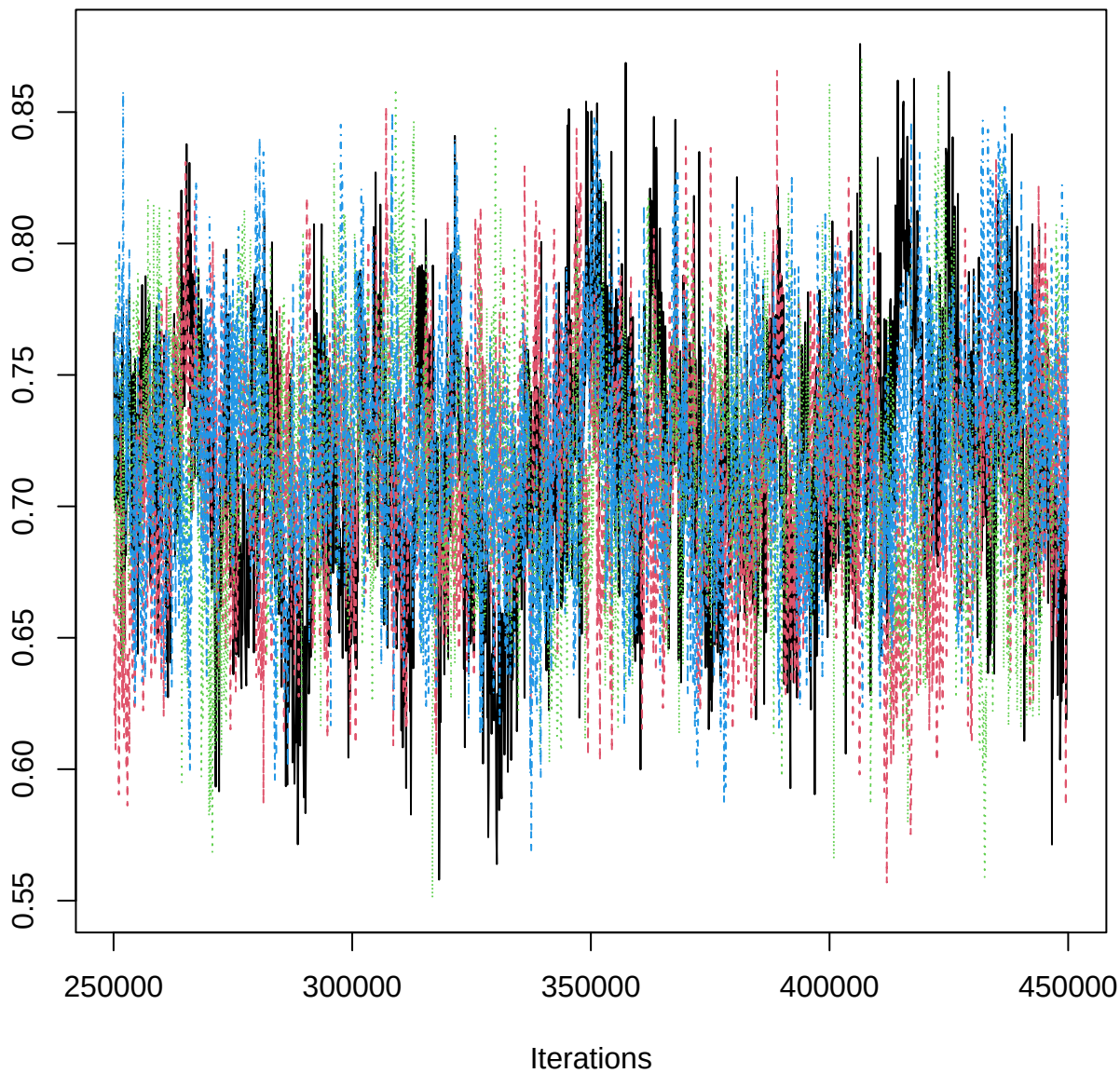
Traceplot – B[MAT (C3), EPB_n (S6)]
