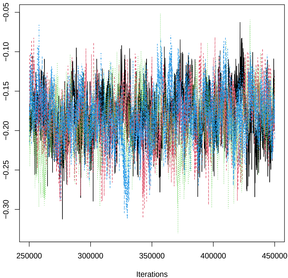
Traceplot – B[twi (C8), PET_n (S12)]
