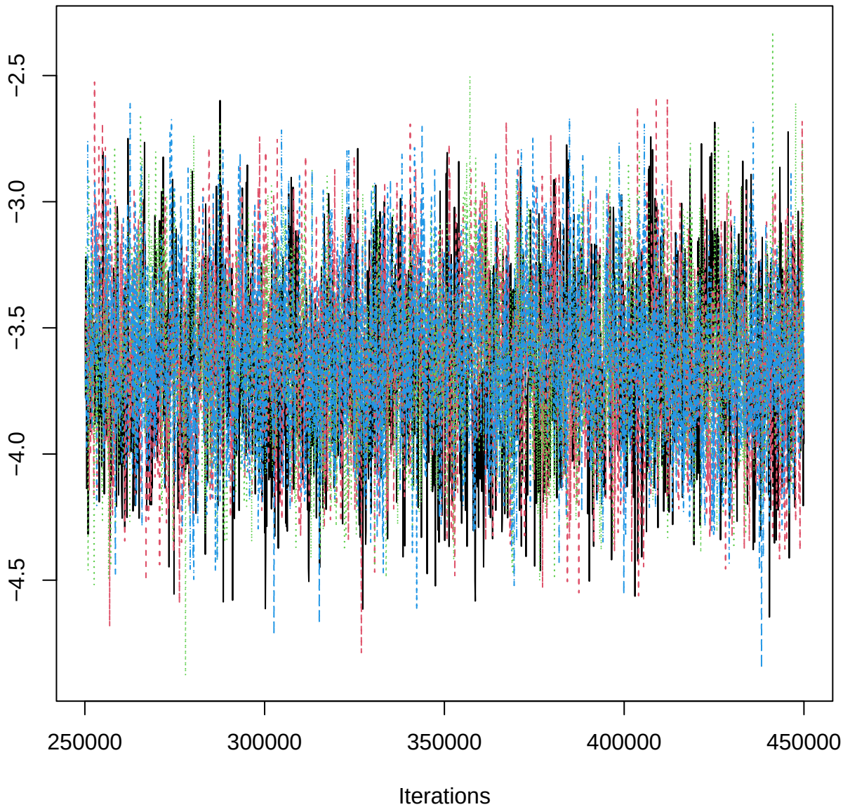
Traceplot – B[pH (C4), SAB_n (S8)]
