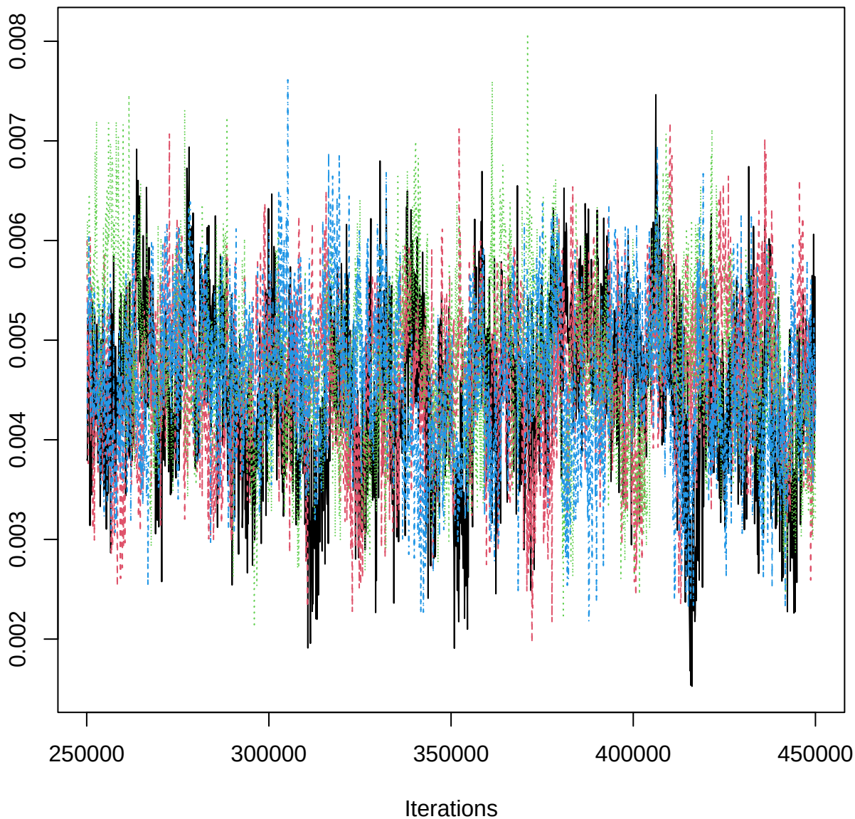
Traceplot – B[MAP (C2), BOJ_n (S4)]
