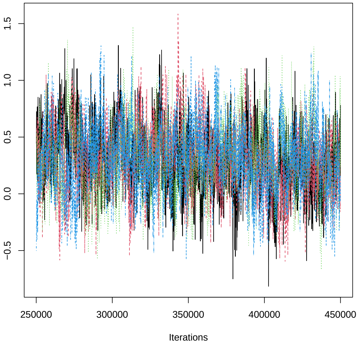
Traceplot – B[aspect_classW (C17), PET_n (S12)]
