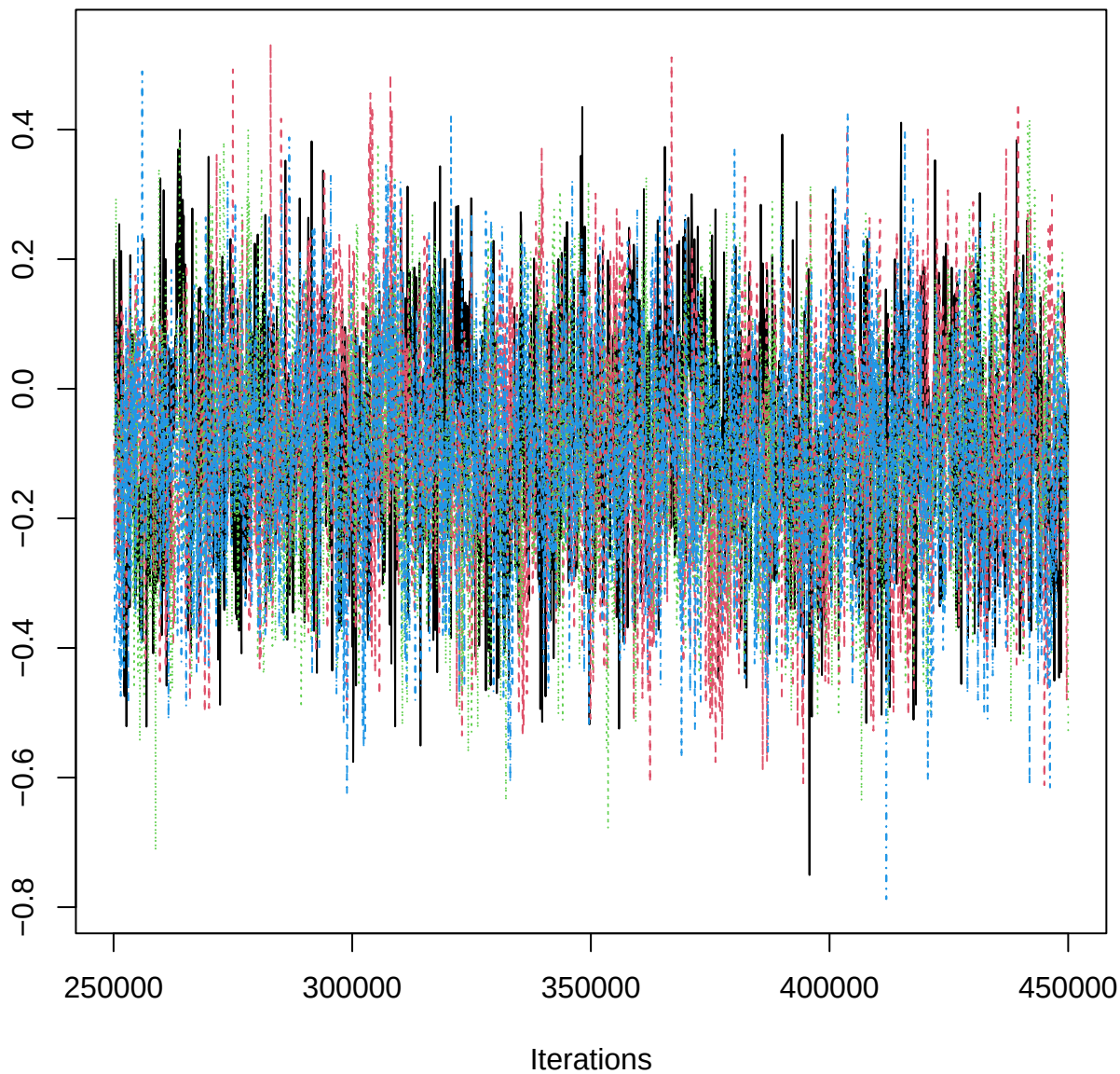
Traceplot – B[aspect_classN (C11), BOP_n (S5)]
