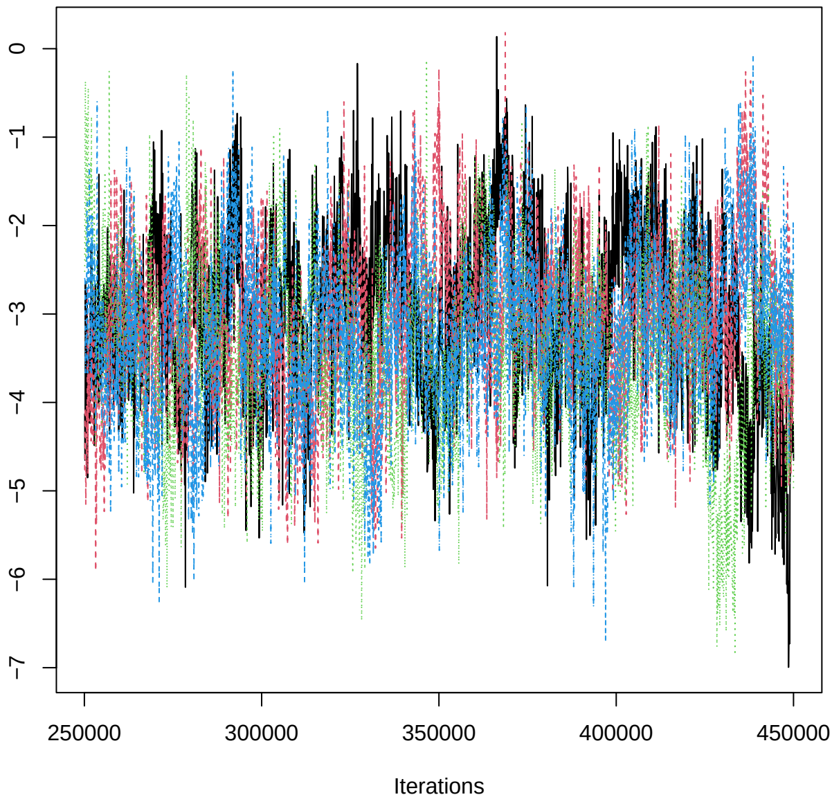
Traceplot – B[pH (C4), THO_n (S10)]
