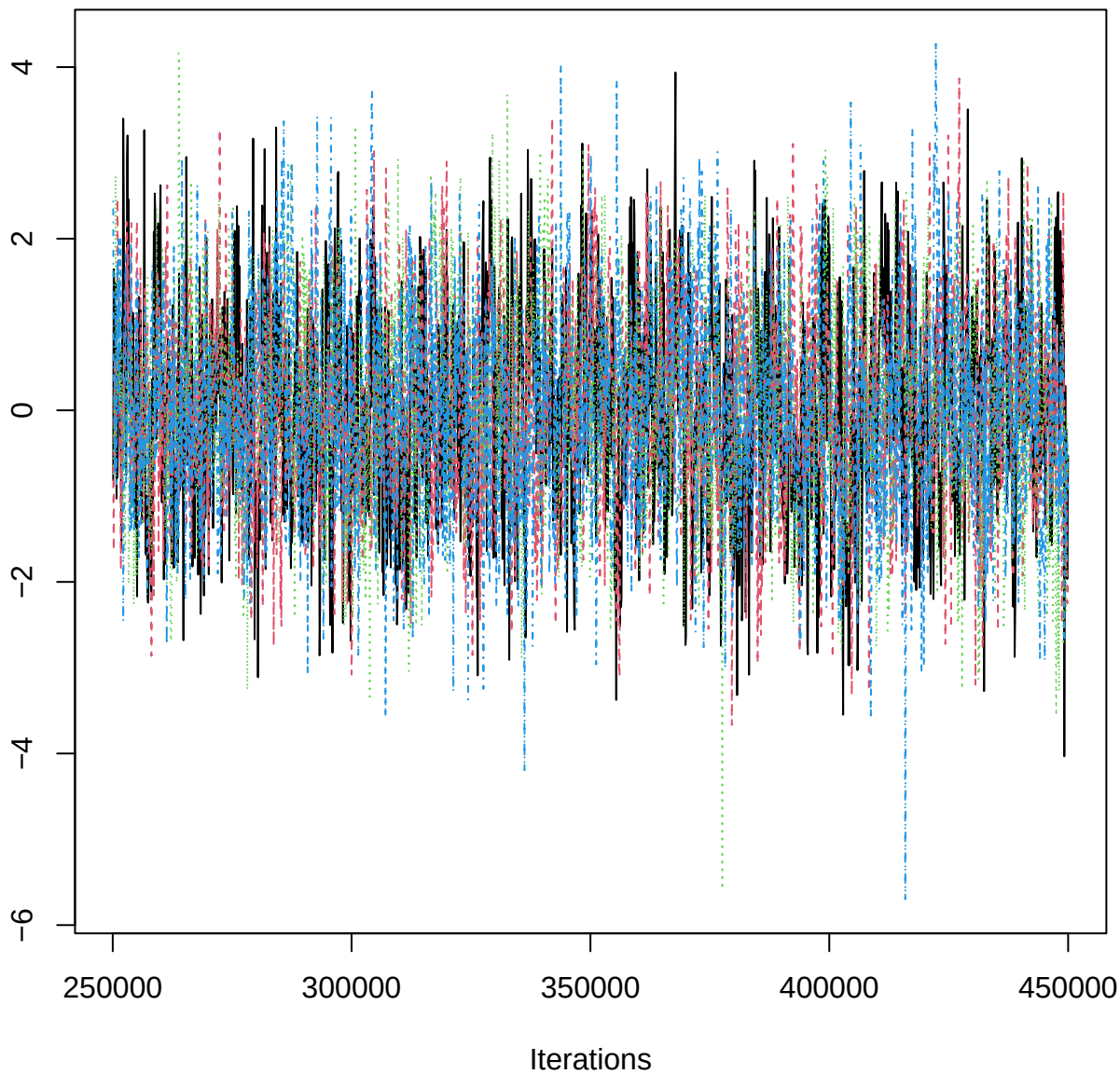
Traceplot – B[aspect_classFlat (C10), BOP_n (S5)]
