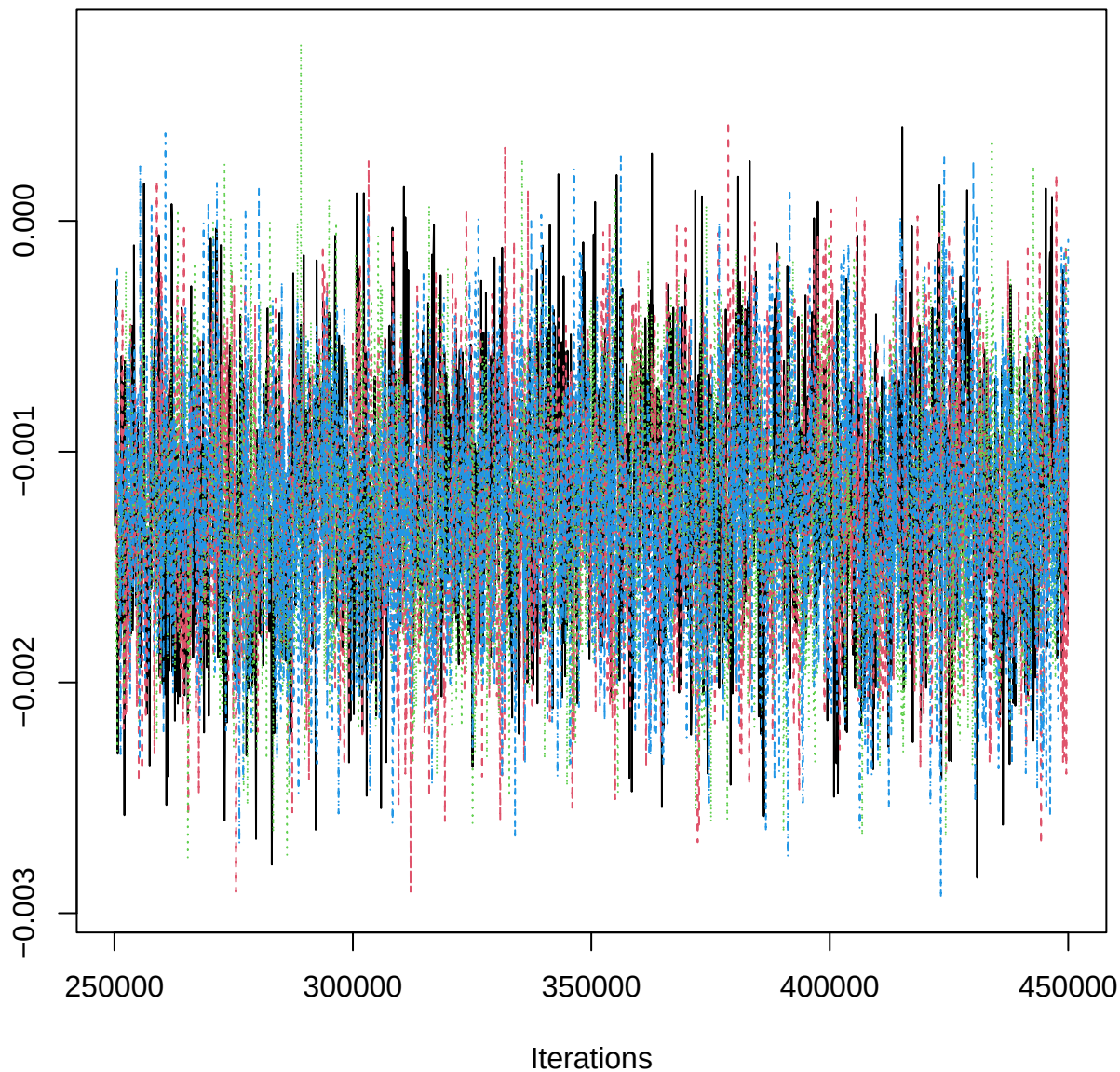
Traceplot – B[MAP (C2), BOP_n (S5)]
