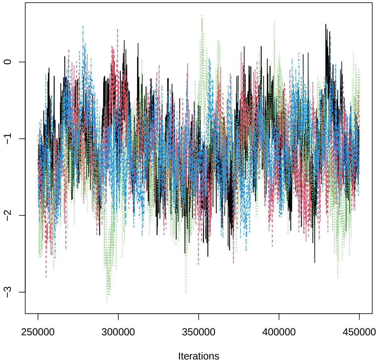
Traceplot – B[aspect_classNW (C13), PIG_n (S14)]
