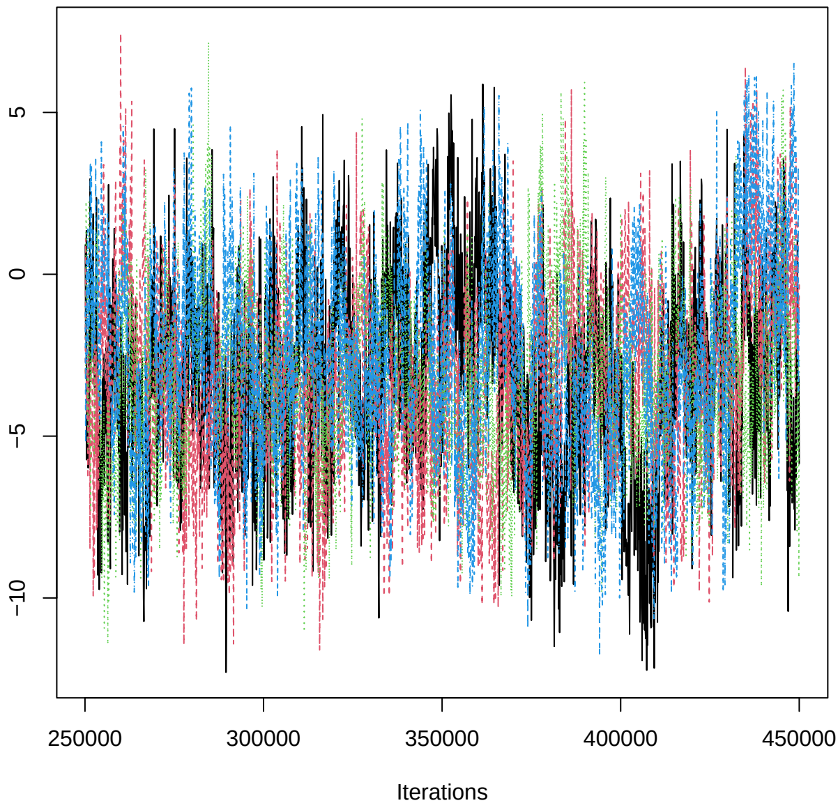
Traceplot – B[(Intercept) (C1), ERS_n (S2)]
