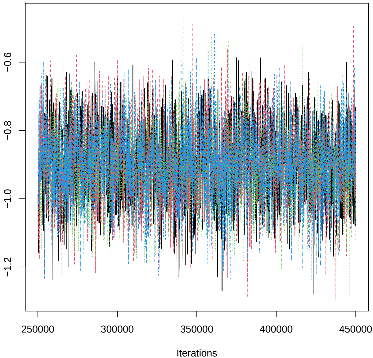
Traceplot – B[rtp (C7), SAB_n (S8)]
