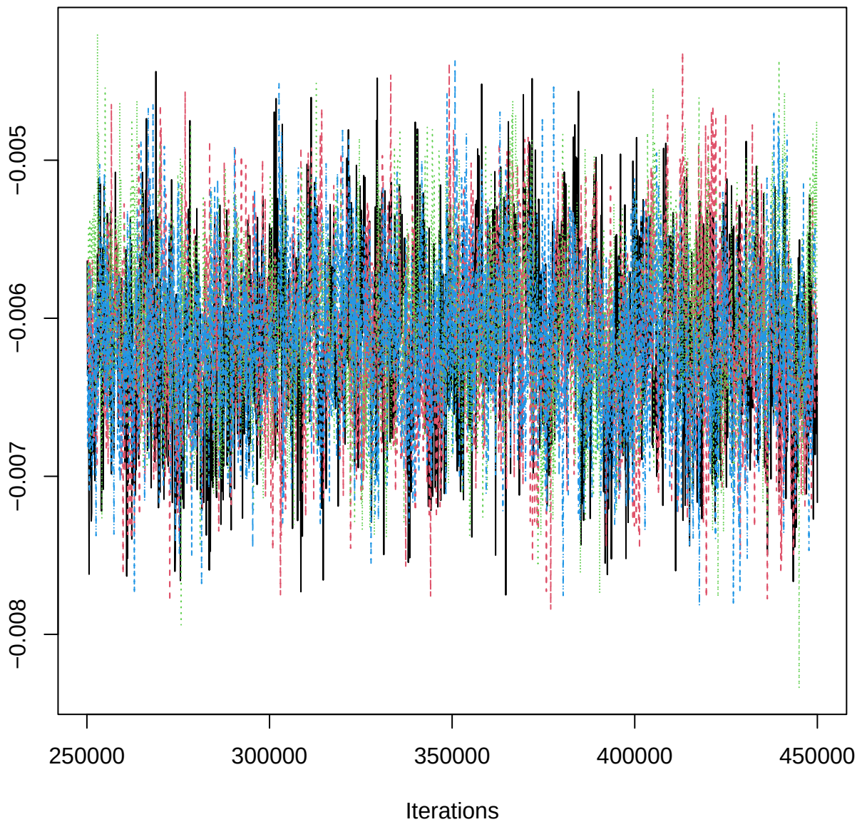
Traceplot – B[MAP (C2), EPN_n (S9)]
