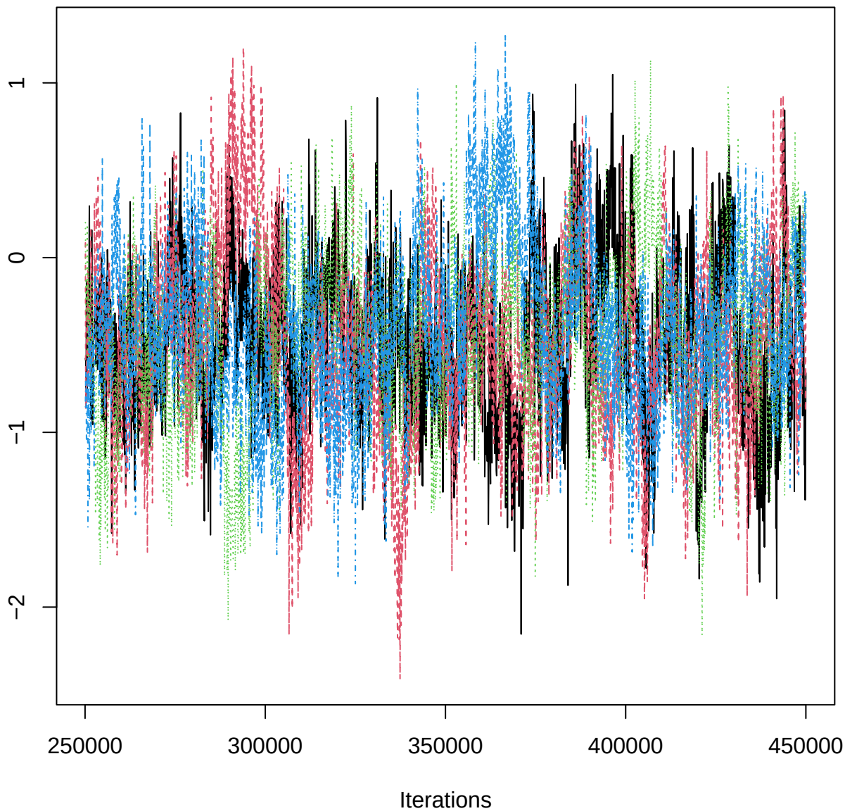
Traceplot – B[aspect_classNE (C12), PIG_n (S14)]
