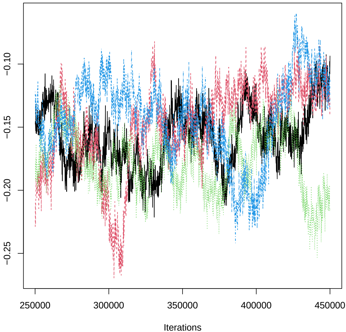
Traceplot – B[Clay (C5), EPR_n (S7)]
