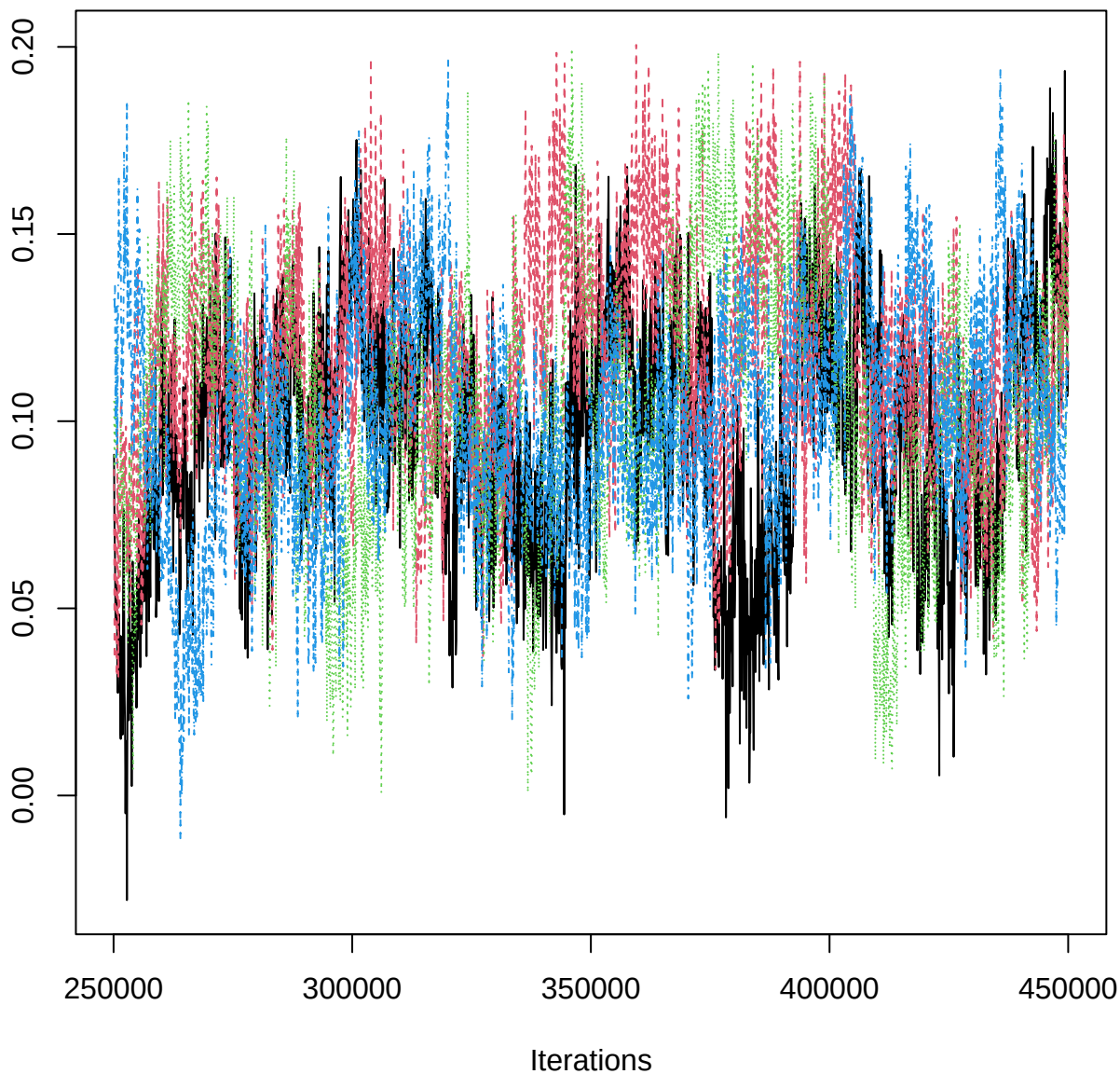
Traceplot – B[slope (C9), HEG_n (S3)]
