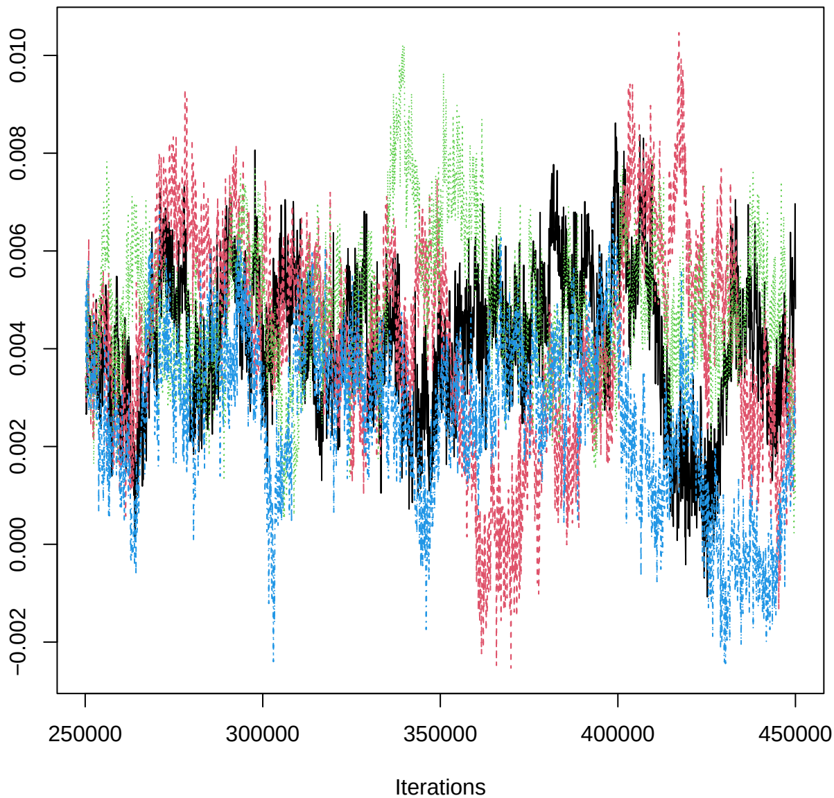
Traceplot – B[MAP (C2), HEG_n (S3)]
