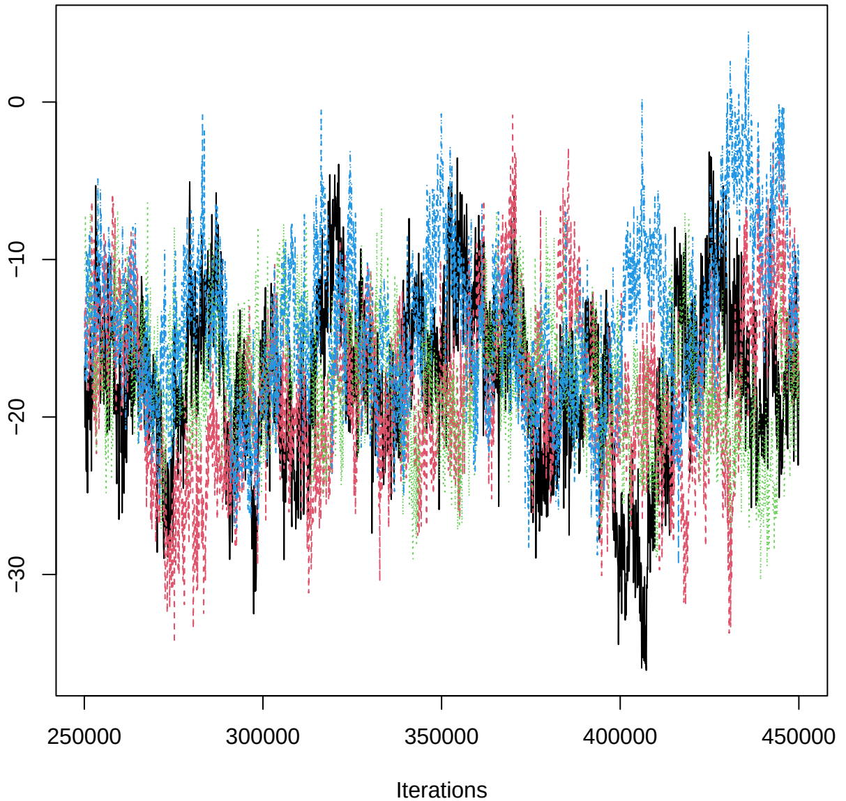
Traceplot – B[(Intercept) (C1), HEG_n (S3)]
