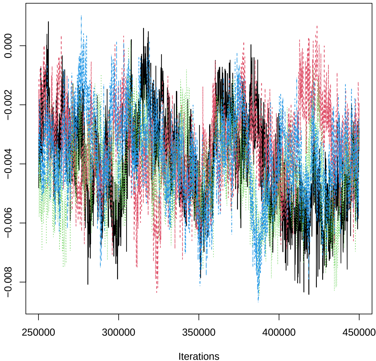
Traceplot – B[MAP (C2), THO_n (S10)]
