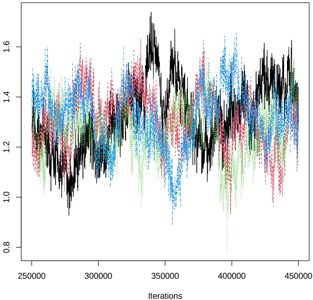
Traceplot – B[MAT (C3), PRP_n (S11)]
