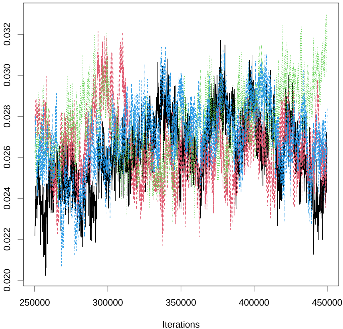
Traceplot – B[MAP (C2), EPR_n (S7)]
