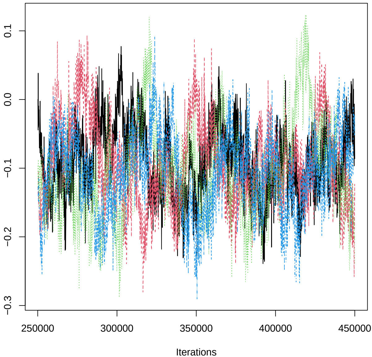
Traceplot – B[twi (C8), EPR_n (S7)]
