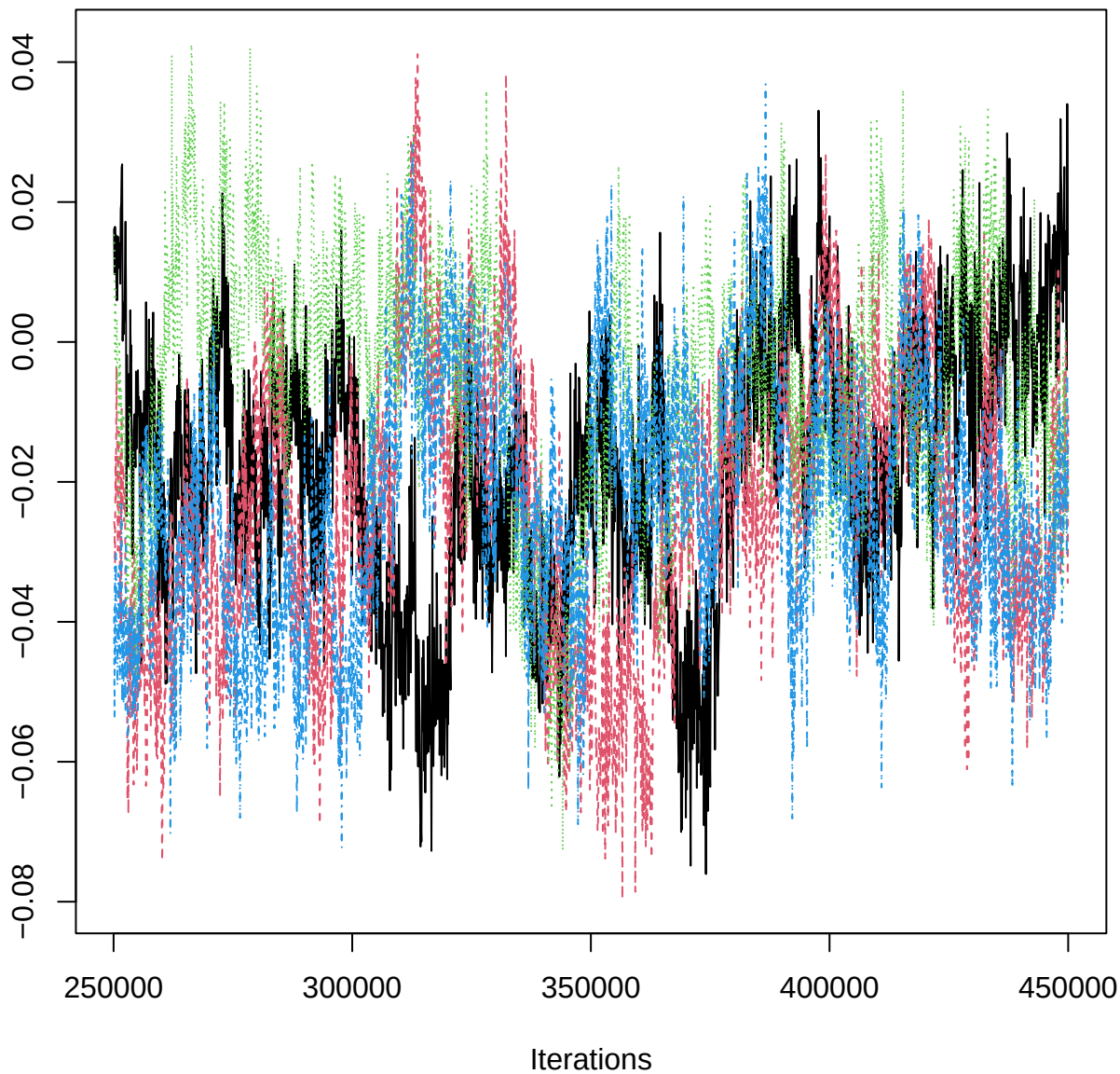
Traceplot – B[Clay (C5), THO_n (S10)]
