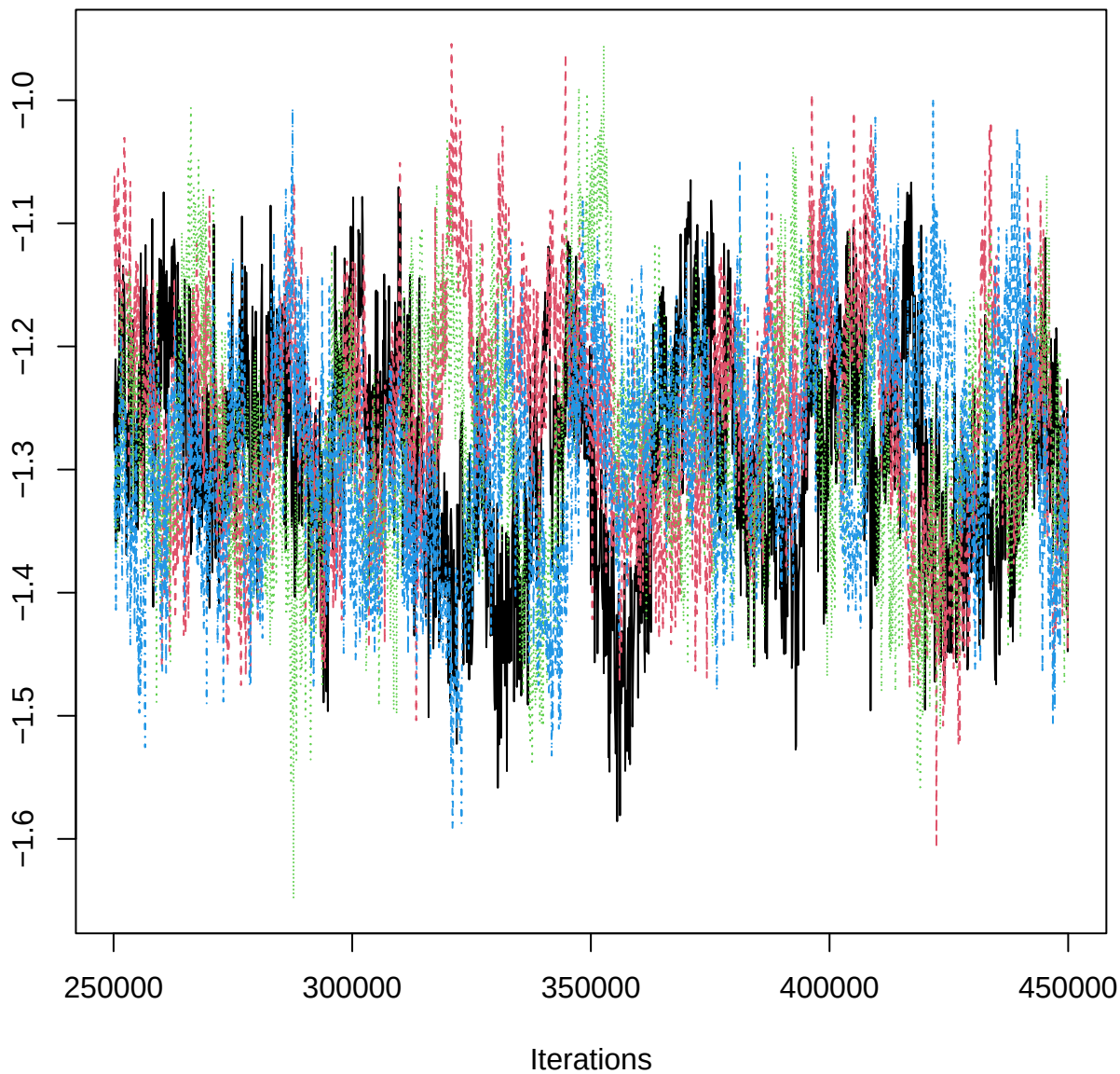
Traceplot – B[OM (C6), PIG_n (S14)]
