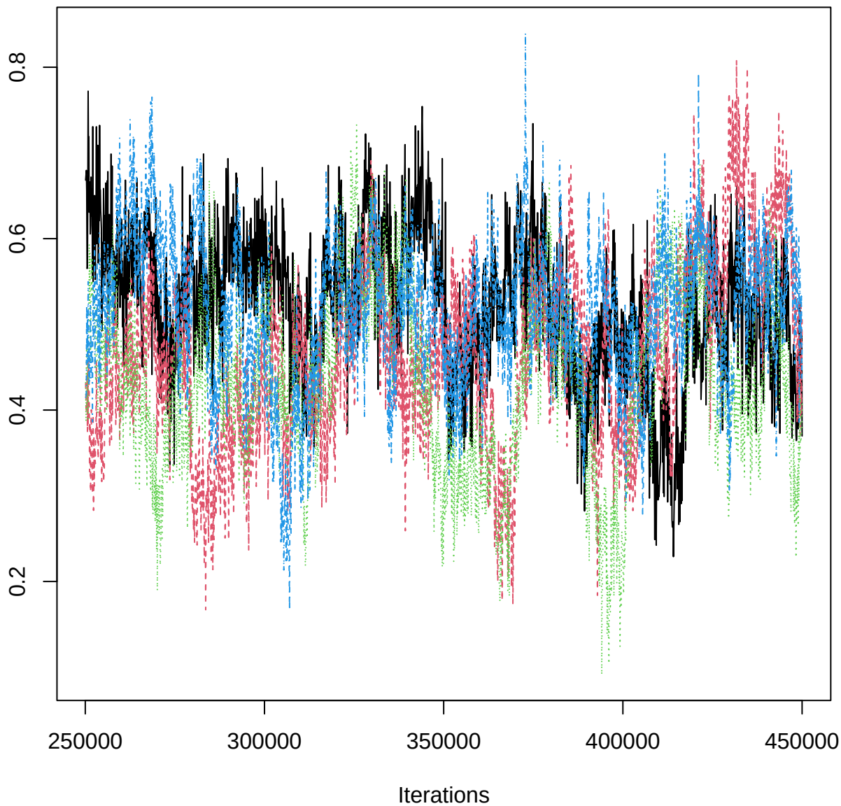
Traceplot – B[OM (C6), PIB_n (S13)]
