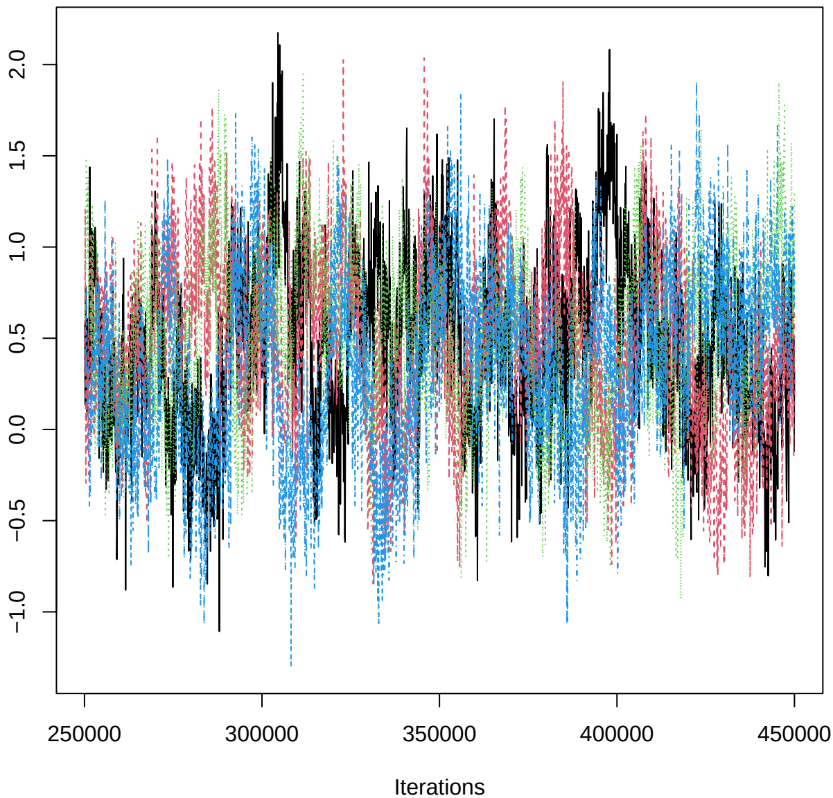
Traceplot – B[aspect_classNW (C13), EPR_n (S7)]
