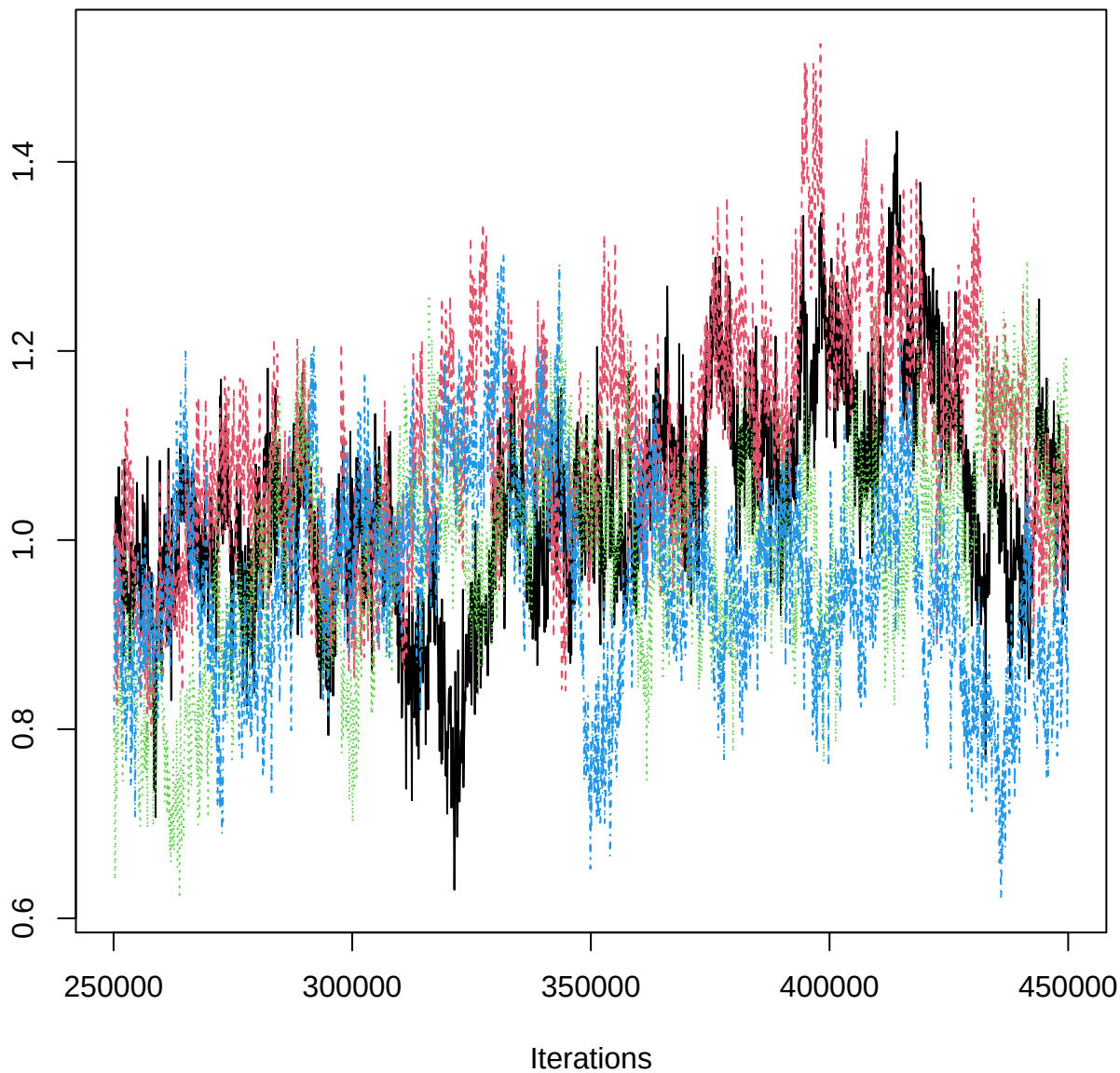
Traceplot – B[OM (C6), HEG_n (S3)]
