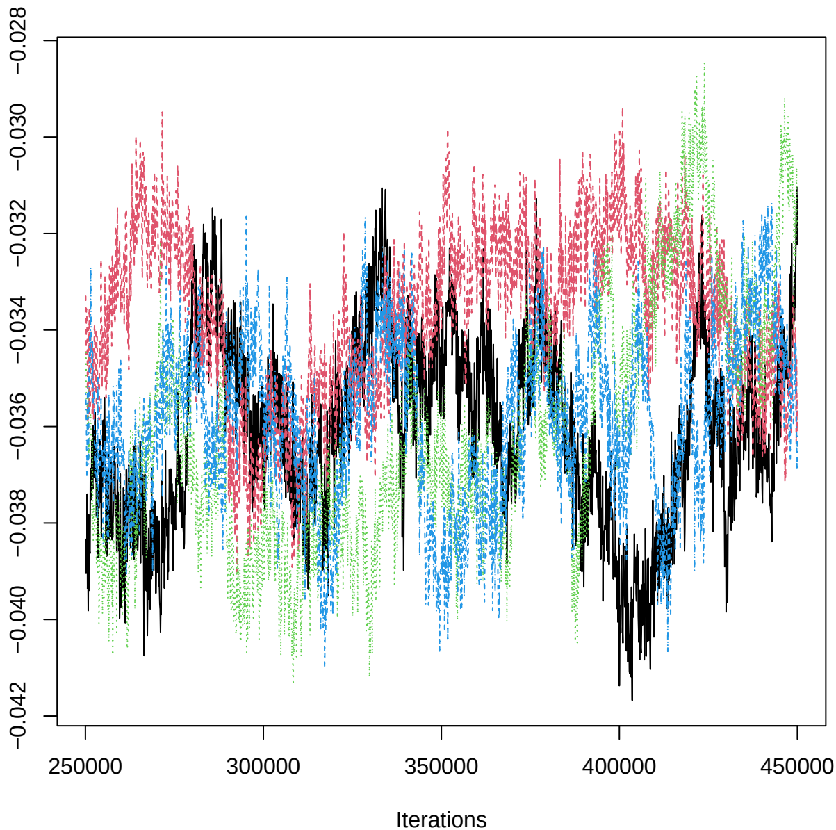
Traceplot – B[MAP (C2), PIB_n (S13)]
