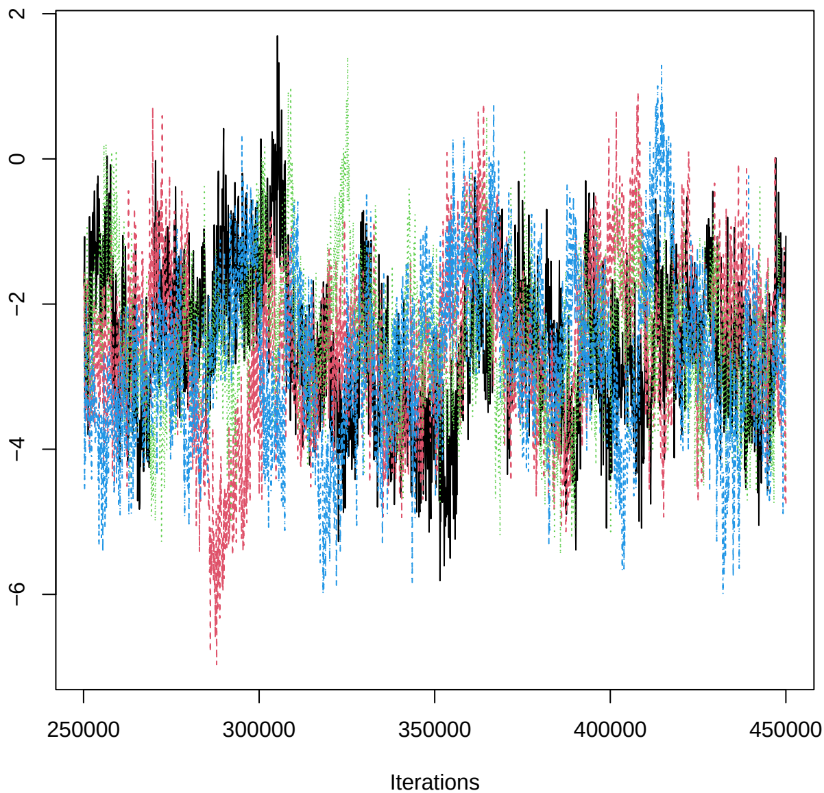
Traceplot – B[pH (C4), PRP_n (S11)]
