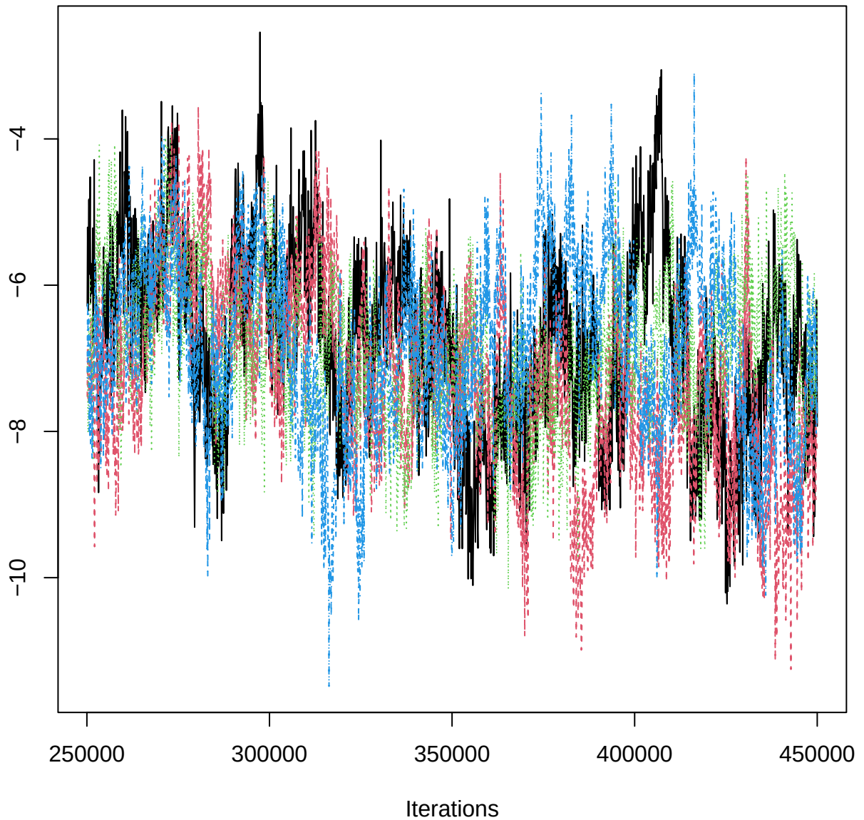
Traceplot – B[pH (C4), HEG_n (S3)]
