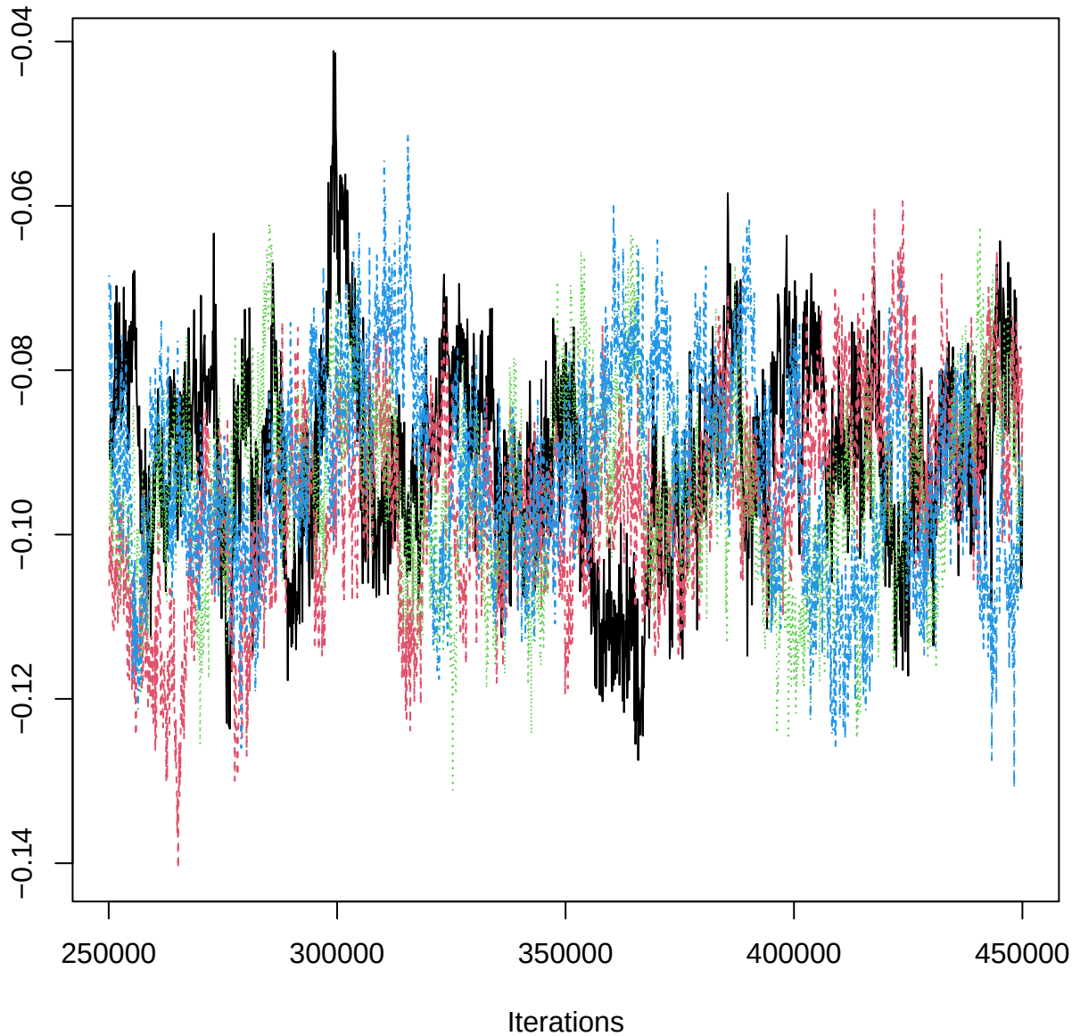
Traceplot – B[Clay (C5), ERR_n (S1)]
