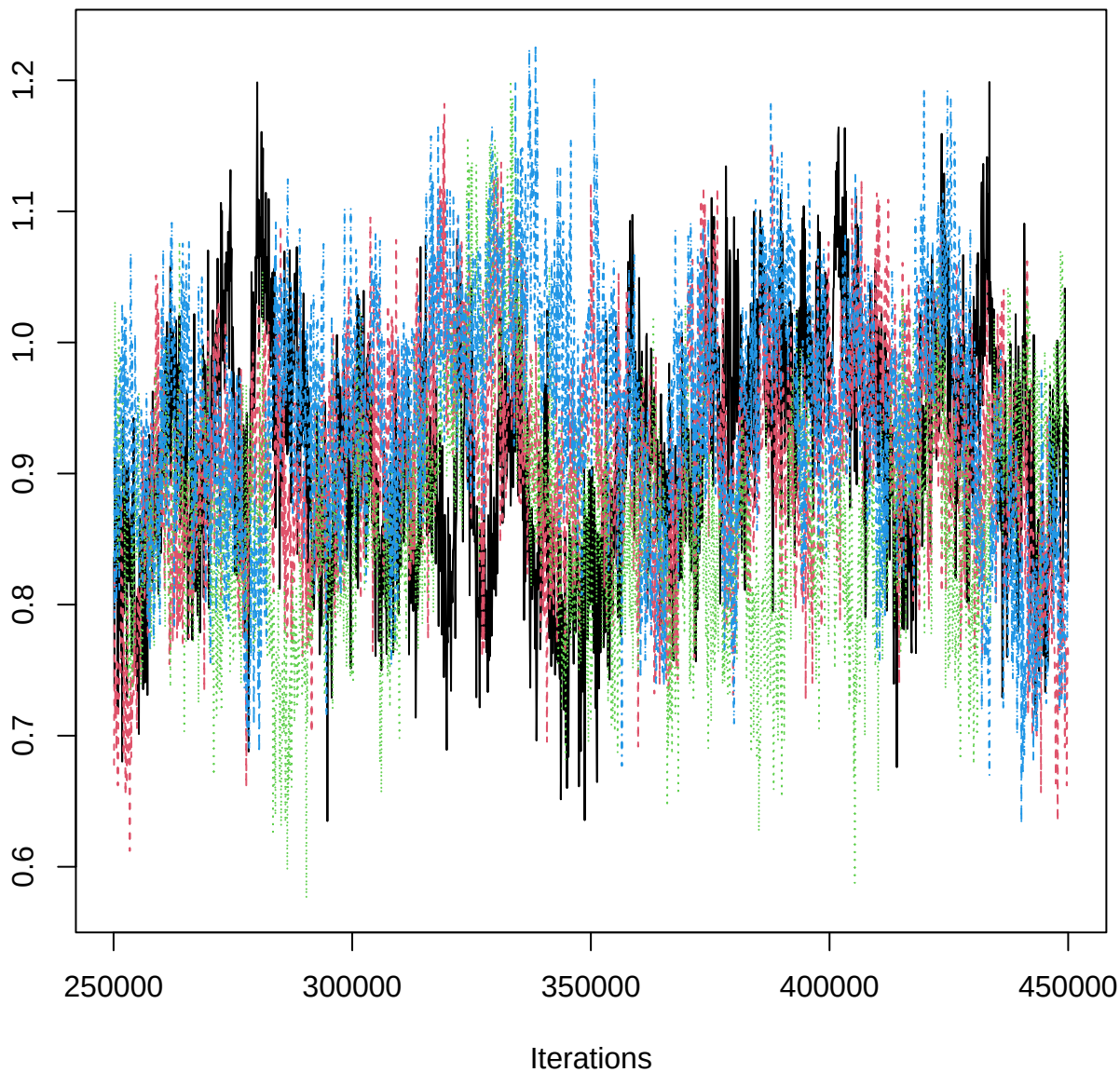
Traceplot – B[OM (C6), THO_n (S10)]
