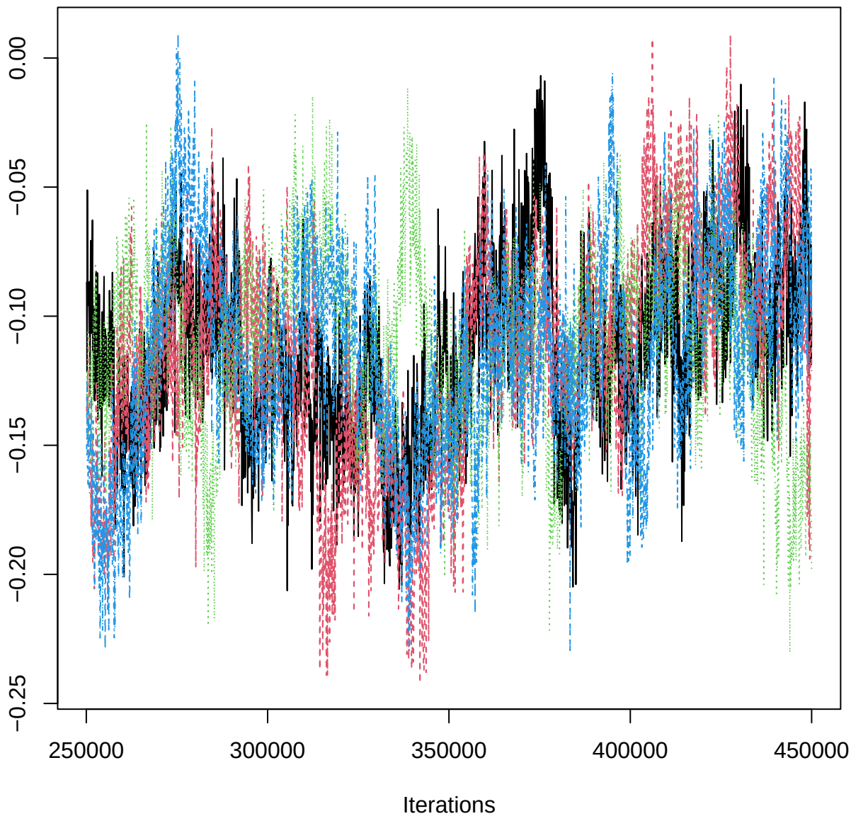
Traceplot – B[slope (C9), EPR_n (S7)]
