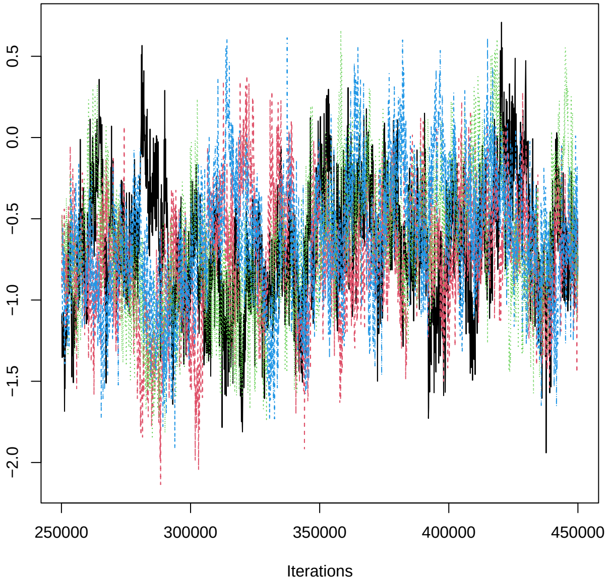
Traceplot – B[rtp (C7), EPR_n (S7)]
