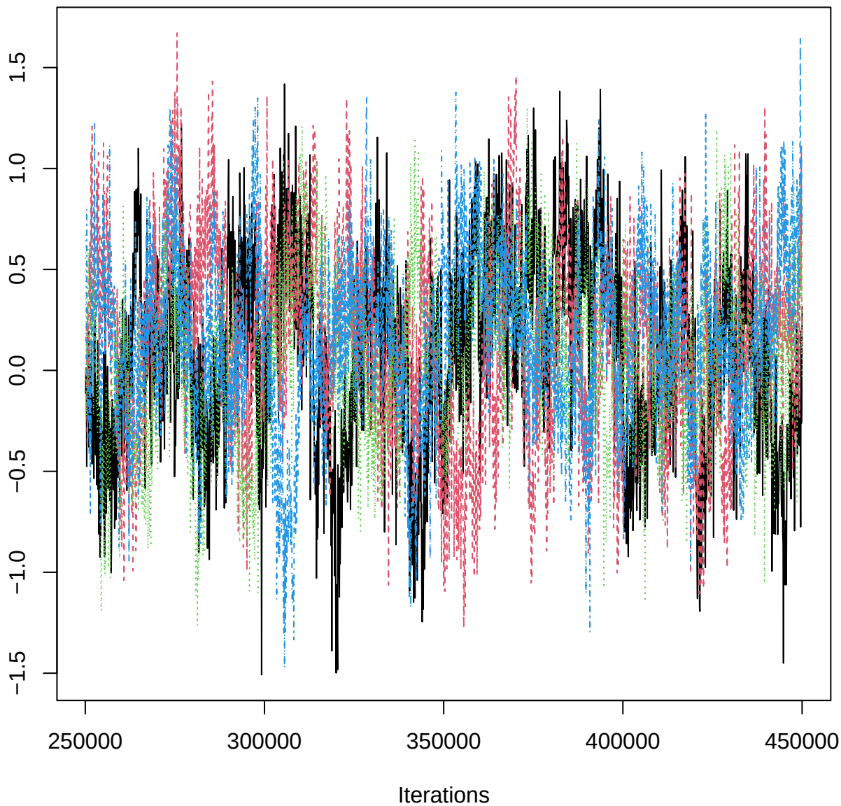
Traceplot – B[aspect_classNW (C13), HEG_n (S3)]
