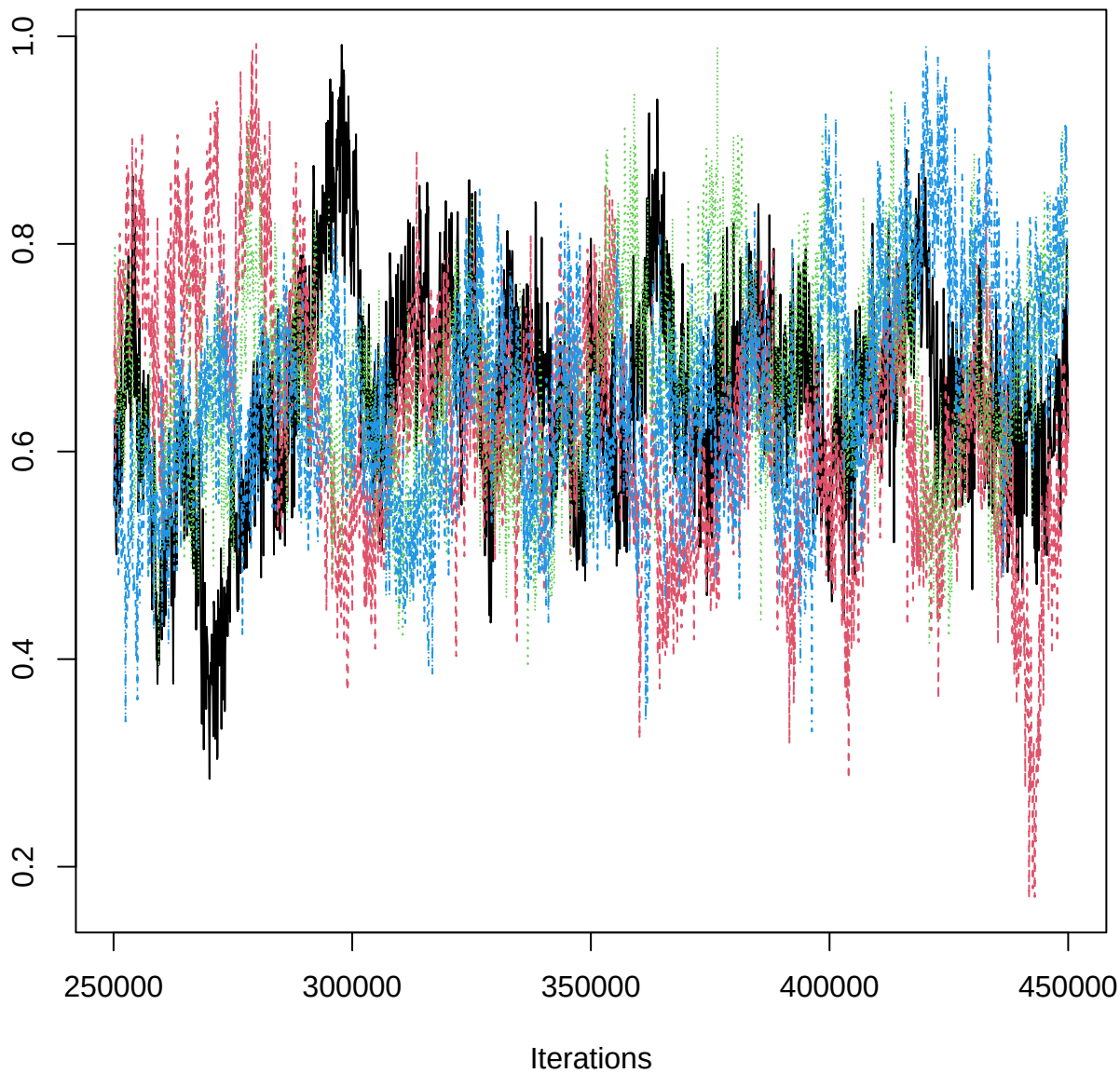
Traceplot – B[OM (C6), EPR_n (S7)]
