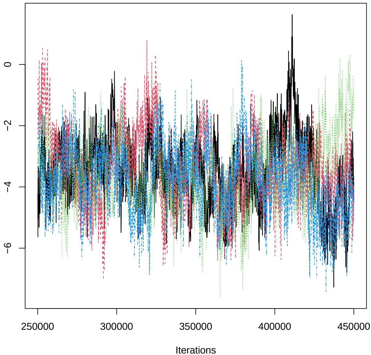
Traceplot – B[pH (C4), EPR_n (S7)]
