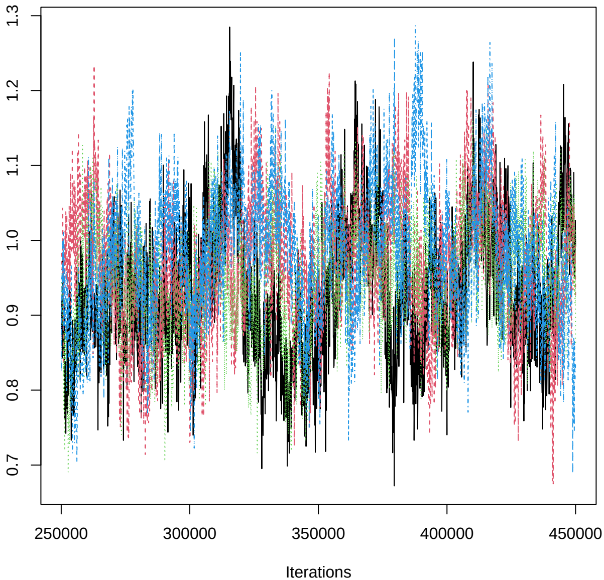
Traceplot – B[OM (C6), PRP_n (S11)]
