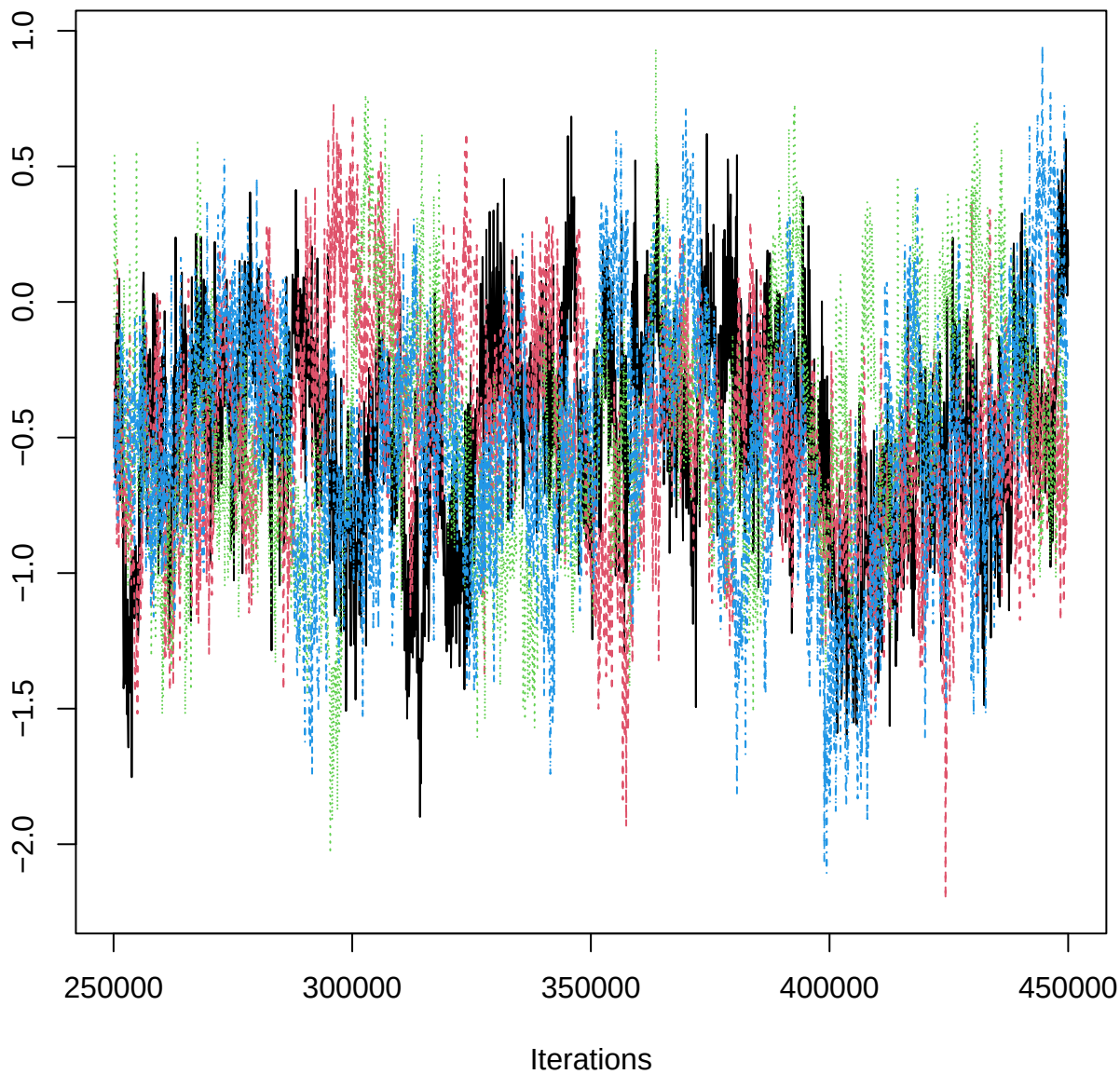
Traceplot – B[aspect_classN (C11), PIB_n (S13)]
