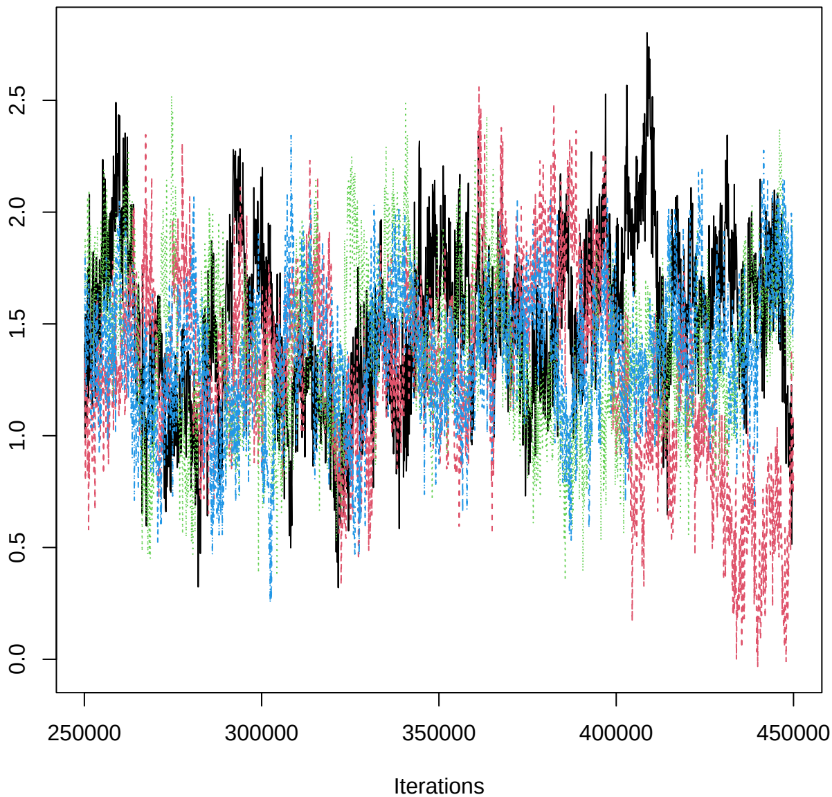
Traceplot – B[rtp (C7), PIB_n (S13)]
