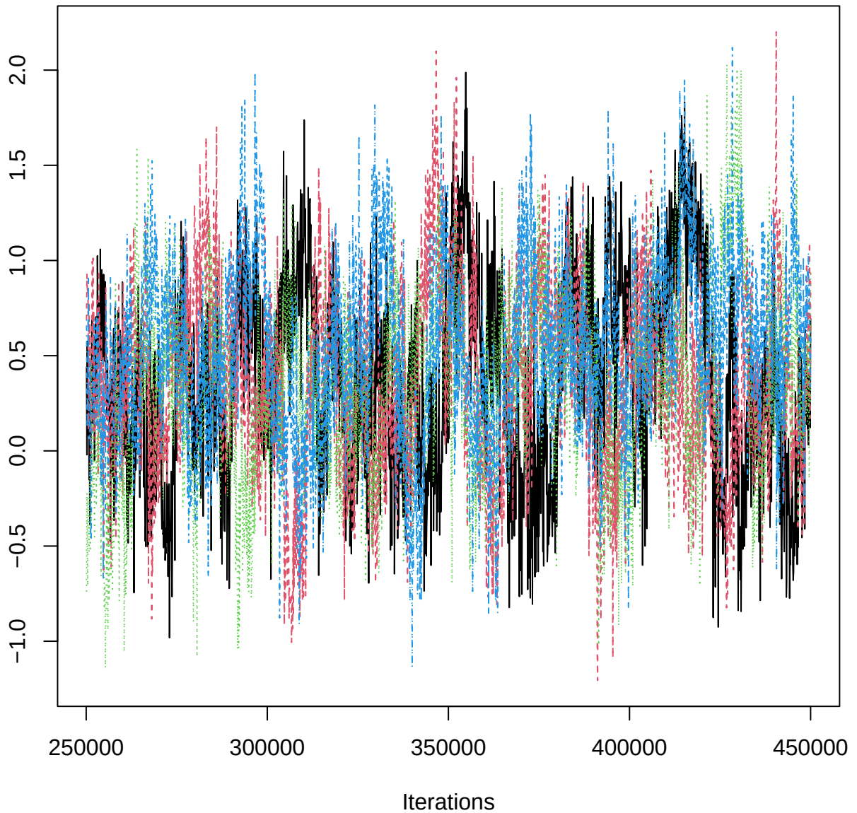
Traceplot – B[aspect_classSW (C16), EPR_n (S7)]
