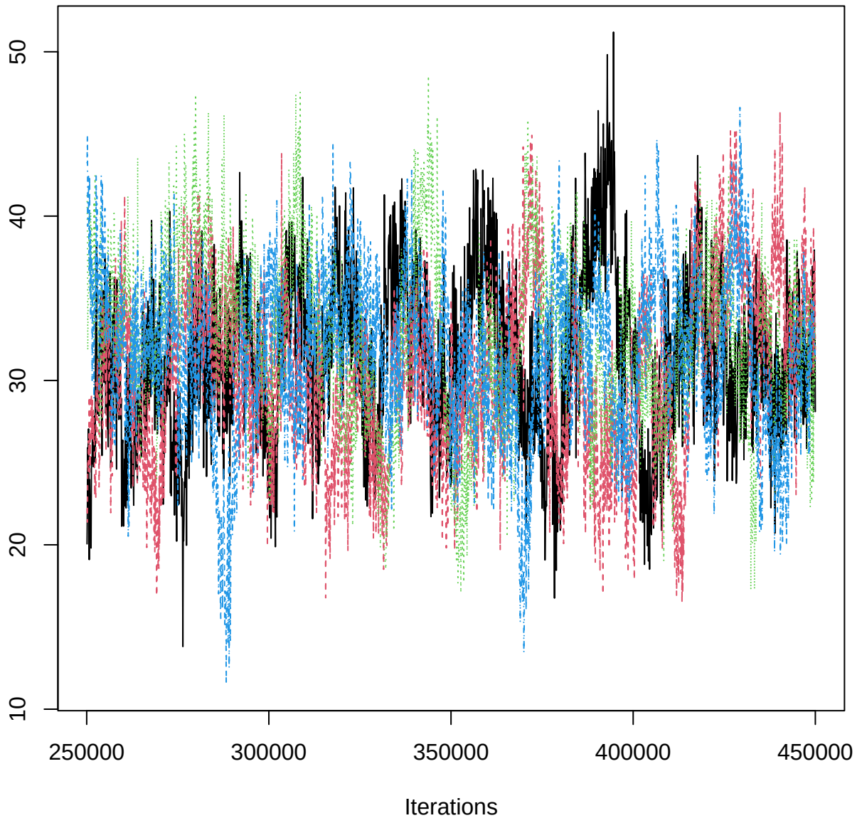
Traceplot – B[(Intercept) (C1), PIG_n (S14)]
