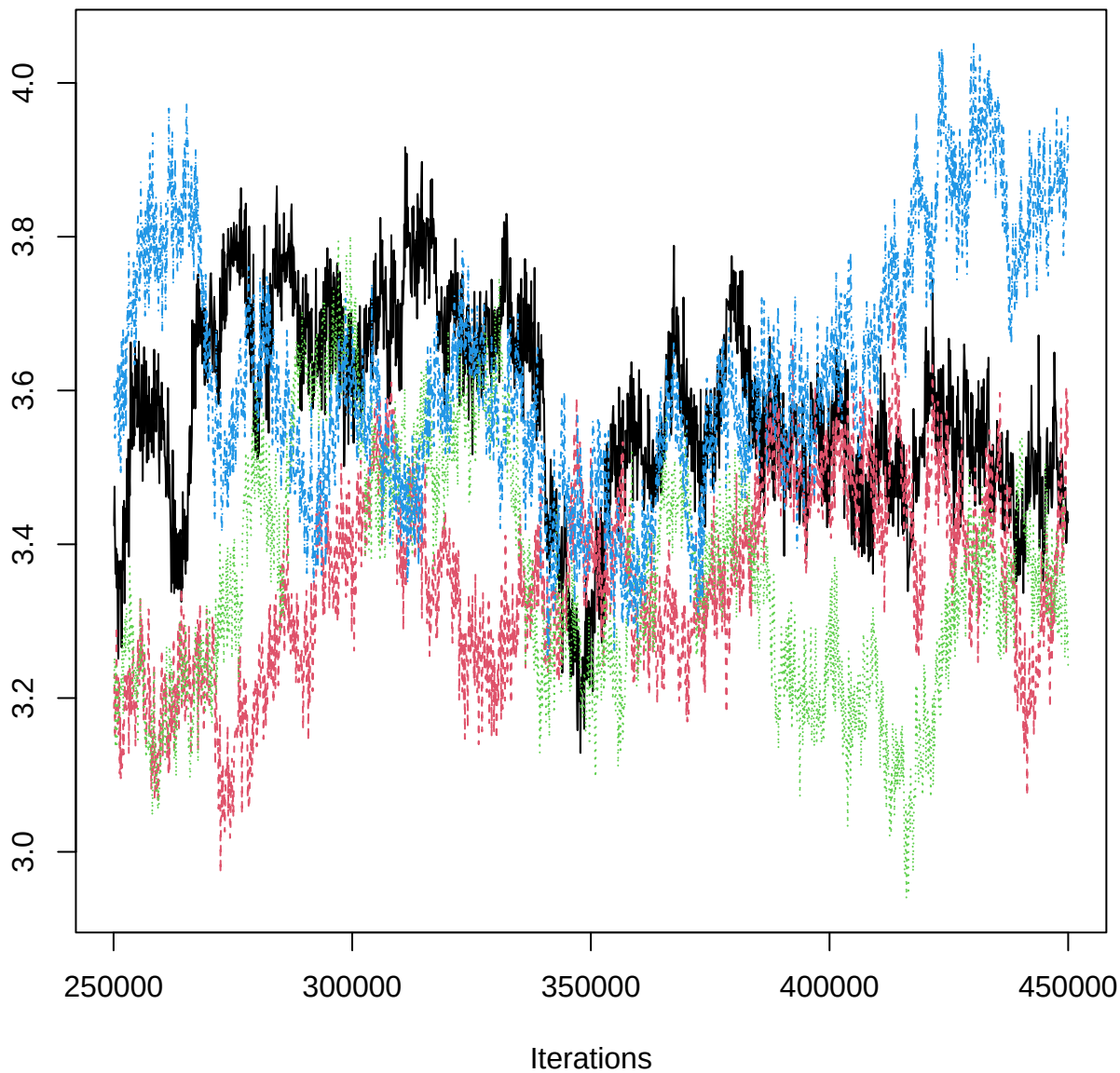
Traceplot – B[MAT (C3), PIB_n (S13)]
