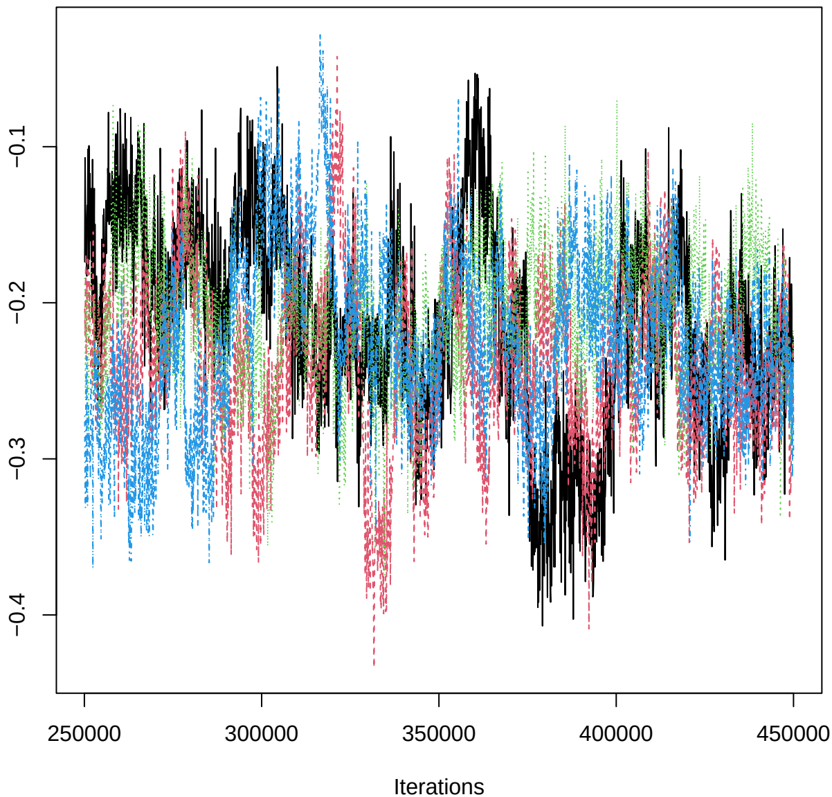
Traceplot – B[twi (C8), PRP_n (S11)]
