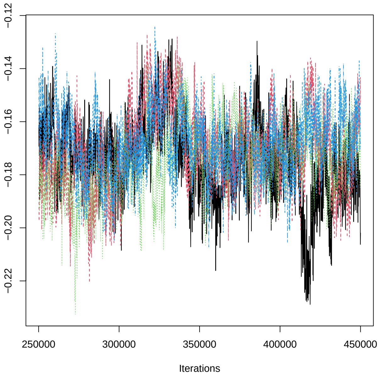
Traceplot – B[Clay (C5), PIG_n (S14)]
