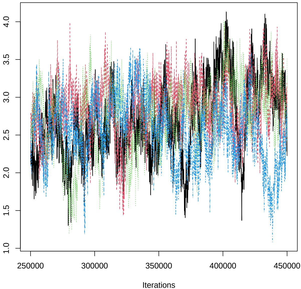
Traceplot – B[rtp (C7), HEG_n (S3)]
