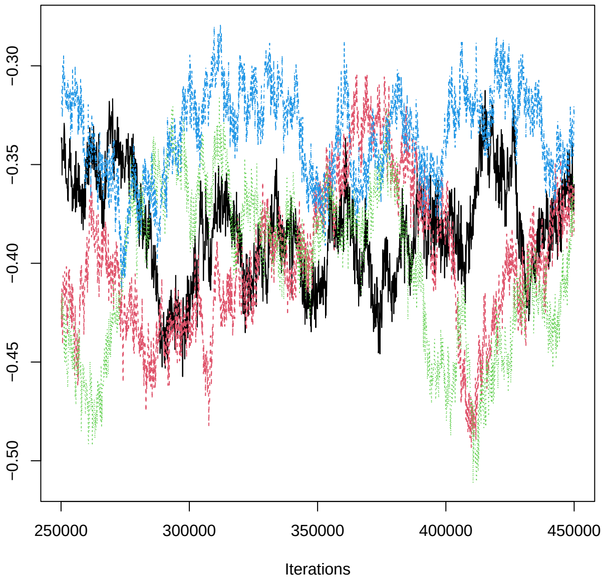
Traceplot – B[Clay (C5), HEG_n (S3)]
