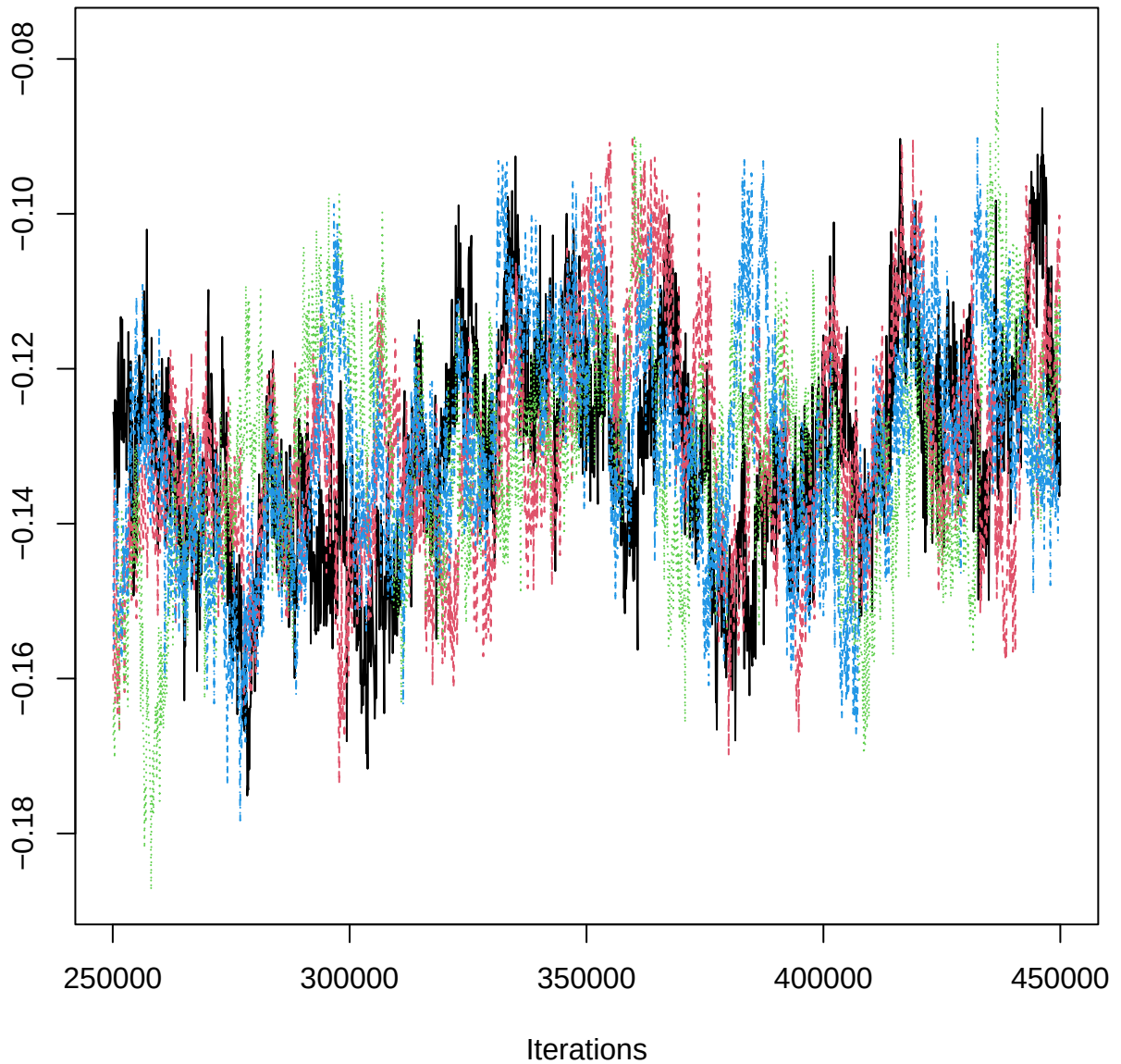
Traceplot – B[Clay (C5), BOJ_n (S4)]
