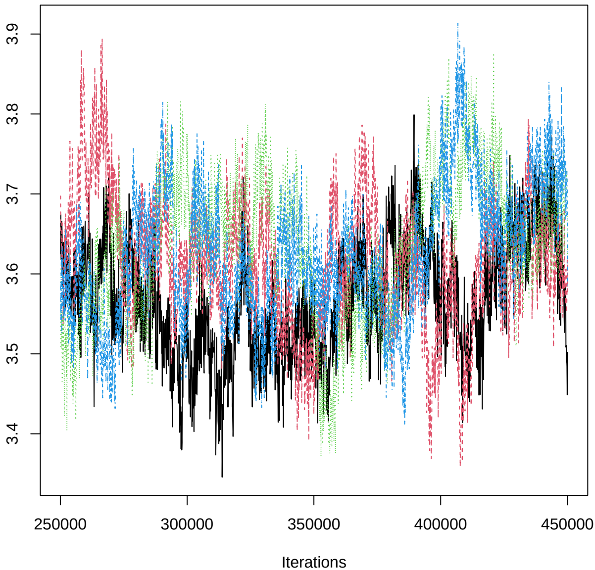
Traceplot – B[MAT (C3), ERR_n (S1)]
