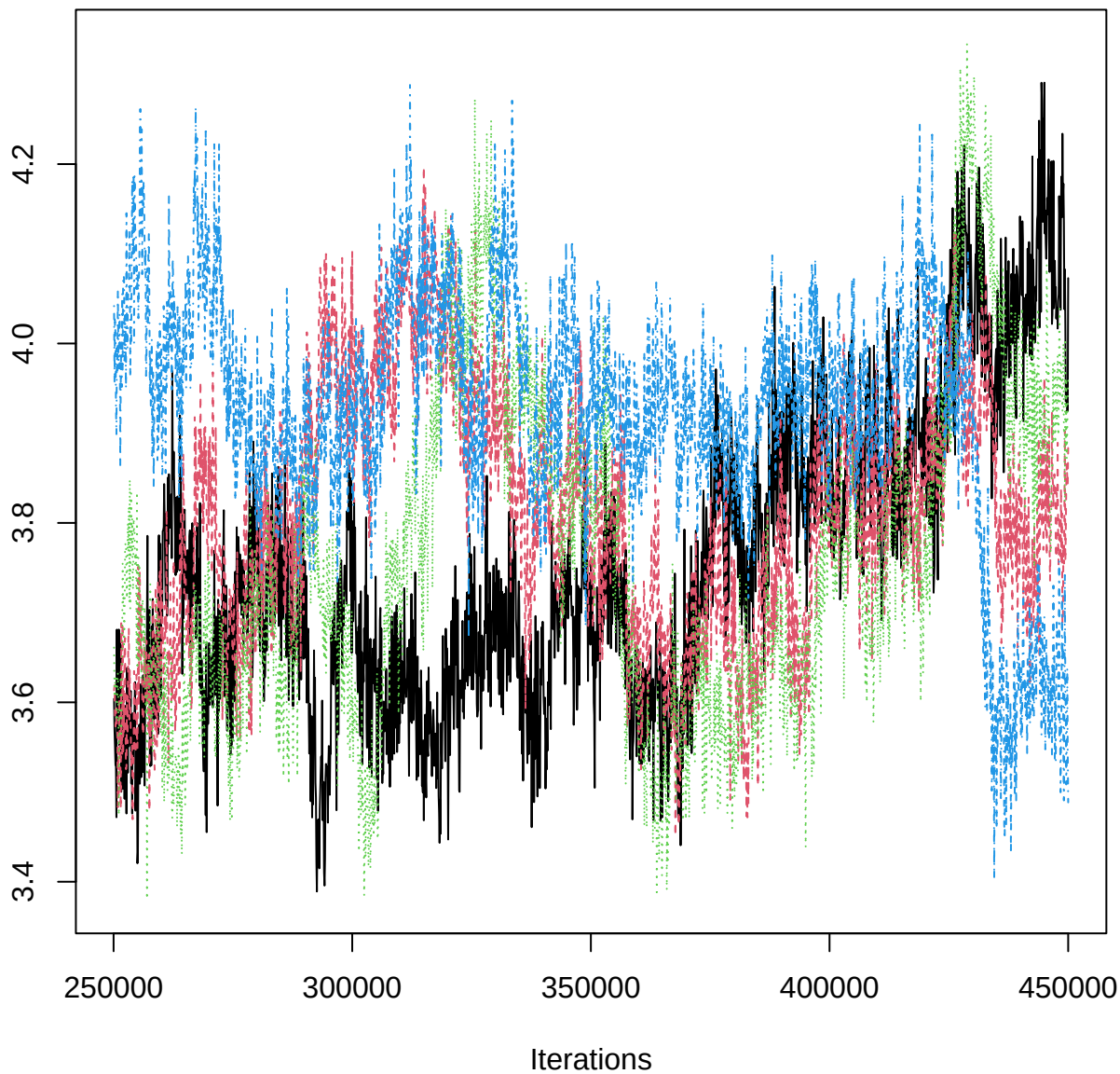
Traceplot – B[MAT (C3), THO_n (S10)]
