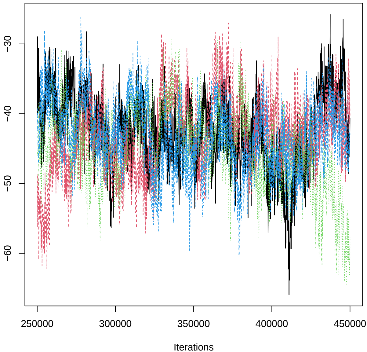
Traceplot – B[(Intercept) (C1), EPR_n (S7)]
