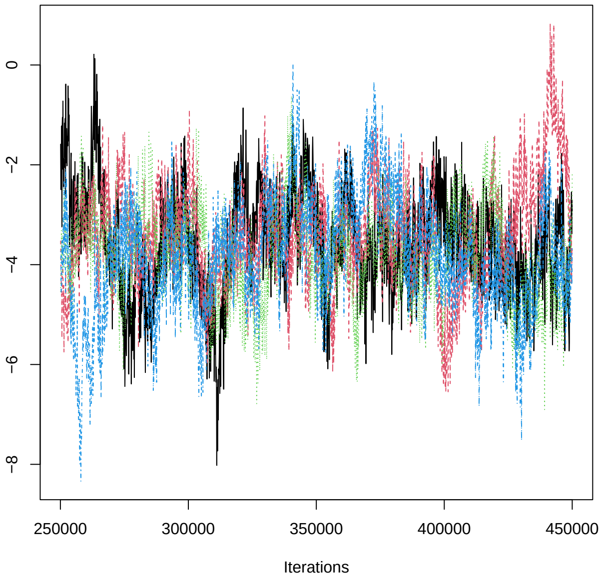
Traceplot – B[pH (C4), PIB_n (S13)]
