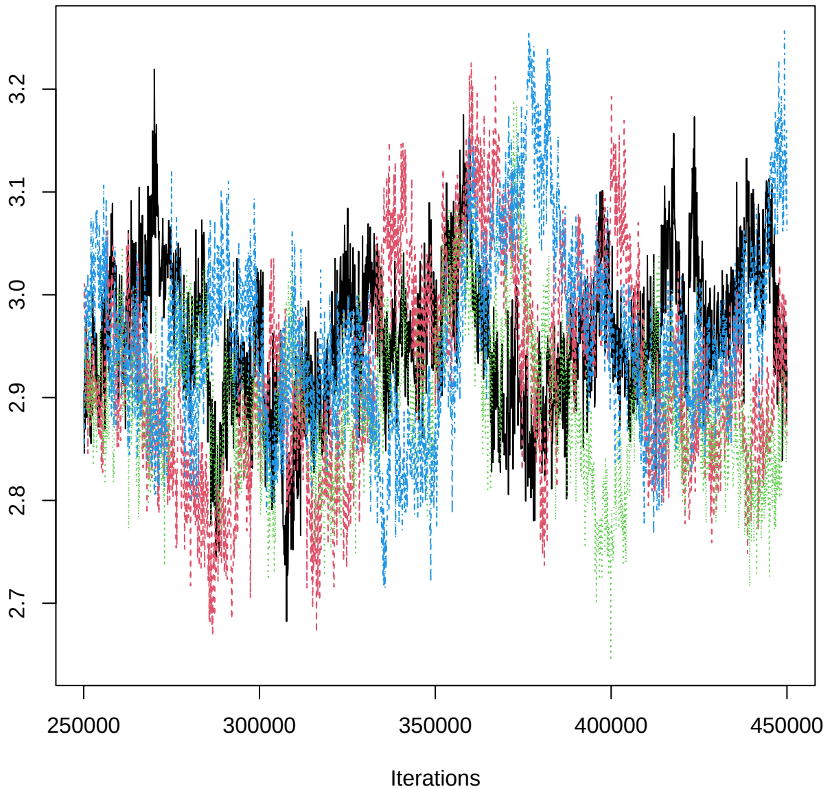
Traceplot – B[MAT (C3), BOJ_n (S4)]
