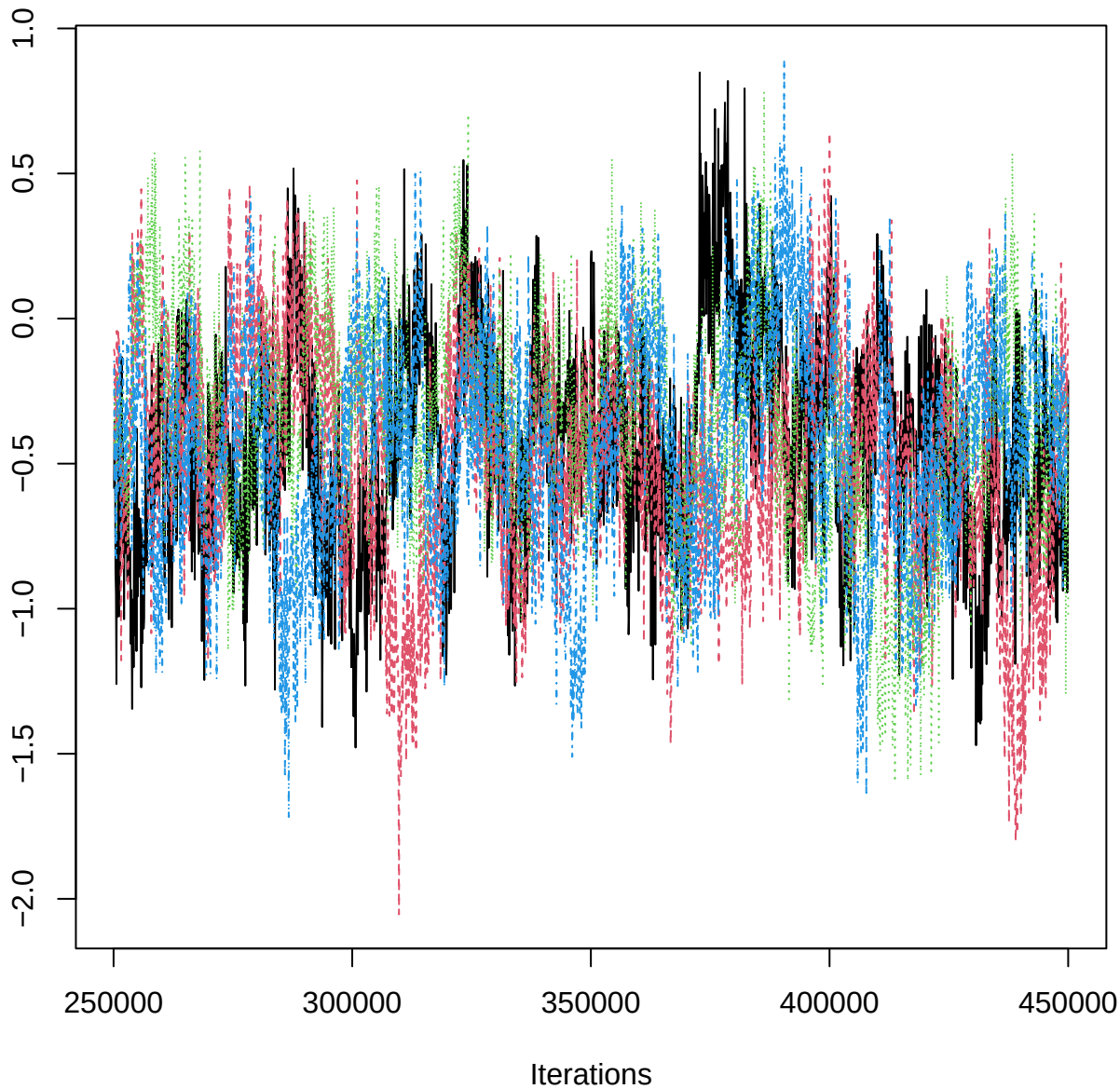
Traceplot – B[rtp (C7), PRP_n (S11)]
