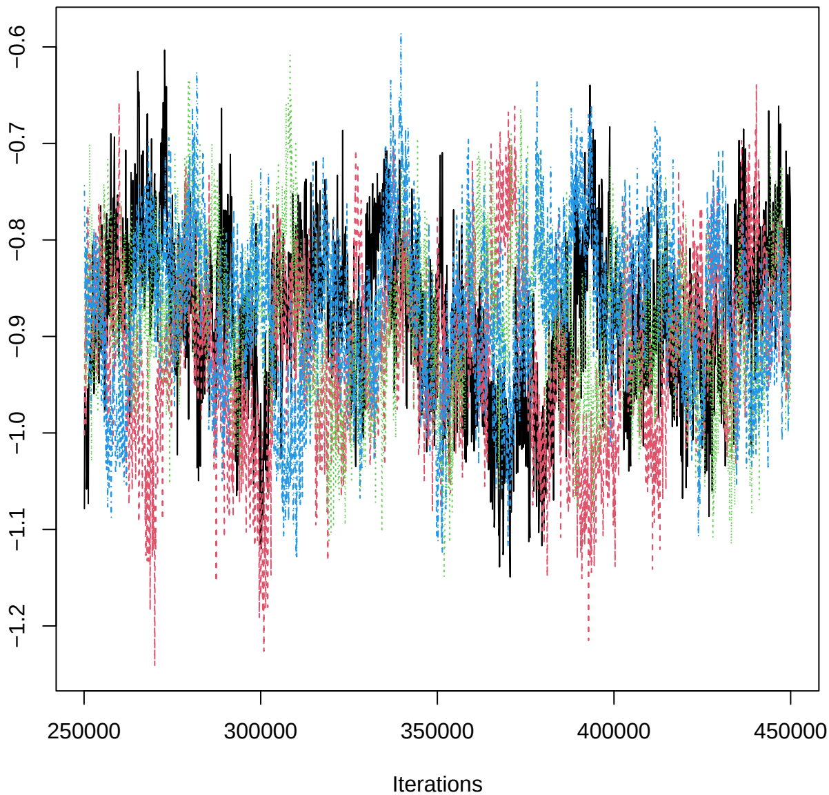
Traceplot – B[MAT (C3), PIG_n (S14)]
