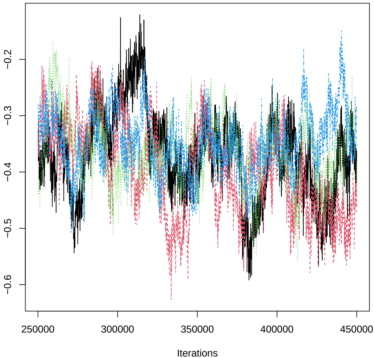
Traceplot – B[twi (C8), HEG_n (S3)]
