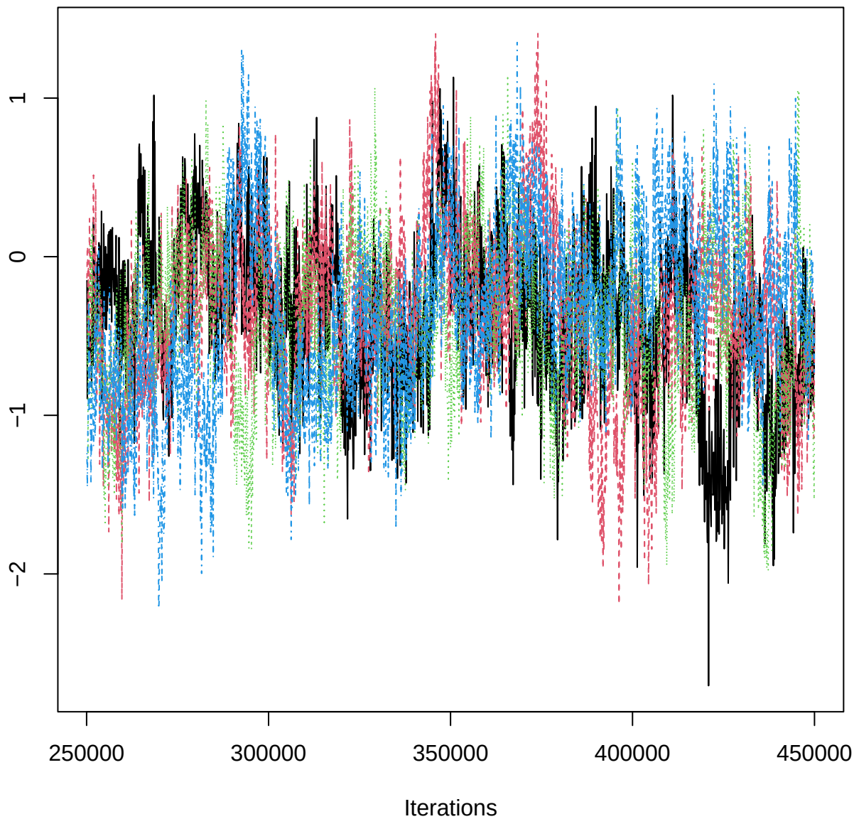
Traceplot – B[aspect_classS (C14), EPR_n (S7)]
