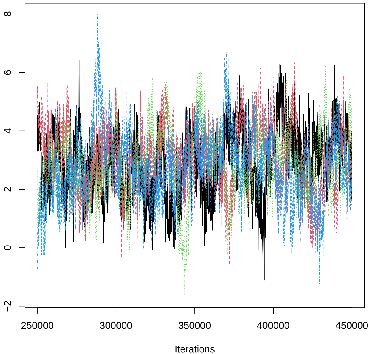
Traceplot – B[pH (C4), PIG_n (S14)]
