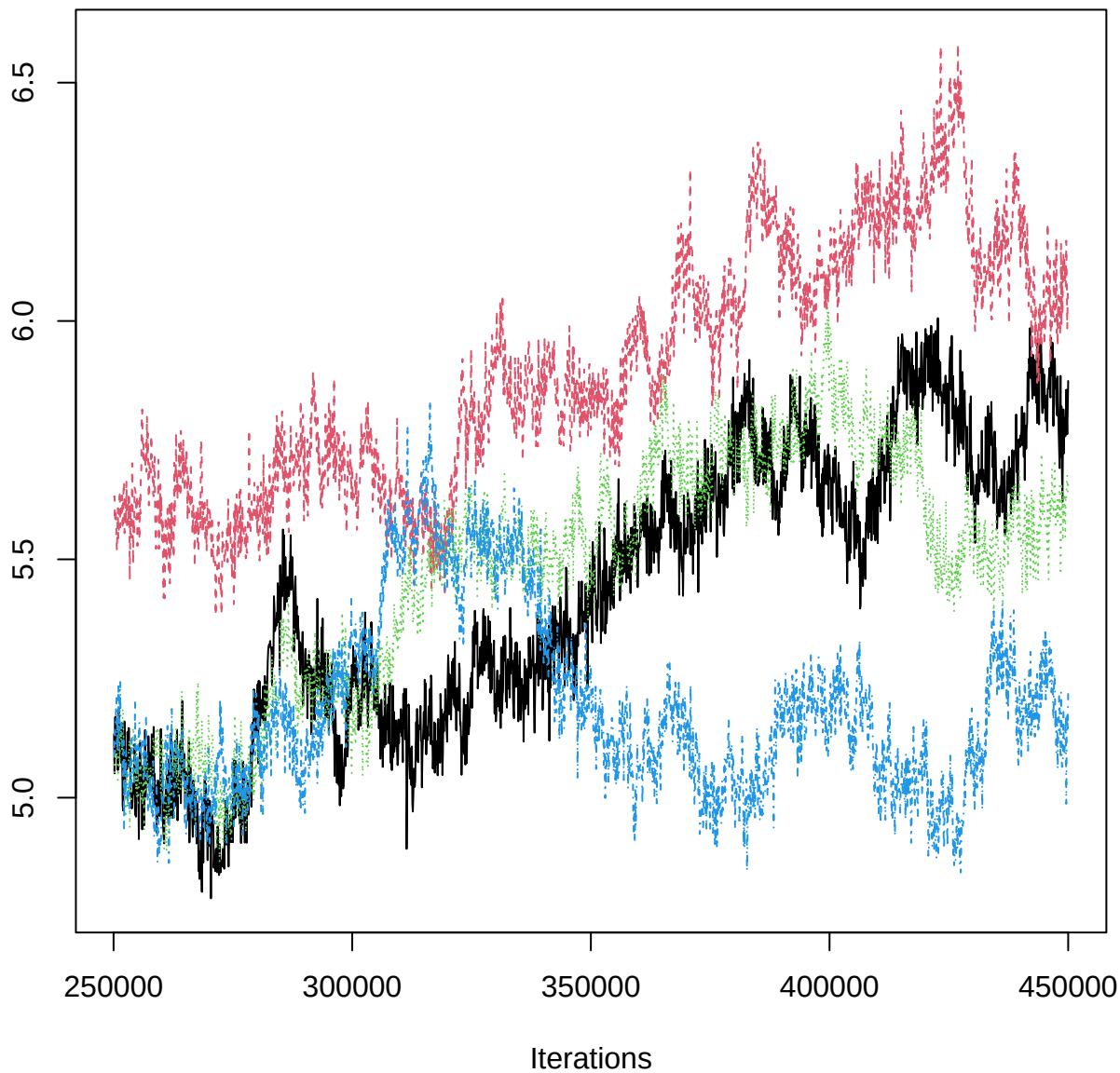
Traceplot – B[MAT (C3), HEG_n (S3)]
