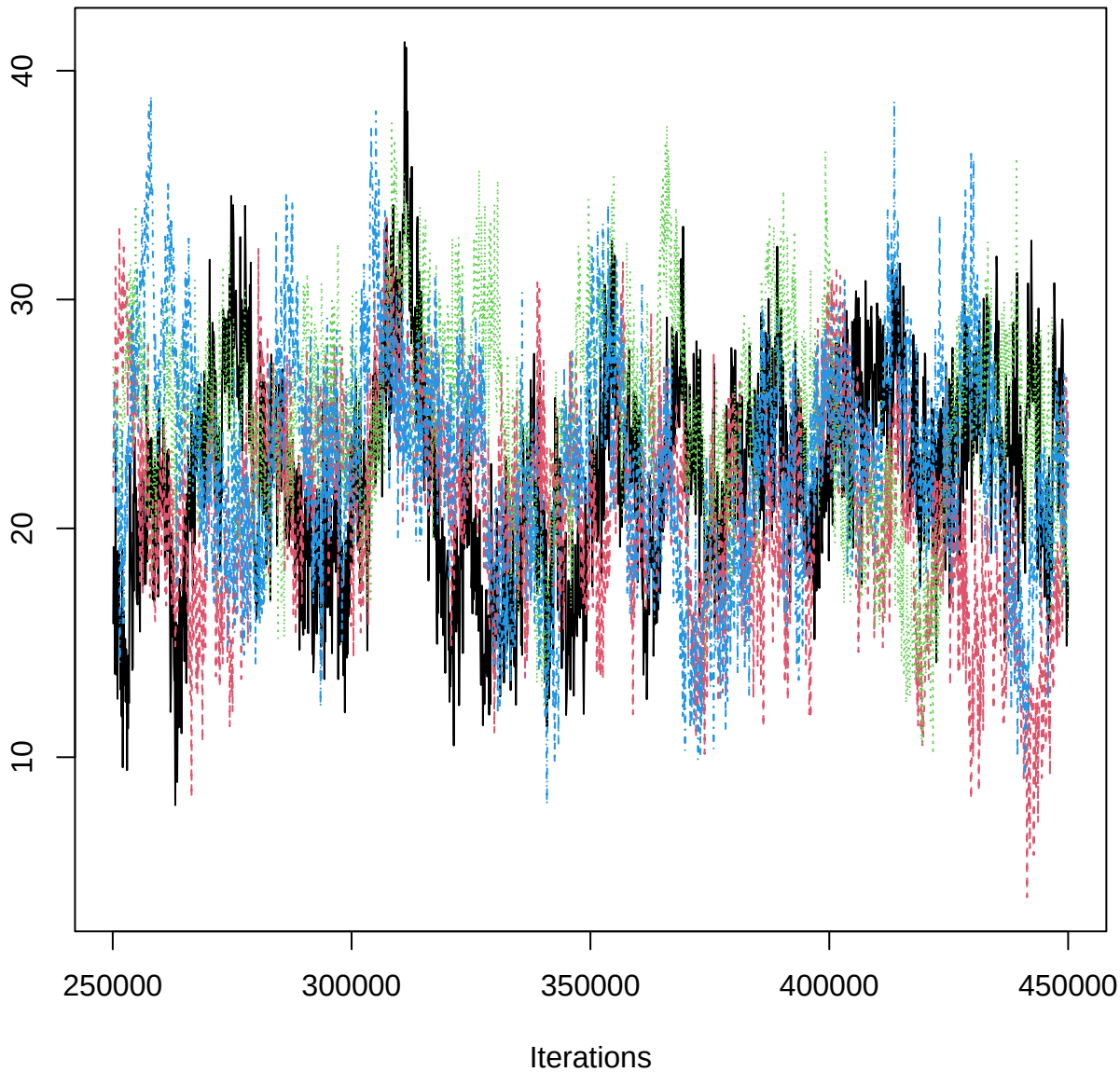
Traceplot – B[(Intercept) (C1), PIB_n (S13)]
