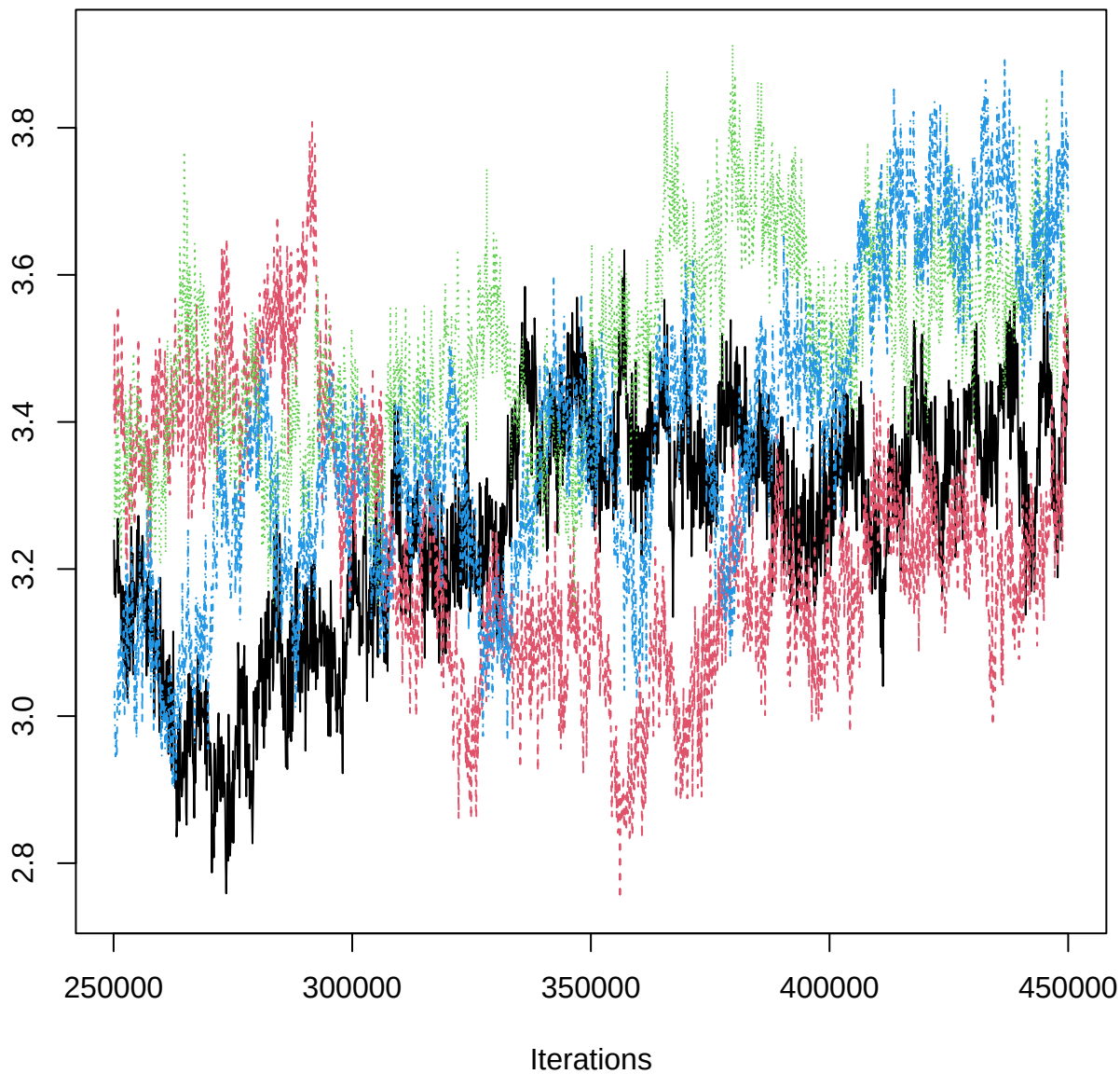
Traceplot – B[MAT (C3), EPR_n (S7)]
