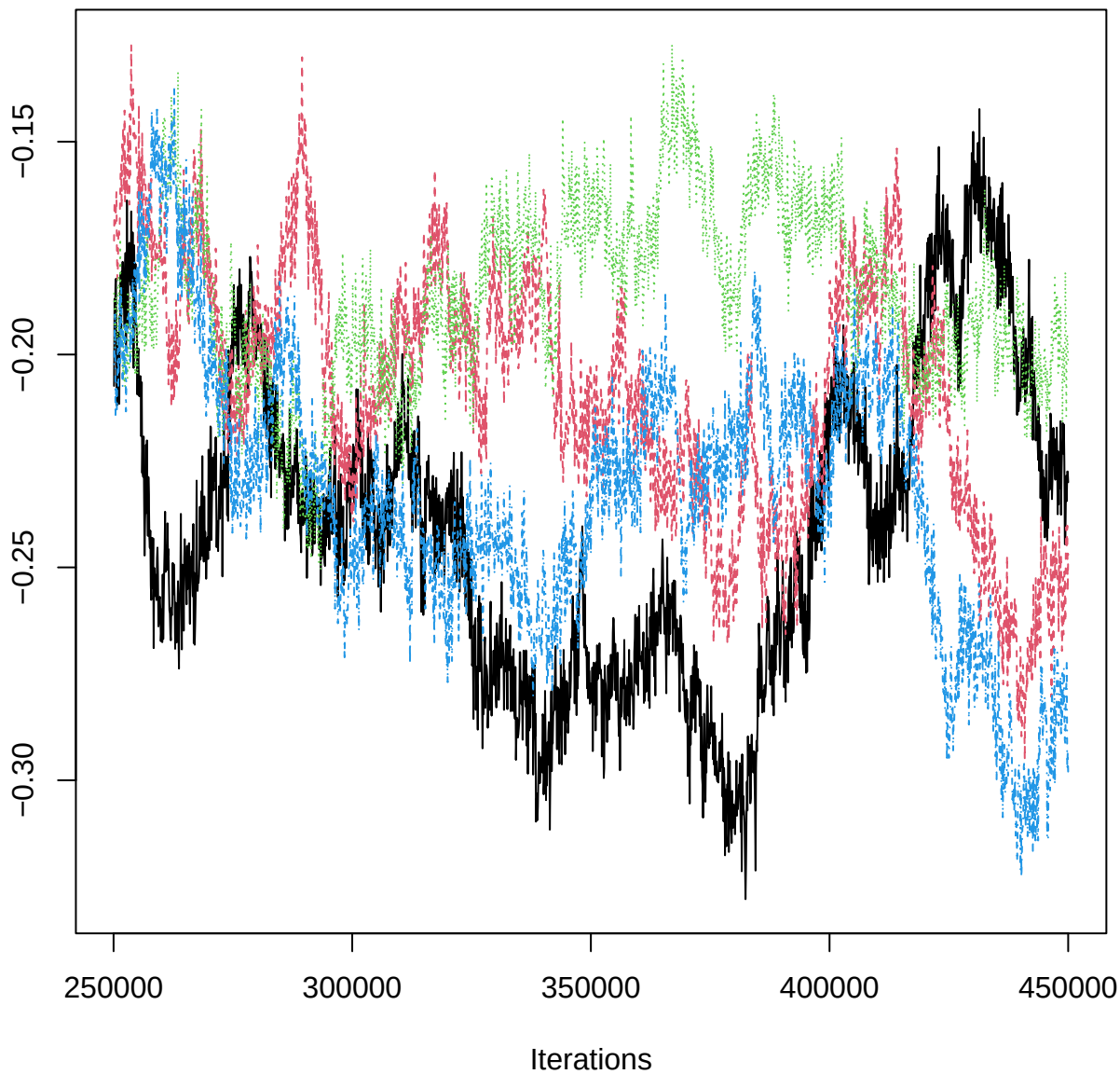
Traceplot – B[Clay (C5), PIB_n (S13)]
