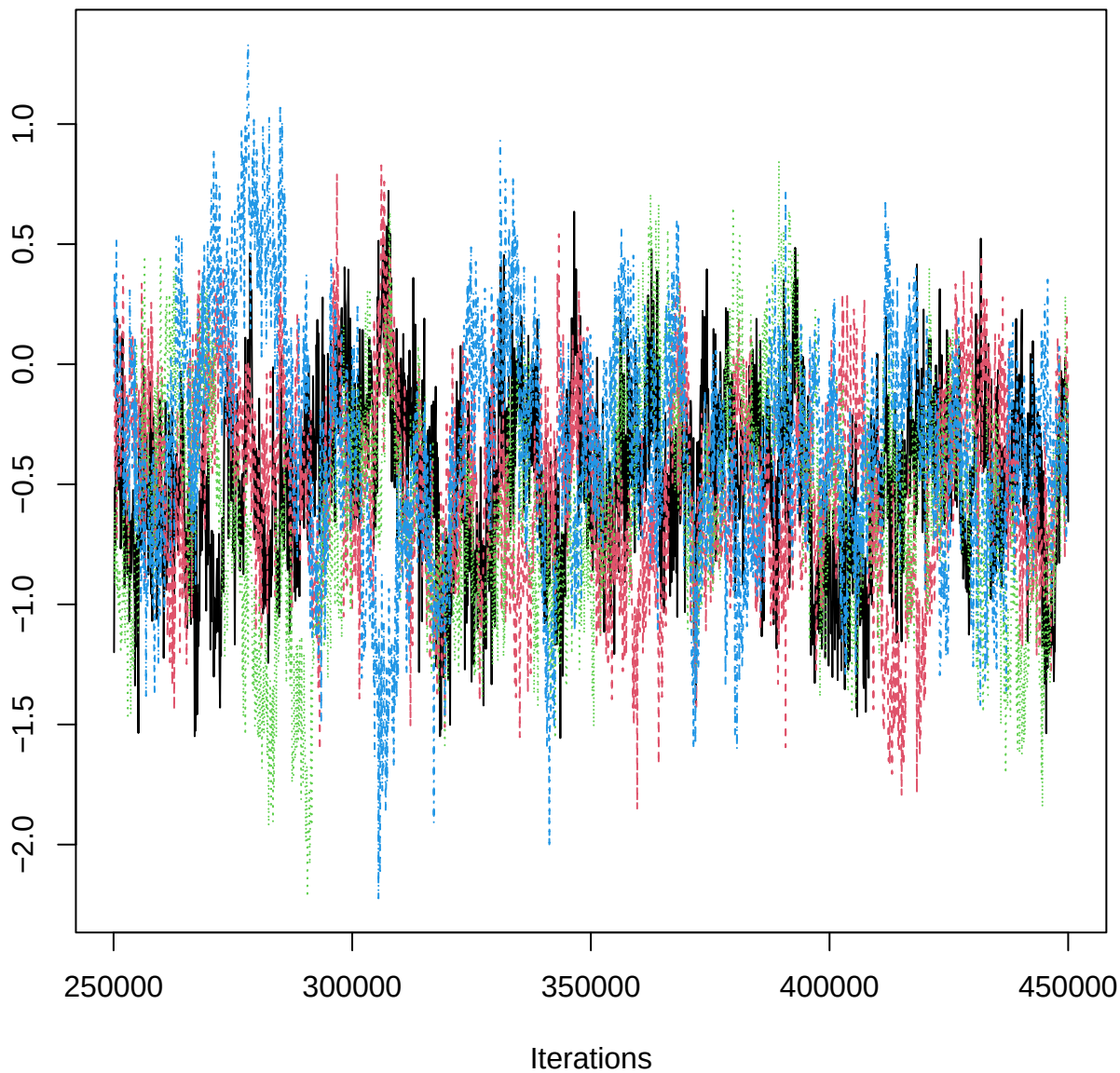
Traceplot – B[aspect_classNW (C13), PIB_n (S13)]
