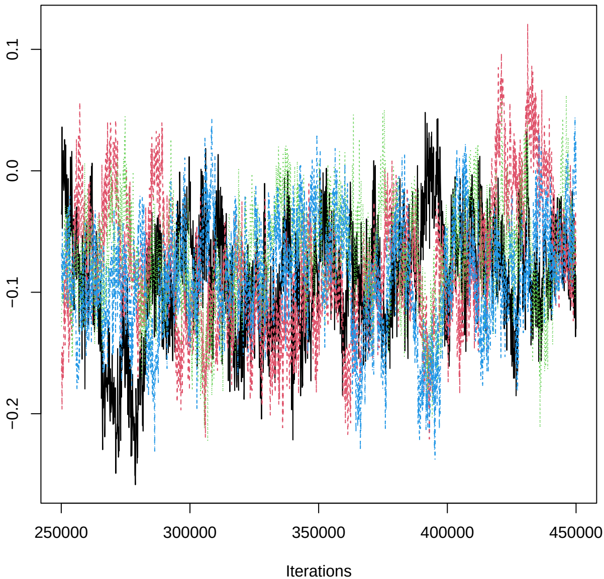
Traceplot – B[twi (C8), PIB_n (S13)]
