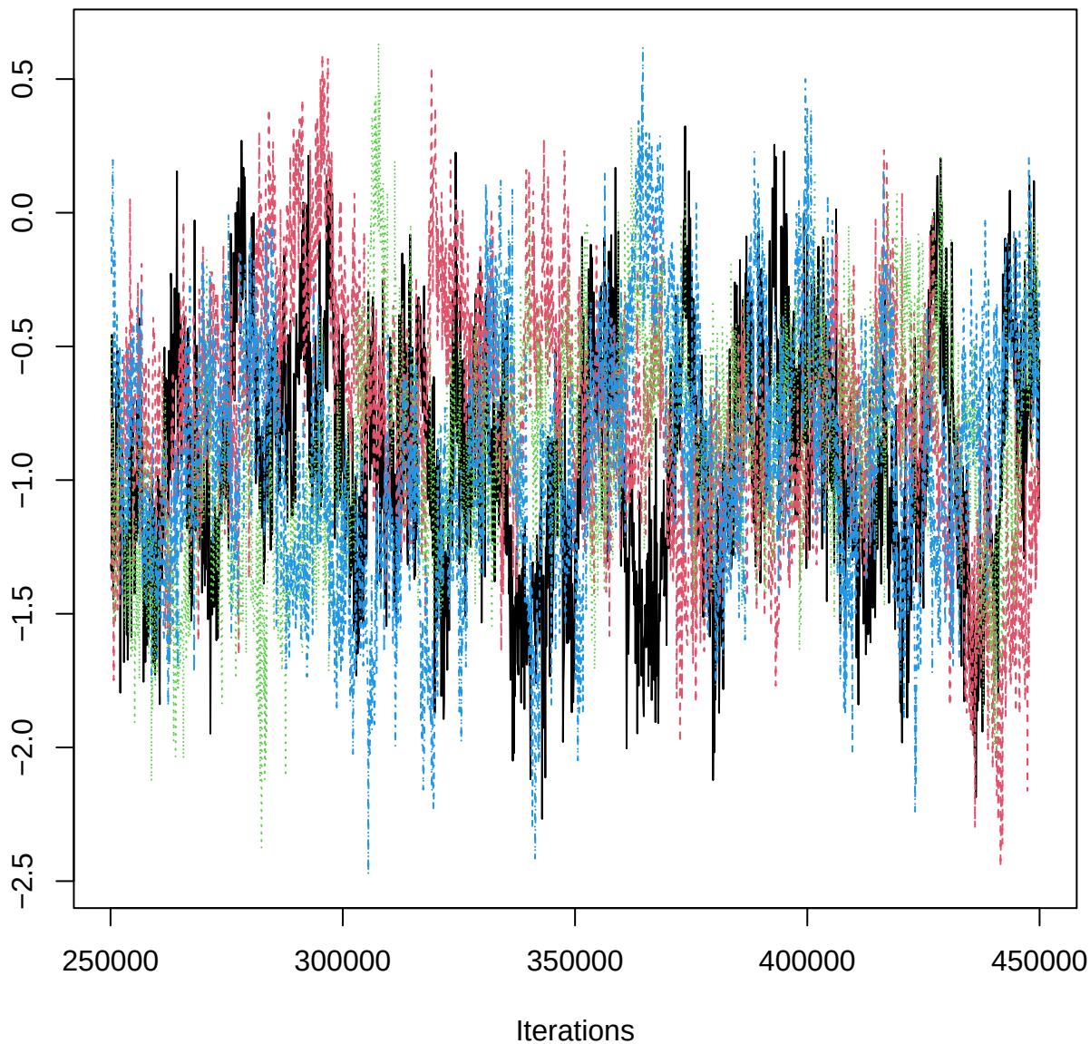
Traceplot – B[aspect_classNE (C12), PIB_n (S13)]
