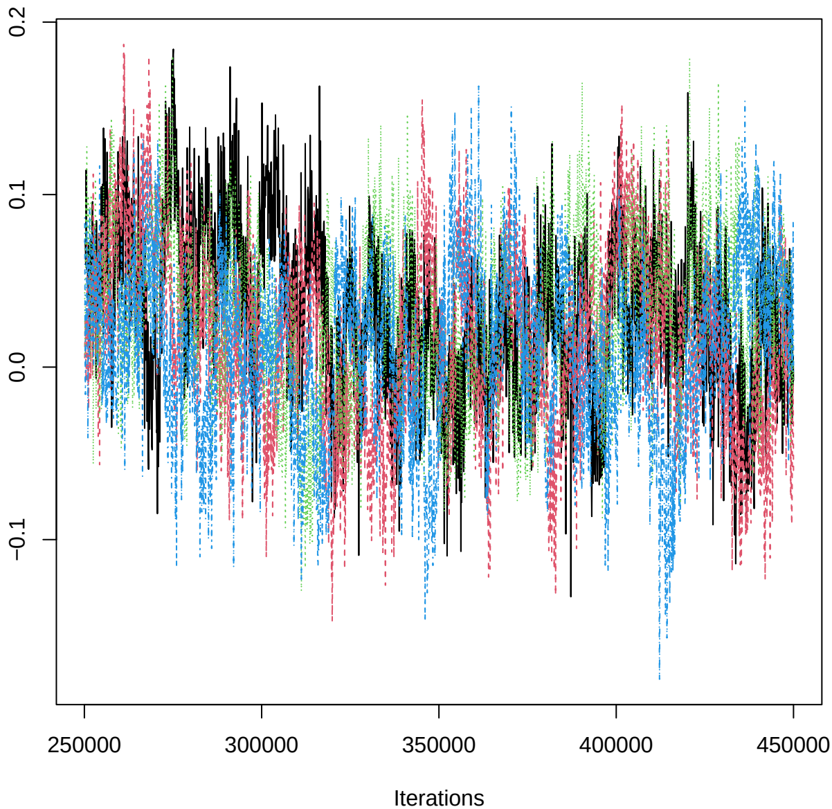
Traceplot – B[twi (C8), THO_n (S10)]
