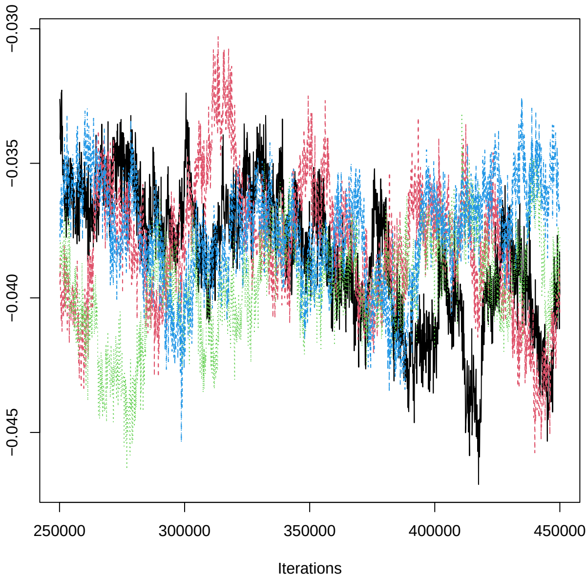
Traceplot – B[MAP (C2), PIG_n (S14)]
