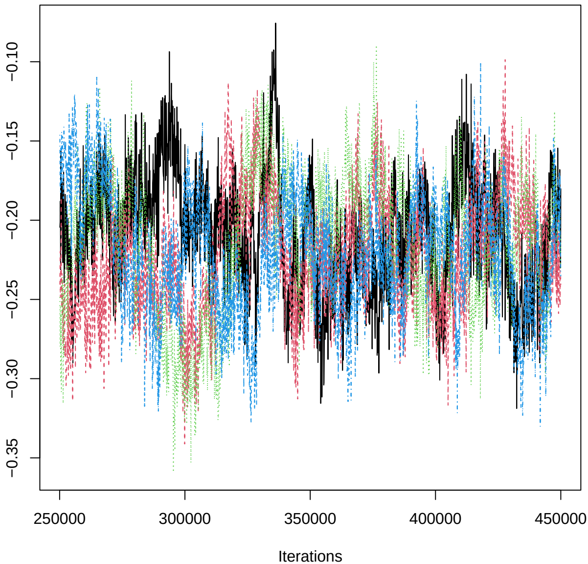
Traceplot – B[slope (C9), PIG_n (S14)]
