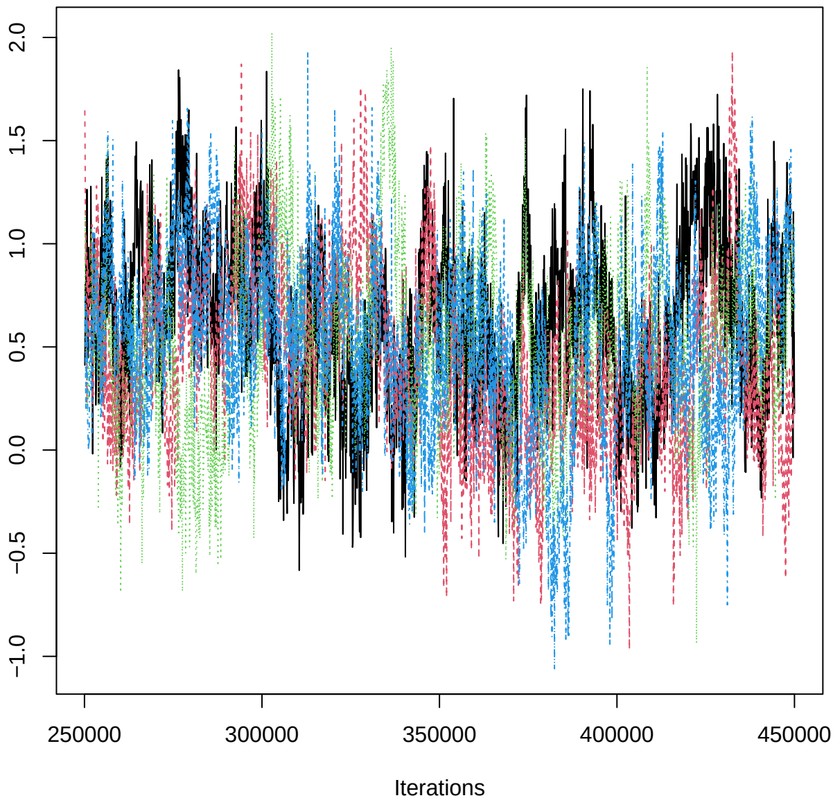
Traceplot – B[aspect_classSE (C15), PIB_n (S13)]
