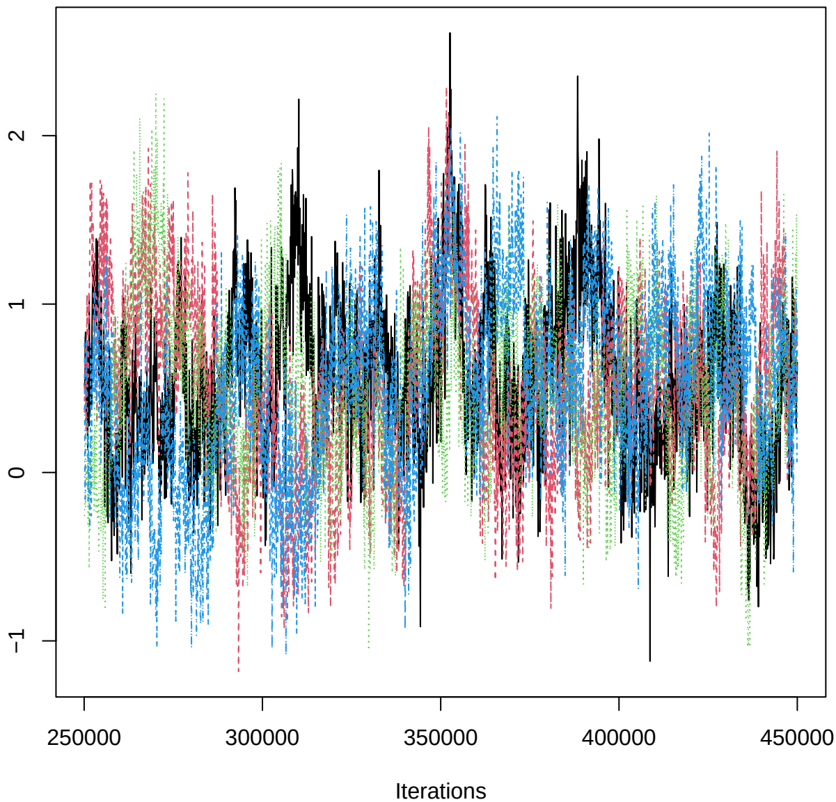
Traceplot – B[aspect_classW (C17), EPR_n (S7)]
