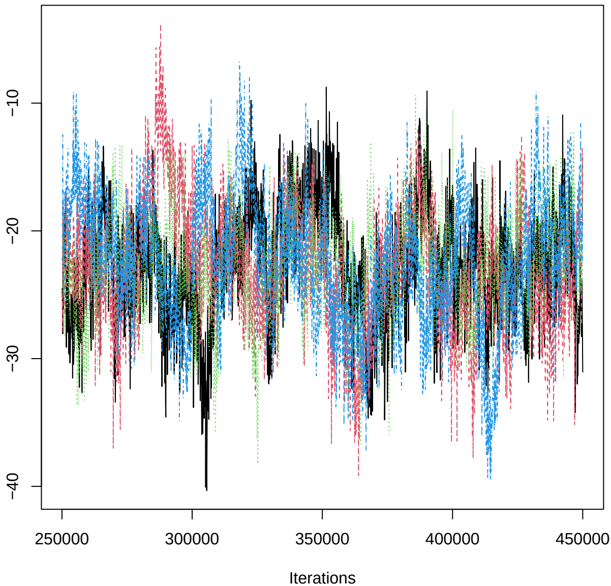
Traceplot – B[(Intercept) (C1), PRP_n (S11)]
