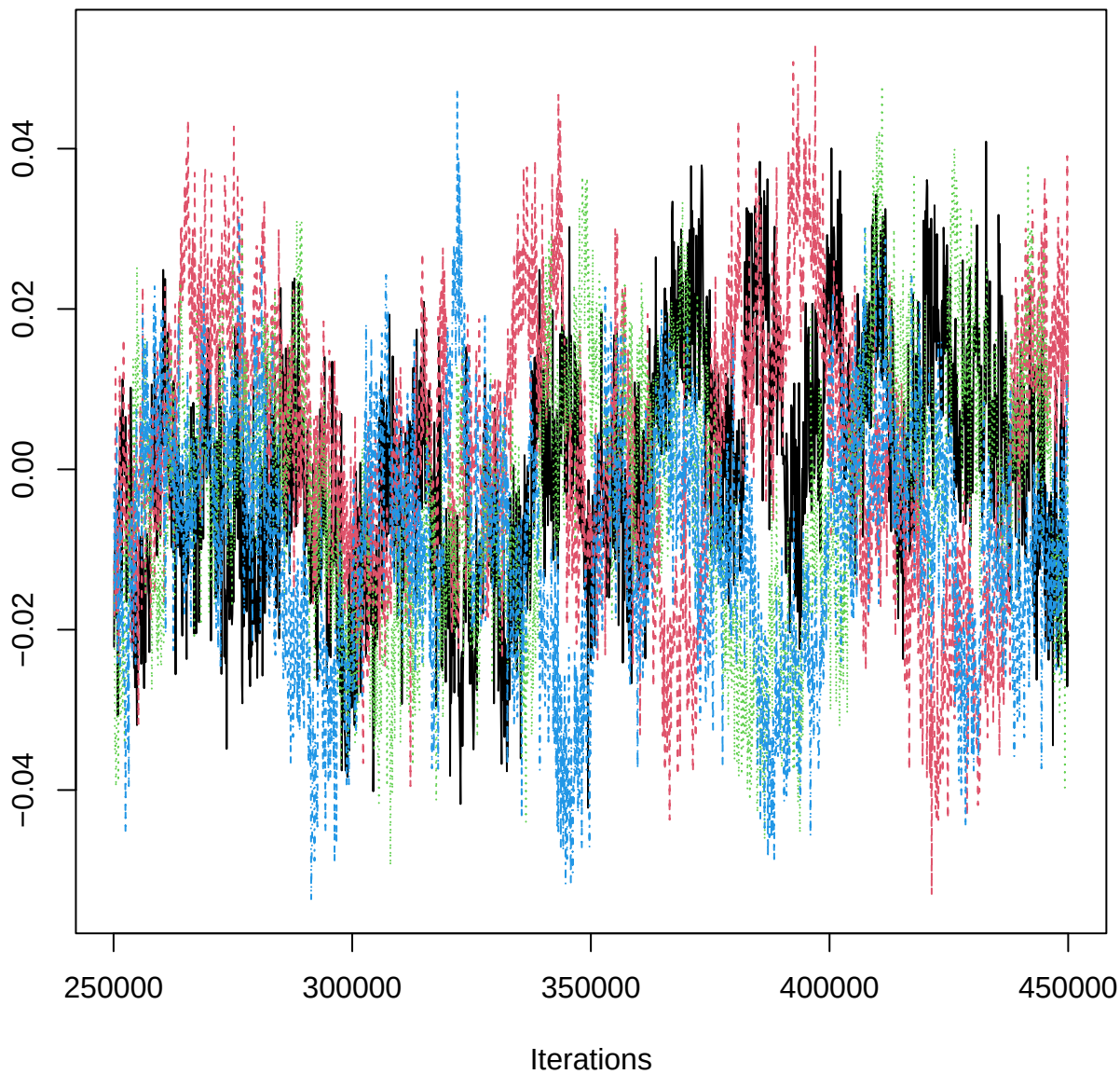
Traceplot – B[Clay (C5), PRP_n (S11)]
