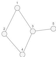
Adjacency Matrix
