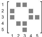
Adjacency Matrix
