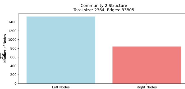
Community 2 Structure
