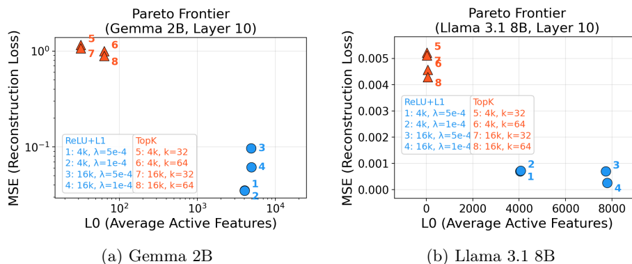
Fig. 2: Pareto frontier: reconstruction loss (MSE) vs. sparsity ( \ell_0 -norm L_0 ) for all 8 SAE configurations per model. Blue circles = ReLU+L1; orange triangles = TopK. Gemma axes are on a log scale; Llama axes are linear.
