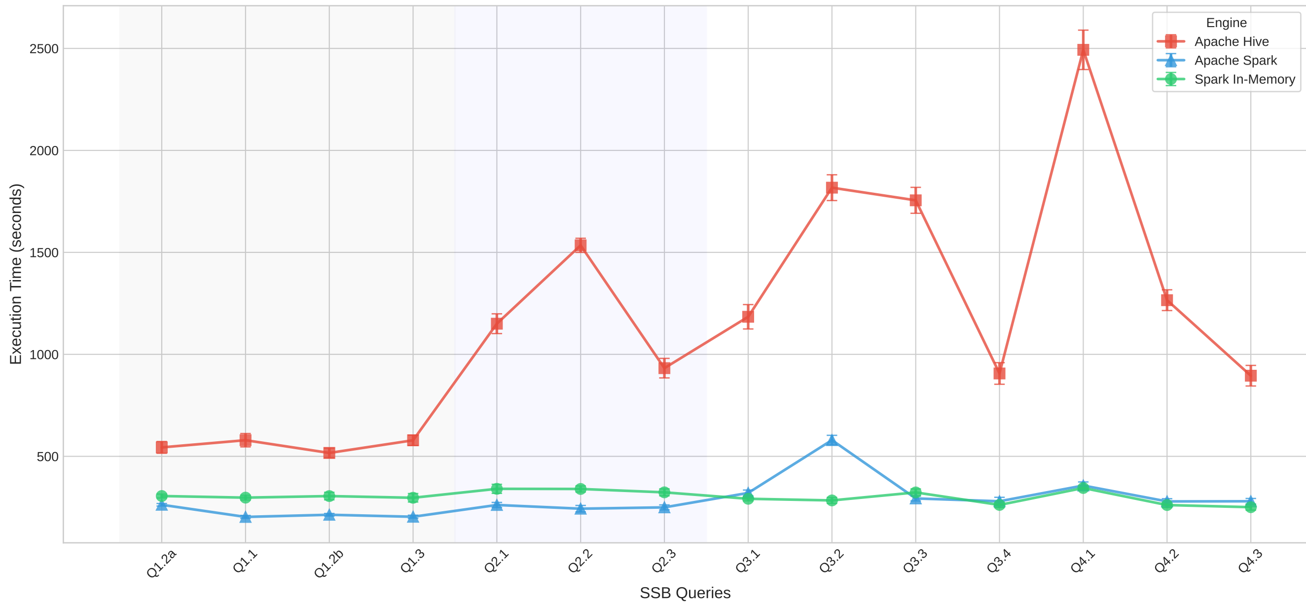
Performance Comparison by Query Groups (SSB Redefined)
