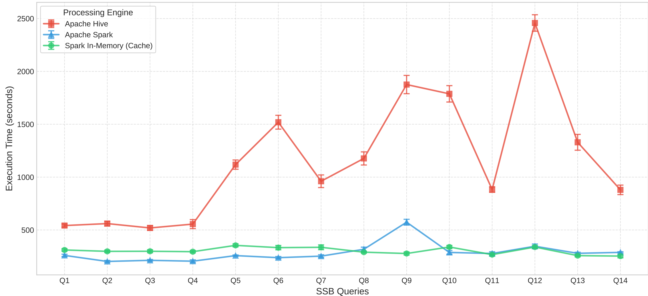
Query Execution Time Comparison: Hive vs. Spark vs. Spark In-Memory (Simulated)
