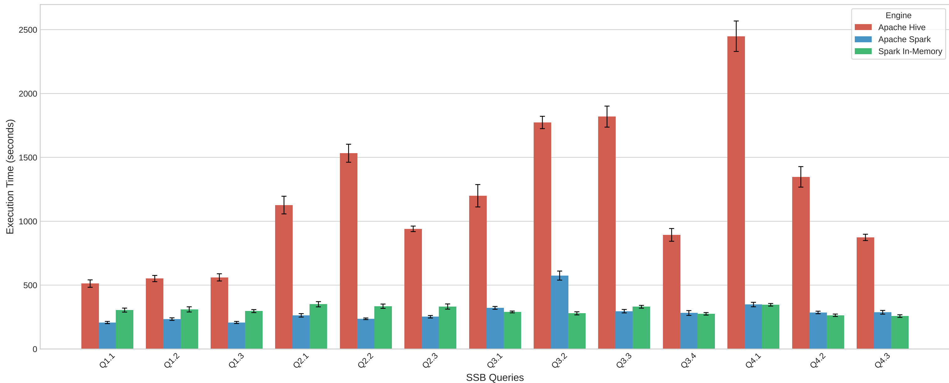
Individual Performance Comparison (Execution Time per Query)
