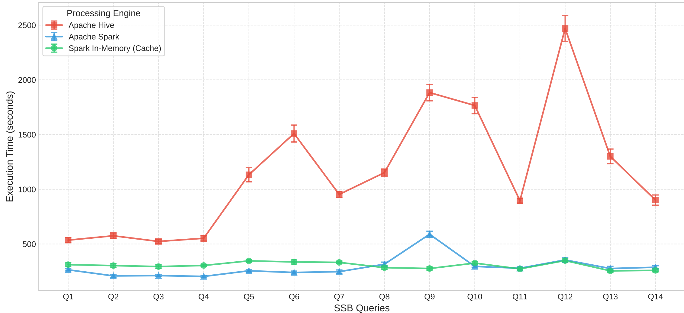
Query Execution Time Comparison: Hive vs. Spark vs. Spark In-Memory
