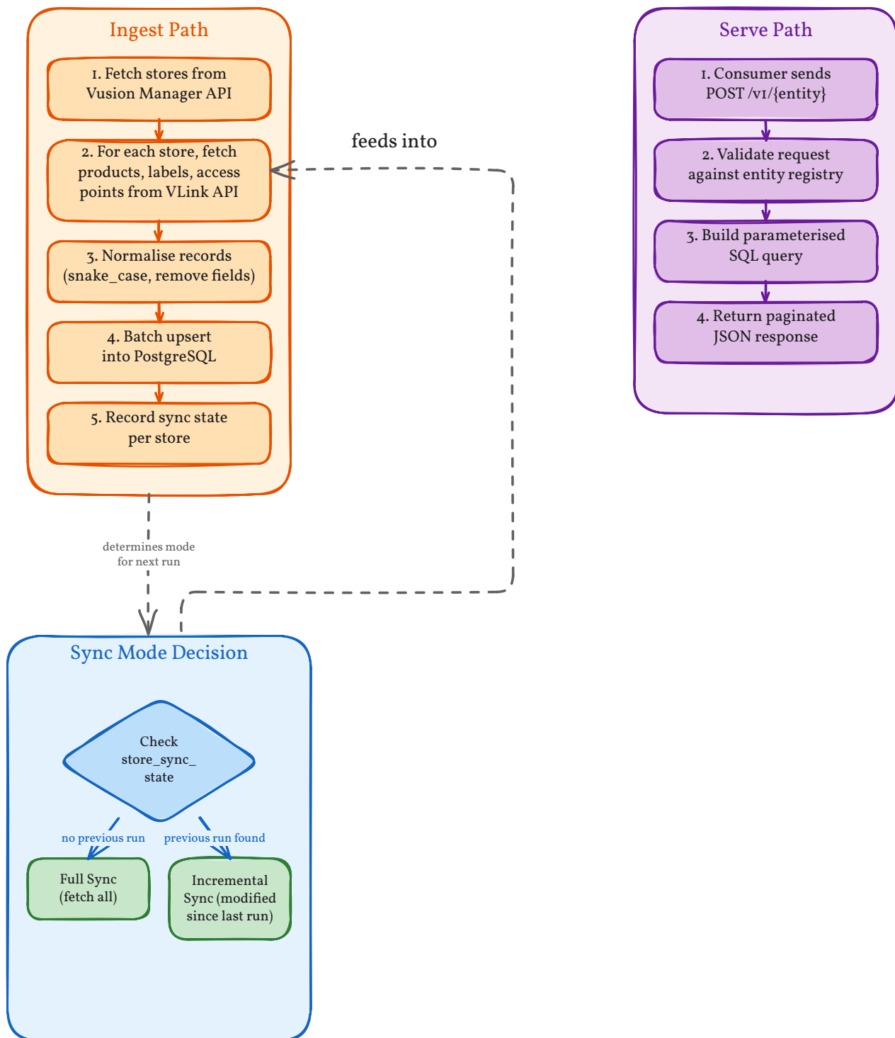
Figure 2: Data Flow
