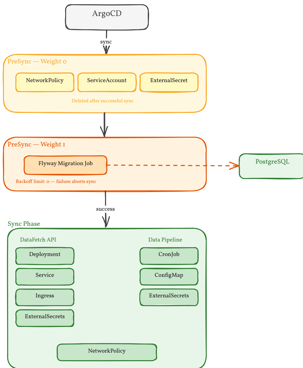
Figure 5: Deployment Flow
