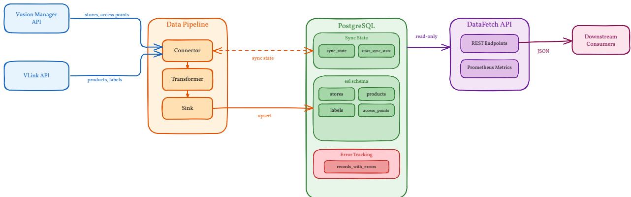
Figure 1: System Architecture
