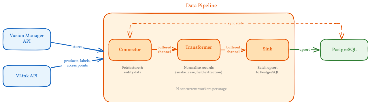
Figure 4: Pipeline Architecture
