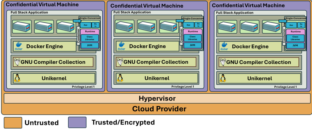
Fig. 5. CVMs deploying Unikernel-based TCB-optimized confidential containers, each encapsulating a full-stack application.
