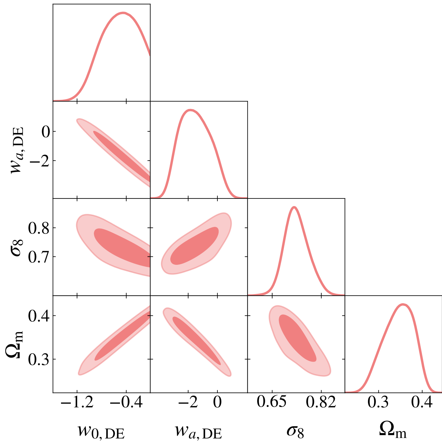
Data: DES-Y3 Cosmic Shear + DESI DR2 BAO
