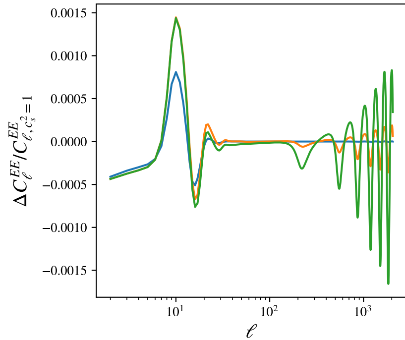
CMB Polarization
