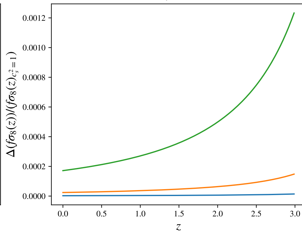
f\sigma_8(z)
