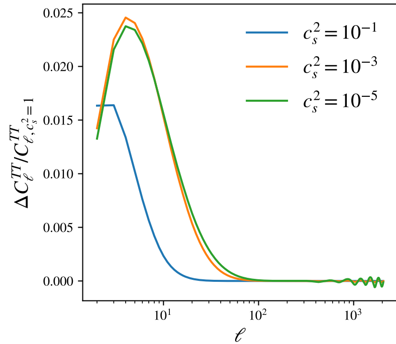
CMB Temperature
