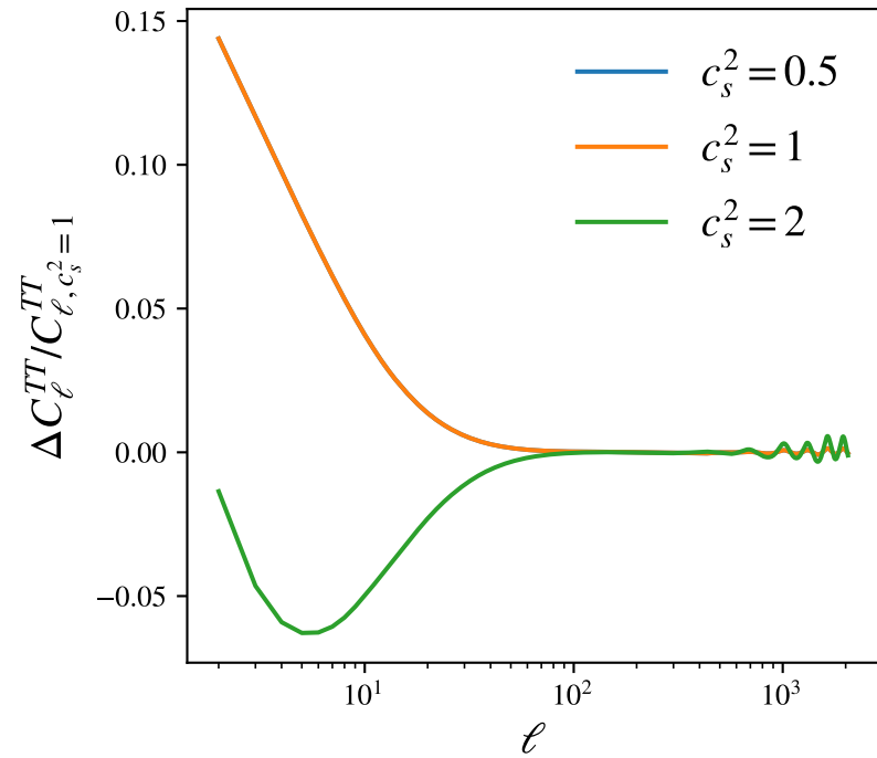
CMB Temperature
