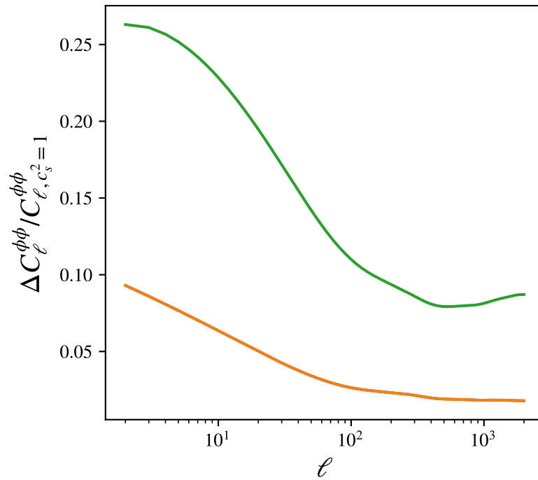
CMB Lensing
