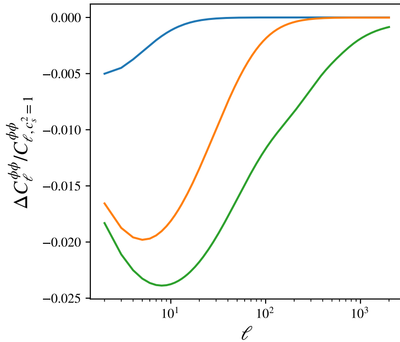
CMB Lensing
