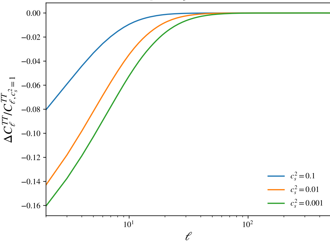
Impact of c_s^2 on CMB TT
