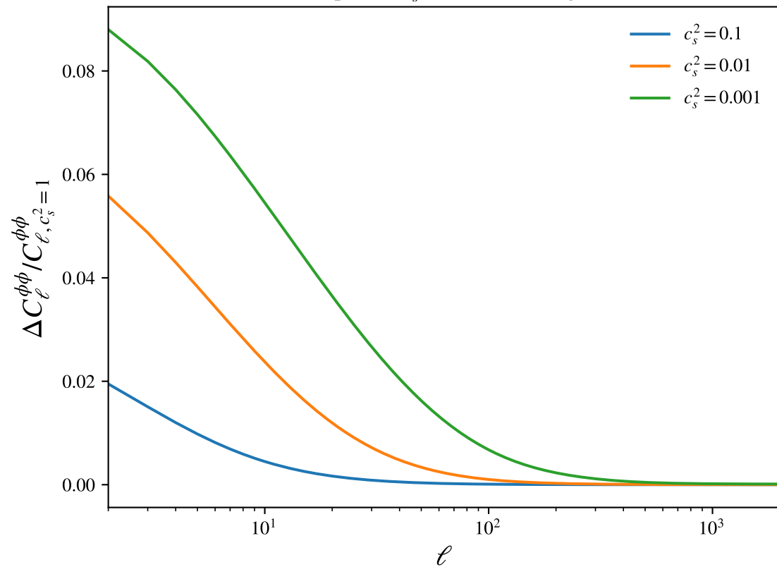
Impact of c_s^2 on CMB lensing
