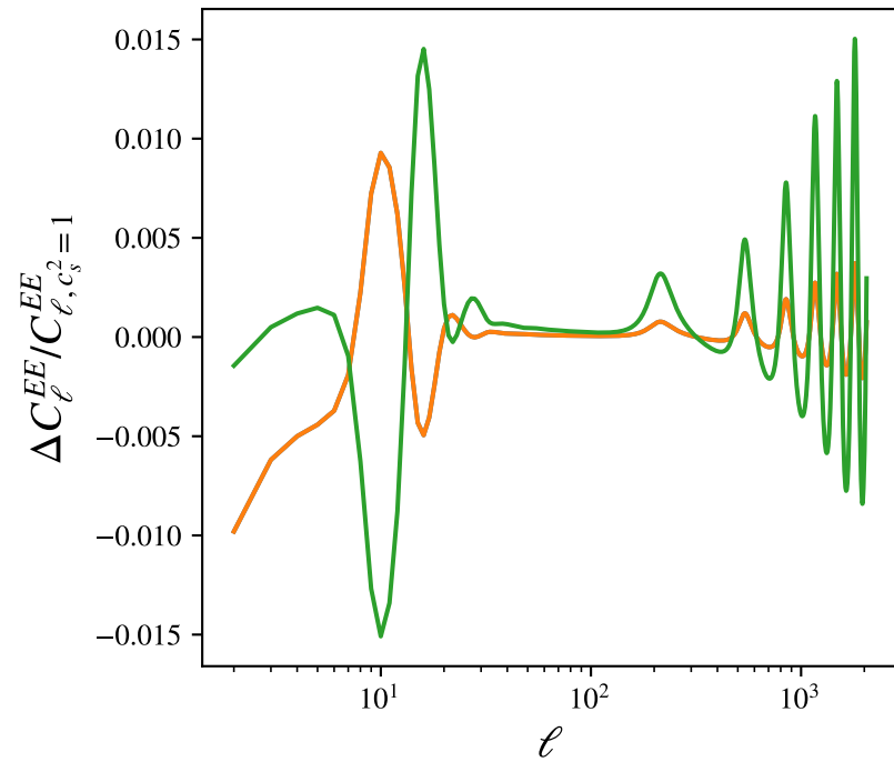
CMB Polarization
