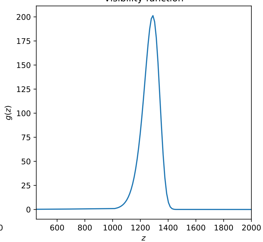
Visibility function
