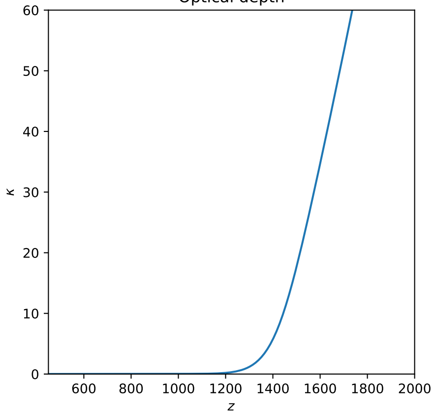
Optical depth
