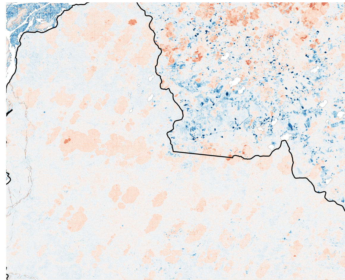
Predicted \Delta NDMI
