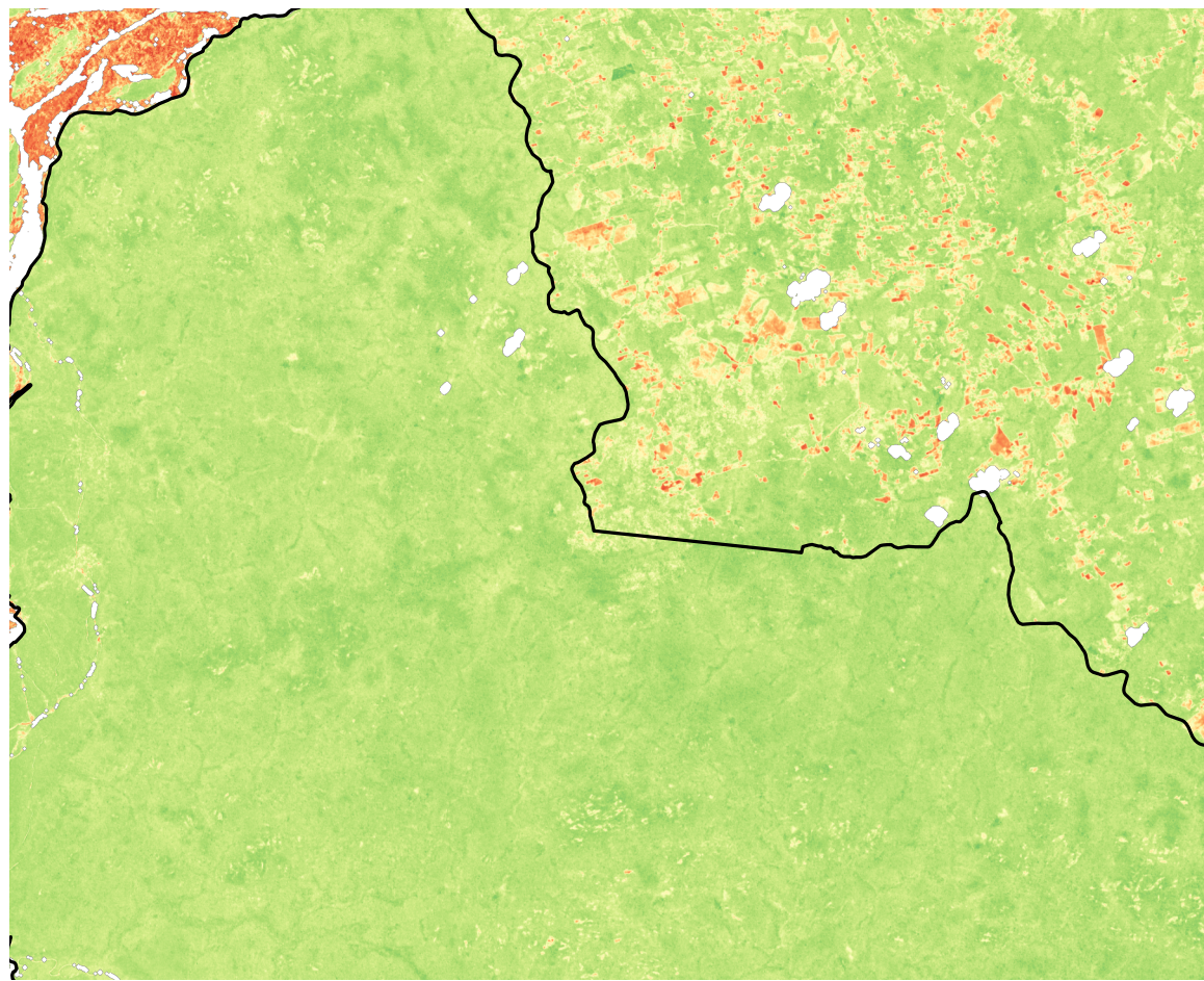
Last Observed NDMI — 2025-08-12
