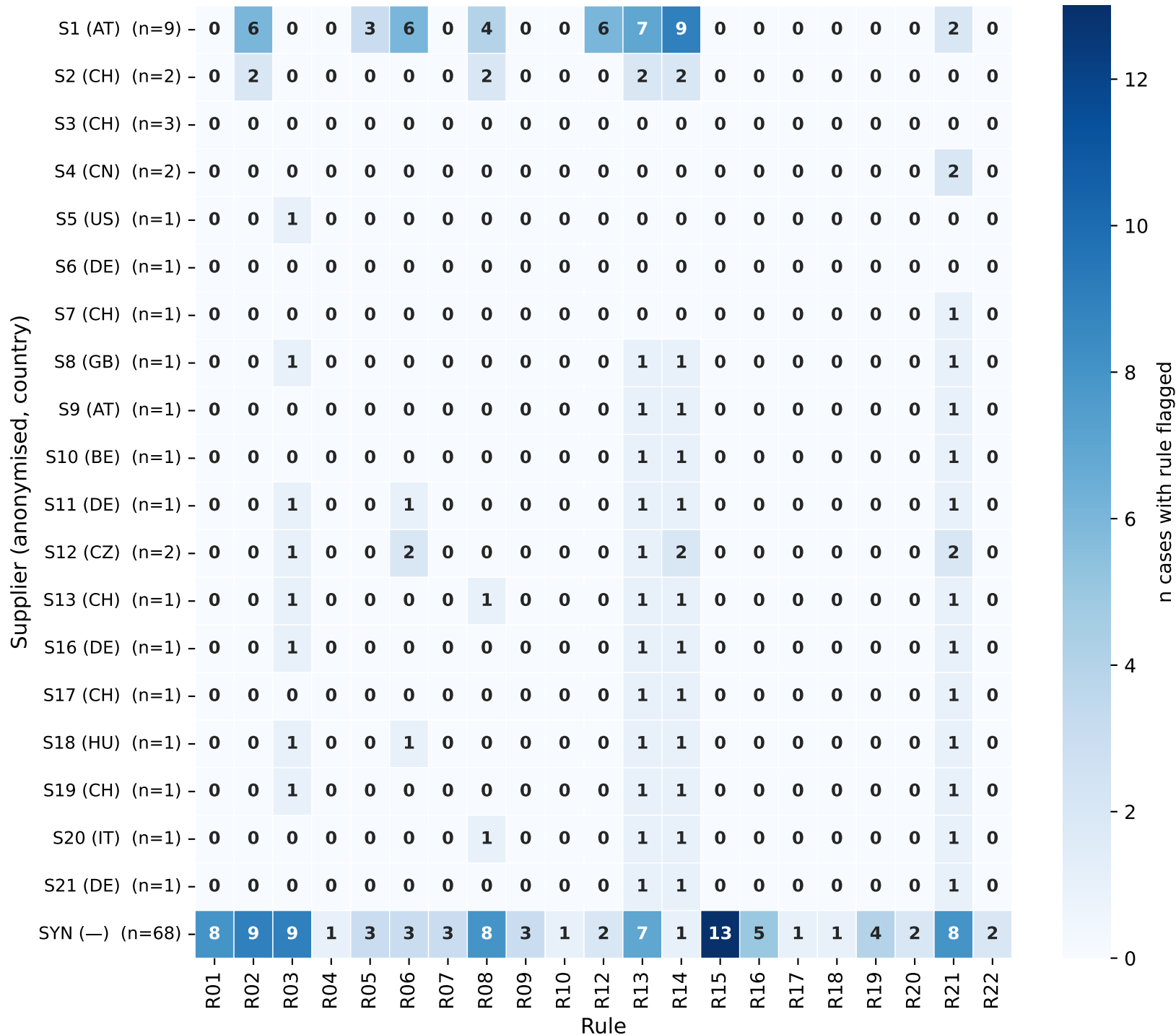
Figure 4.10 — Per-supplier rule fingerprint (blocks A+B real suppliers, 19; block C synthetic shown as 'SYN' for reference)
