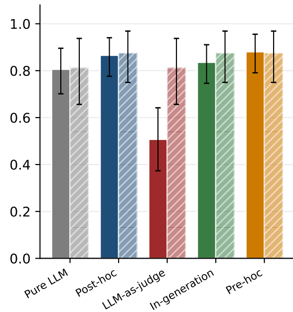
Accuracy
