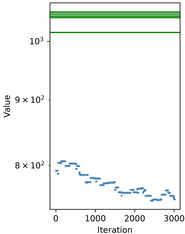
Trace
