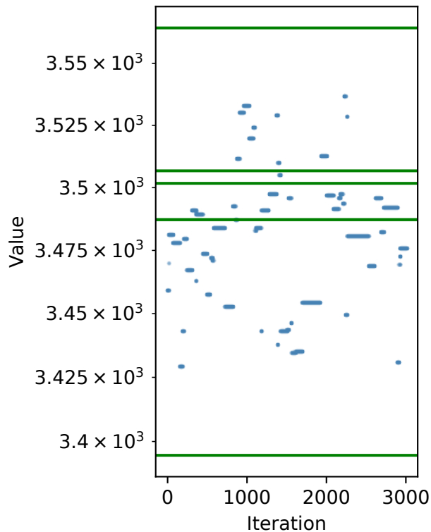
Trace
