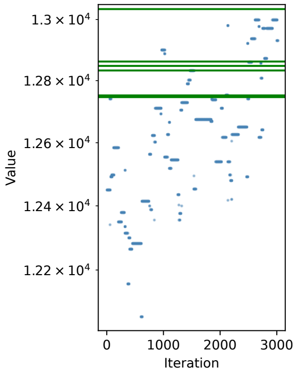
Trace
