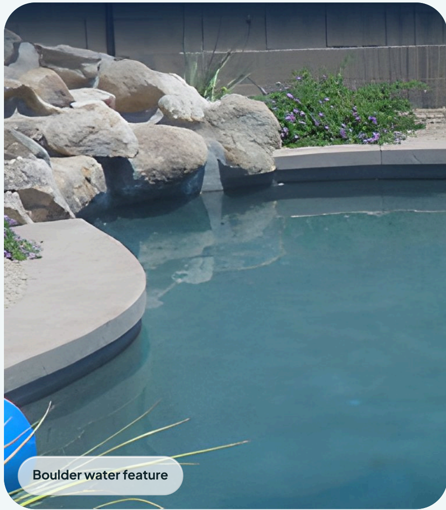
Rock waterfall
