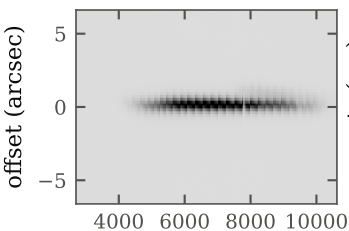
VPH-All, 1.0" longslit
