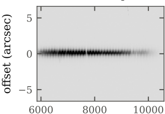
VPH-Red, 1.0" longslit
