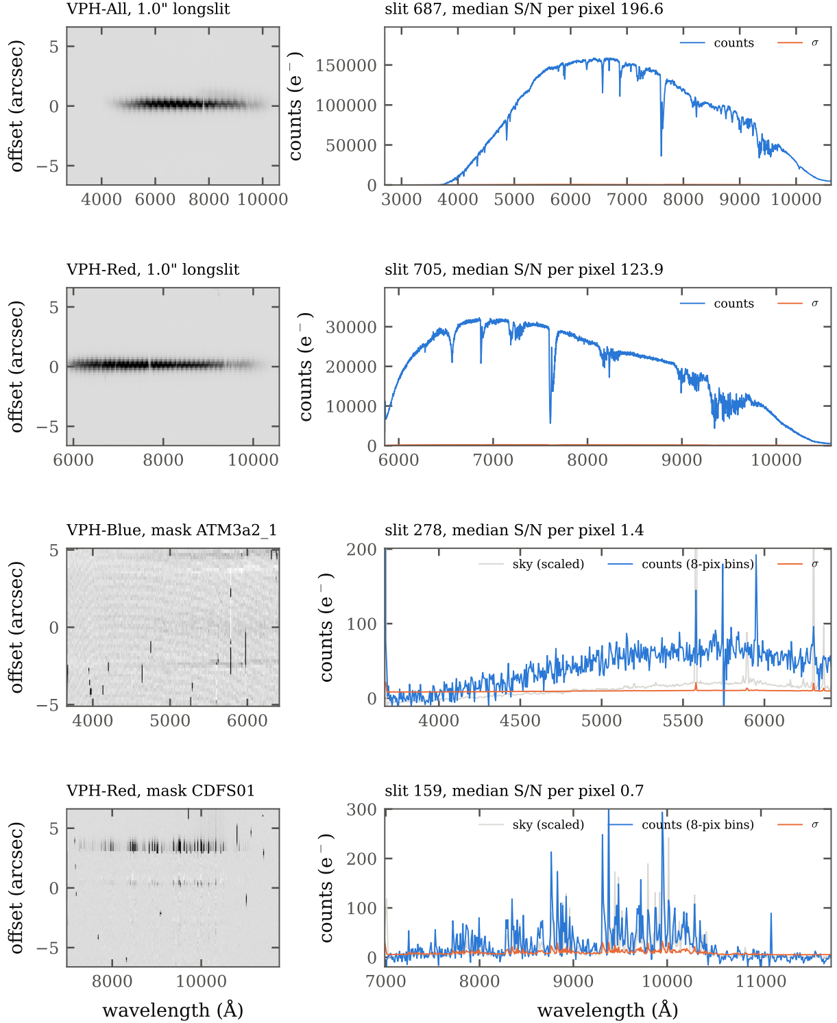
Figure 12: Examples of reduced data. Left: sky-subtracted two-dimensional spectrum around the object, with wavelength increasing to the right. Right: optimally extracted spectrum (blue) and its uncertainty (orange), in electrons, before flux calibration.
