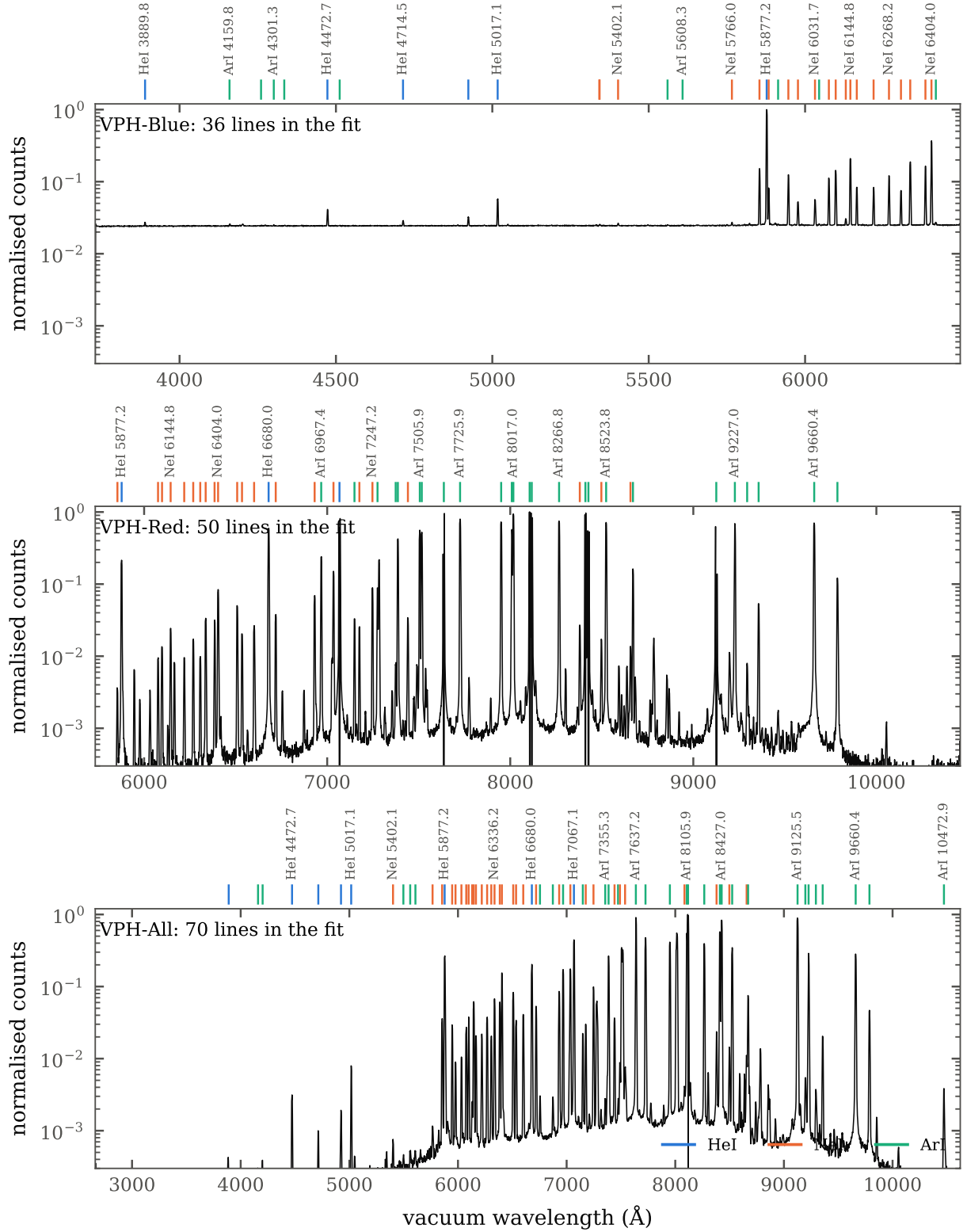
Figure 8: Archived HeNeAr arc templates for the three gratings, with the lines used in the wavelength solution of the longslit data marked by element (HeI blue, NeI orange, ArI green). The brightest lines are labelled with their vacuum wavelength in Å.
