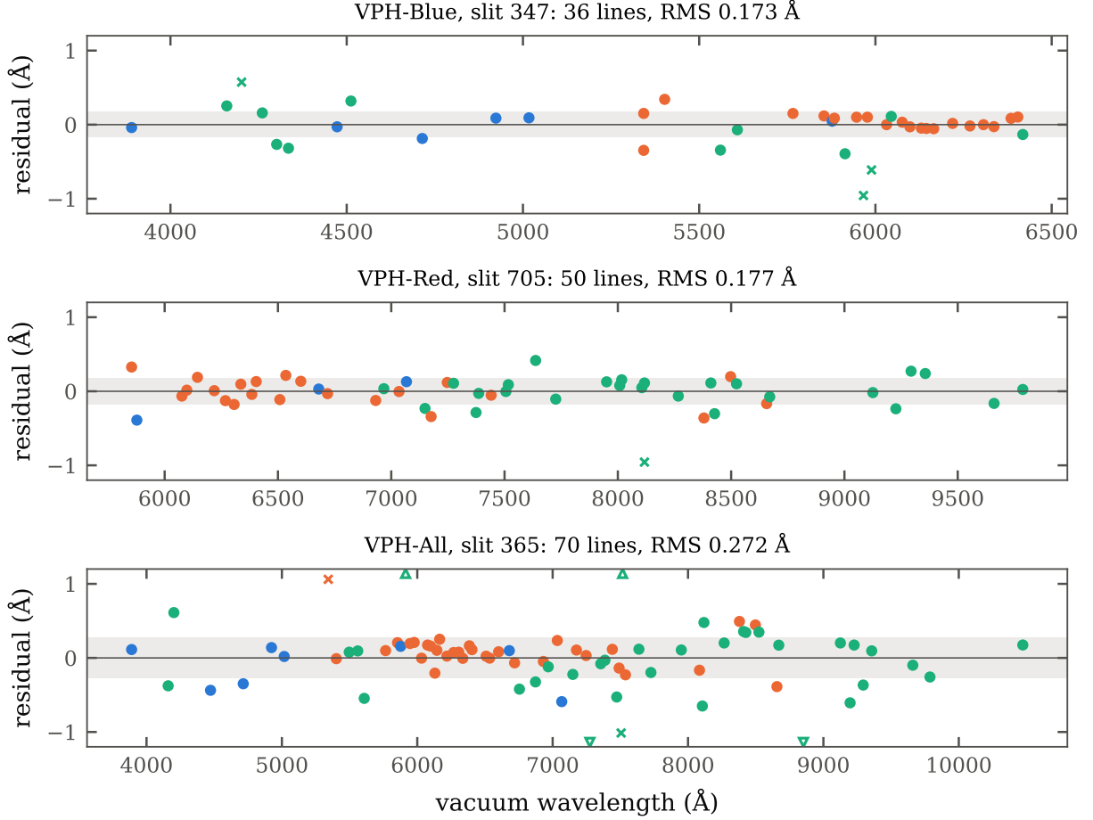
Figure 9: Residuals of the wavelength solutions for the longslit data, for the slit segment with the most identified lines. Filled symbols are lines used in the fit, crosses are rejected lines; the shaded band is \pm RMS.
