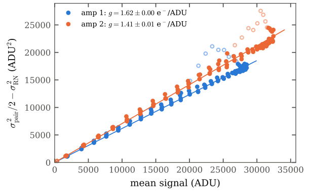
Figure 6: Photon-transfer curve for VPH-All 1.0_center flats of e180403_04 (10s). Filled points are used in the fit; the lines have slope 1/g .
