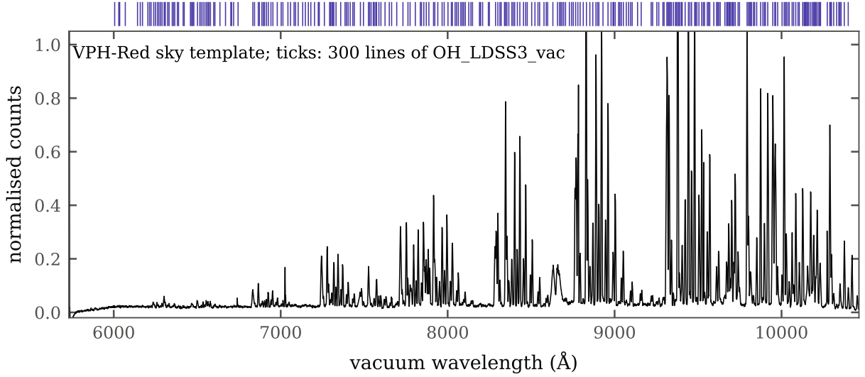
Figure 11: VPH-Red sky template with the positions of the OH_LDSS3_vac lines.
