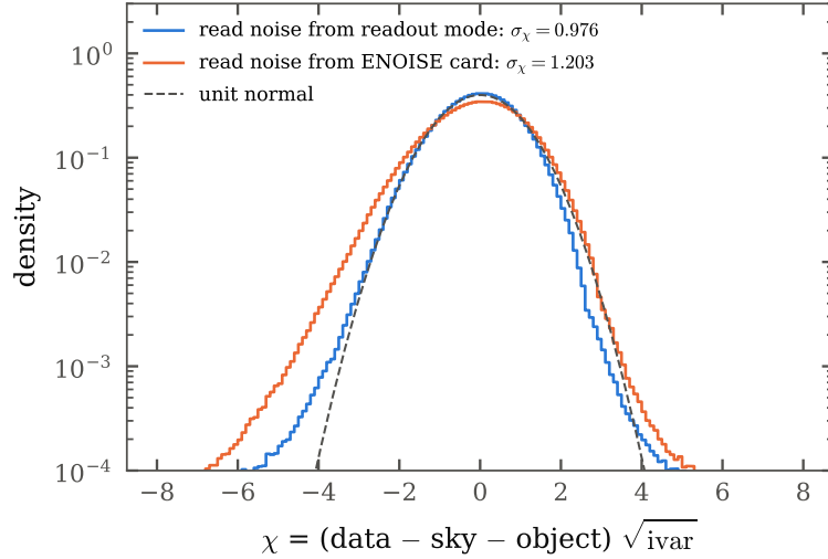
Figure 7: Distribution of the normalised residuals \chi over the good pixels of the science frames in Table 2, for the variance computed with the published read noise (as used by the pipeline) and with the ENOISE header values. The dashed line is a unit normal.
