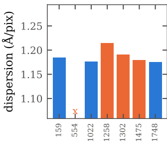
VPH-Red, mask CDFS01
