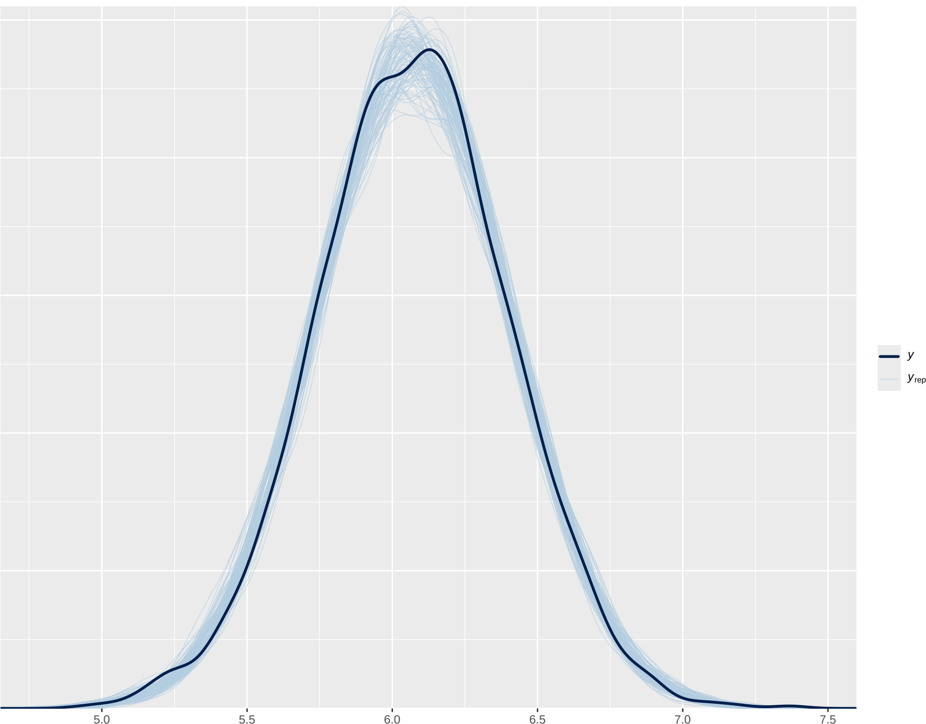
Density overlay: Observed vs. Posterior predictions
