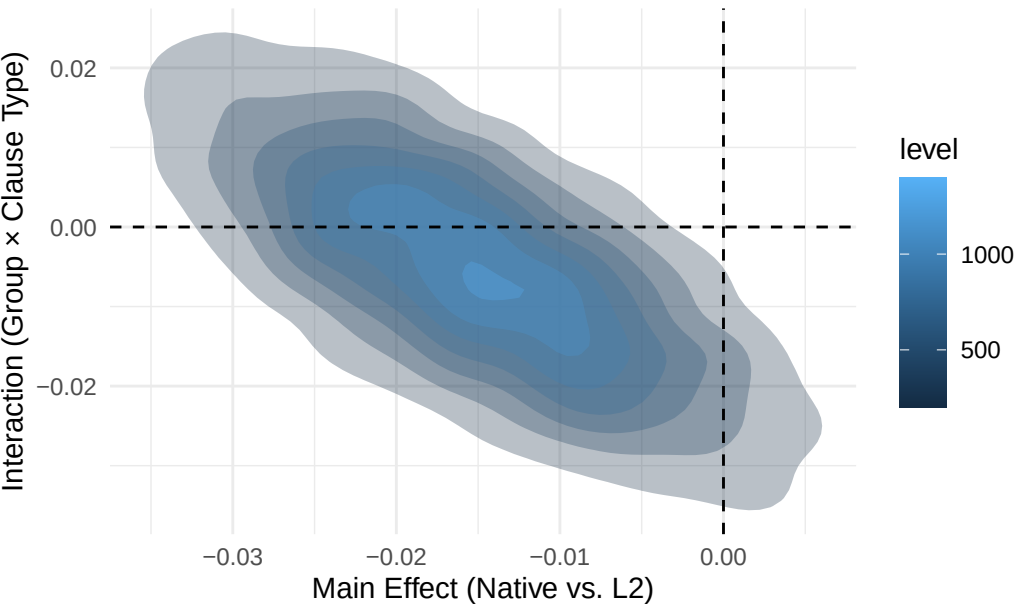
Joint Distribution: Group Effect and Interaction
