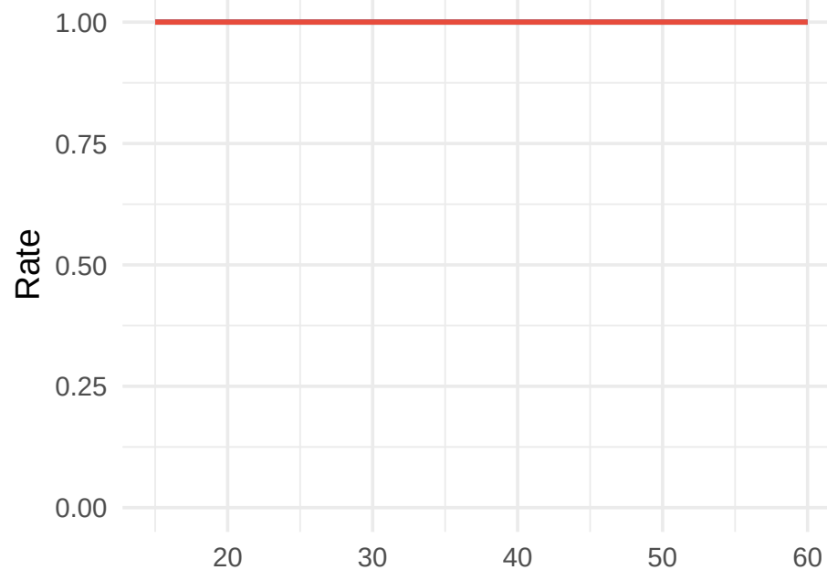
Power (High Noise)
