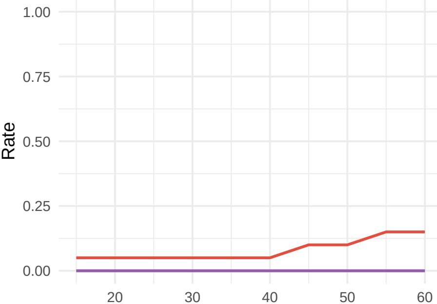
False Positives (High Noise)
