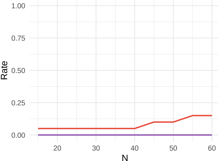
False Positives (High Noise)
