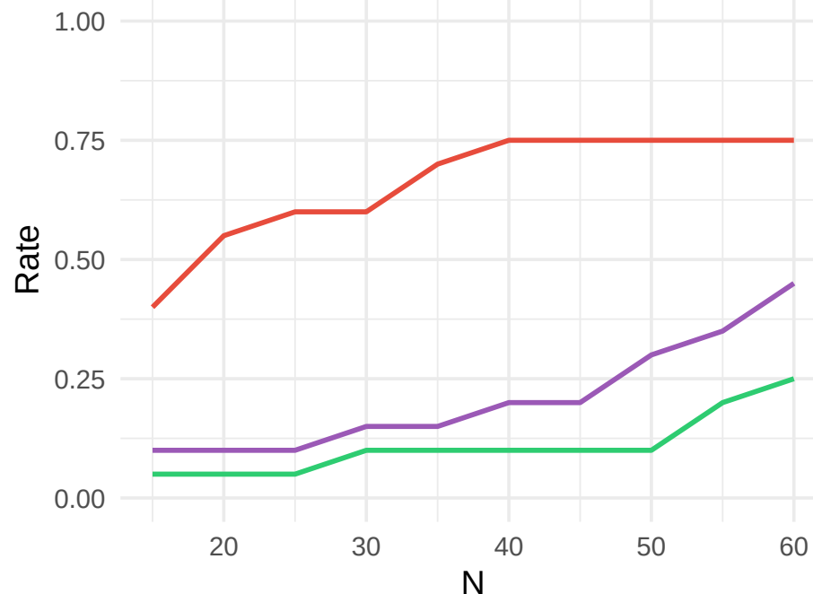
Power (High Noise)
