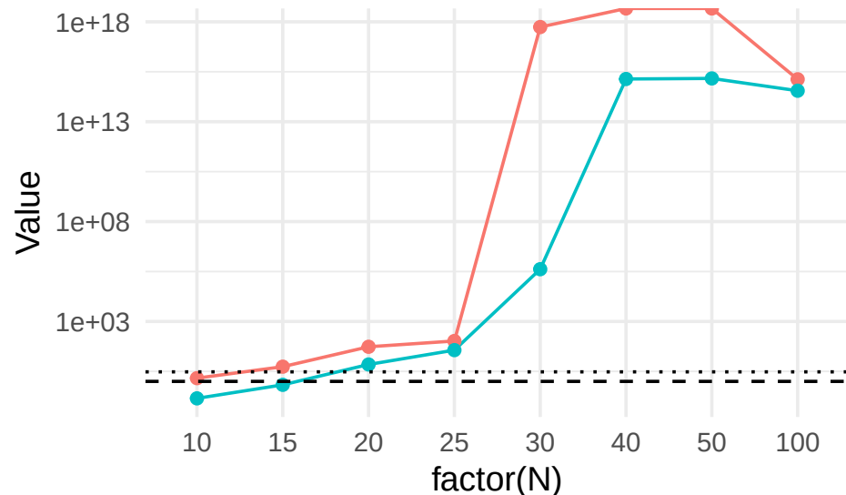
Predictive Gain (LOO)
