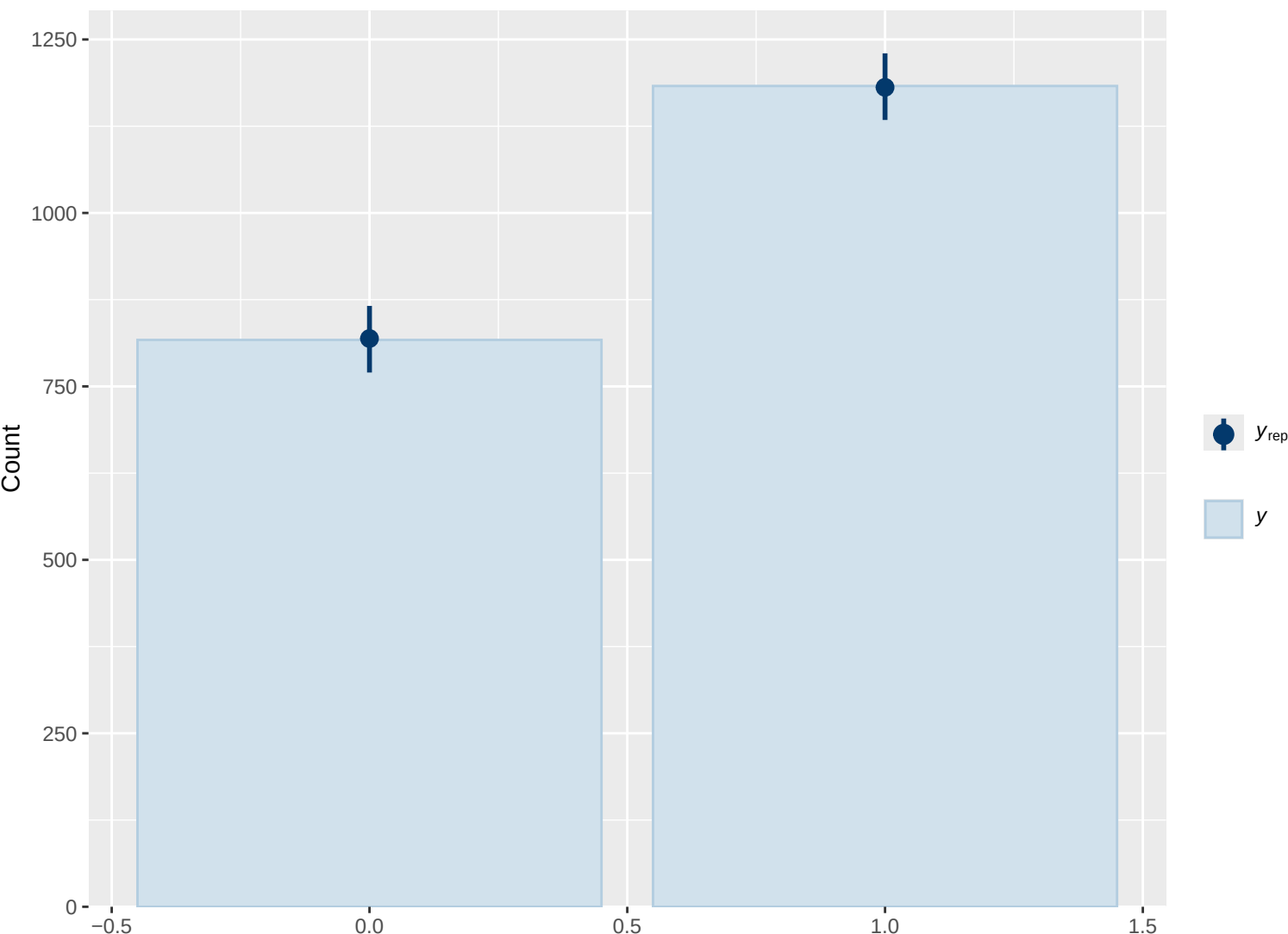
Bar plot: Observed vs. Predicted counts
