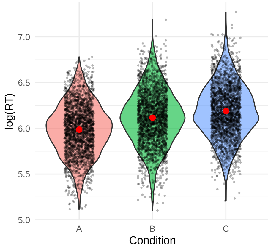
Log-Transformed RTs
