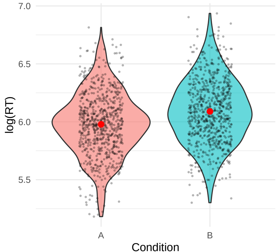
Log-Transformed RTs
