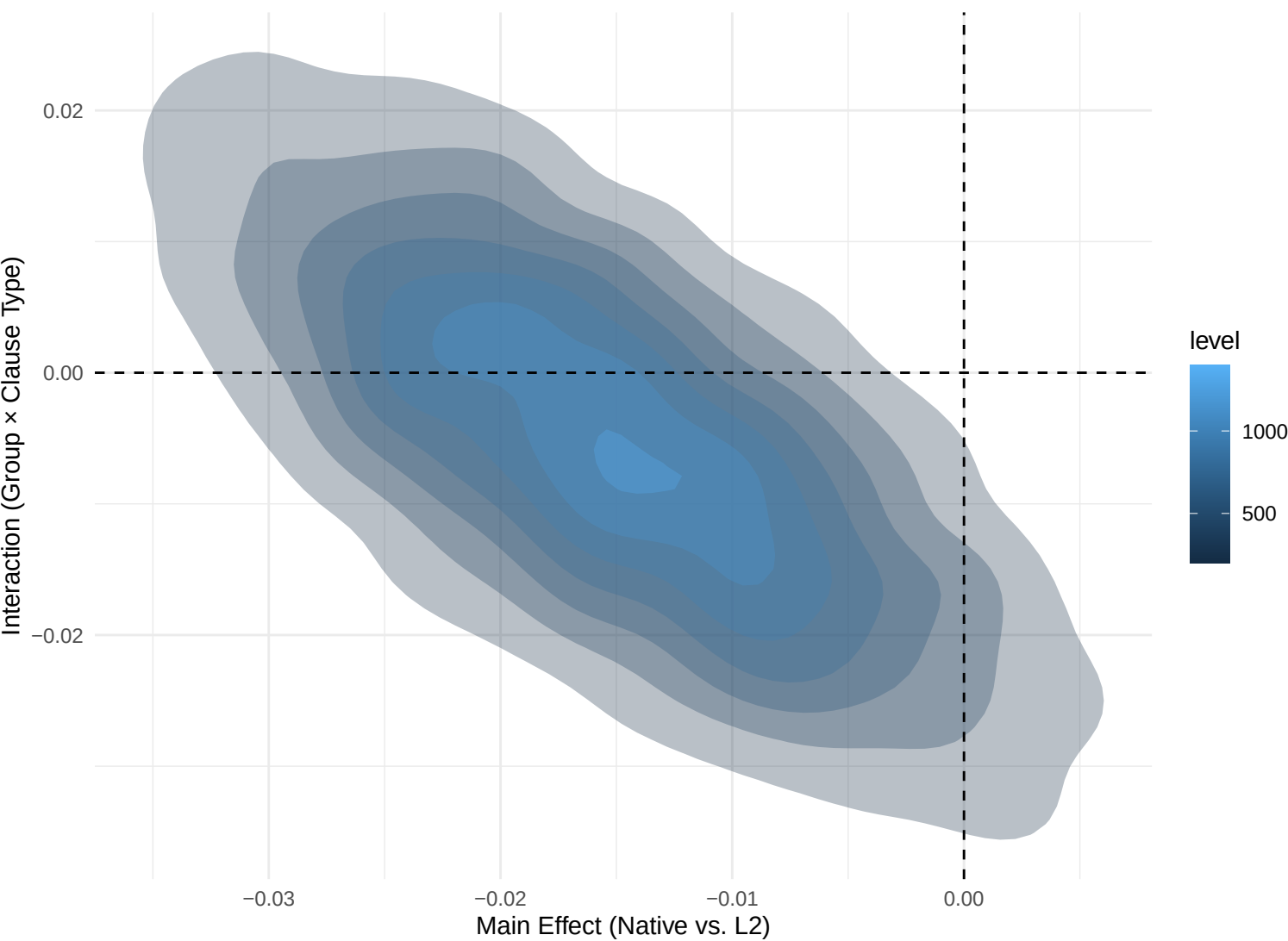
Joint Distribution: Group Effect and Interaction
