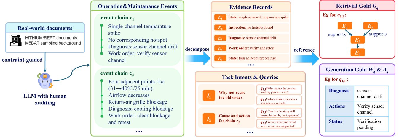
Fig. 2. Construction pipeline and example for TEF-RAG v6 Semantic Benchmark v1. Public sources constrain the equipment and data background; an O&M event chain c is then constructed and used to derive evidence records e_i , task intents I_j , and queries q_{j,p} . Retrieval reference evidence flows and structured generation reference answers are subsequently created for each query to support retrieval and downstream generation evaluation.
