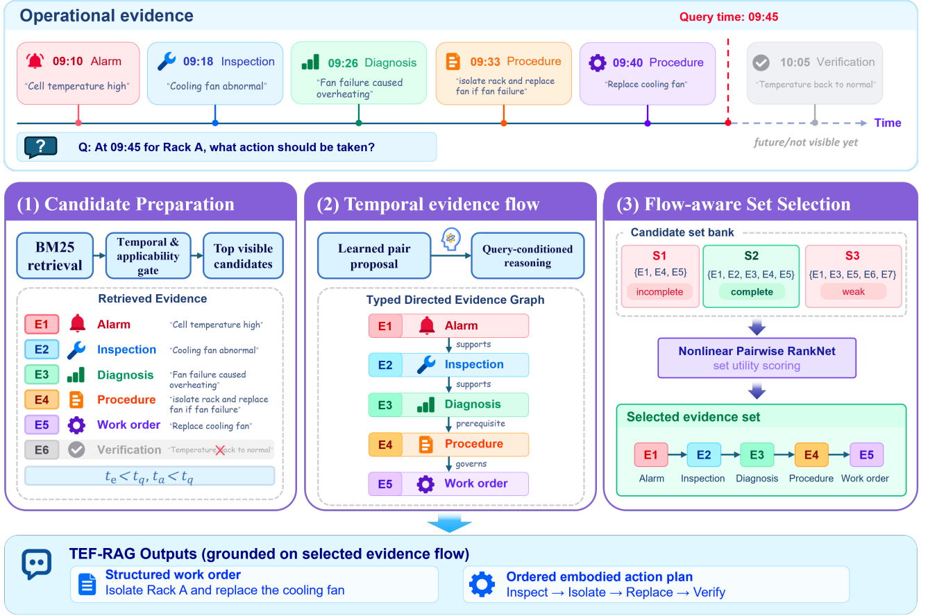
Fig. 1. Overview of TEF-RAG. The system first selects candidate evidence pairs from records that are legal at the query time, then constructs a query-conditioned Temporal Evidence Flow. A nonlinear pairwise ranker selects at most five records from the candidate-set space as the evidence flow, which is then used as controlled context for a shared downstream generator.
