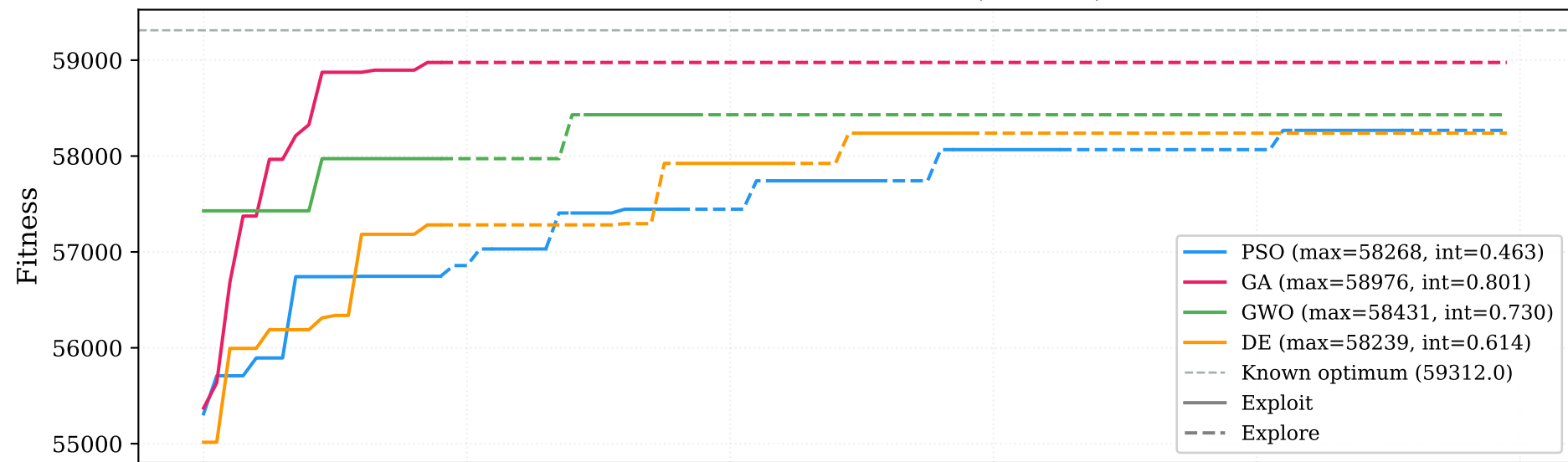
B3 D2-Direct — All MHs (seed=3)
