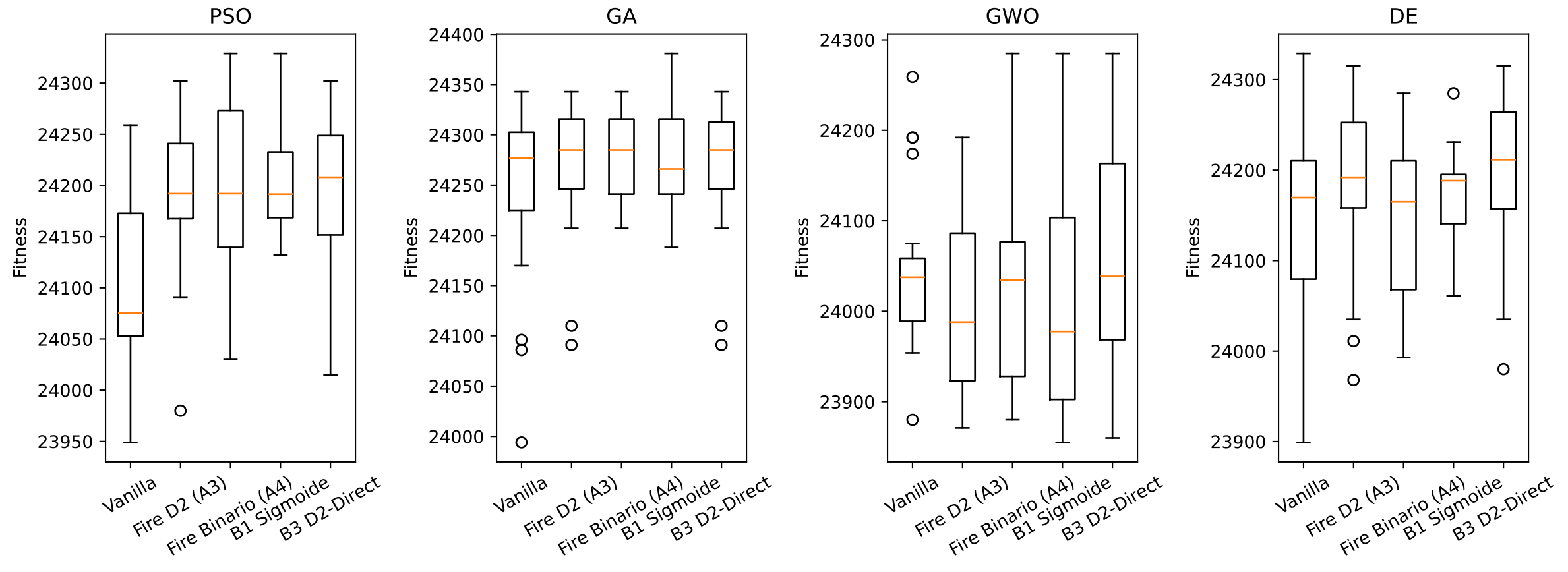
DTW Adaptations vs Vanilla — mknapcb1[0] — Fitness Distribution
