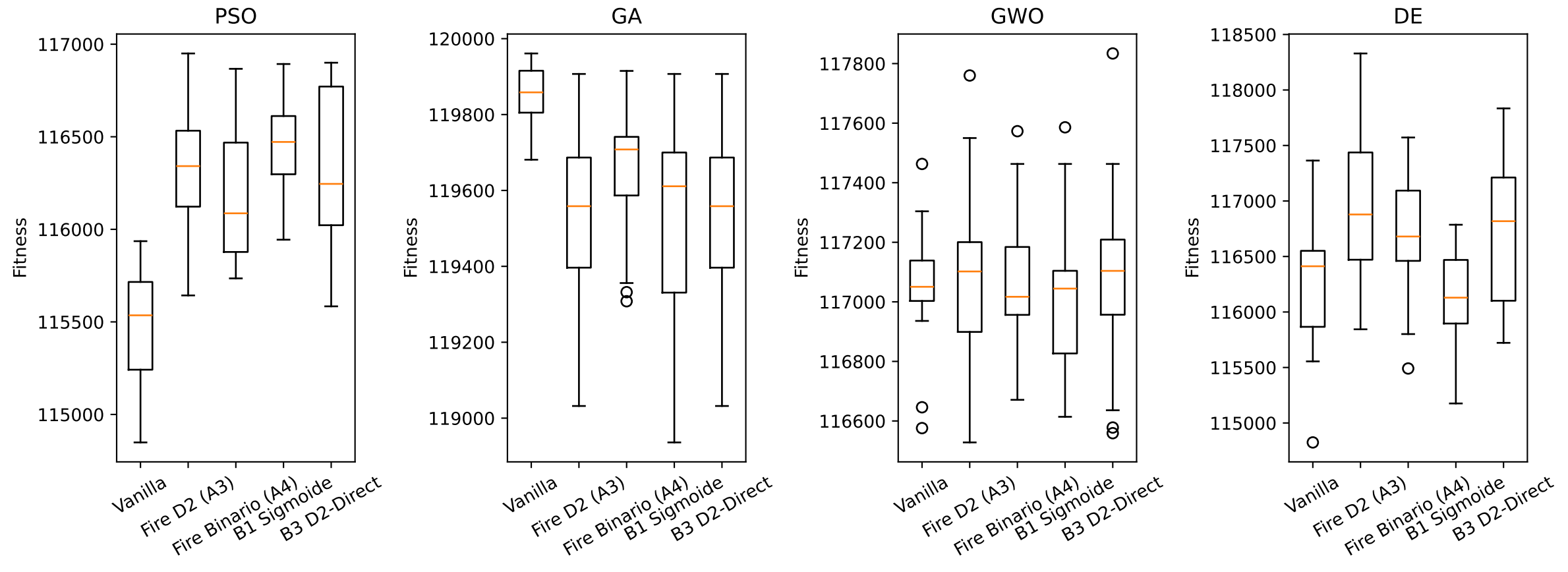
DTW Adaptations vs Vanilla — mknapcb3[0] — Fitness Distribution
