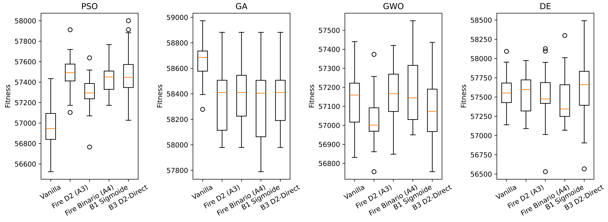
DTW Adaptations vs Vanilla — mknapcb5[0] — Fitness Distribution
