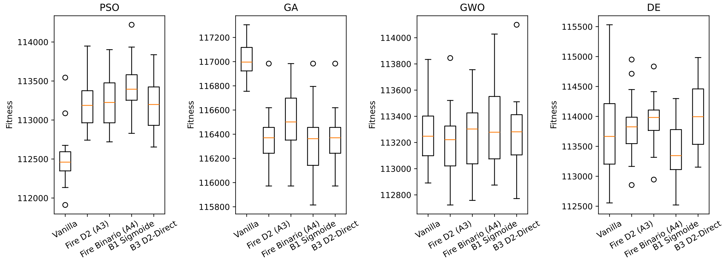
DTW Adaptations vs Vanilla — mknapcb6[0] — Fitness Distribution
