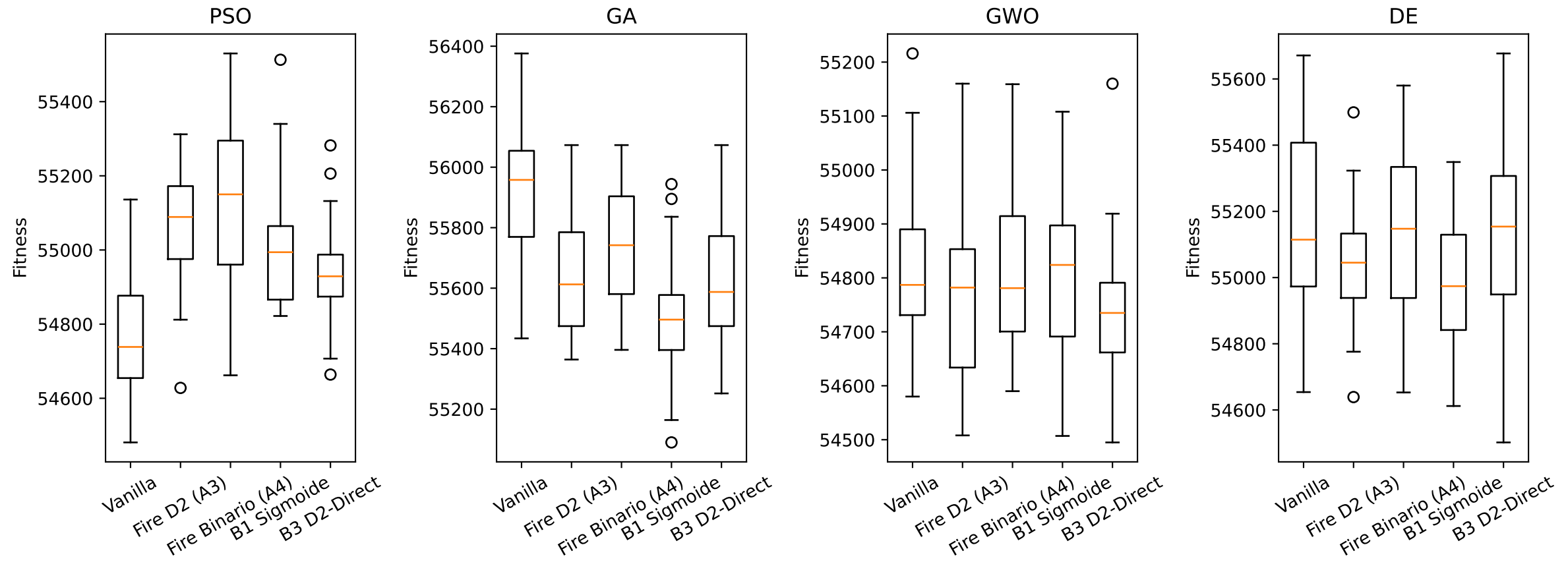
DTW Adaptations vs Vanilla — mknapcb8[0] — Fitness Distribution
