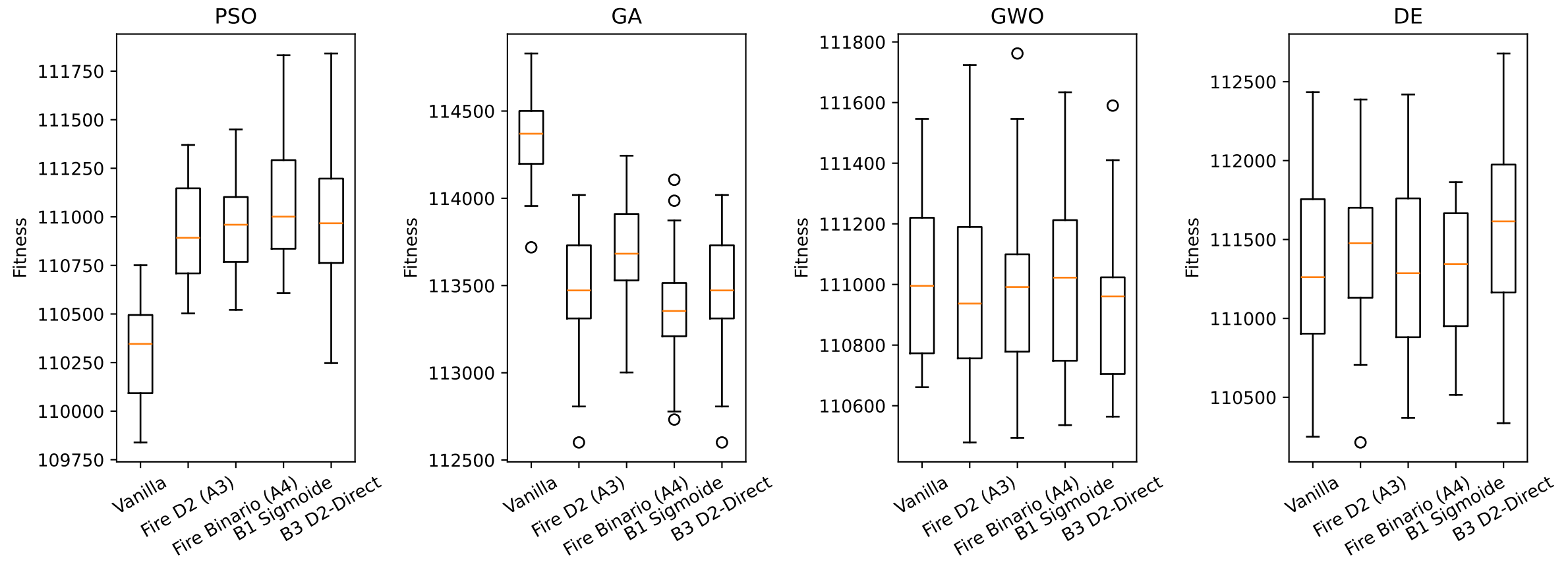
DTW Adaptations vs Vanilla — mknapcb9[0] — Fitness Distribution
