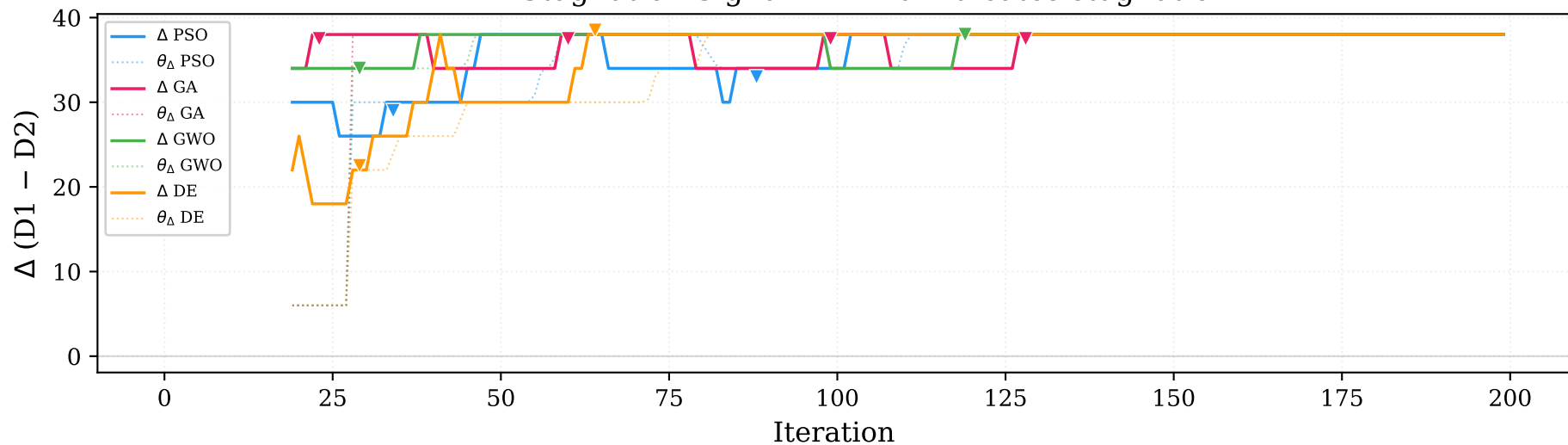
DTW Stagnation Signal — \Delta > 0 indicates stagnation
