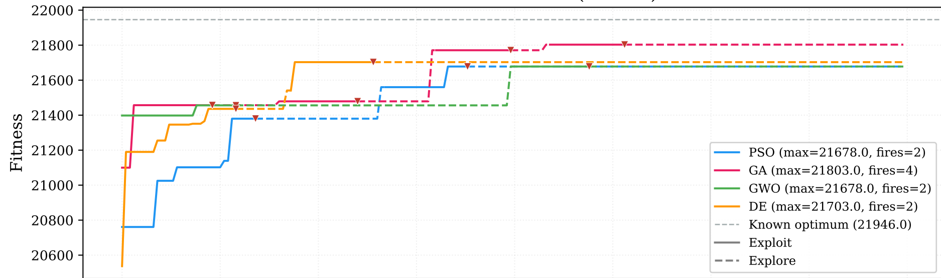
Fire binario — All MHs (seed=1)
