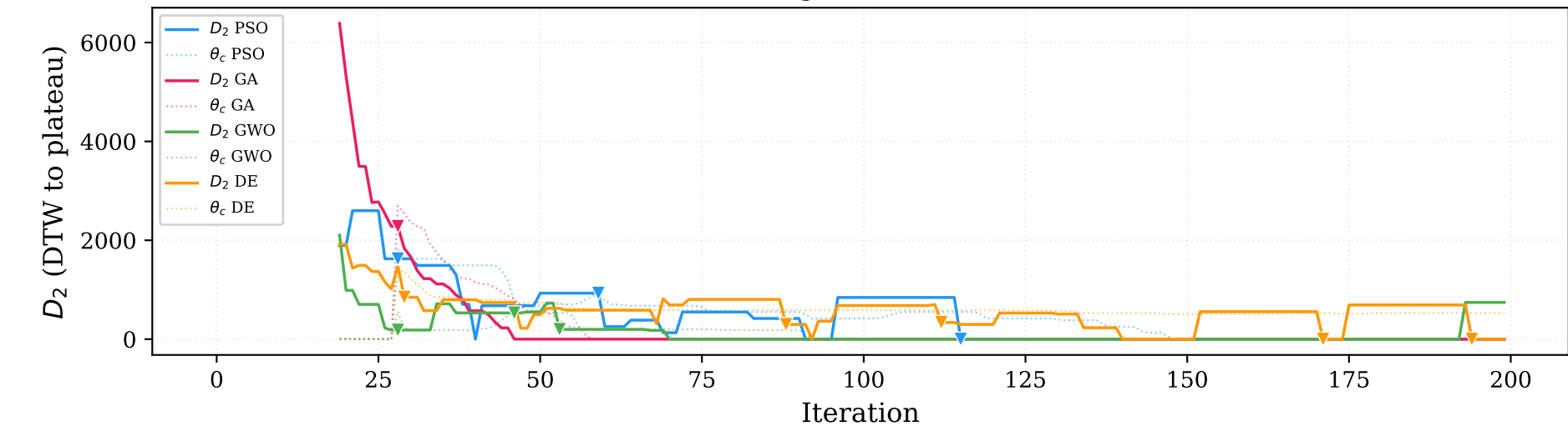
DTW Decision Signal — Fire when D_2 \leq \theta_c
