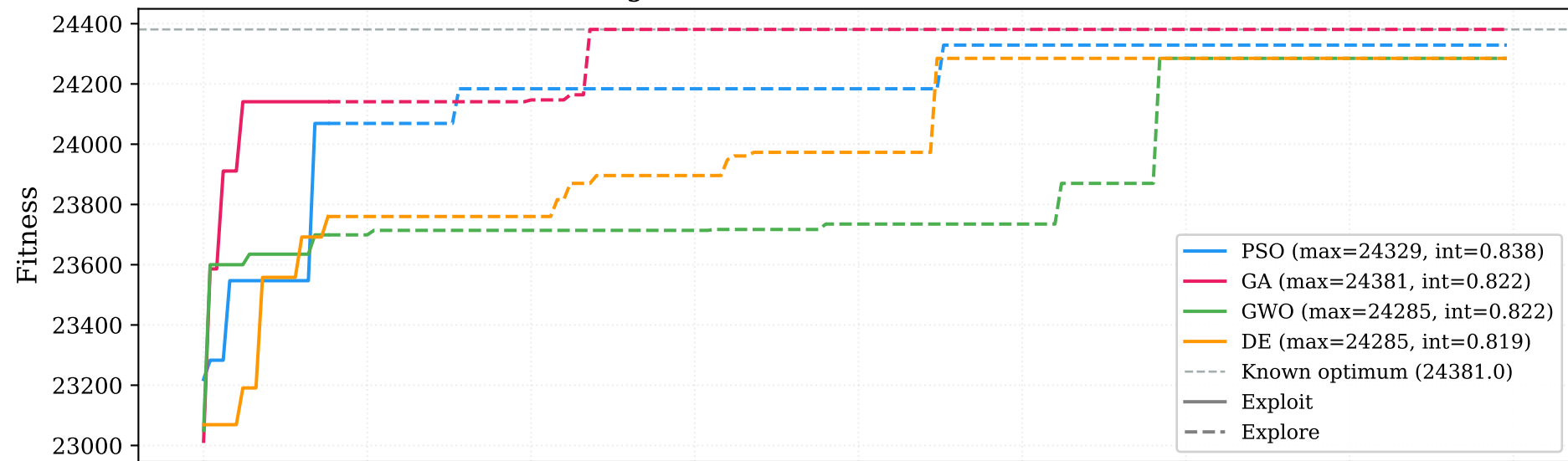
Sigmoid Delta — All MHs (seed=1)
