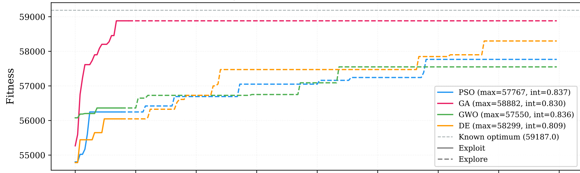
Sigmoid Delta — All MHs (seed=1)
