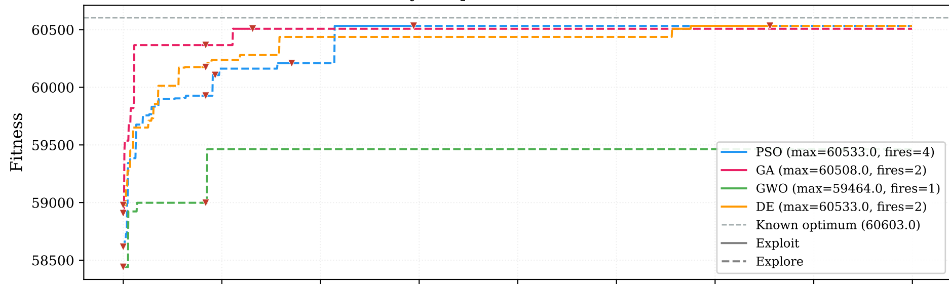
Binary-Simple — All MHs (seed=1)
