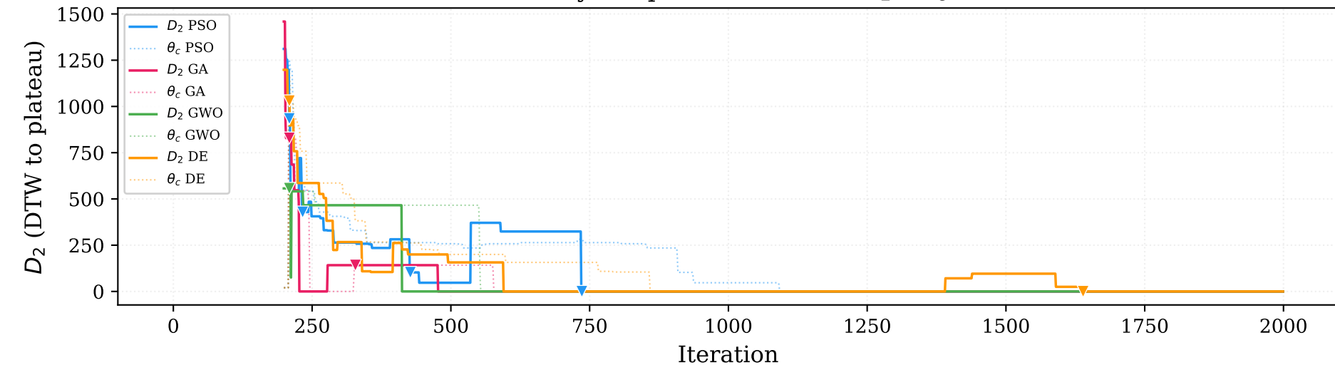
Binary-Simple — Fire when D_2 \leq \theta_c
