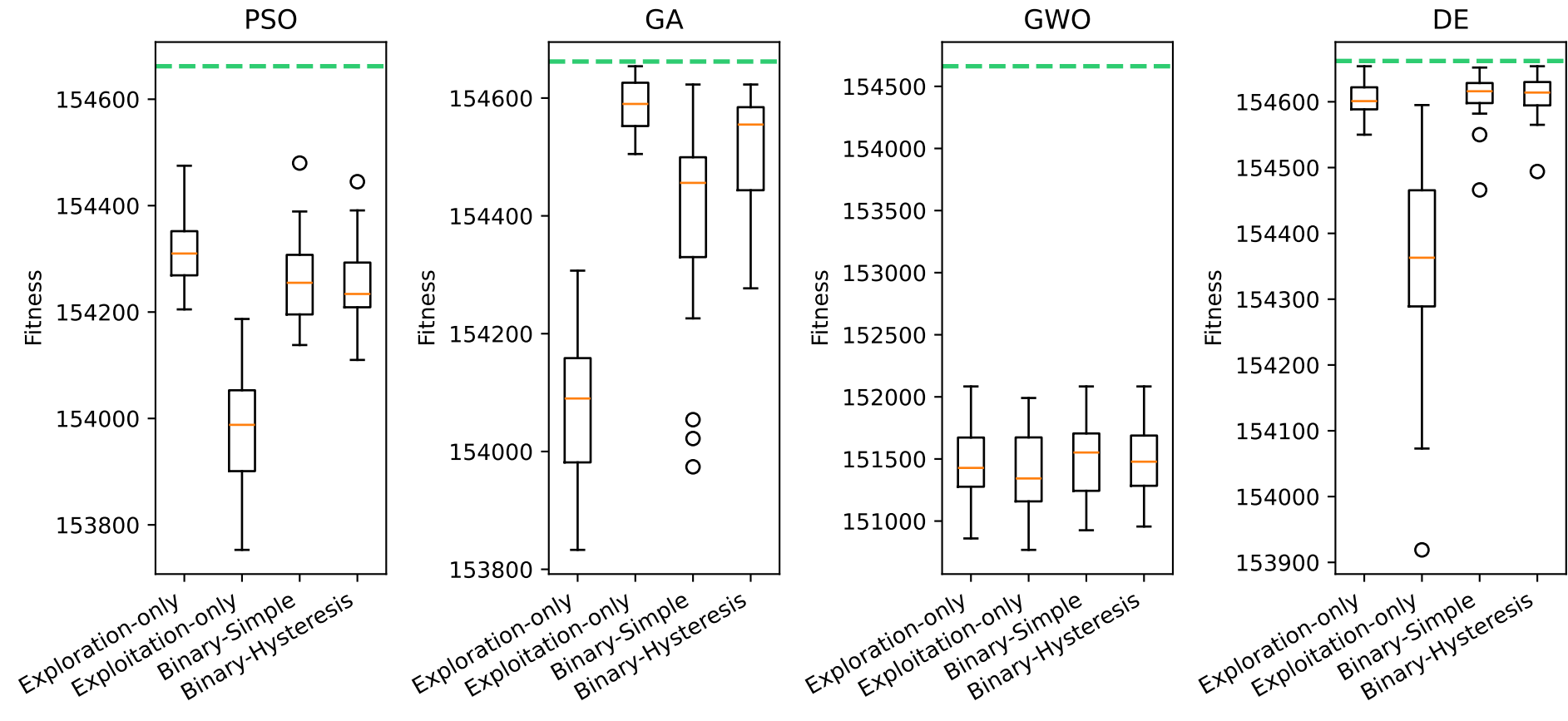
Fitness distribution across MH variants — mknapcb2[29] (opt=154662)
