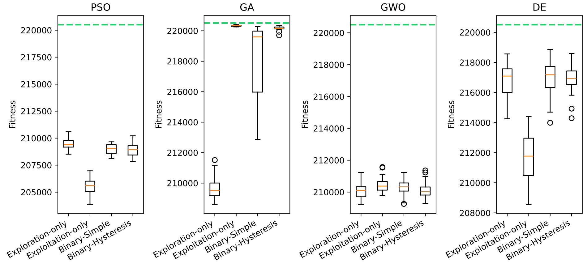
Fitness distribution across MH variants — mknapcb3[15] (opt=220514)
