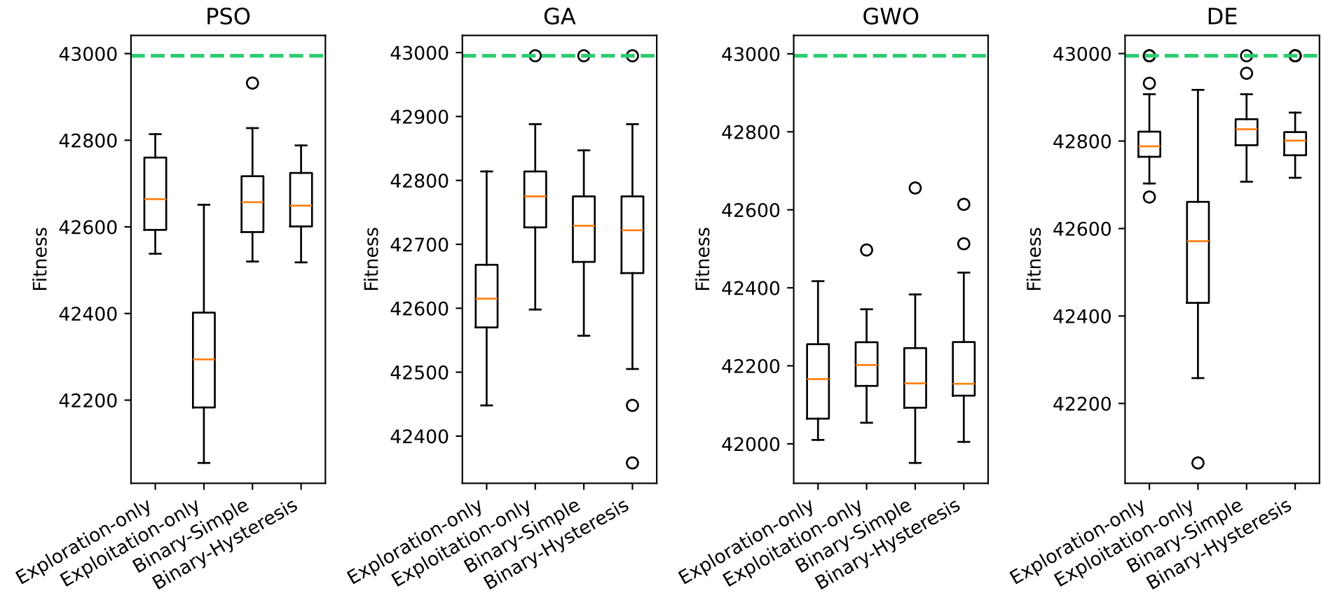
Fitness distribution across MH variants — mknapcb4[15] (opt=42995)
